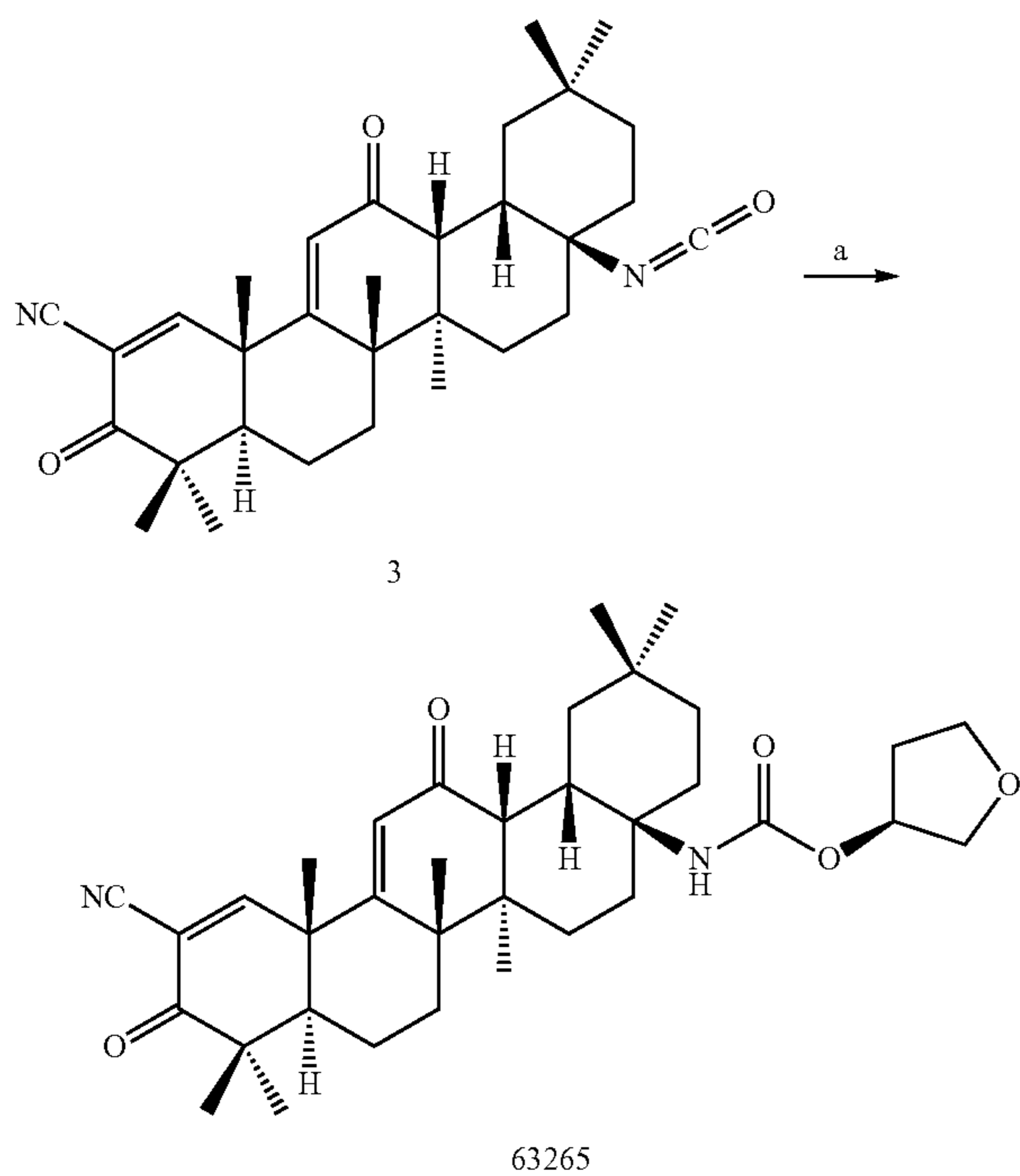
Scheme 10:
