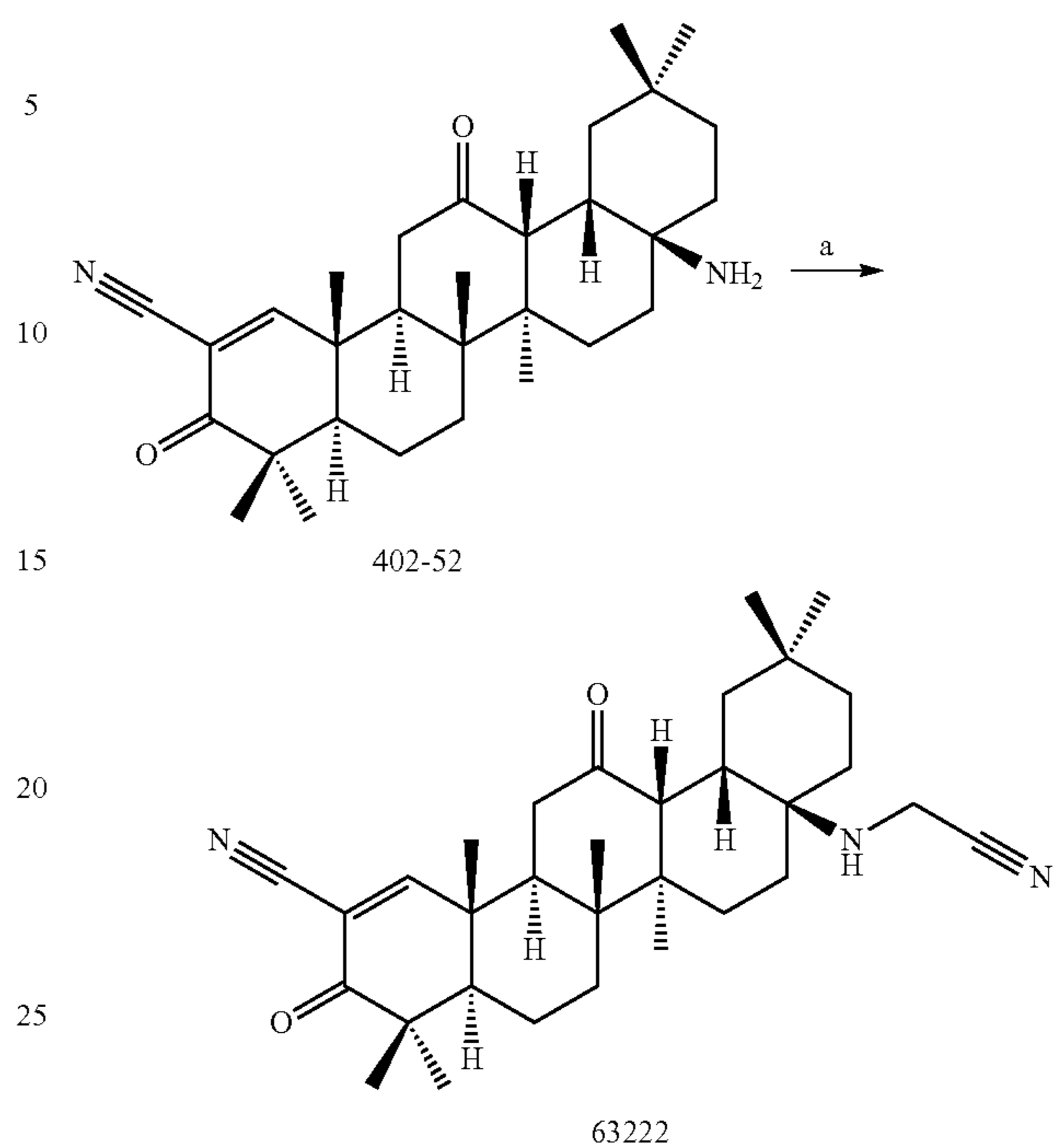
Scheme 12:
