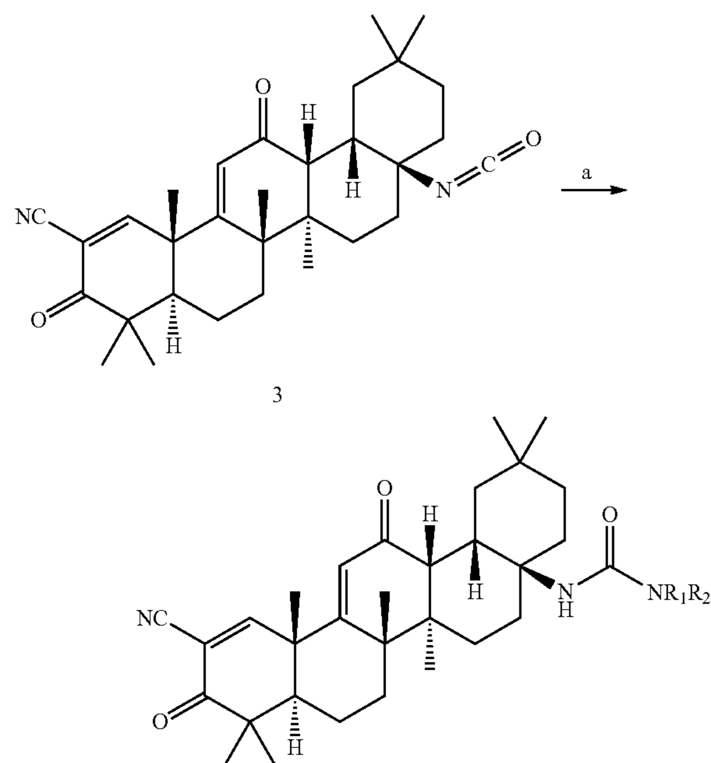
Scheme 7:
