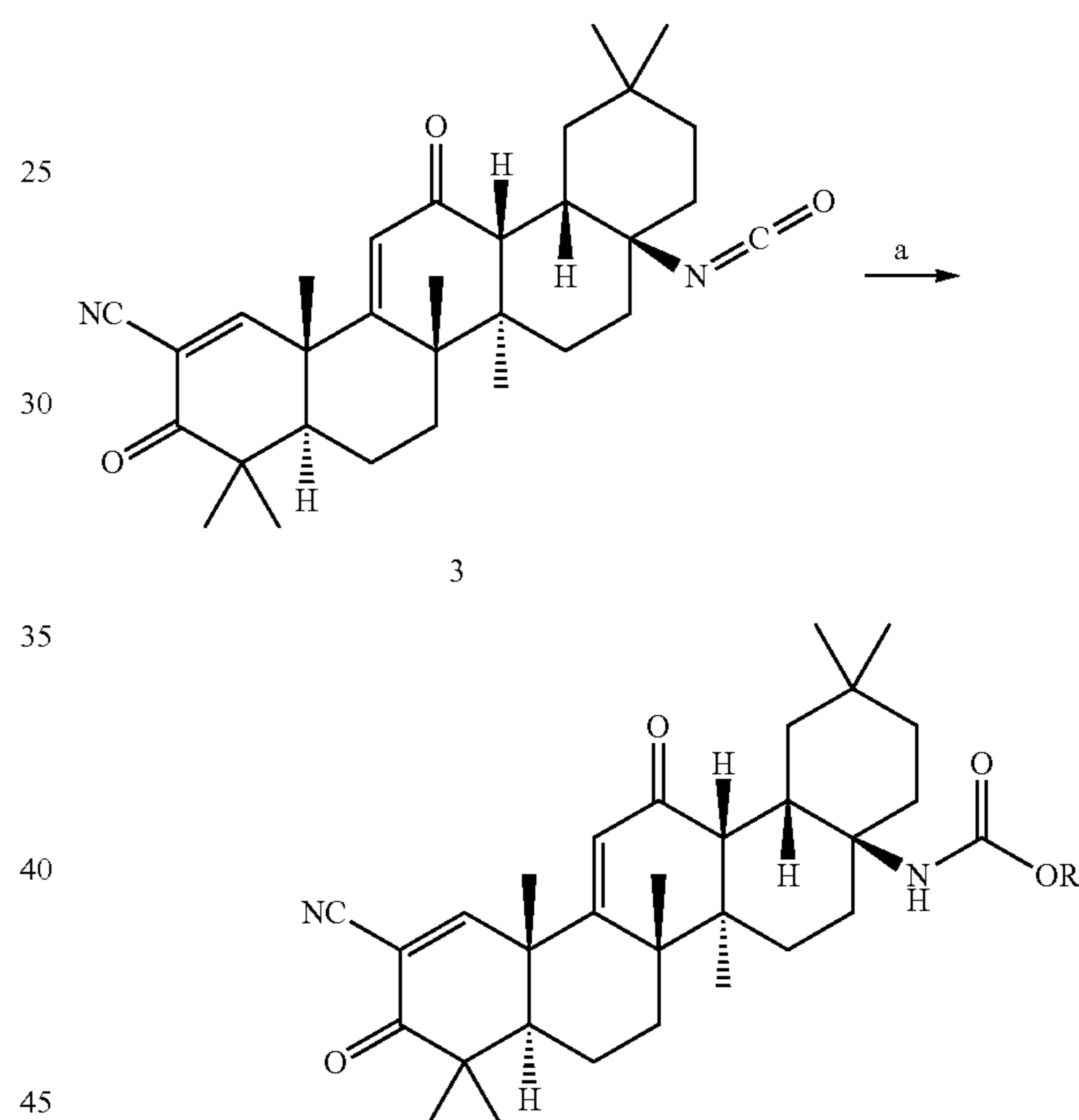
Scheme 8:
