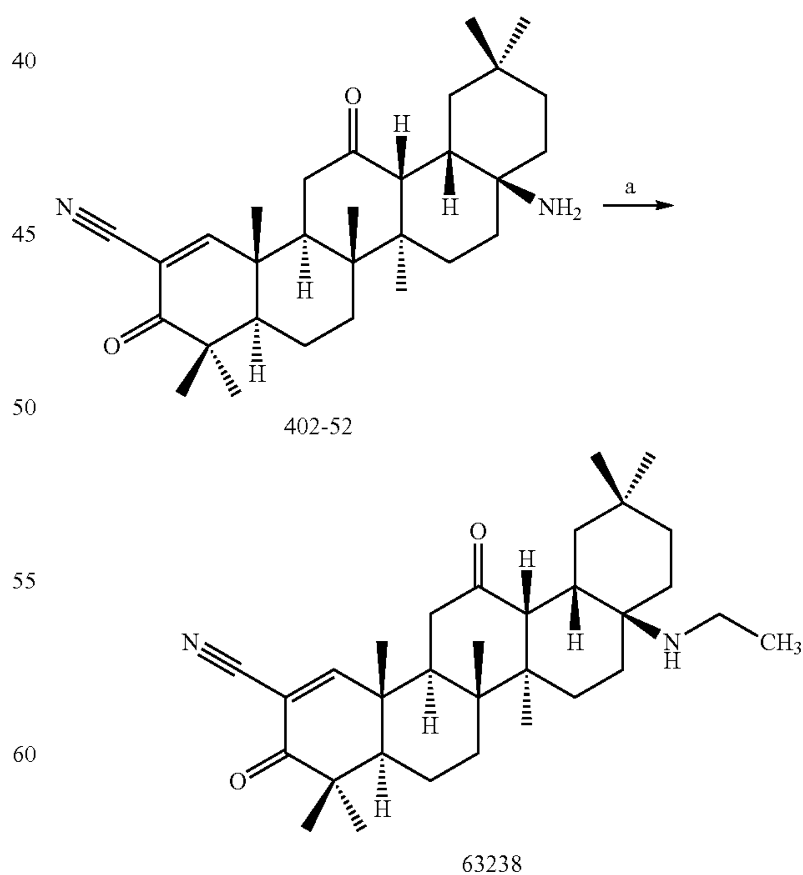
Scheme 13:
