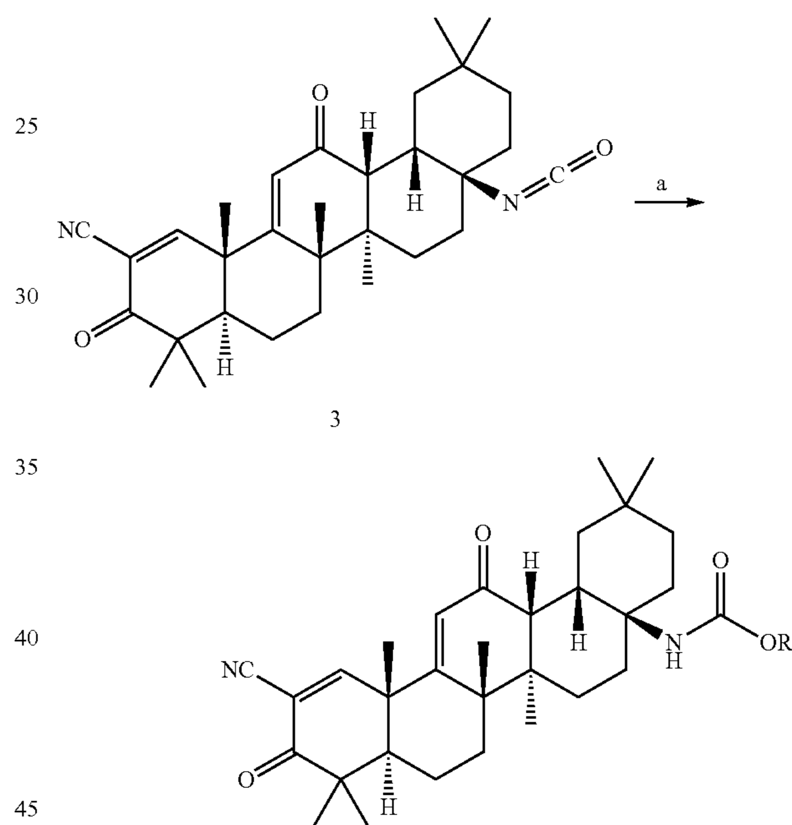
Scheme 8:
