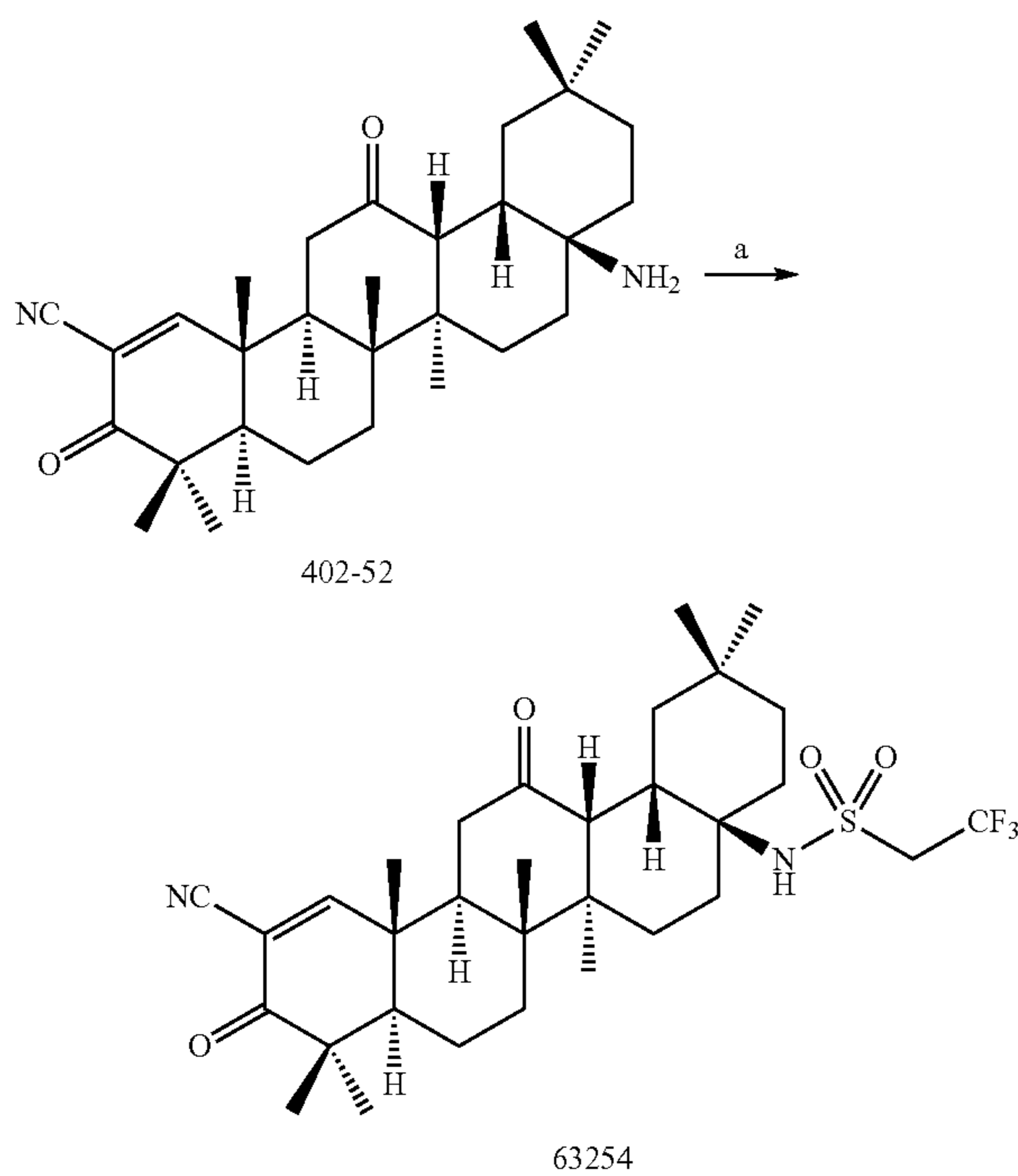
Scheme 11:
