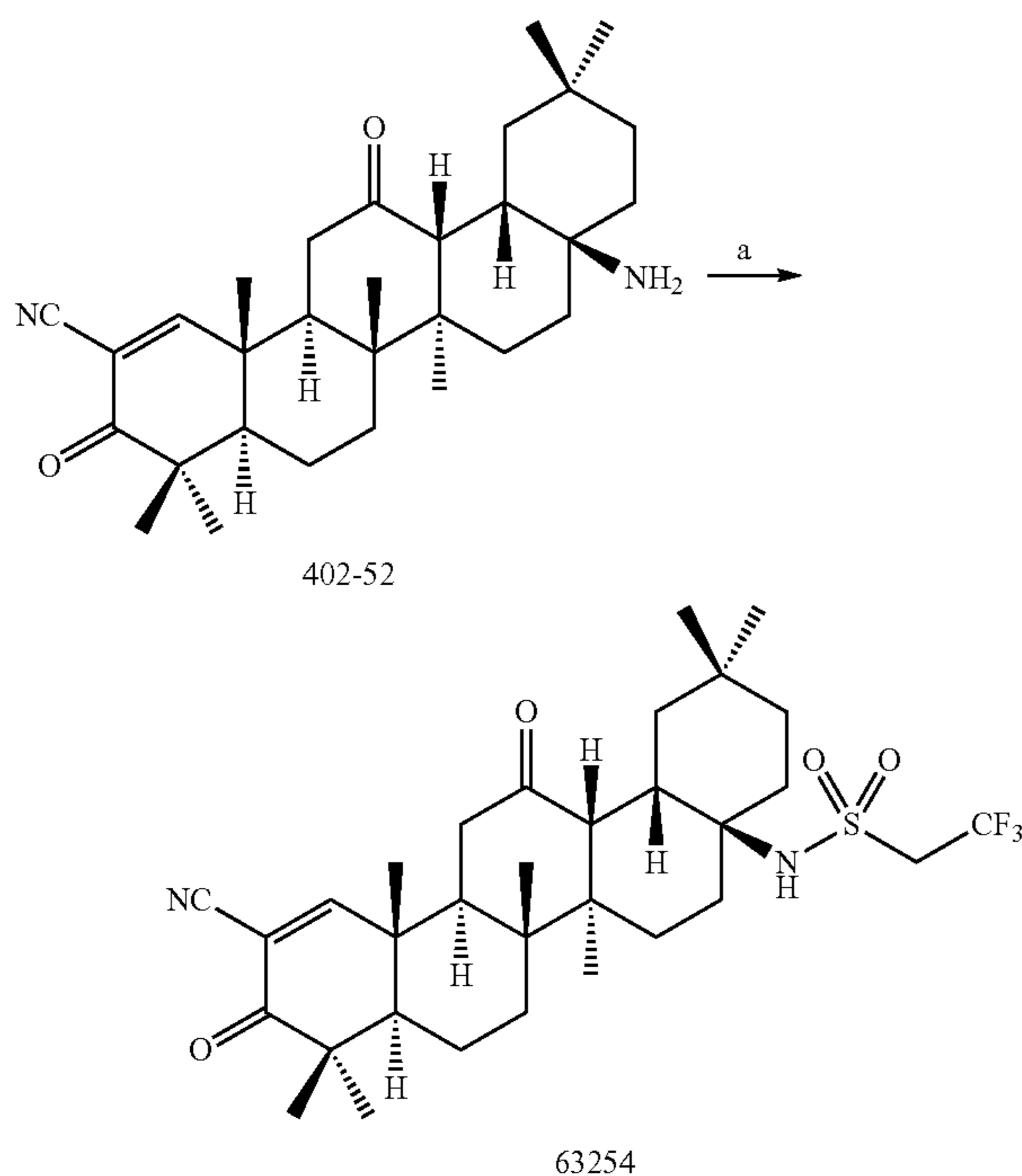
Scheme 11:
