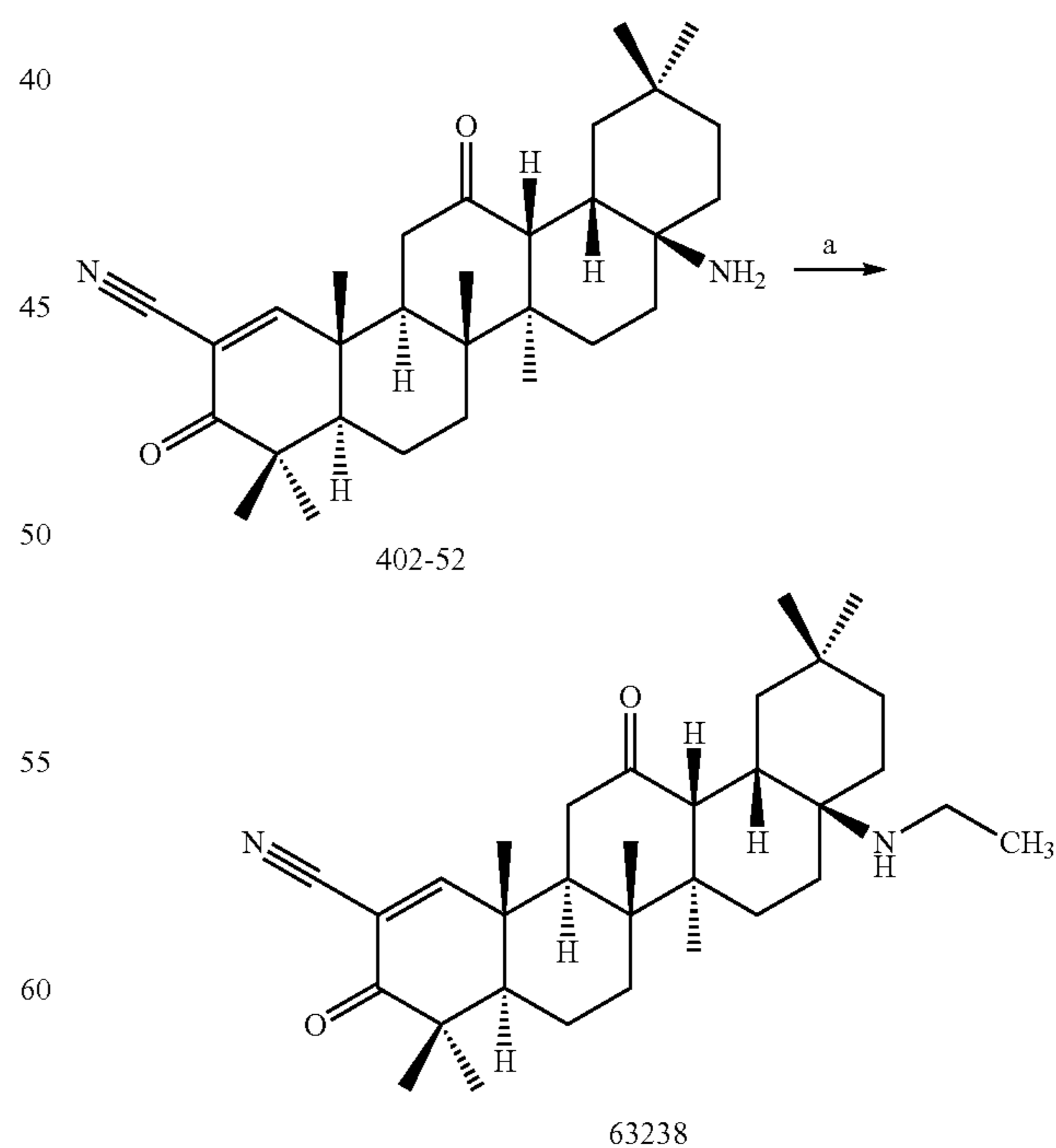
Scheme 13:
