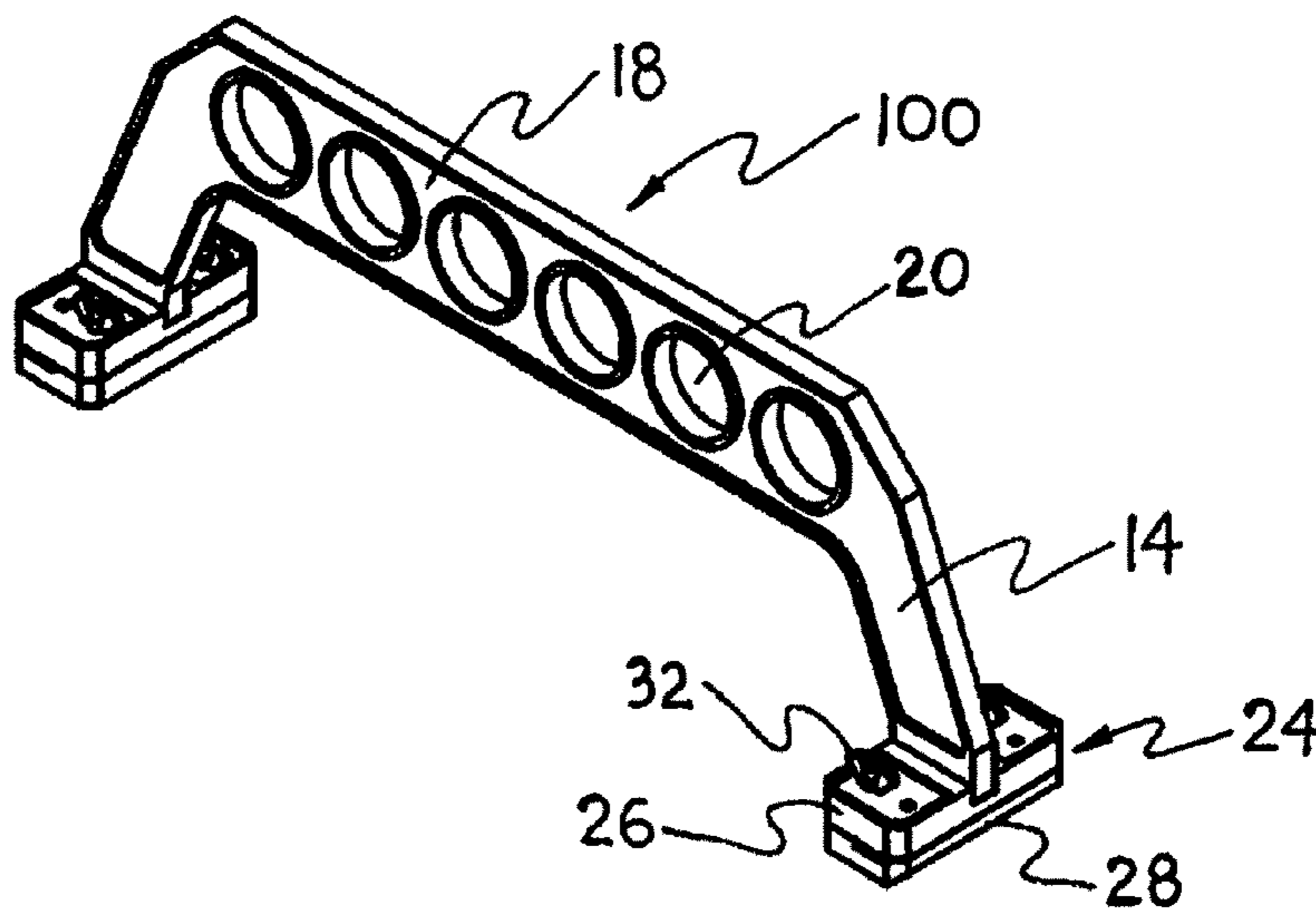
ISOMETRIC VIEW
