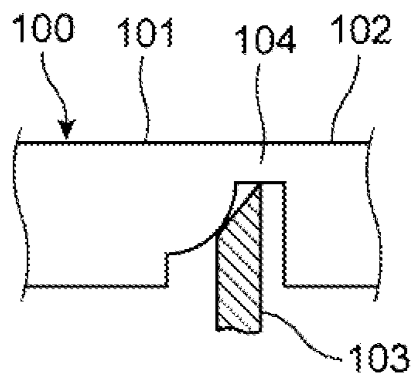
FIG. 11C - PRIOR ART
