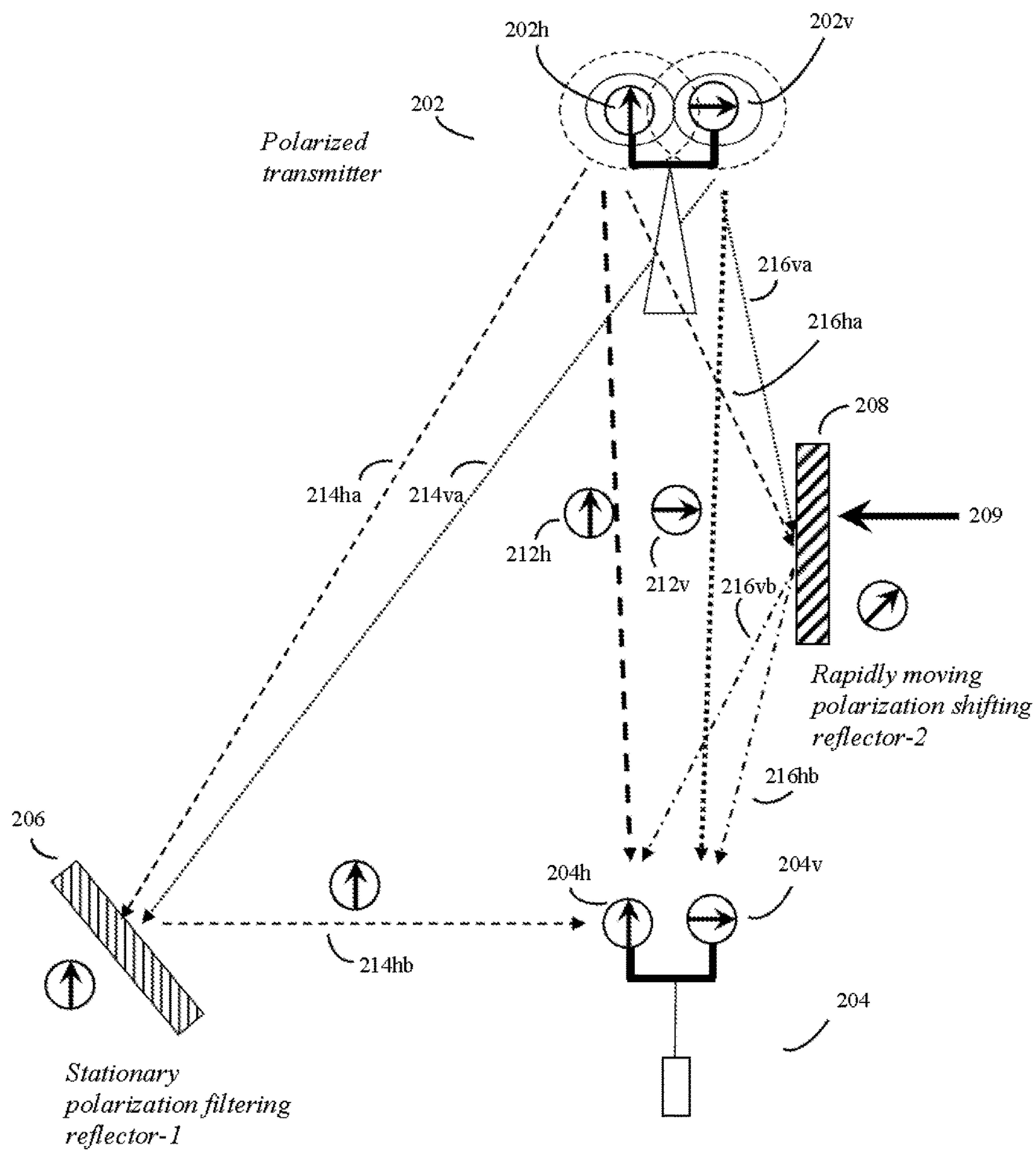
Figure 2A polarization
