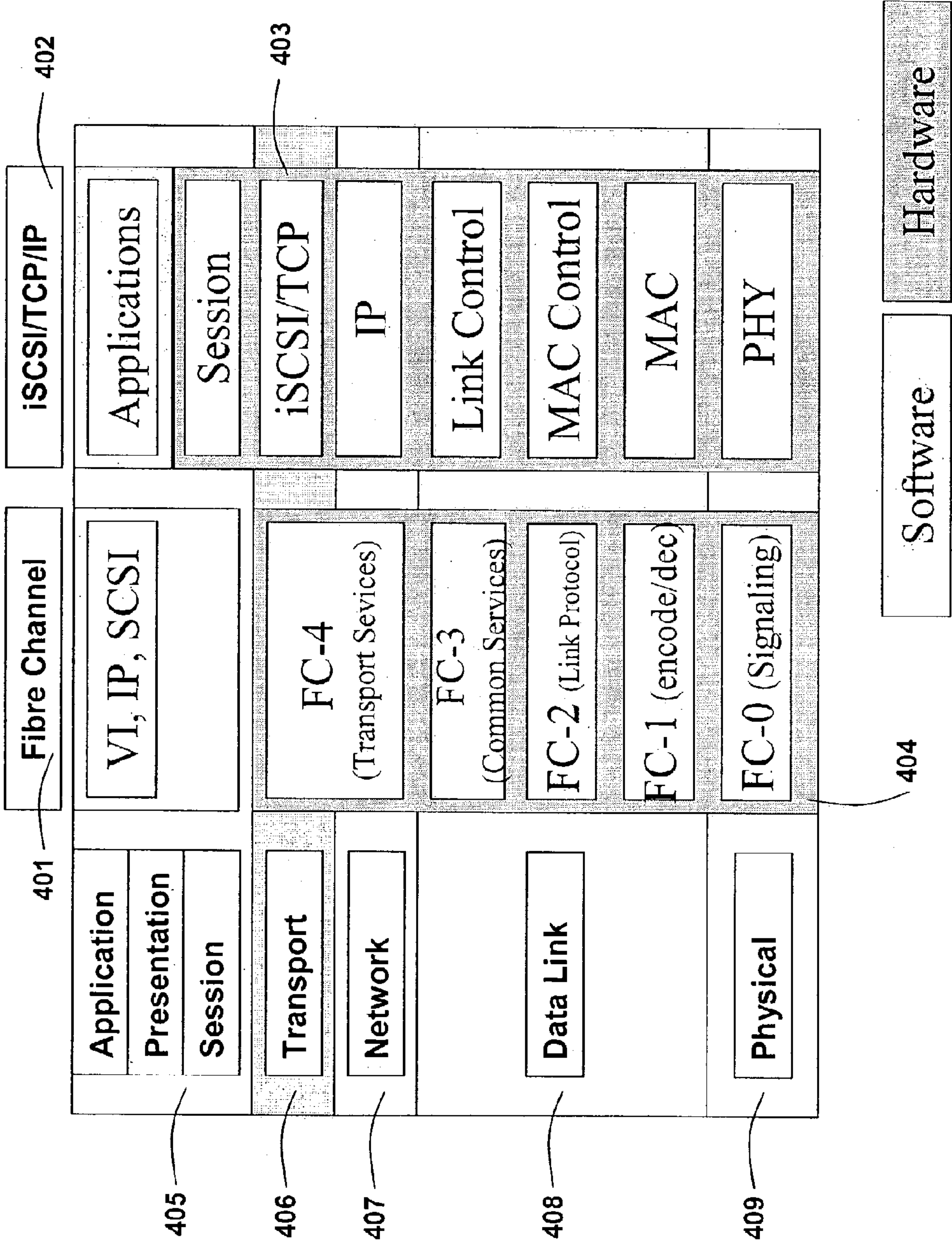
Fig. 4 OSI Stack (w/ HW TCP/IP)
