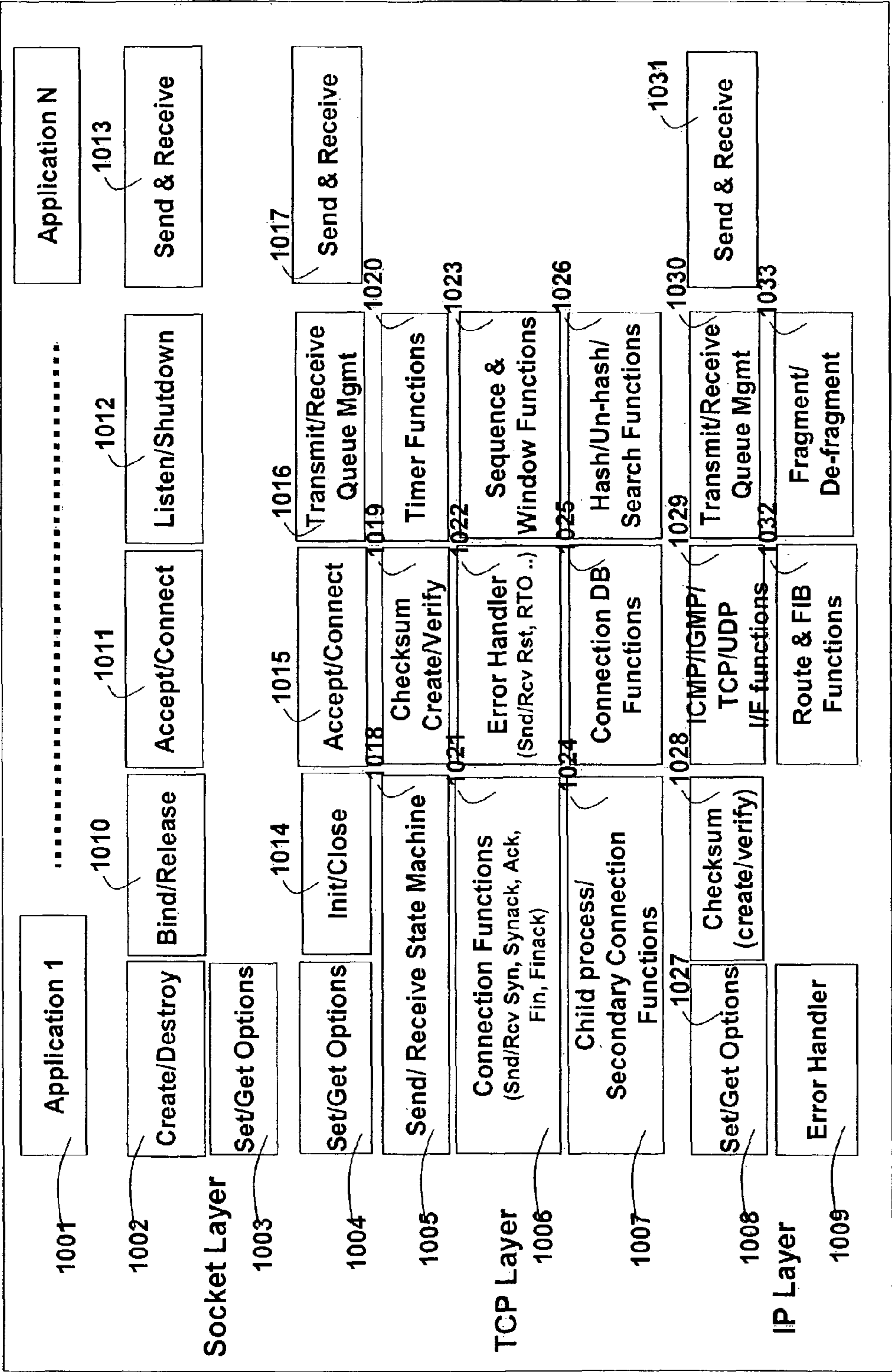
Fig. 10 TCP/IP Stack
