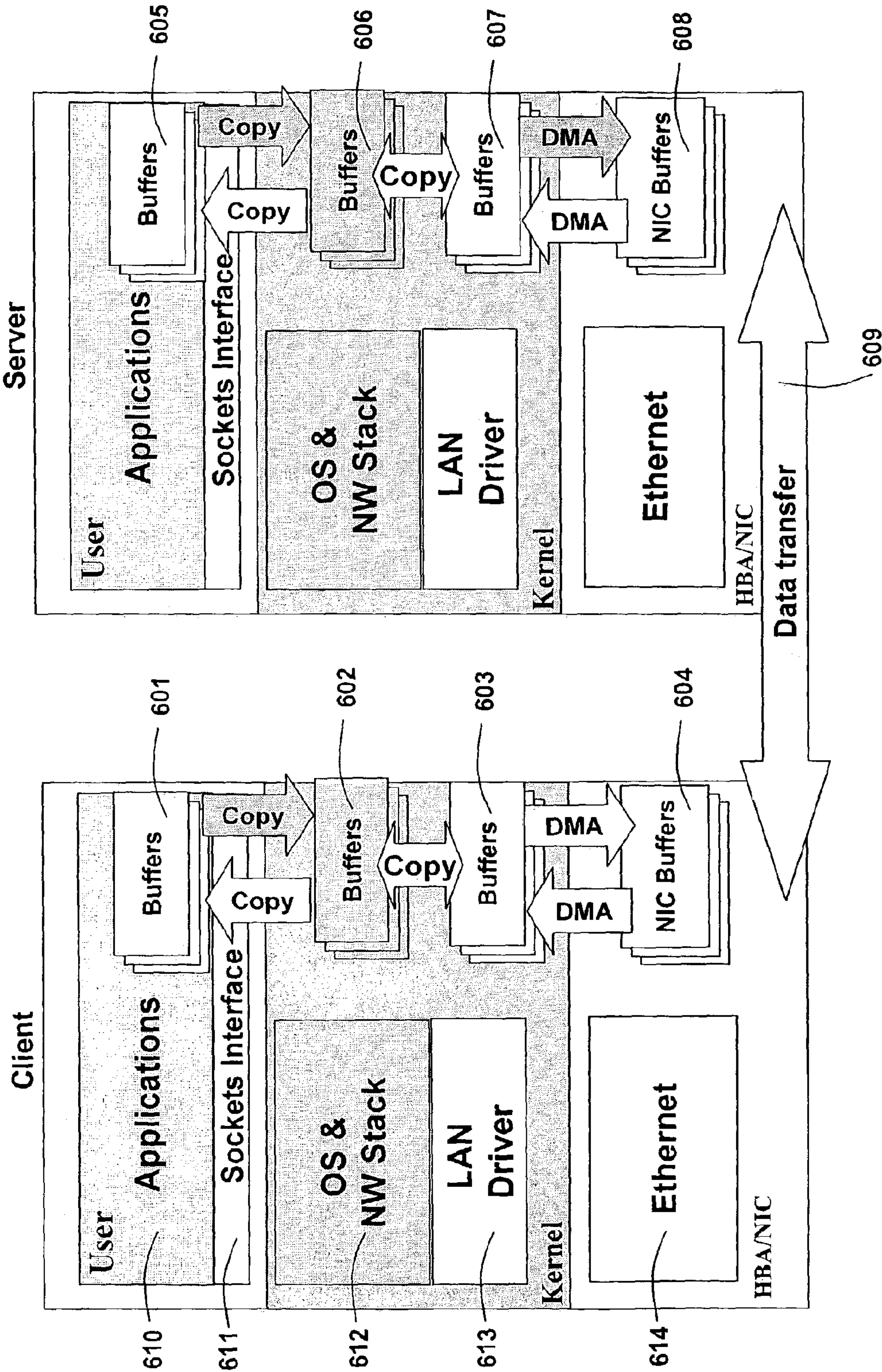
Fig. 6 S/W TCP Stack Data Transfer
