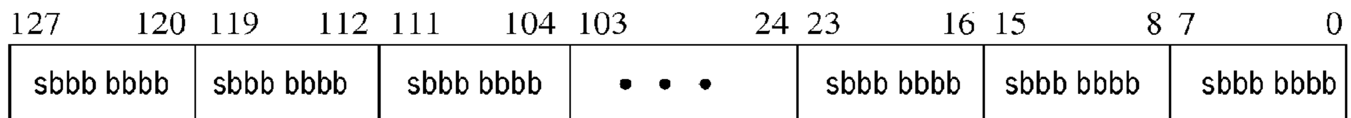
345 SIGNED PACKED BYTE REPRESENTATION
