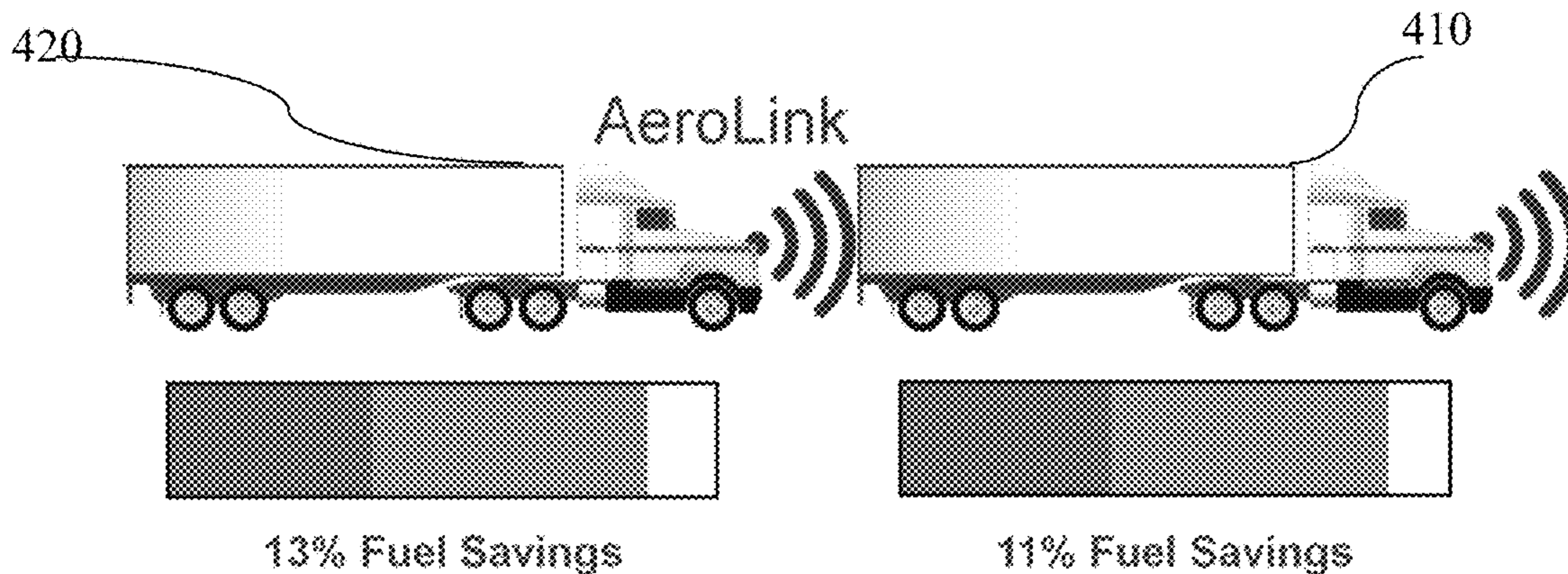
Figure 4: Typical Fuel Savings
