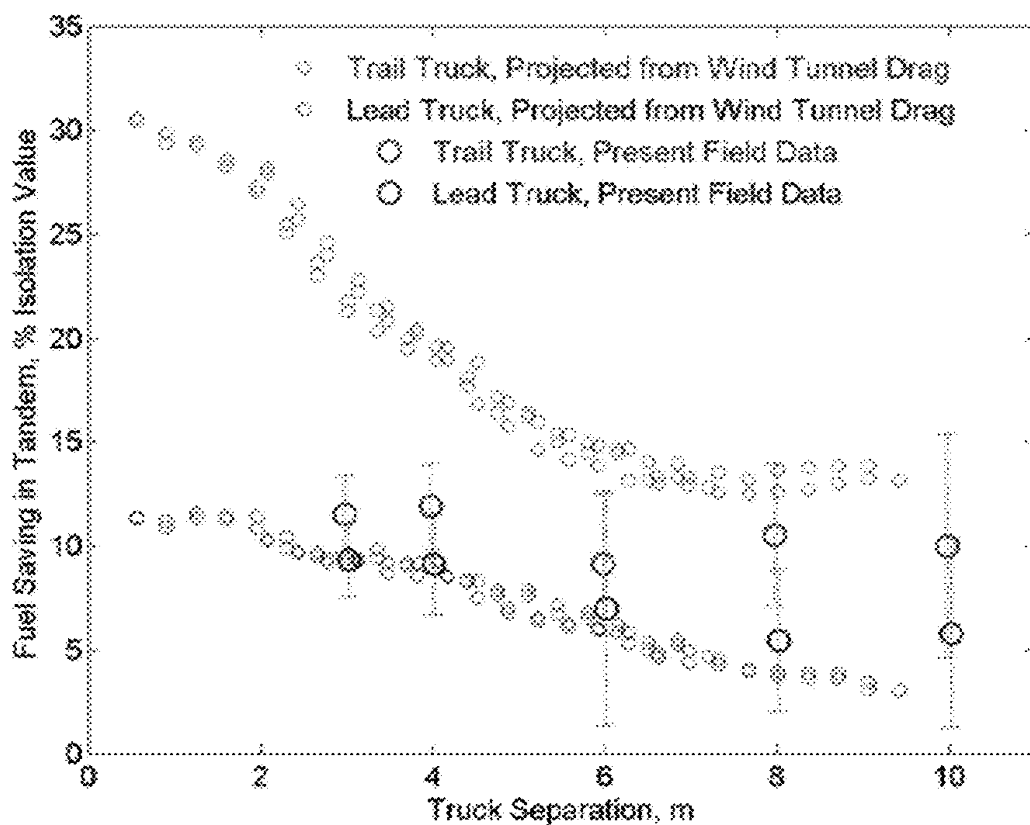
Figure 5: Fuel savings versus vehicle gap (Heavy Trucks)
