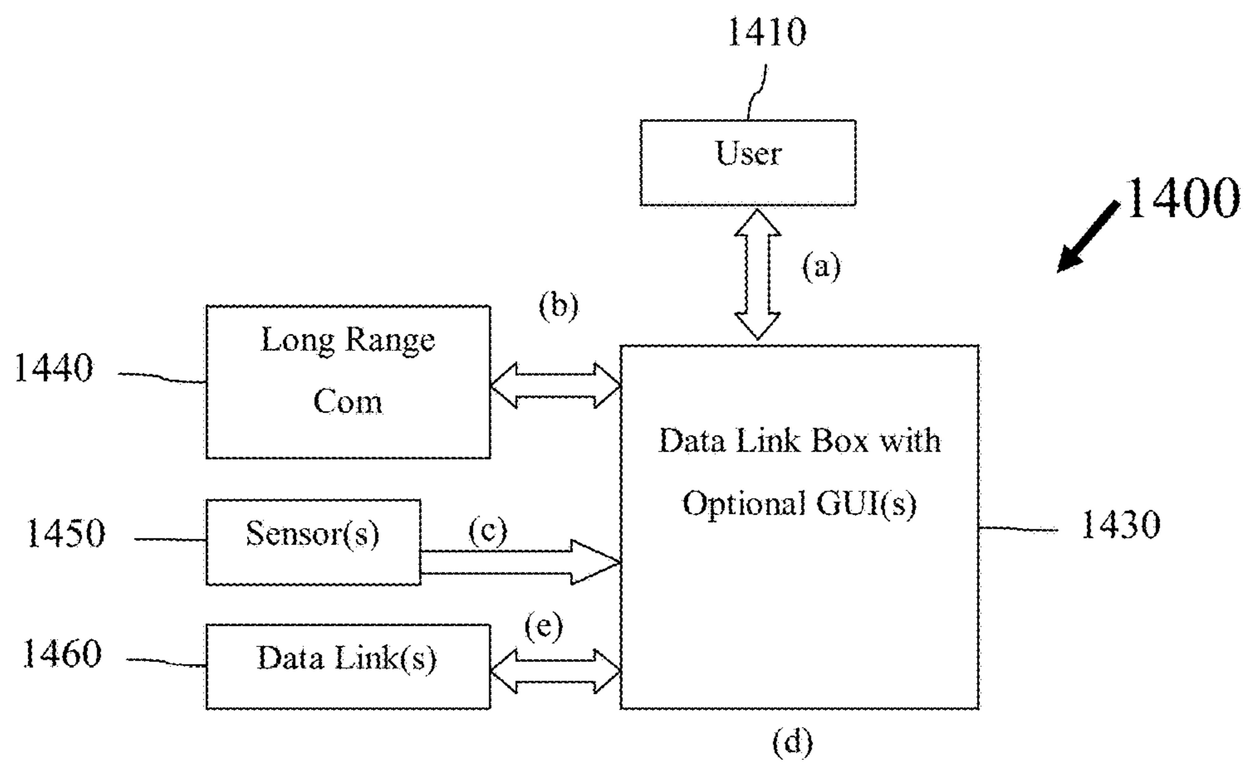
Figure 14: Simplified System for Lead Vehicle
