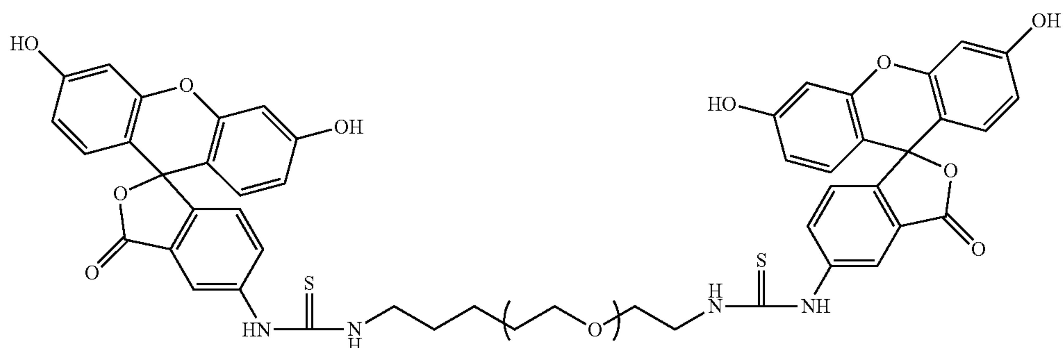
Equation 2
