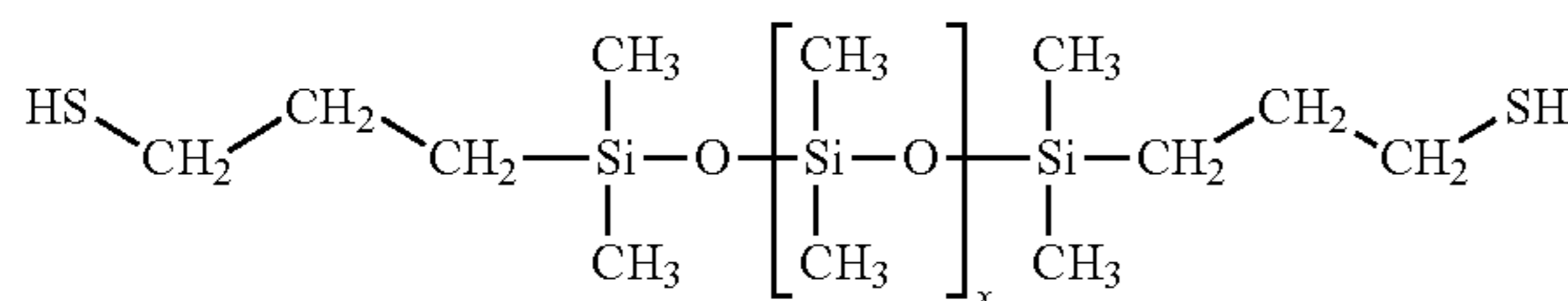
Formula IIb
