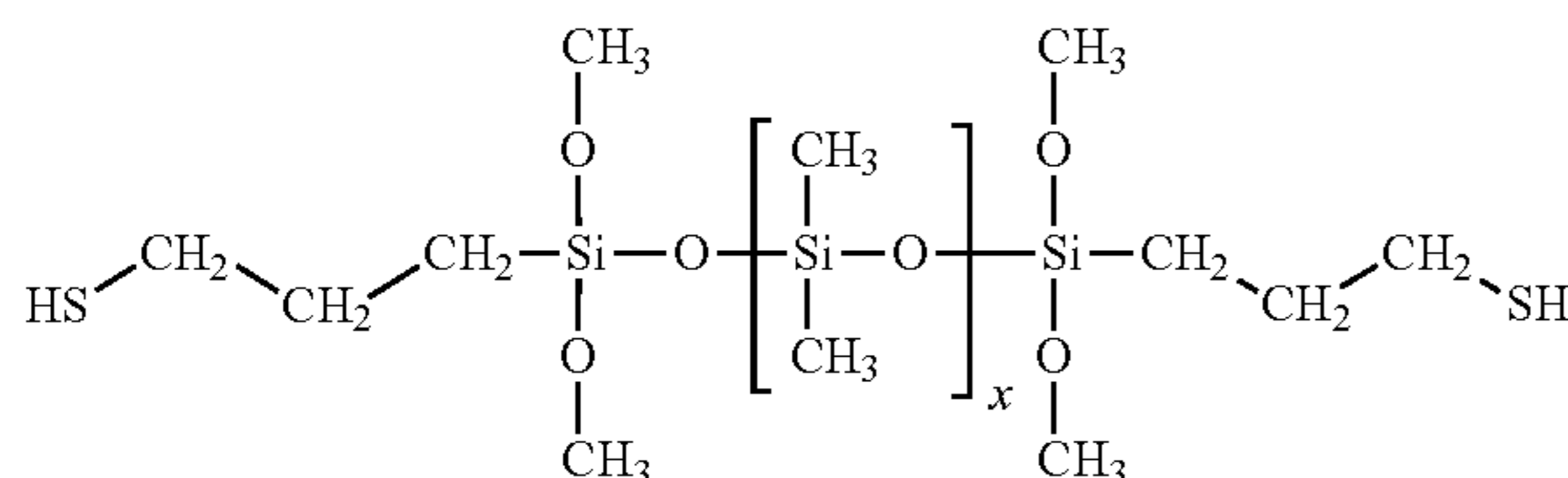
Formula IIc
