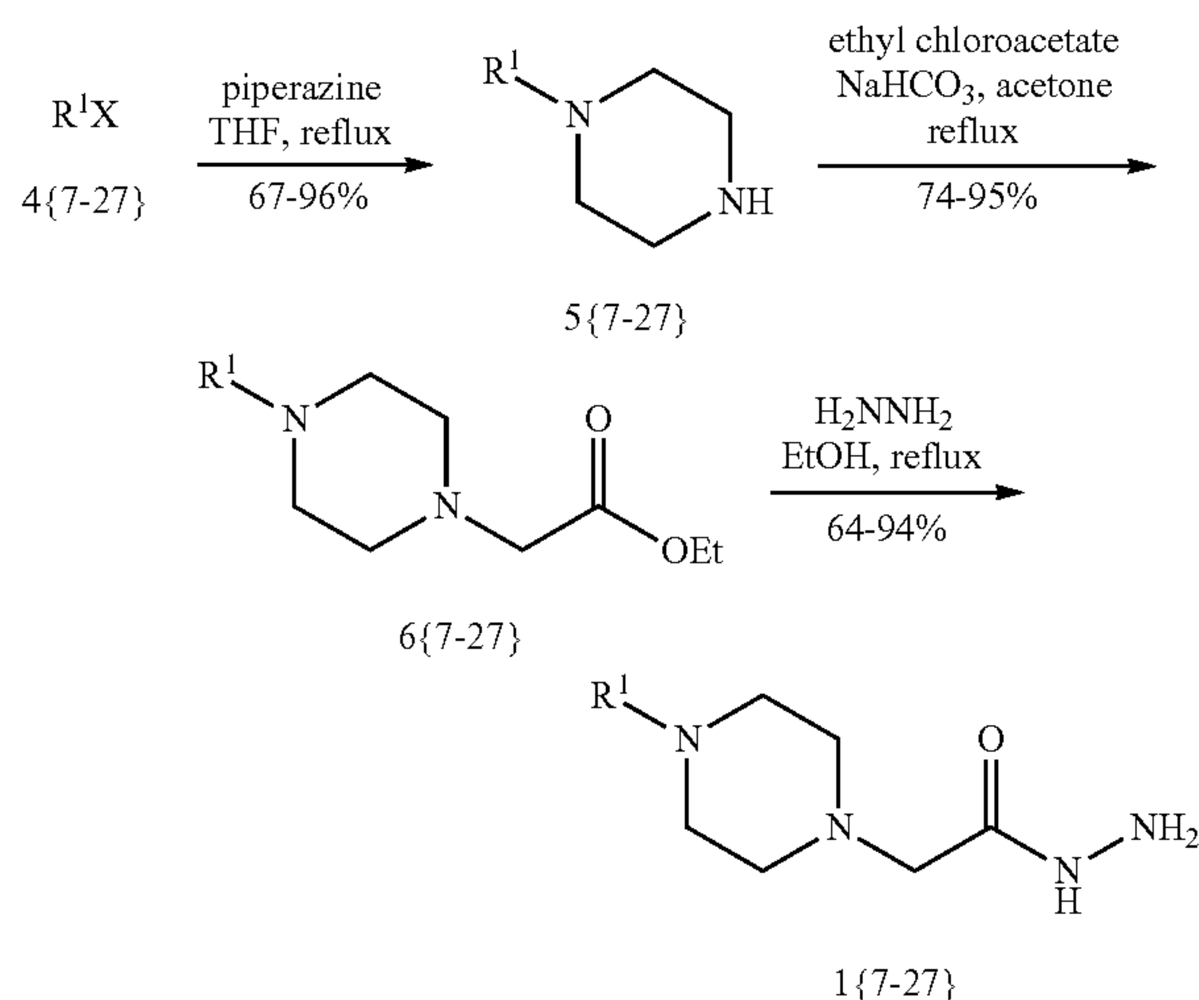
Scheme 1: Synthesis of hydrazides 1{7-27}.
