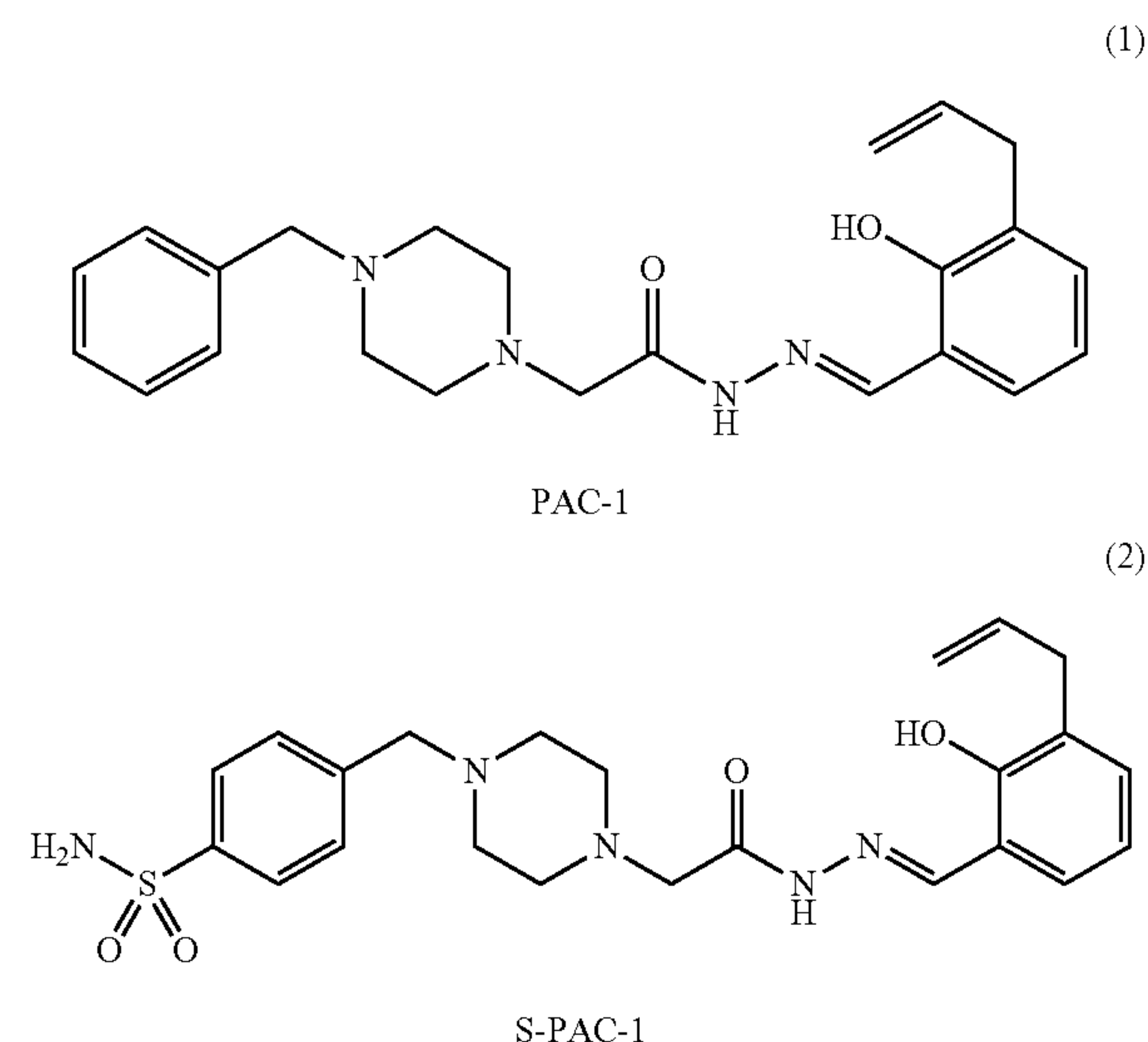
Scheme A1. Structure of PAC-1(1) and S-PAC-1(2).
