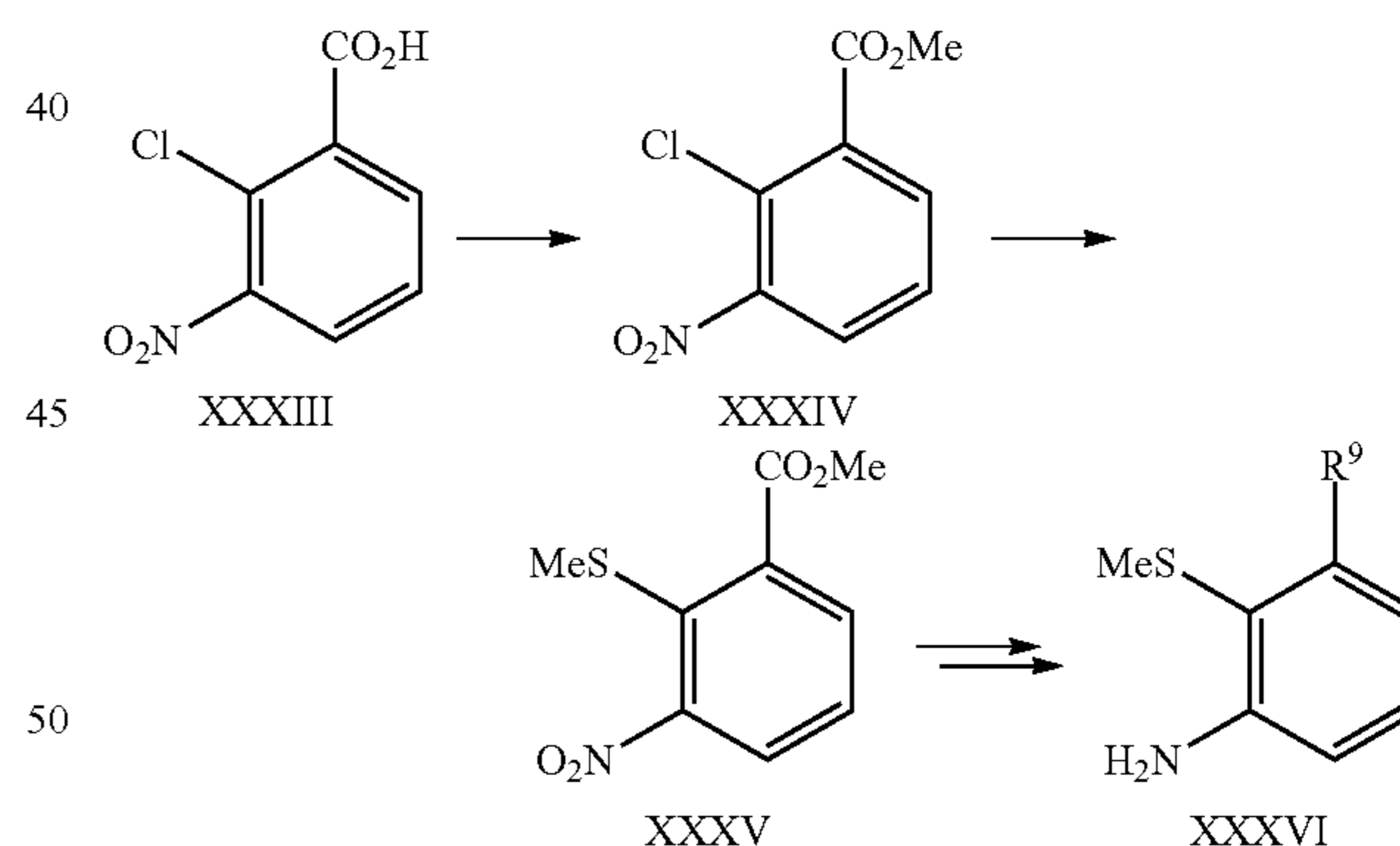
Scheme 10. Synthesis of thioanilines XXXVI
