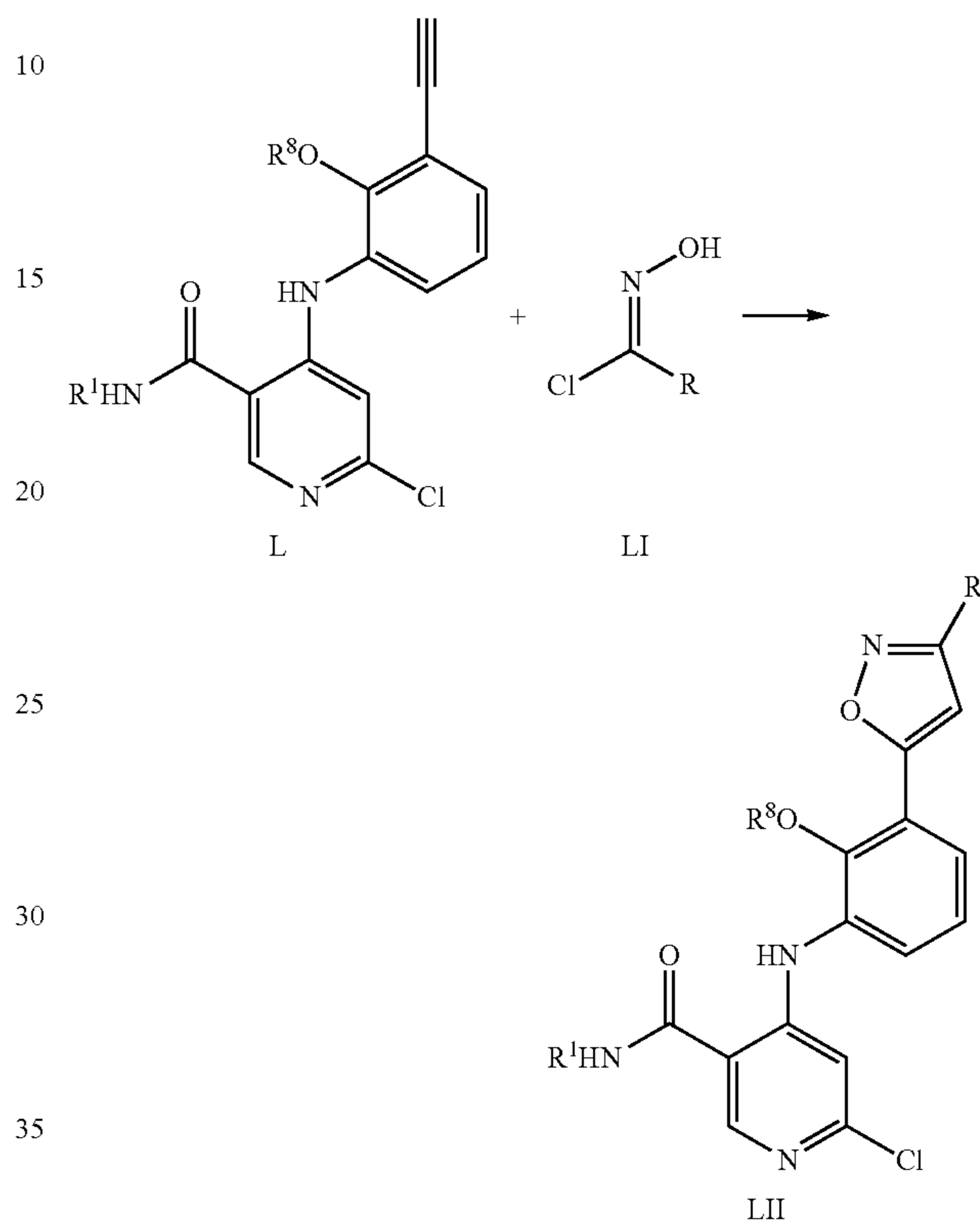
Scheme 14. Synthesis of LII
