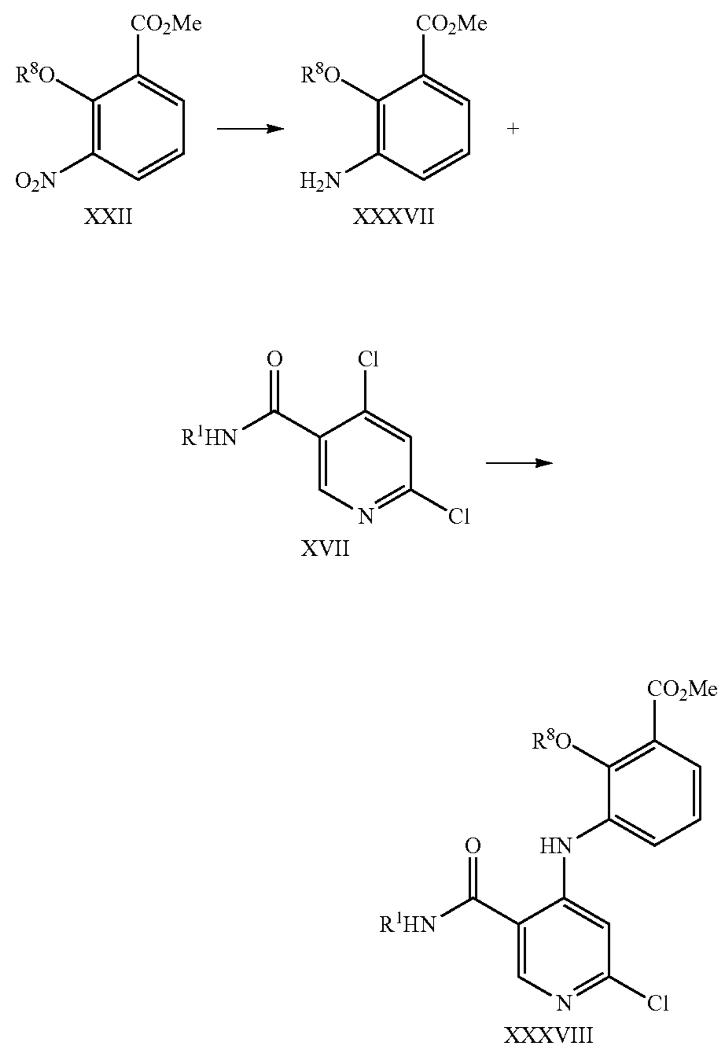
Scheme 11. Synthesis of final compounds XLII
