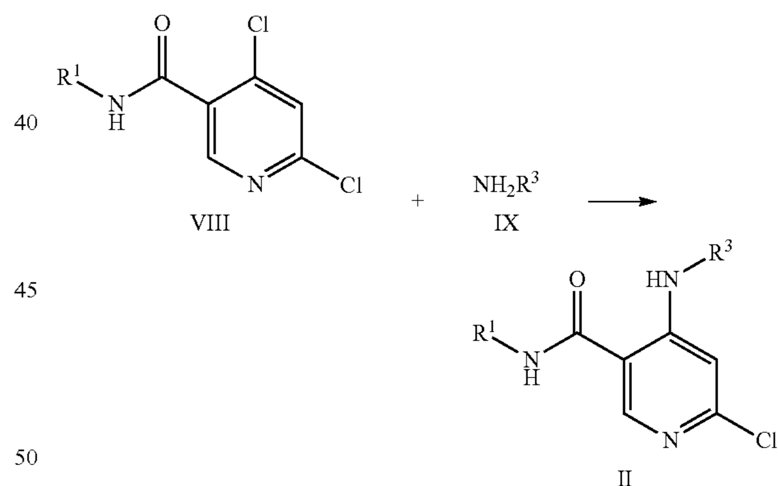
Scheme 4. Coupling of halo-pyridine VIII with amine IX
