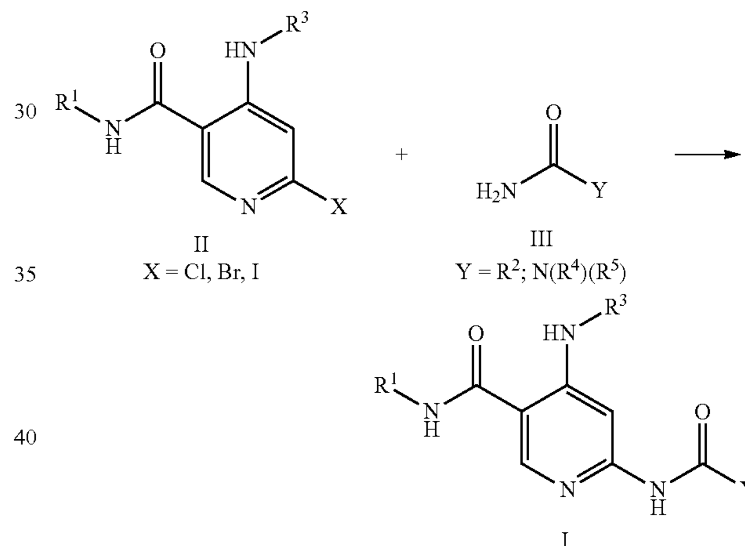
Scheme 1. Coupling of halo-pyridine II with amide III
