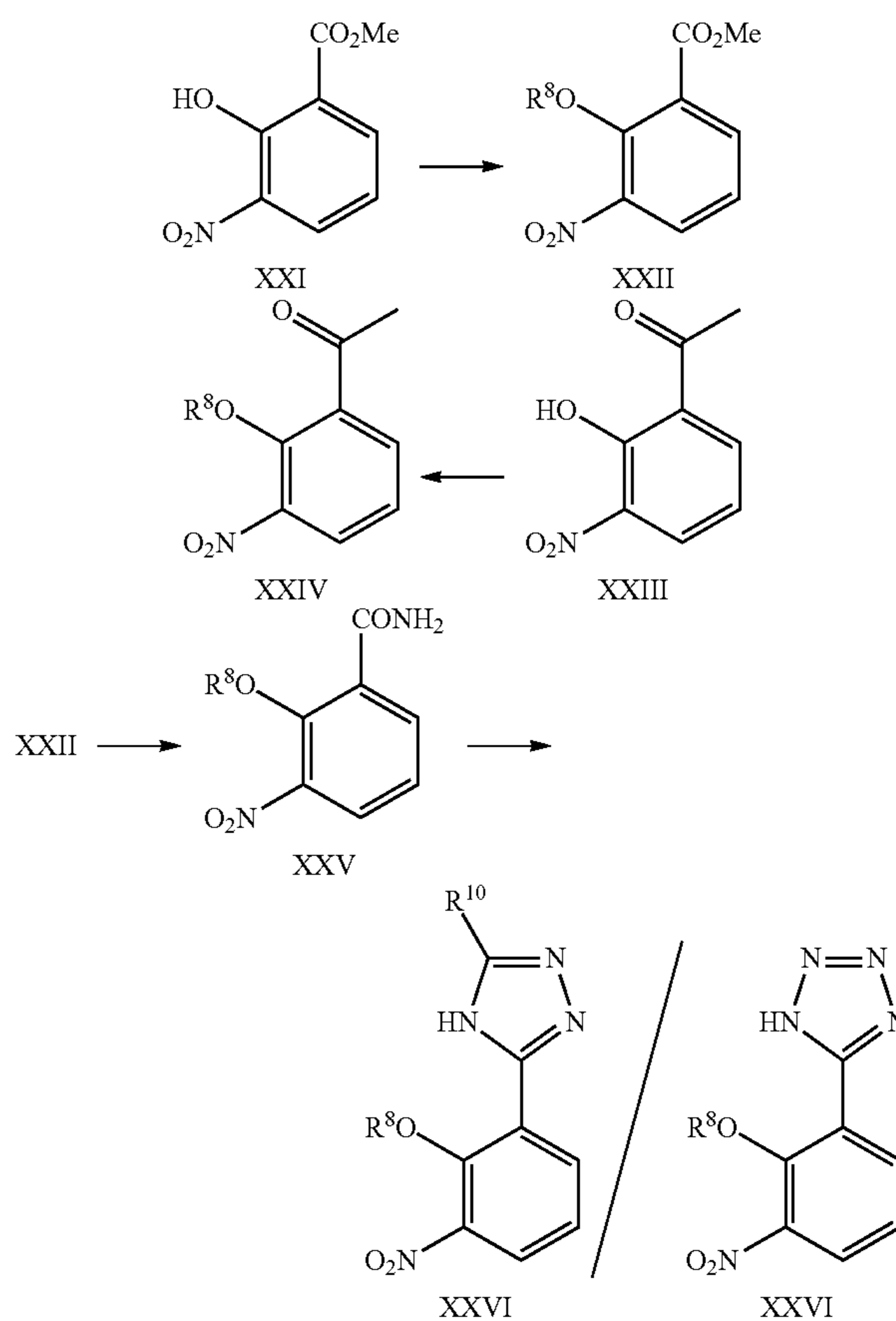
Scheme 9. Alternate synthesis of anilines IX
