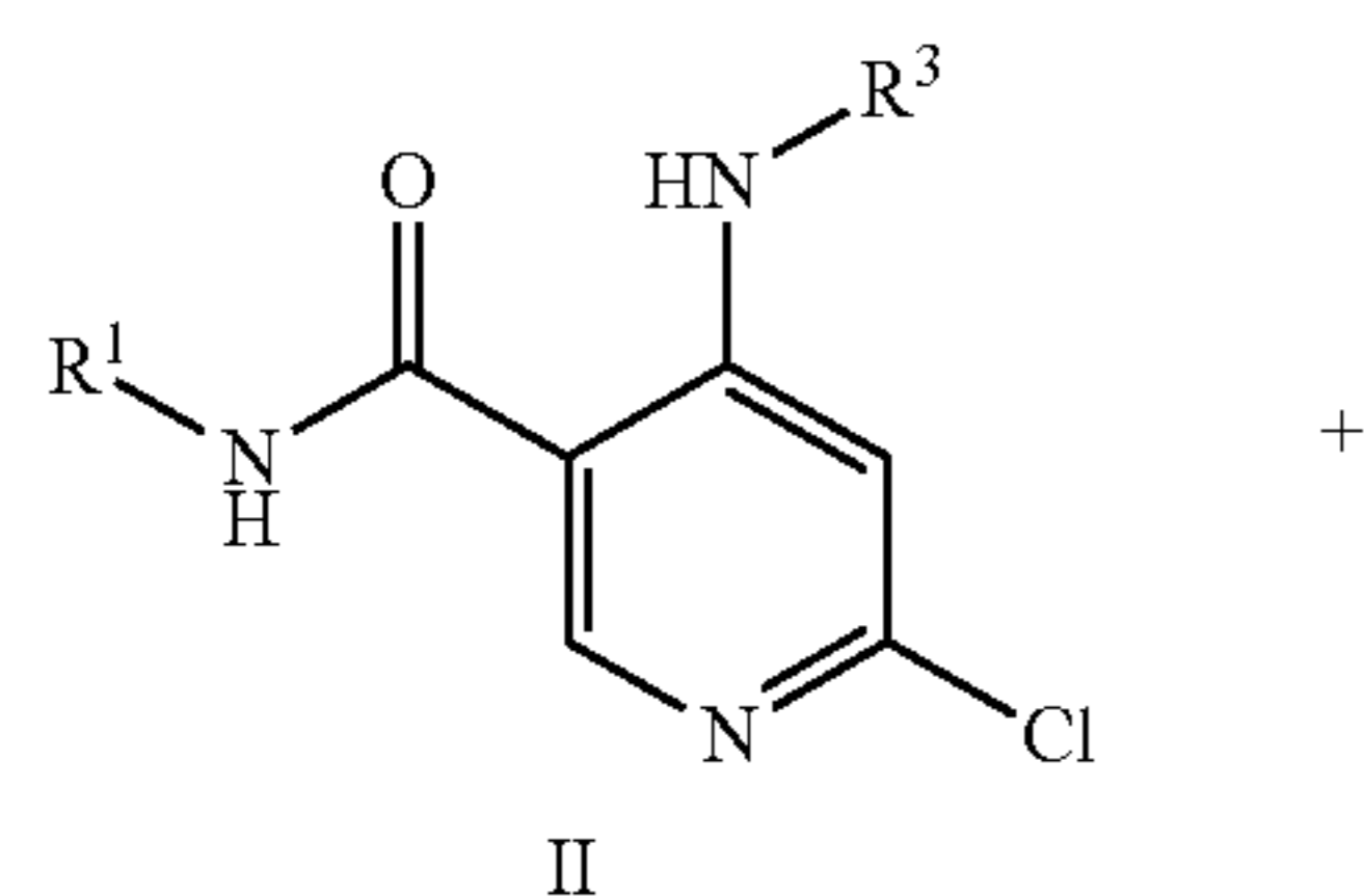
Scheme 3. Coupling of halo-pyridine II with VII
