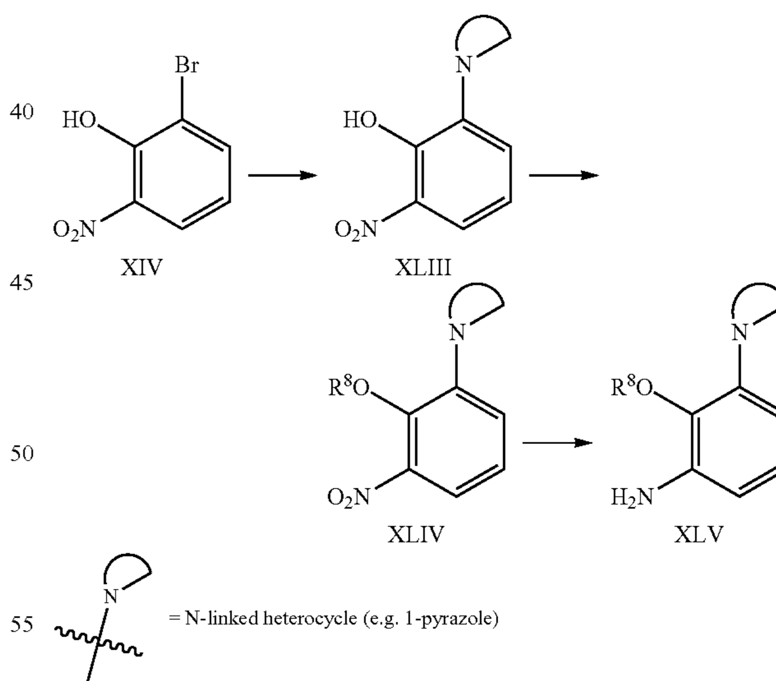
Scheme 12. Synthesis of anilines XLV (variant of IX)
