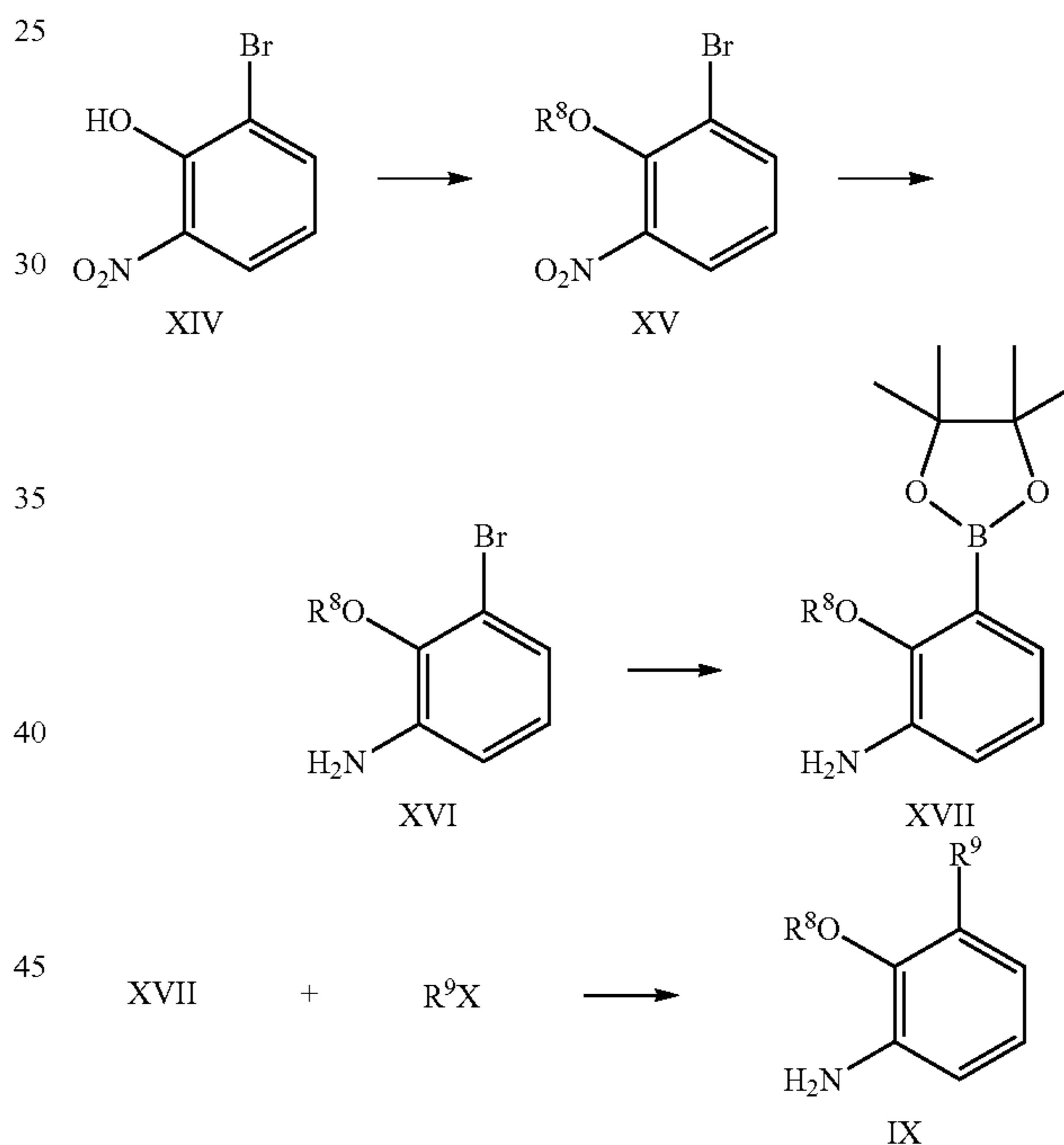
Scheme 7. Synthesis of anilines IX
