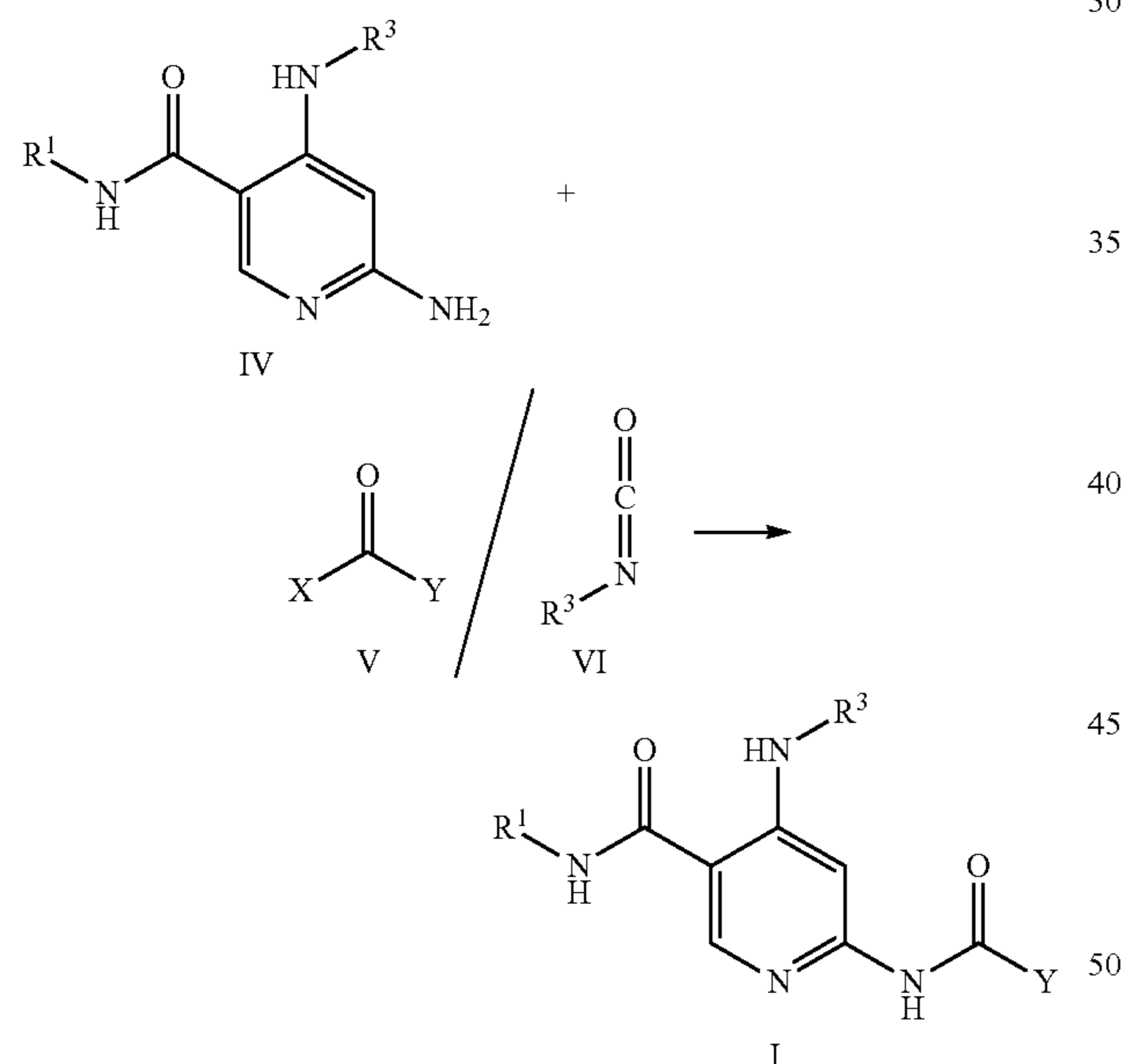
Scheme 2. Coupling of amino-nicotinamide IV with V/VI
