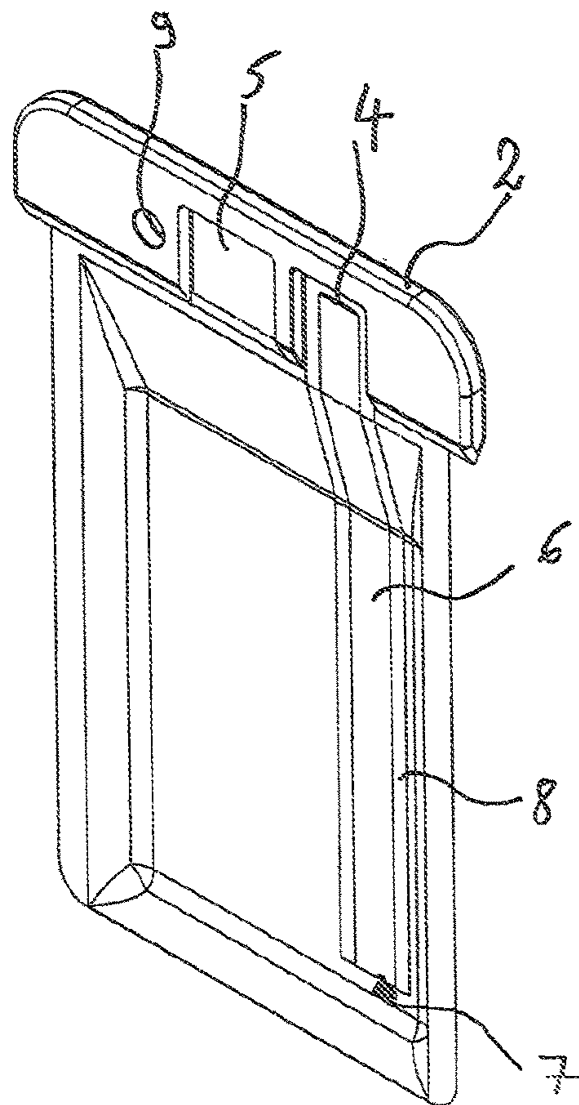
Fig 2
