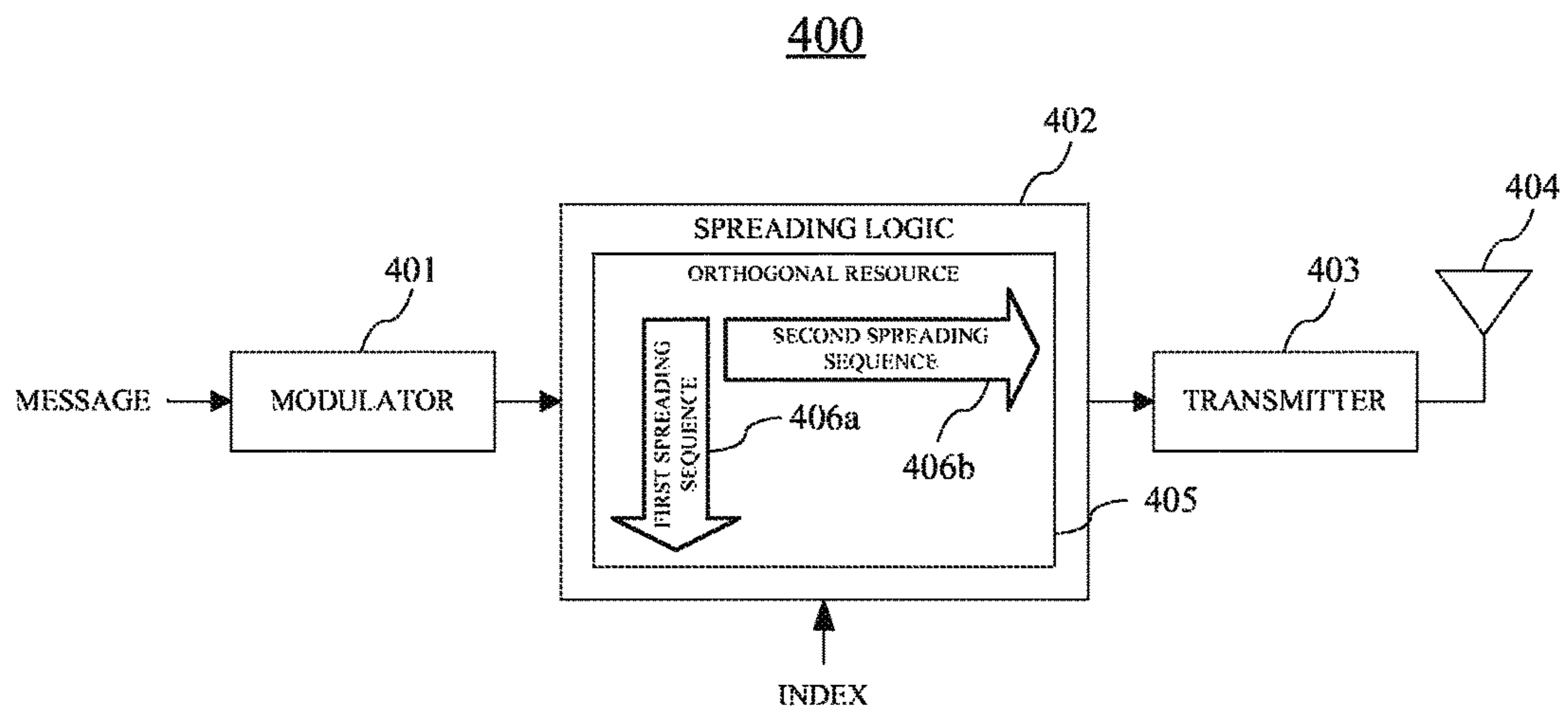
FIG. 4 (PRIOR ART)
