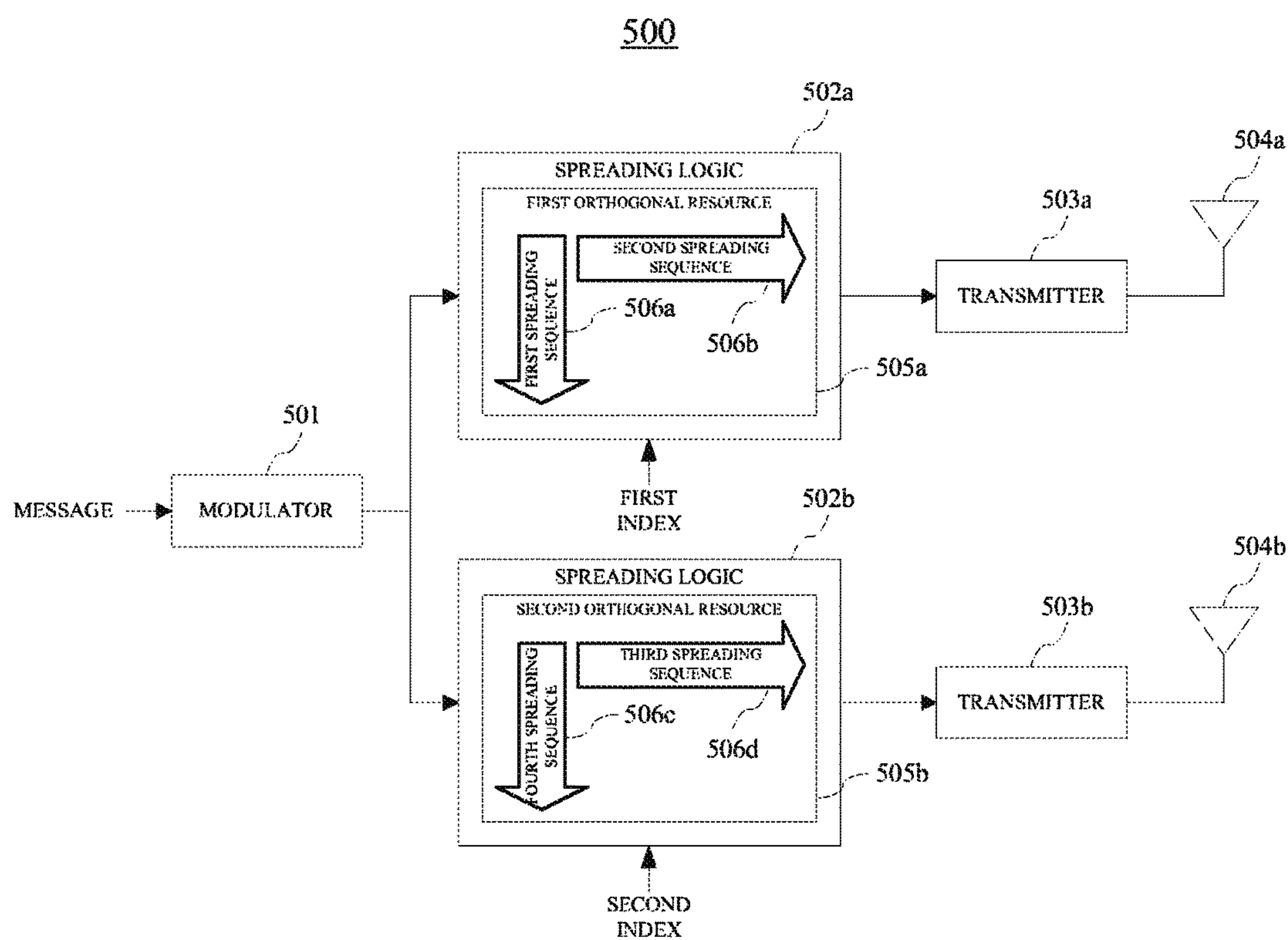
FIG. 5 (PRIOR ART)
