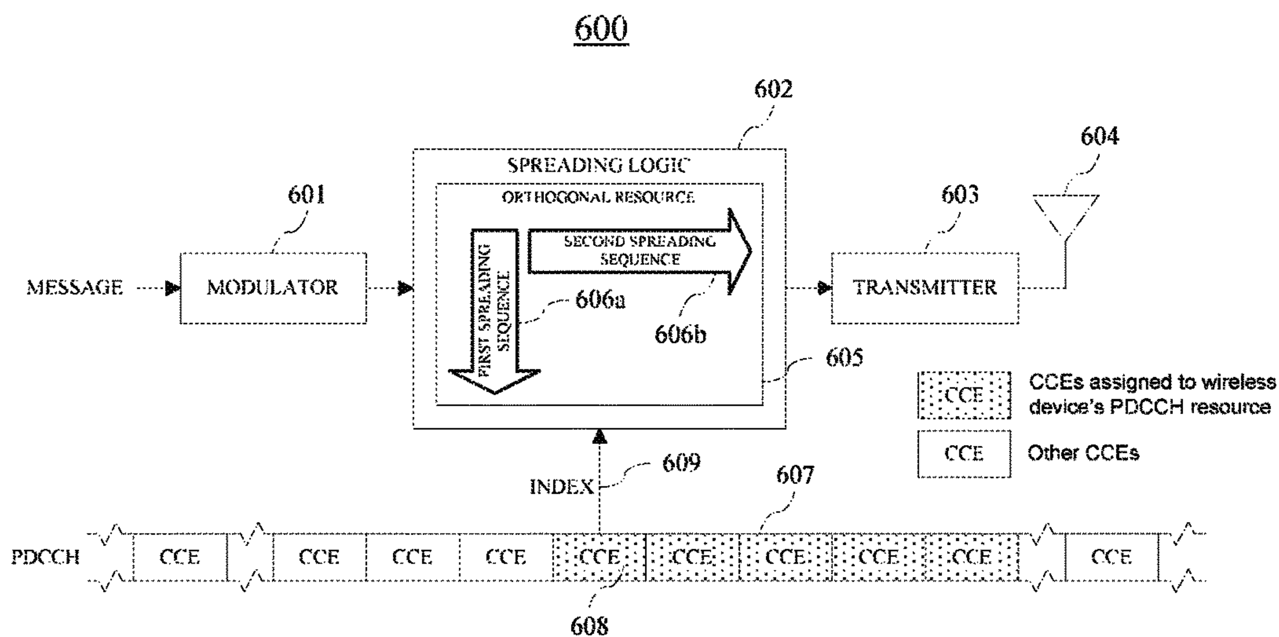
FIG. 6 (PRIOR ART)
