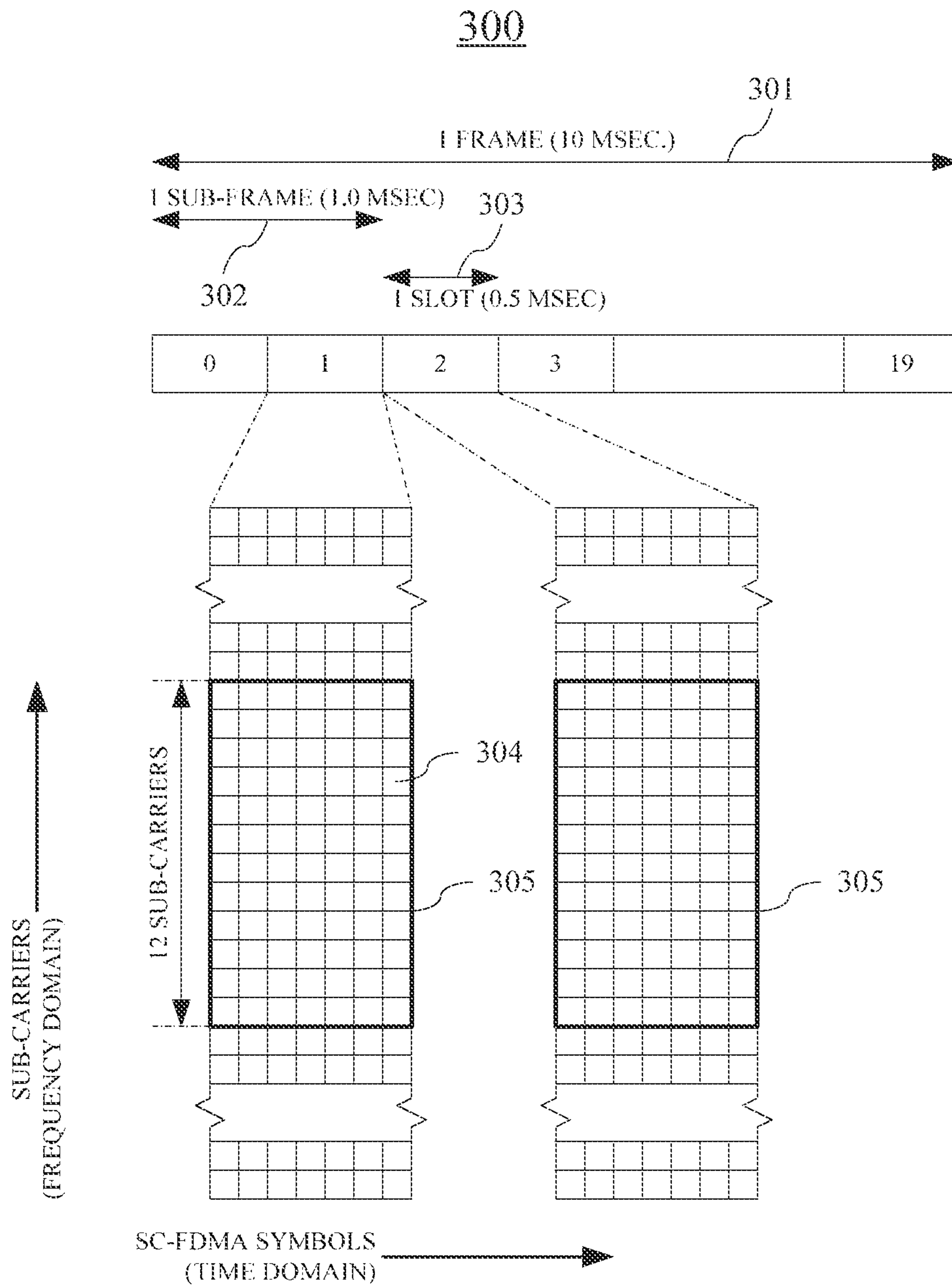
FIG. 3 (PRIOR ART)
