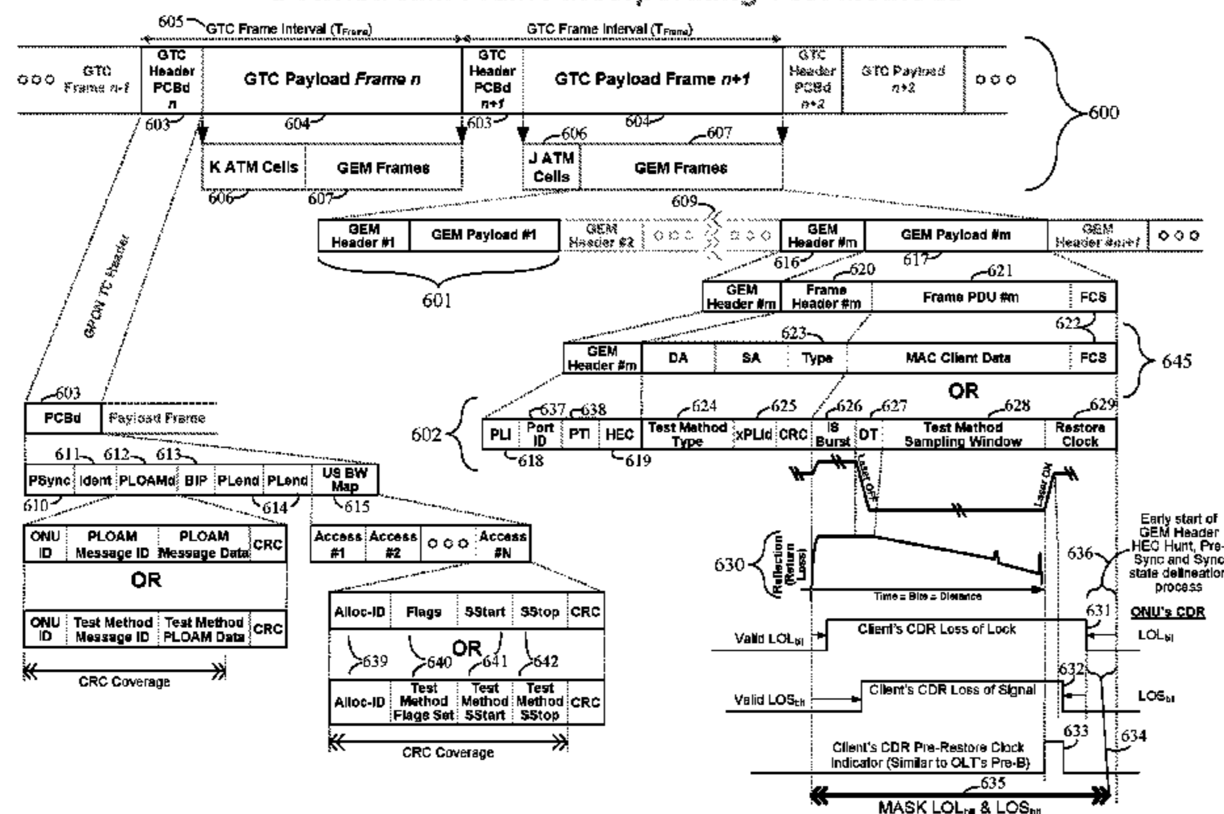
ITU-T G.984 GPON and ITU-T G.987 XG-PON Transmission Convergence (GTC) Downstream Frame Incorporating Test Methods
