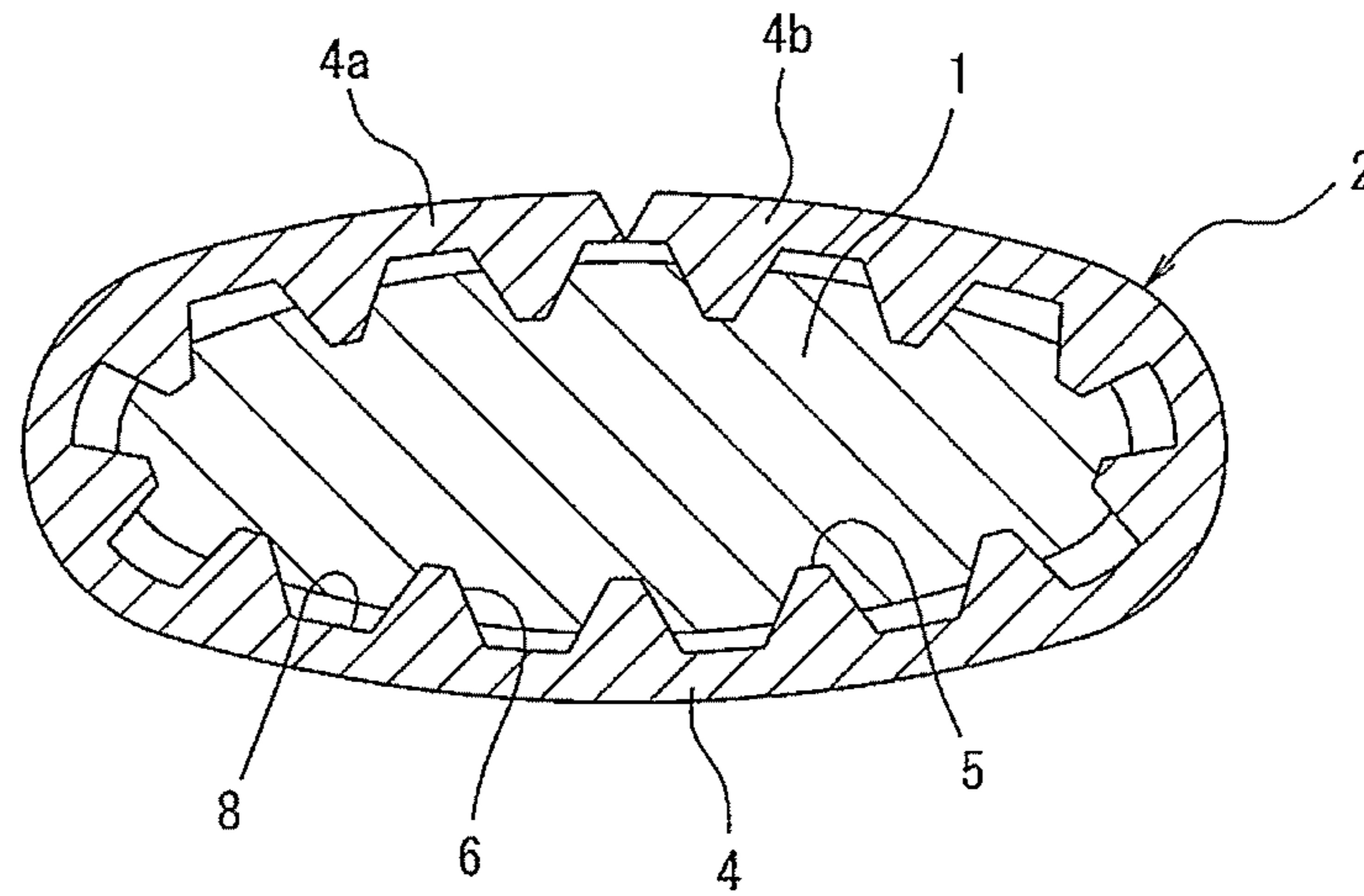
FIG. 16 Prior Art
