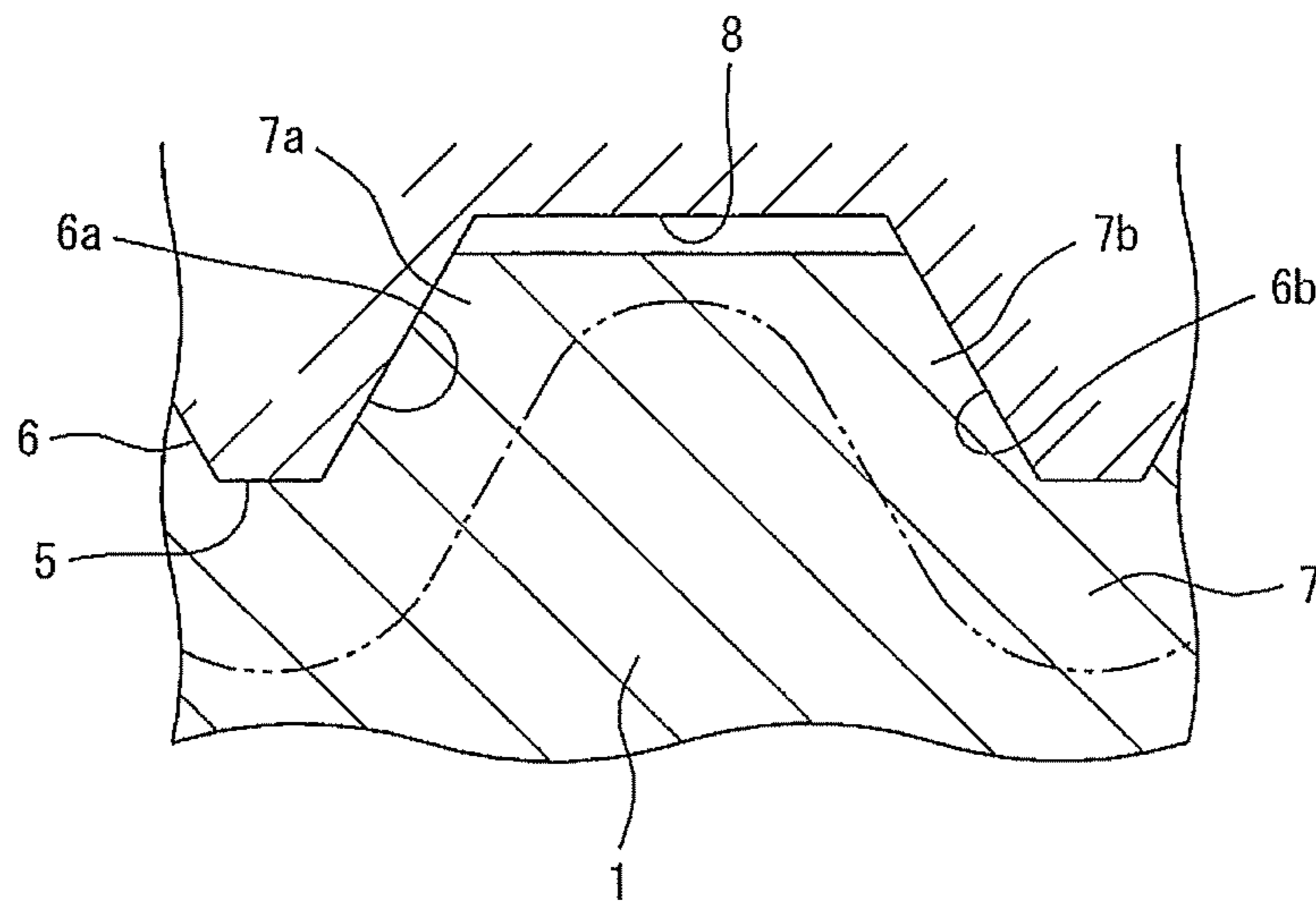
FIG. 17 Prior Art
