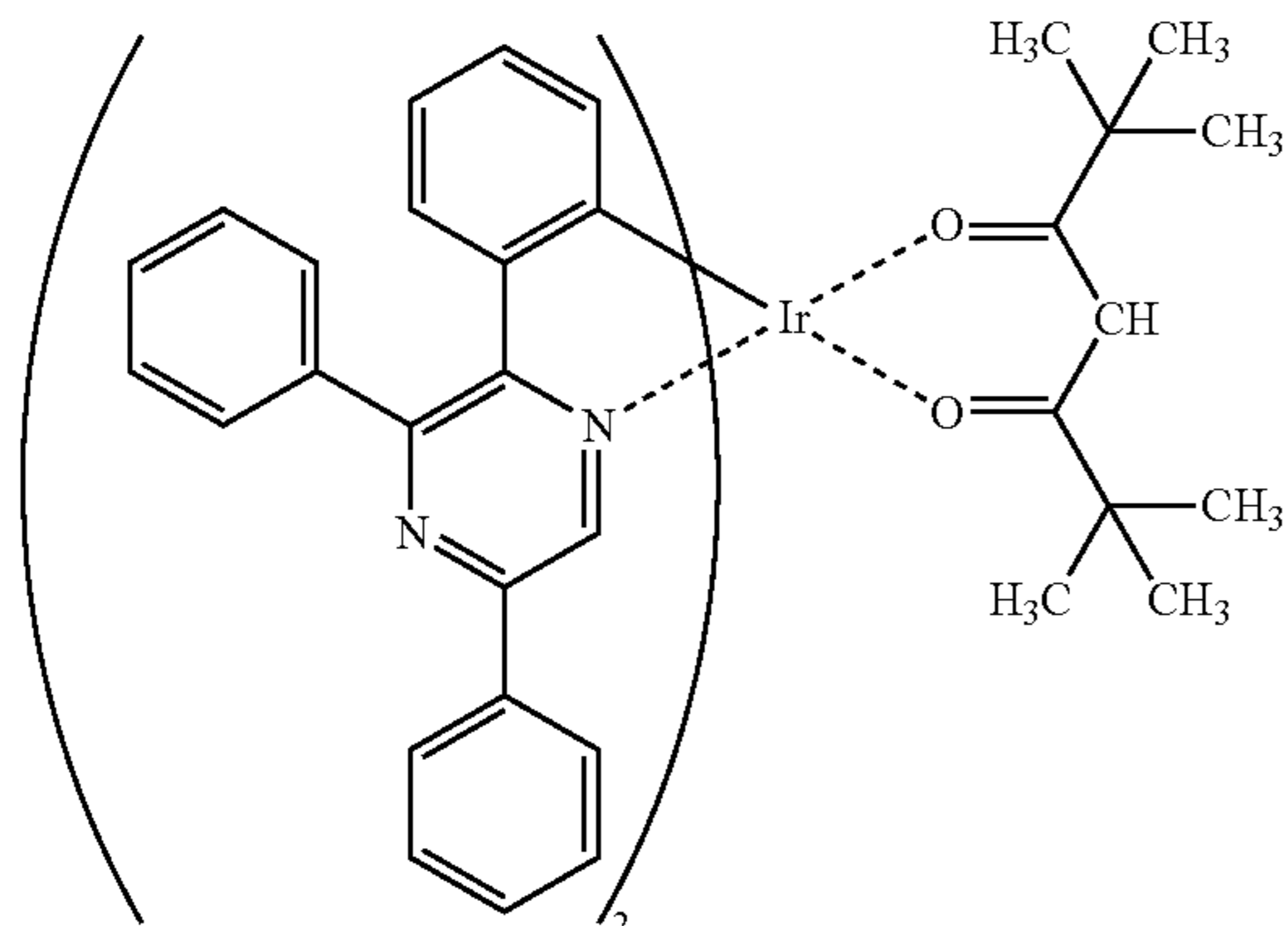
Ir(tppr) 2 (dpm)
