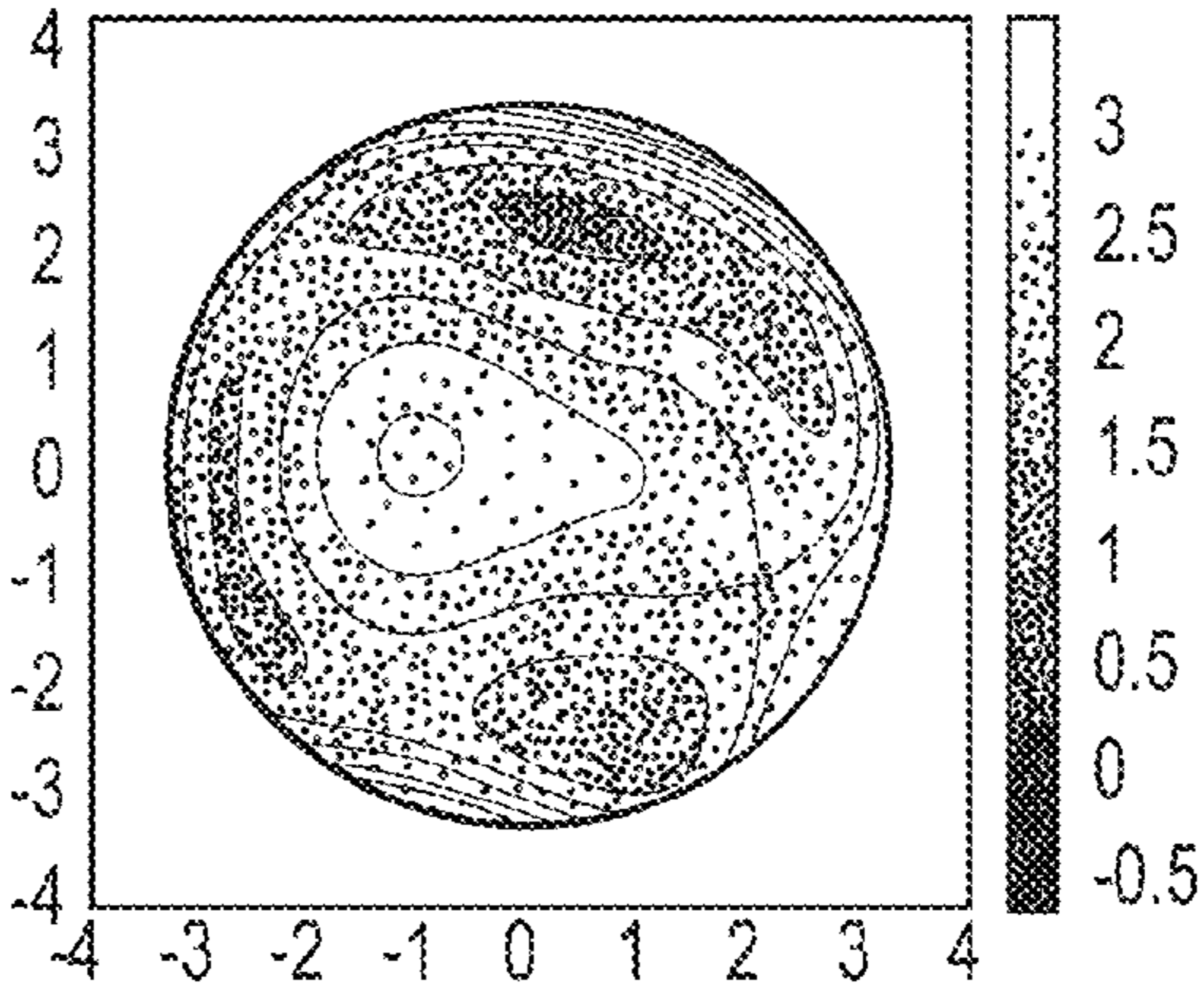
RMS ERROR = 0.124um AMONG (0.061, 0.124, 0.057, 0.094)
