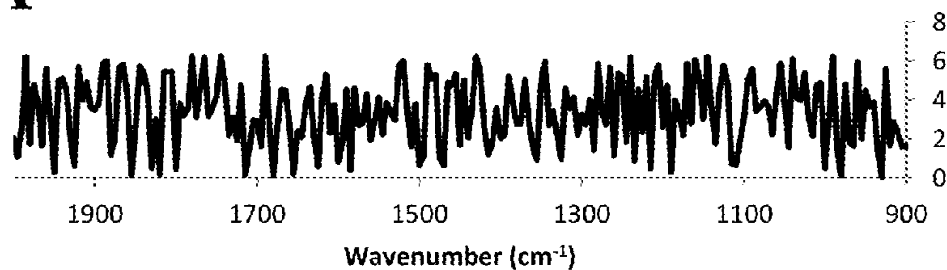
Raw spectrum
