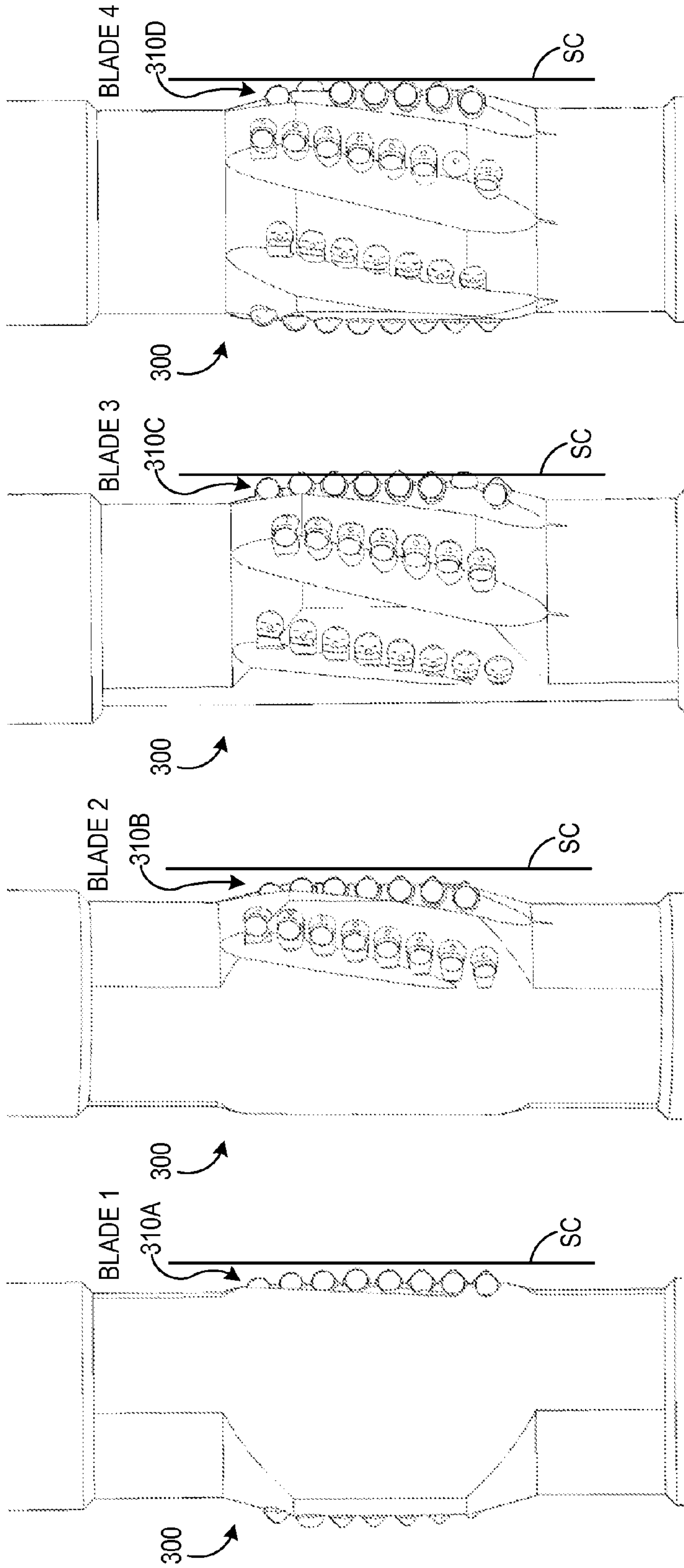
BLADE 1 5-1/4" TO 5-1/2"
