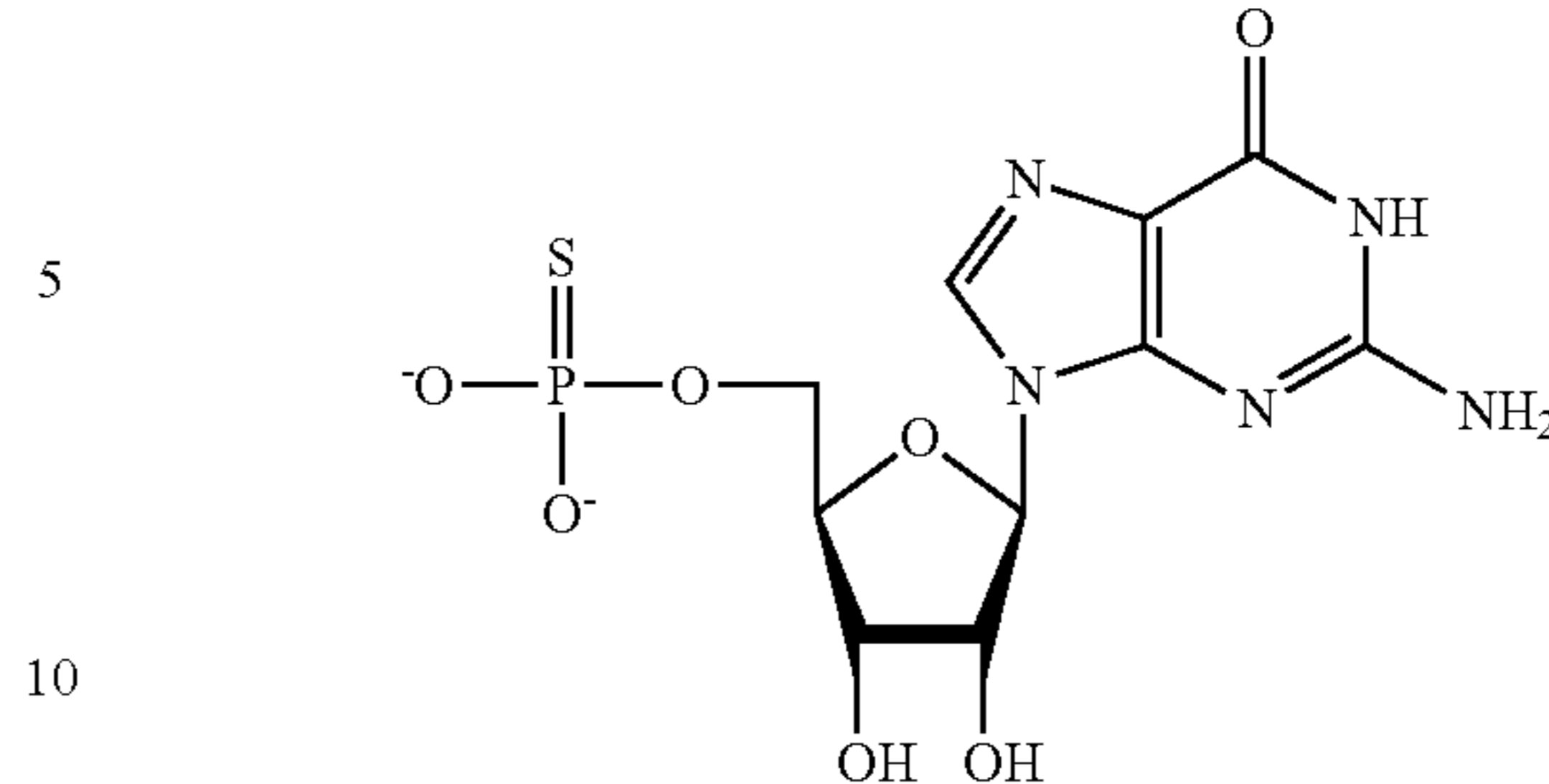
5'-O-(1-Thiophosphate)-Guanosine
