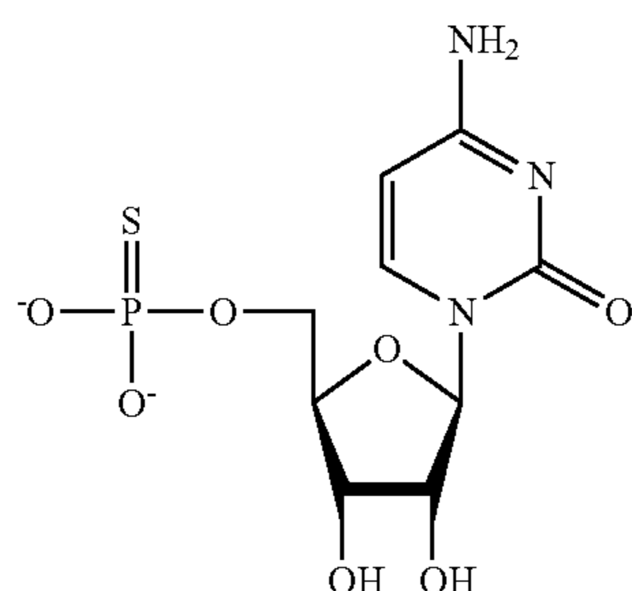
5'-O-(1-Thiophosphate)-Cytidine
