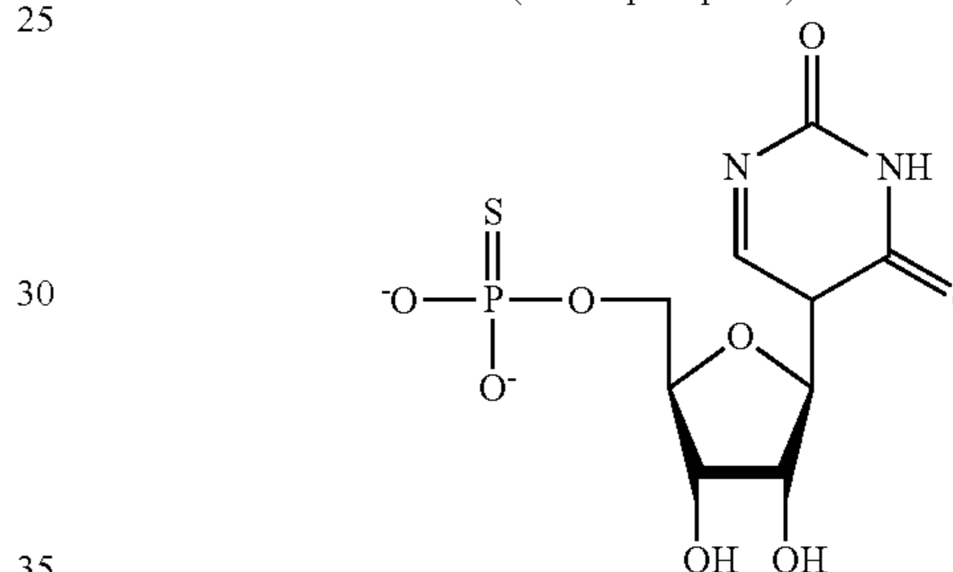
5'-O-(1-Thiophosphate)-Pseudouridine
