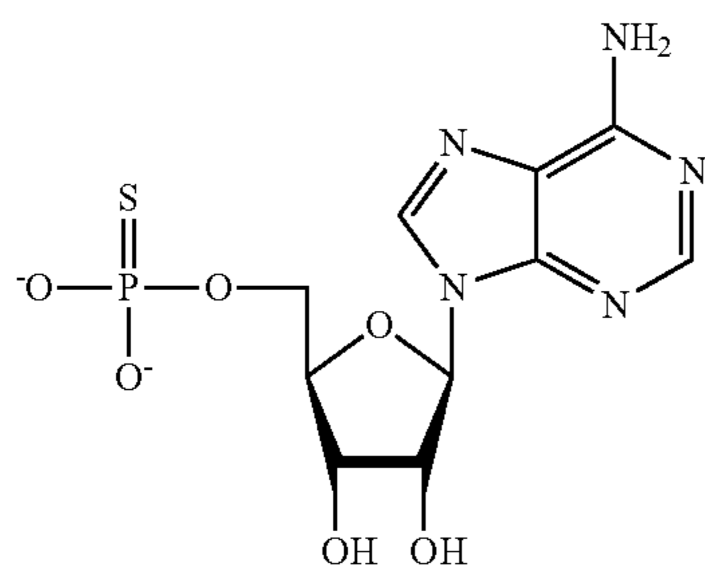
5'-O-(1-Thiophosphate)-Adenosine
