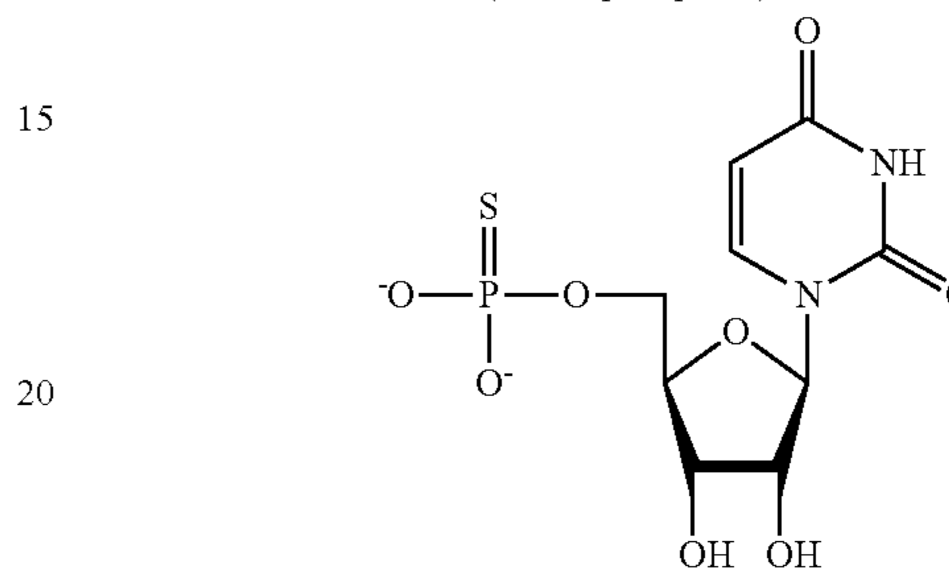
5'-O-(1-Thiophosphate)-Uridine
