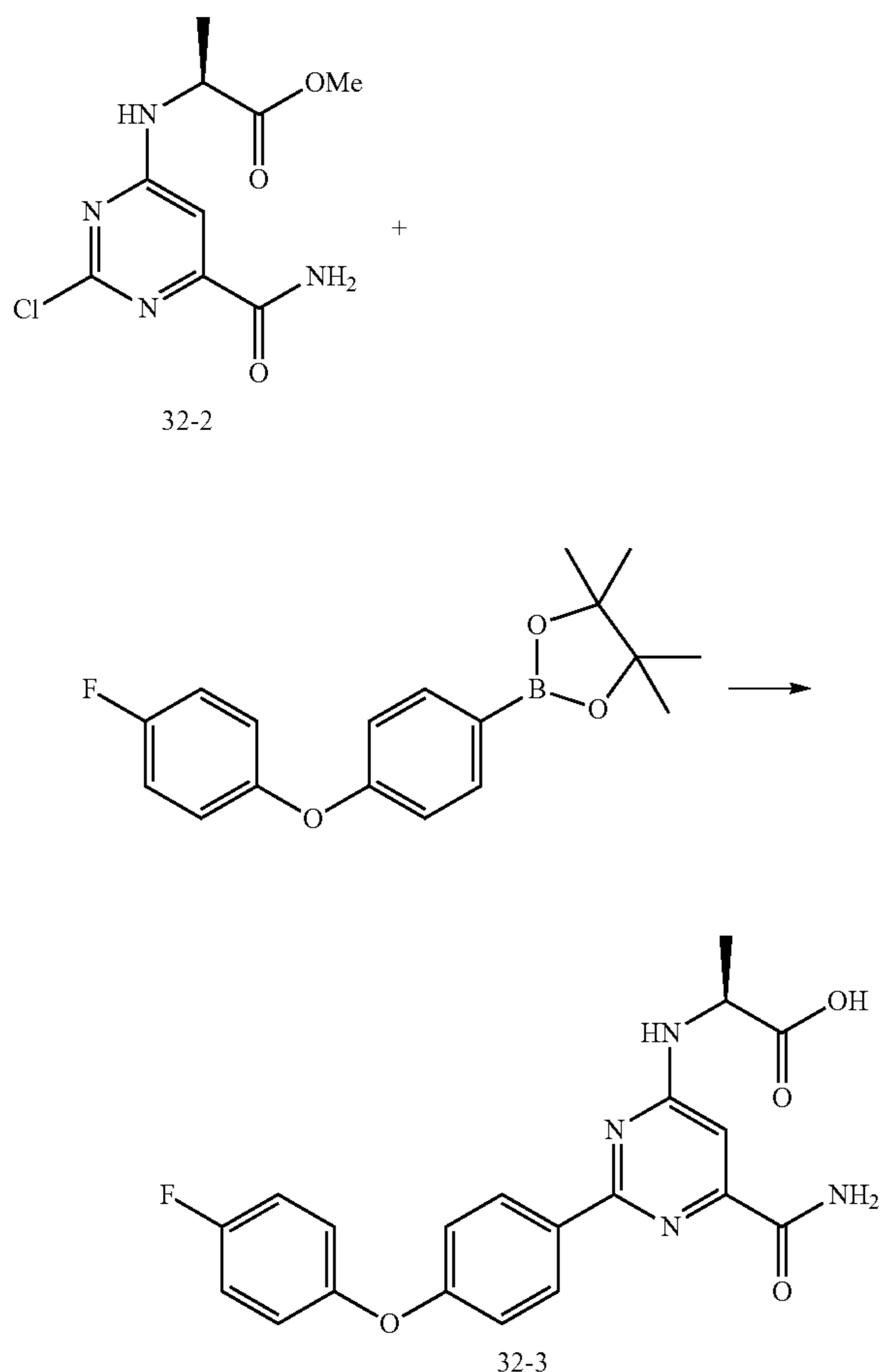
Scheme 74
