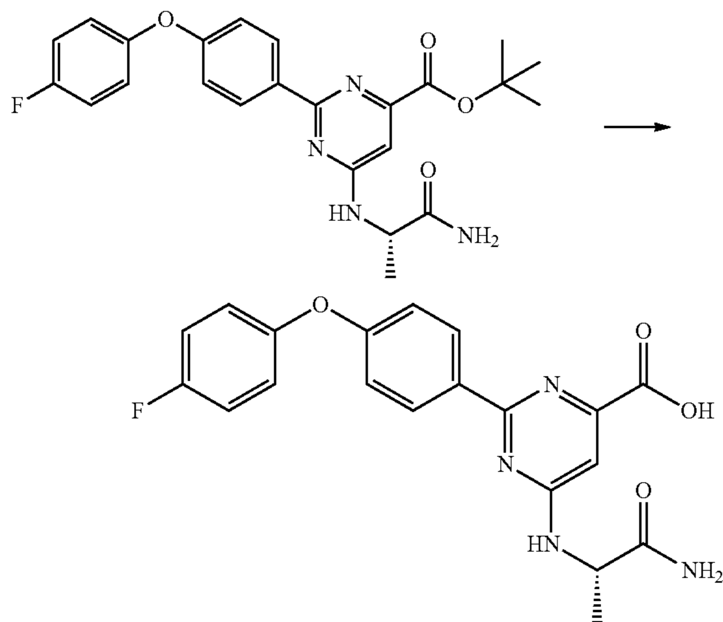
Scheme 16
