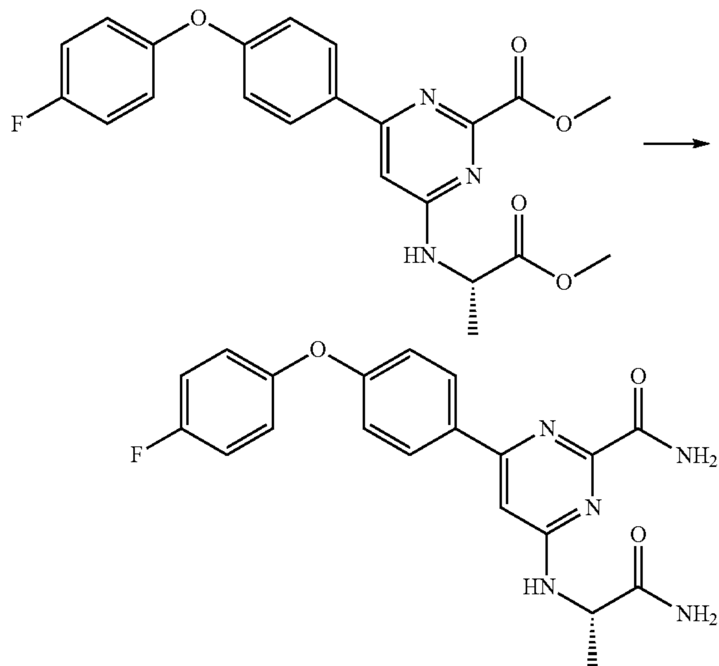
Scheme 41
