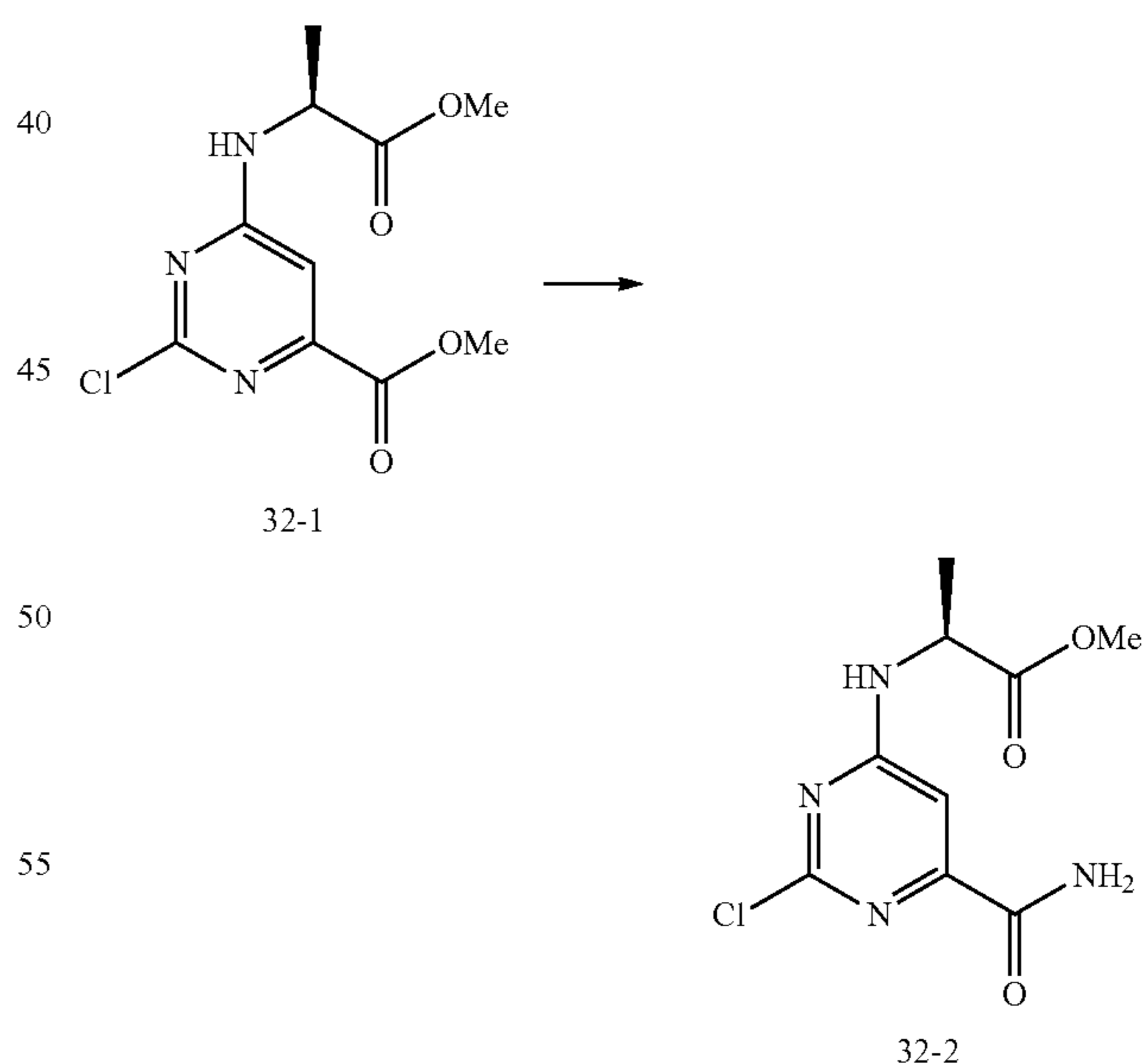
Scheme 73
