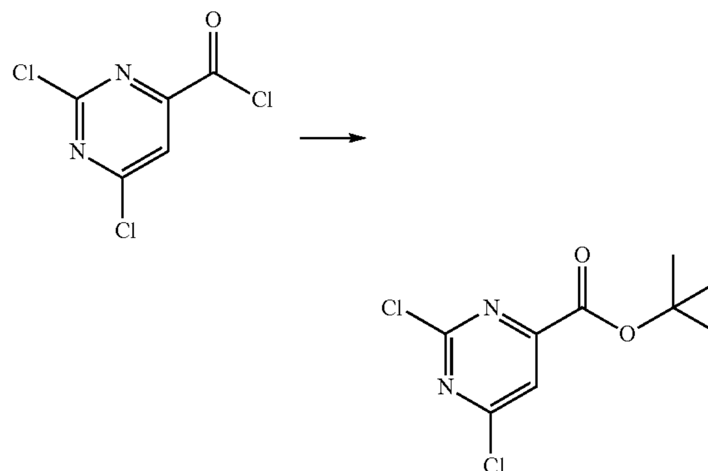
Scheme 10
