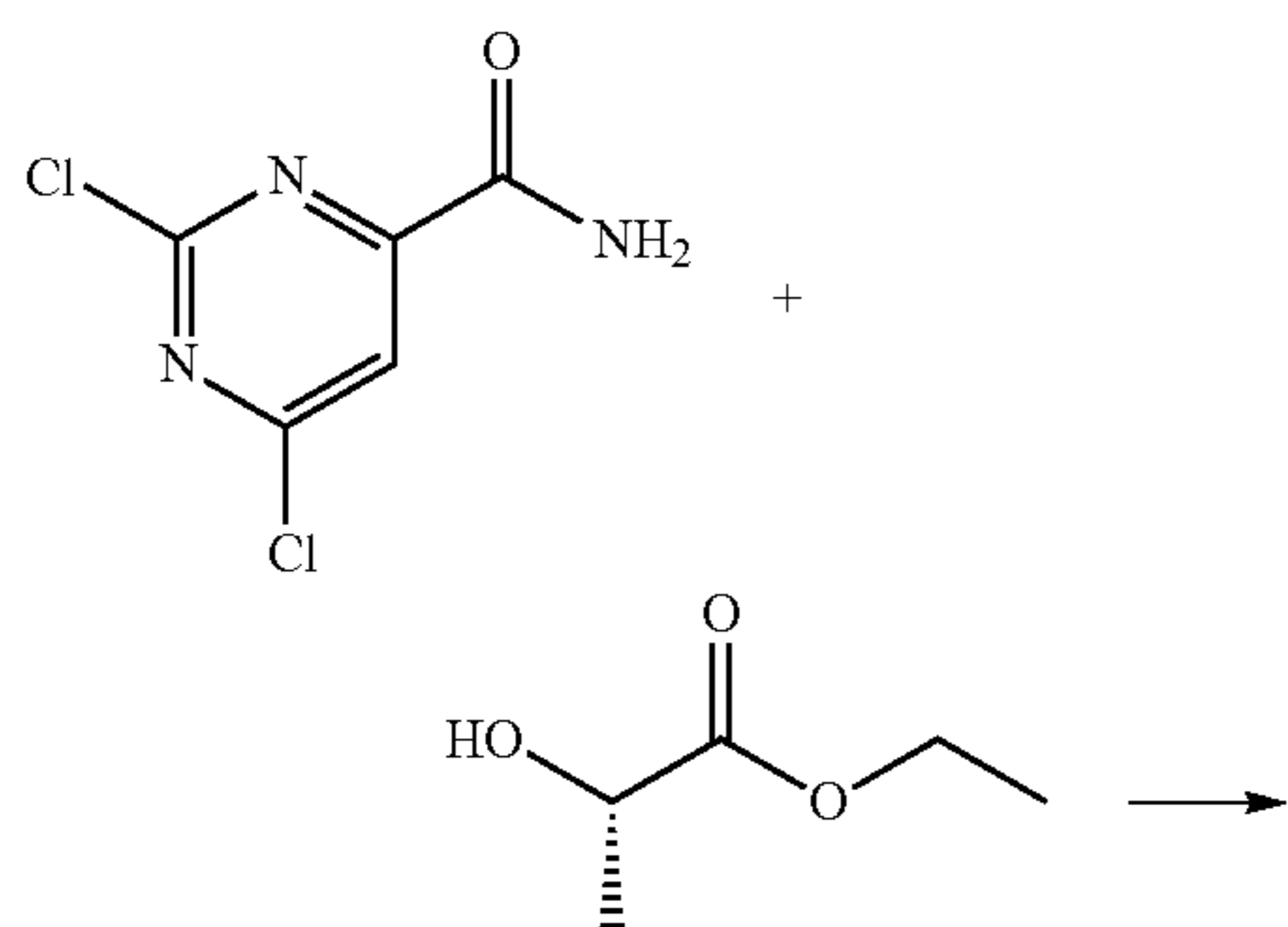
Scheme 42
