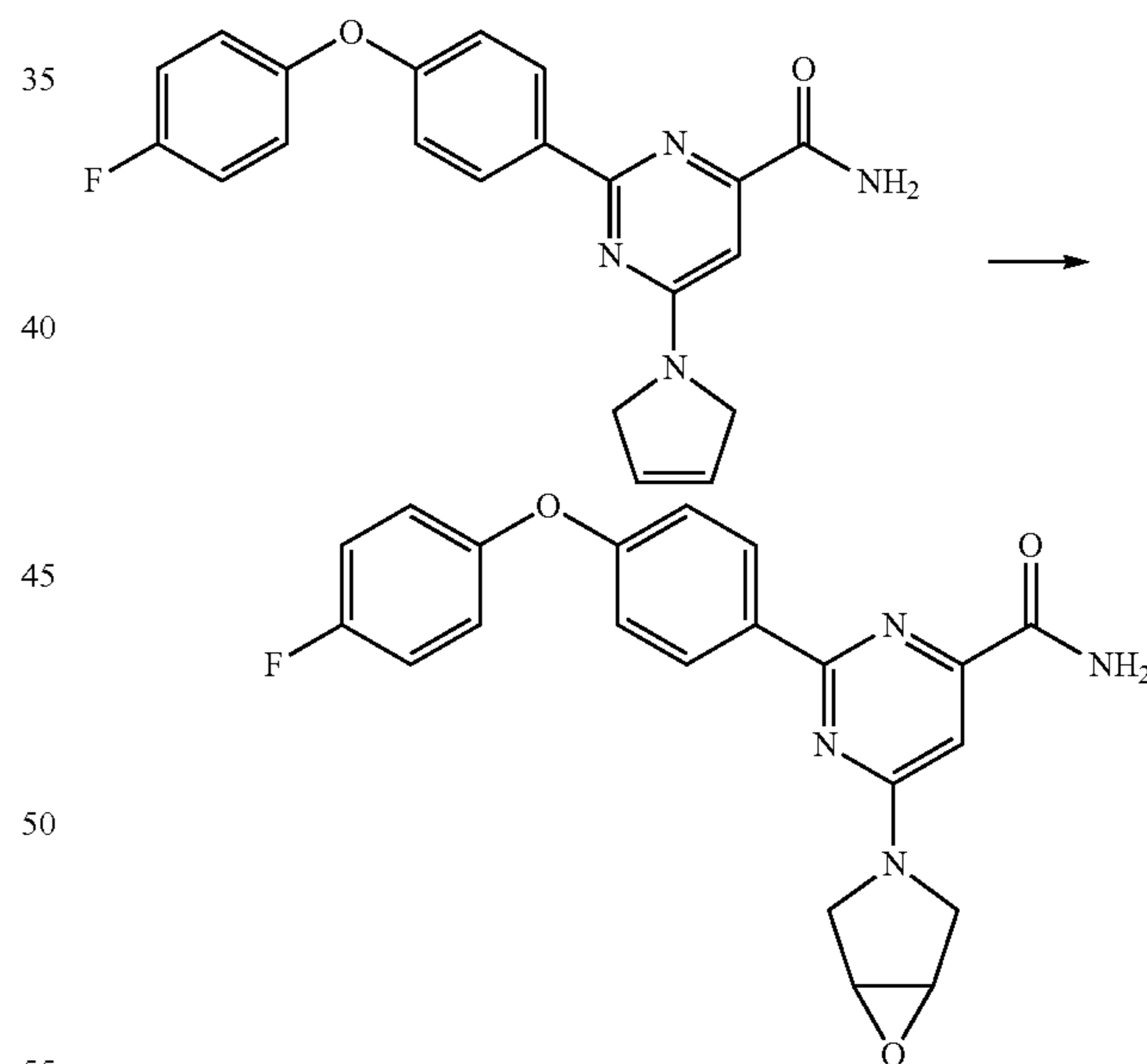
Scheme 25
