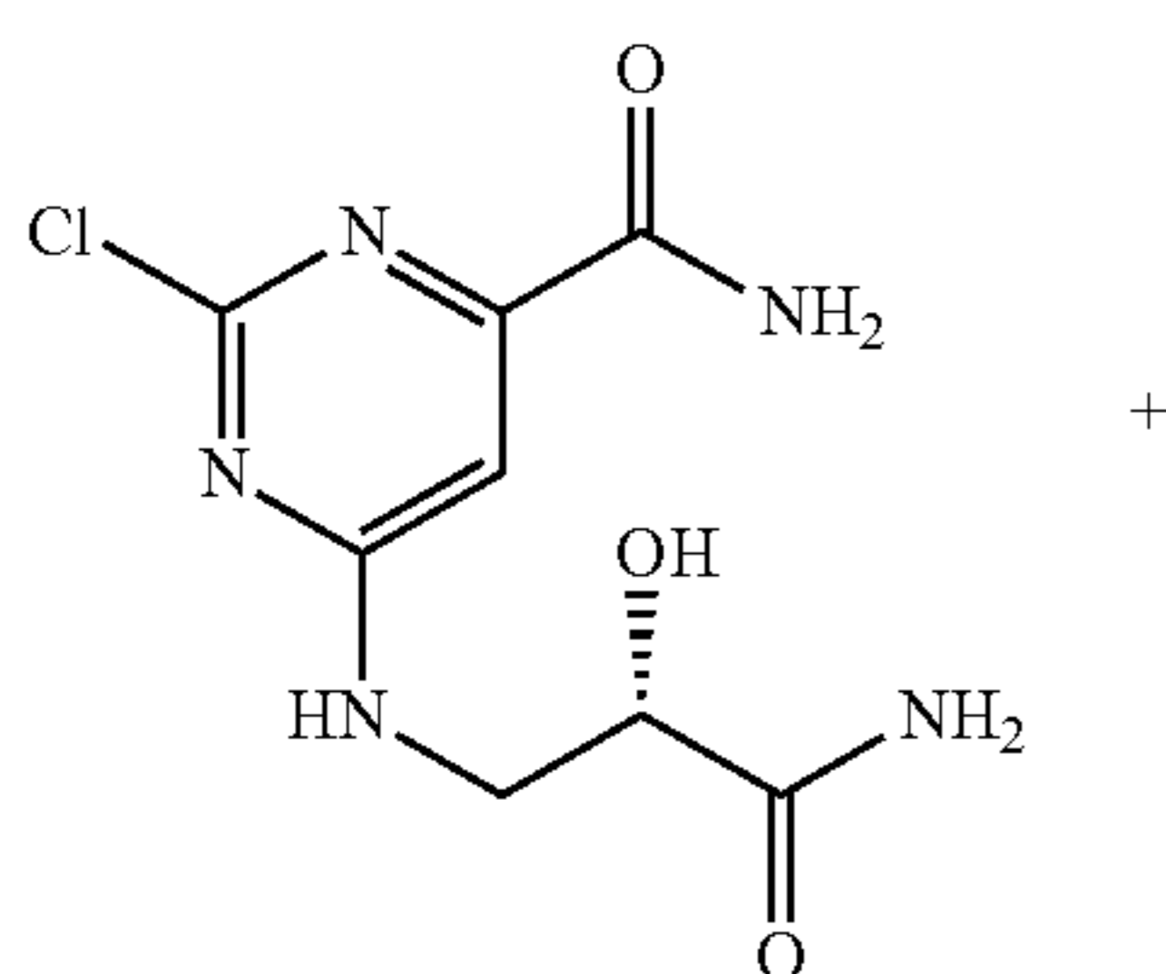
Scheme 30
