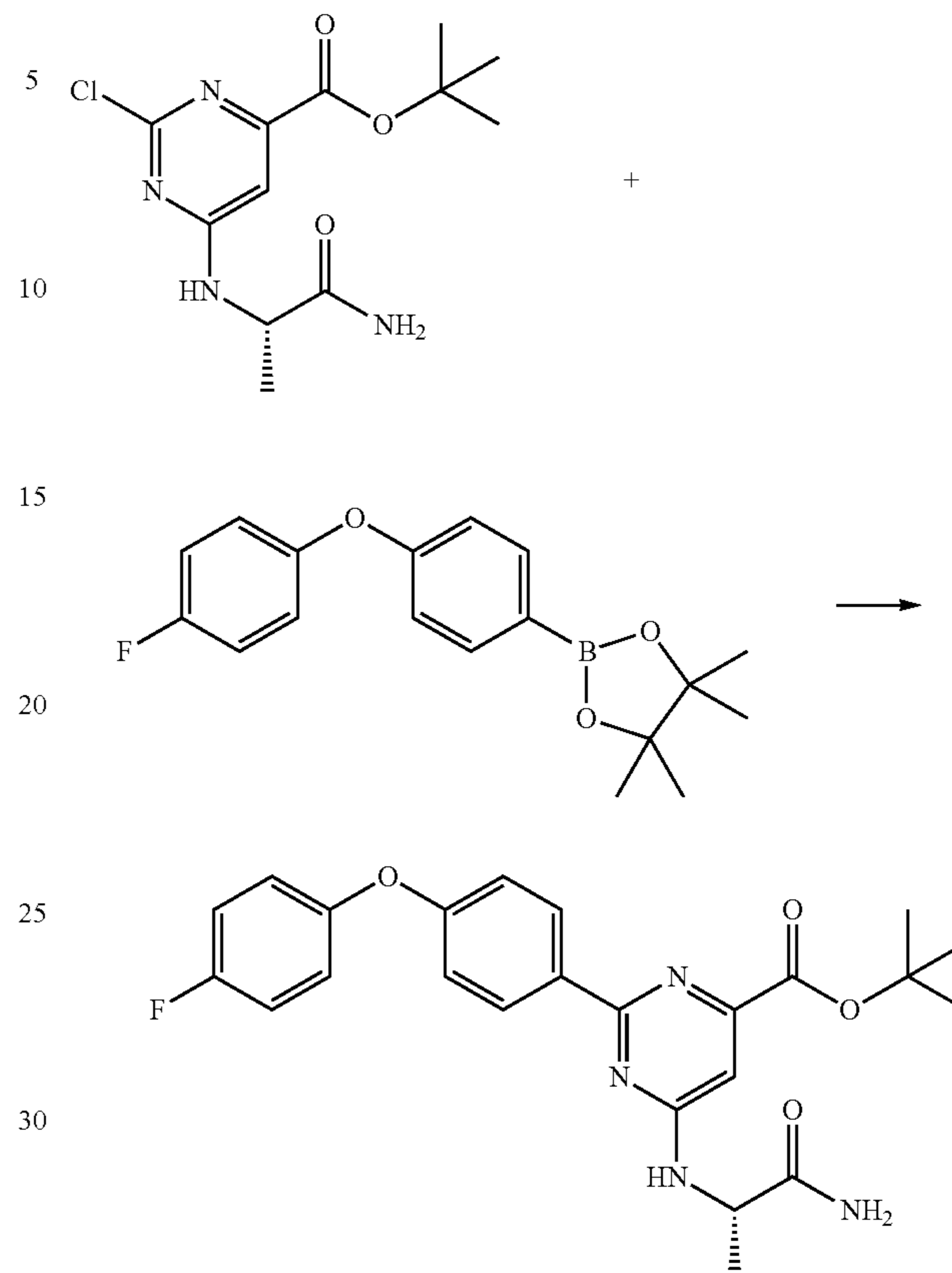
Scheme 15
