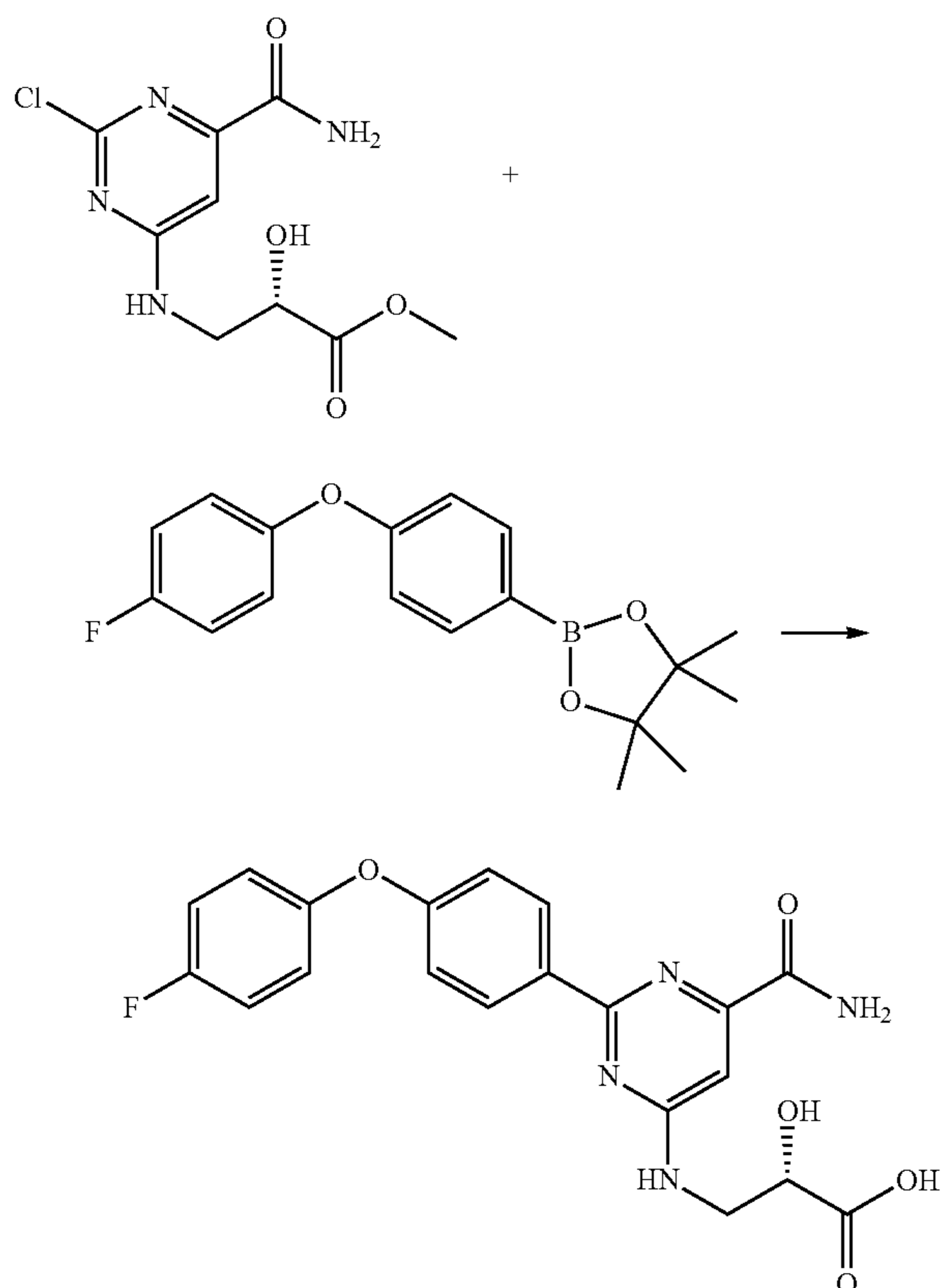
Scheme 31
