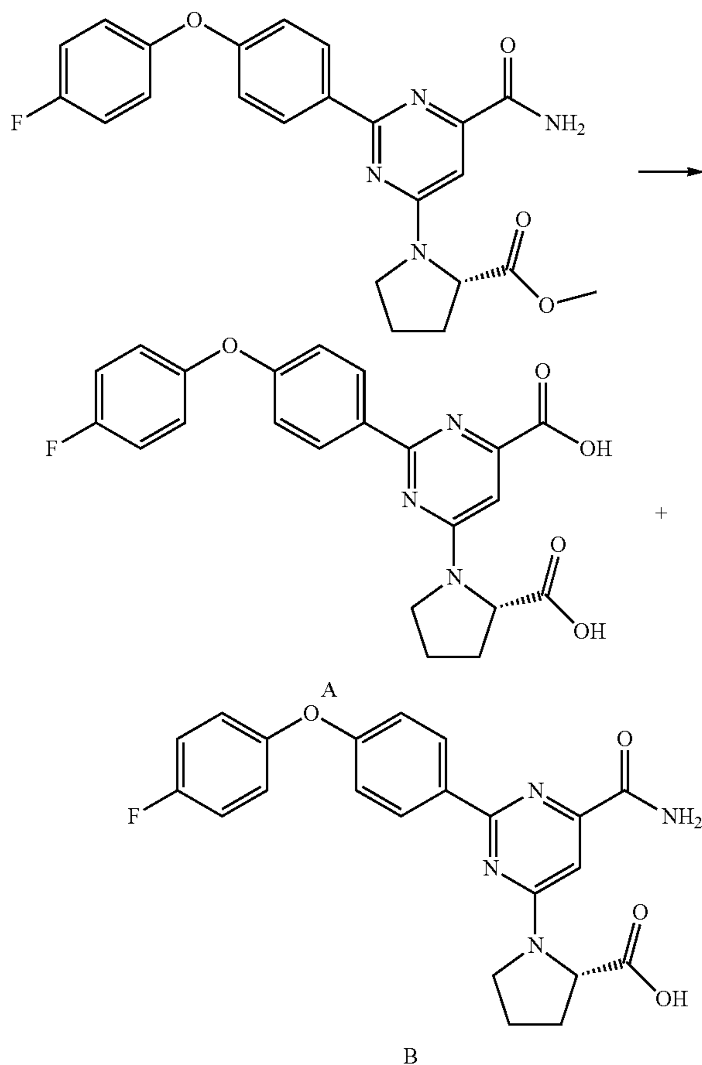
Scheme 9
