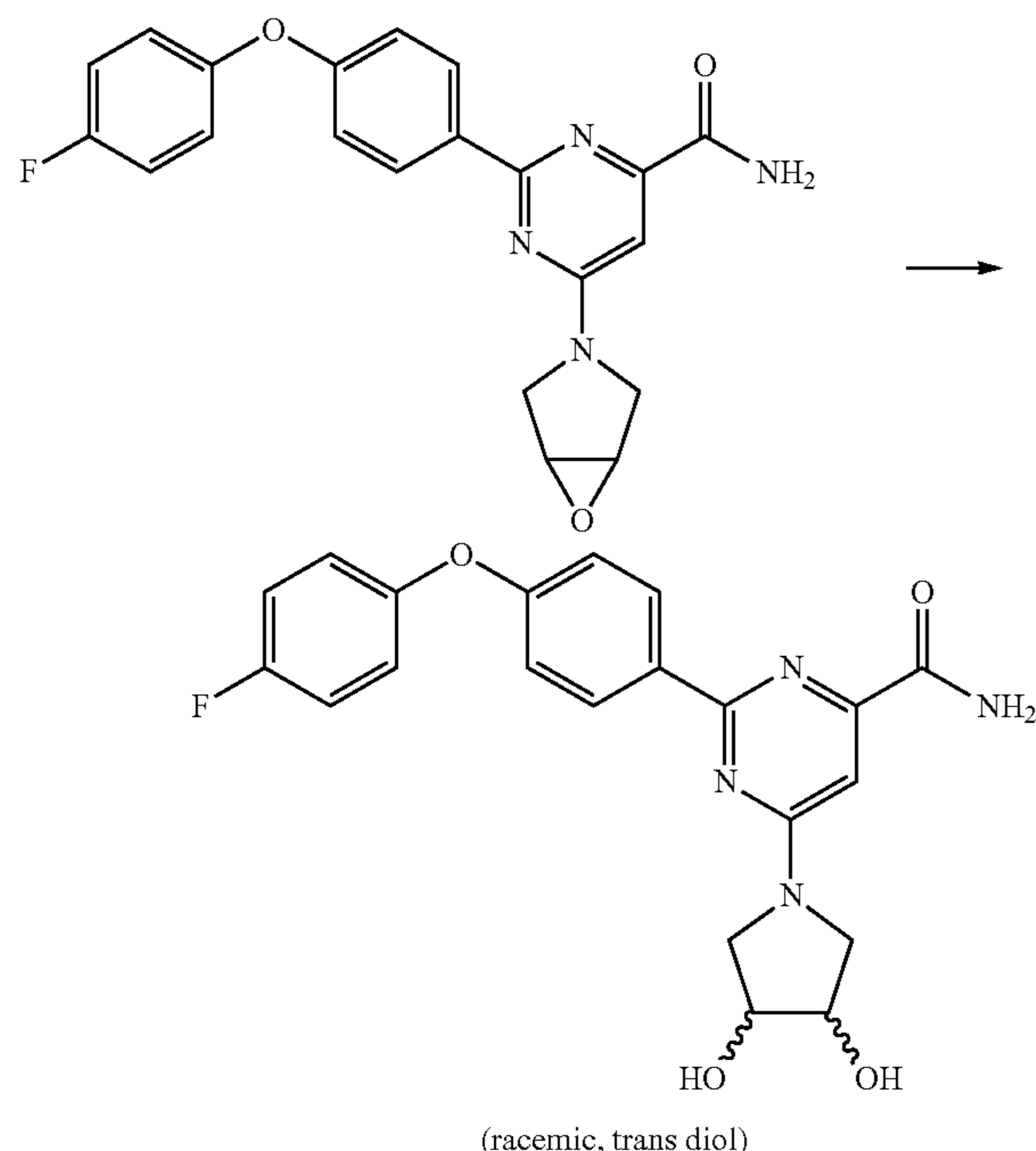
Scheme 26
