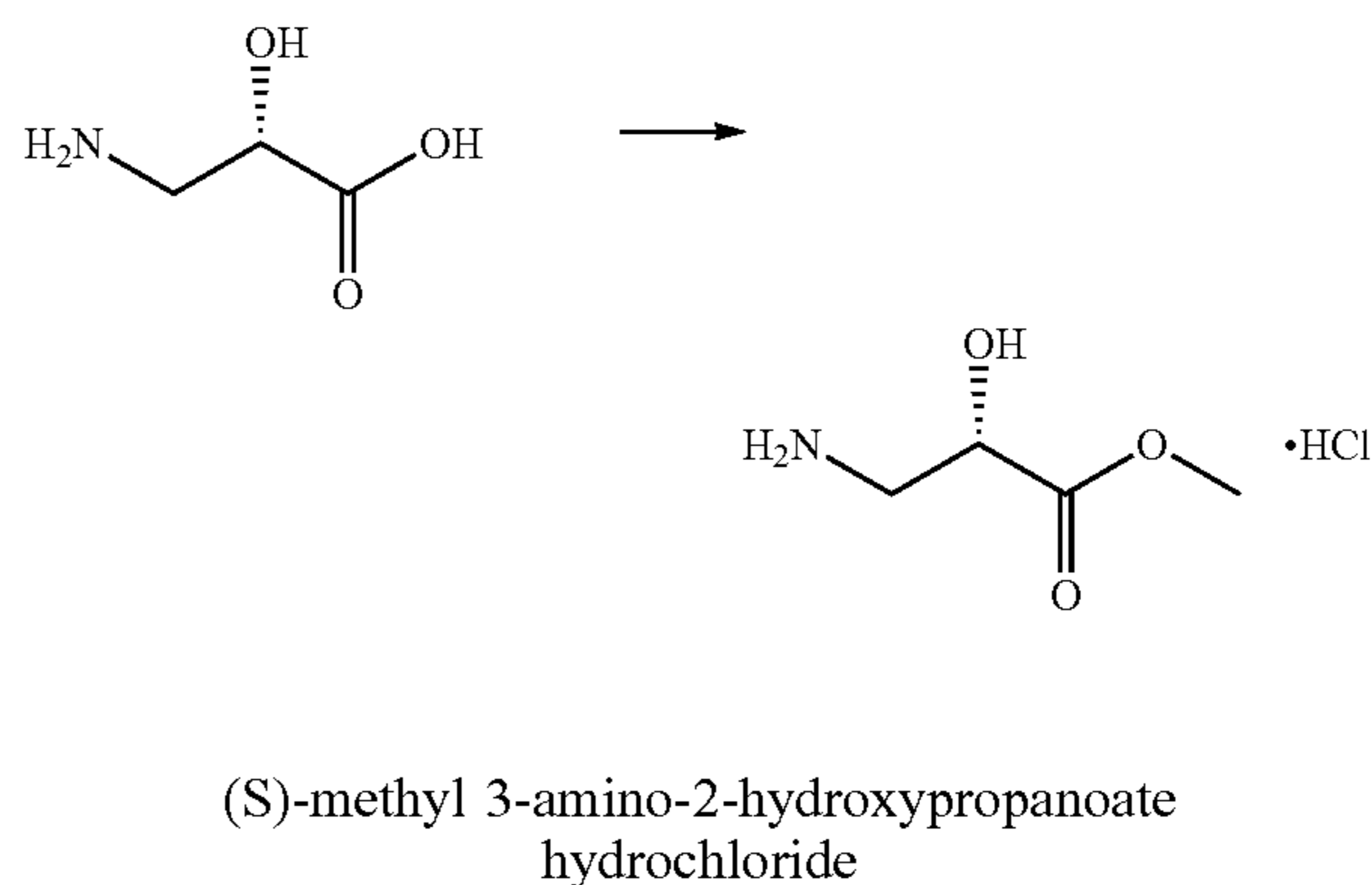
Scheme 27
