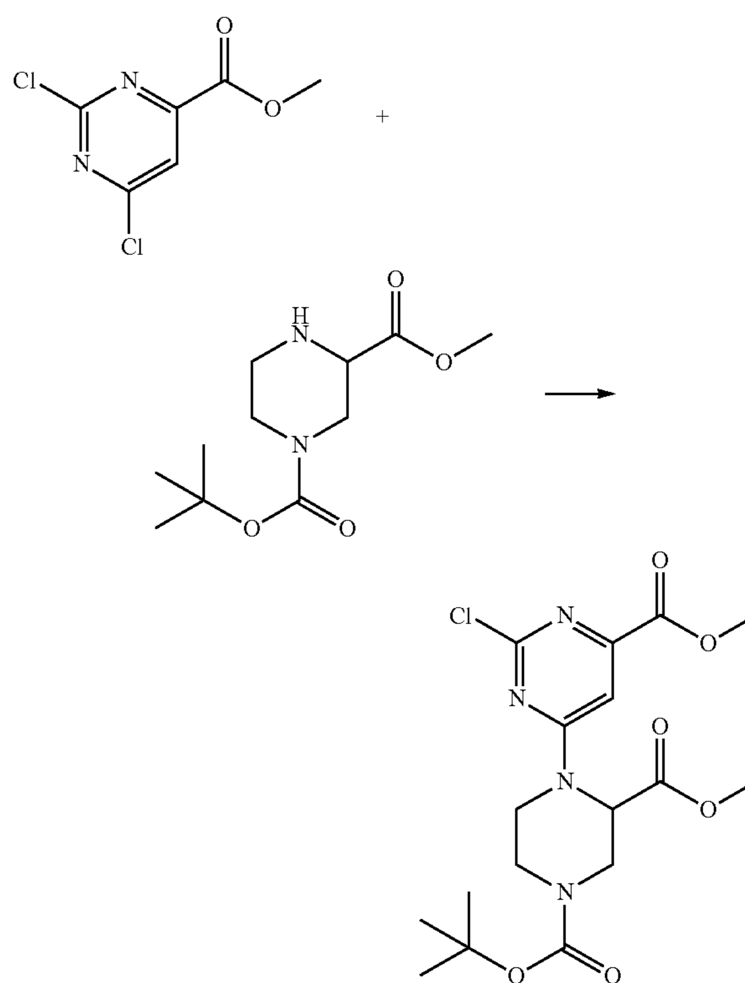
Scheme 61
