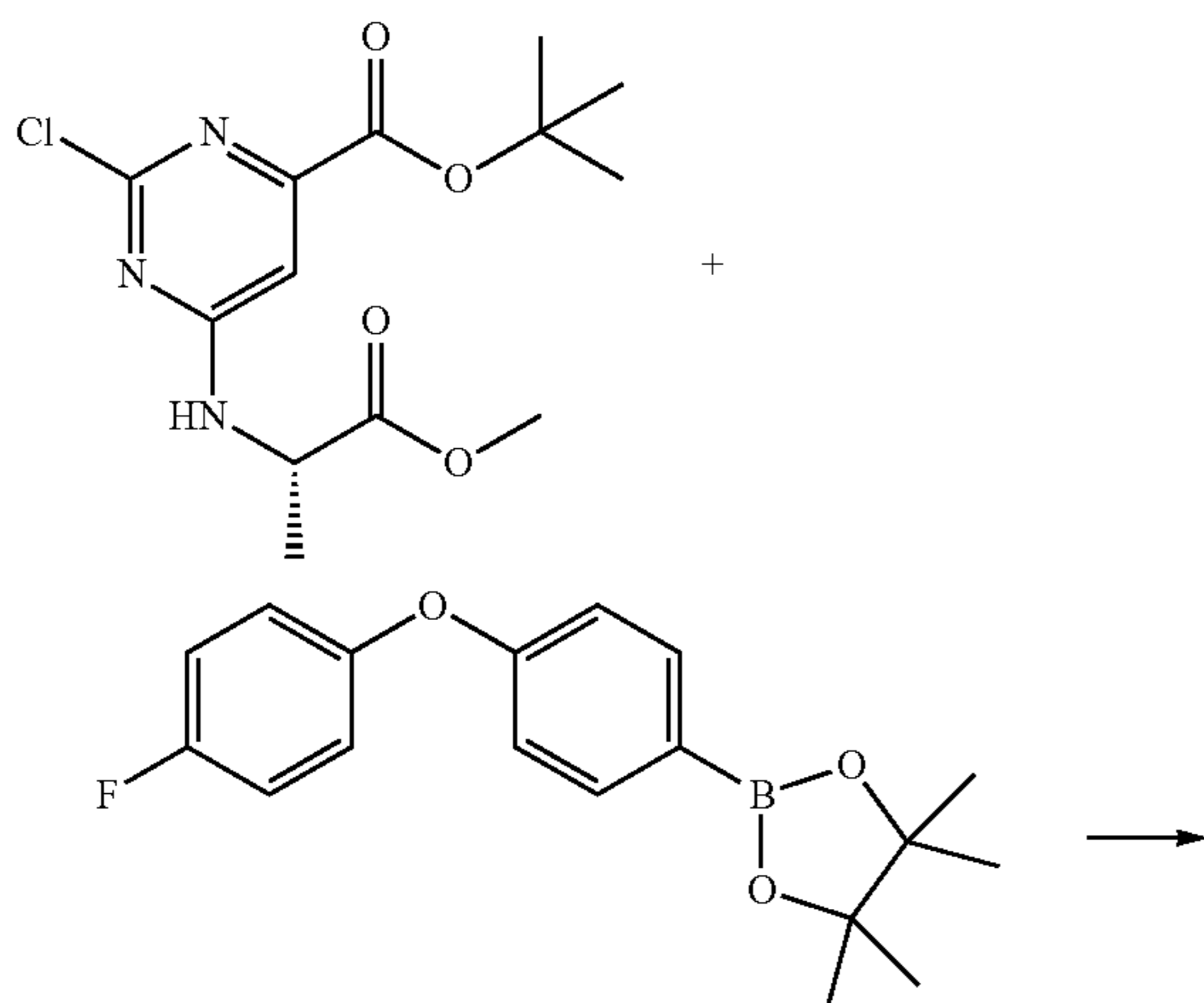
Scheme 12
