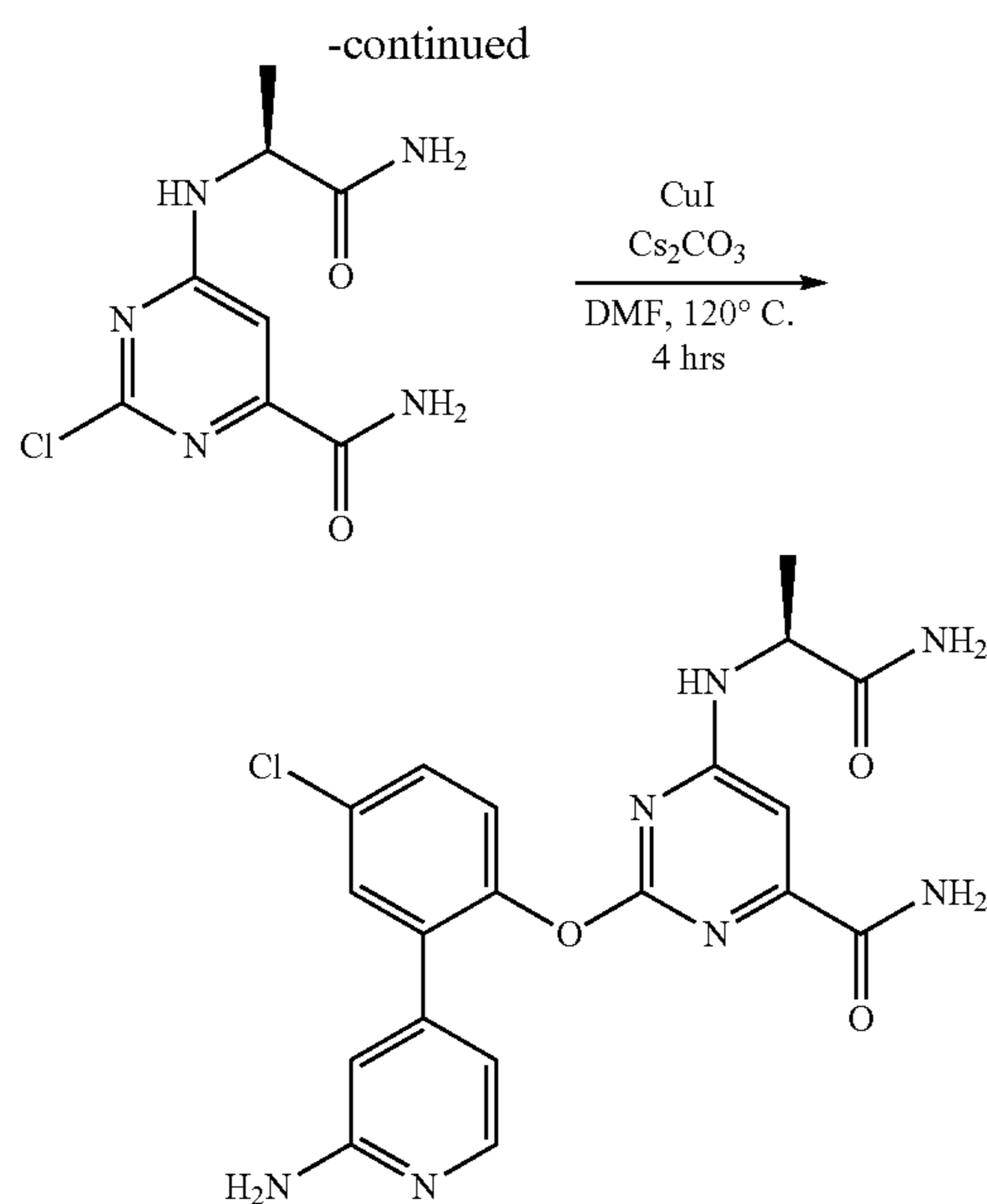
(S)-6-((1-amino-1-oxopropan-2-yl)amino)-2-(2-(2-aminopyridin-4-yl)-4-chlorophenoxy)pyrimidine-4-carboxamide
