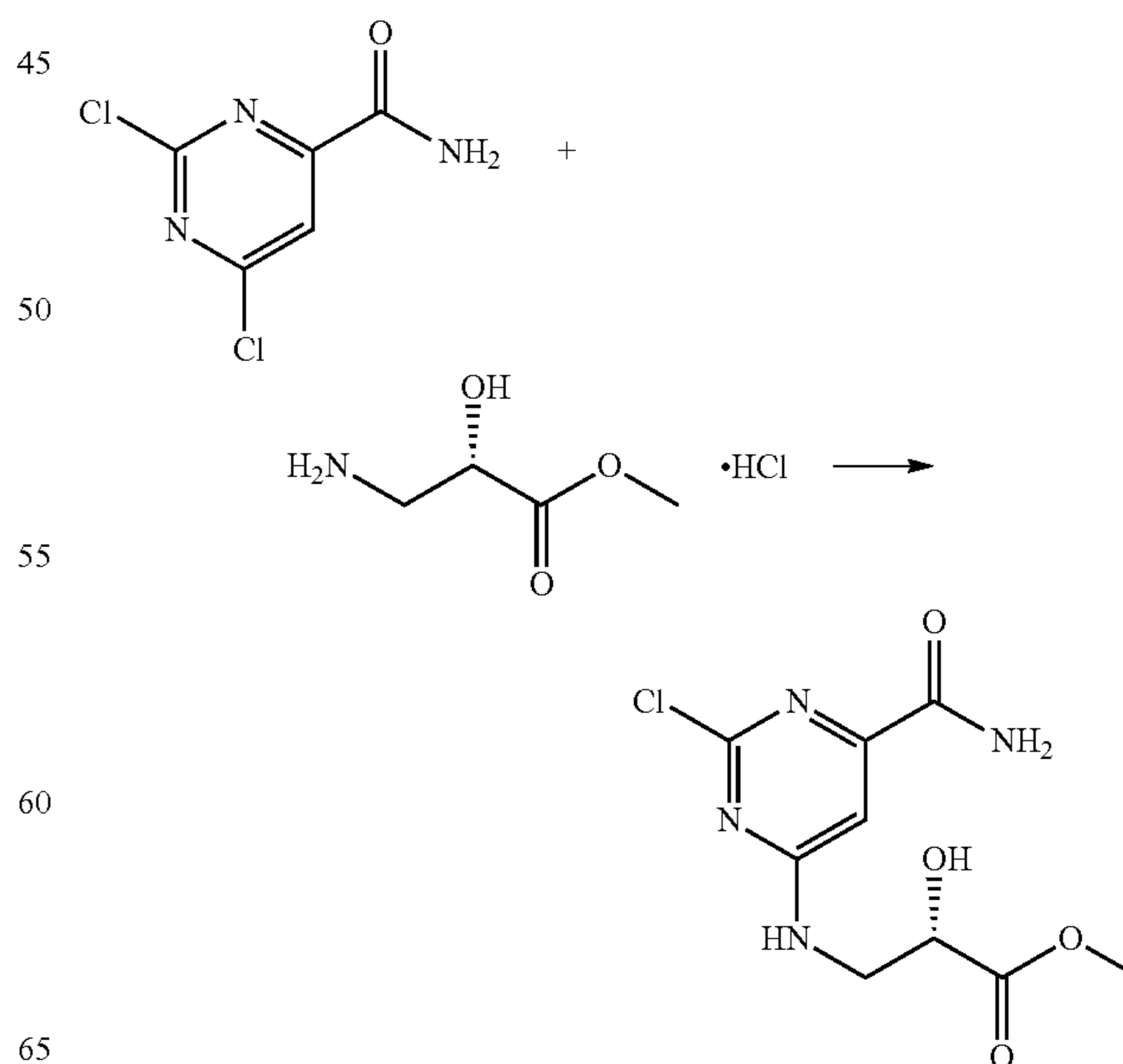
Scheme 28
