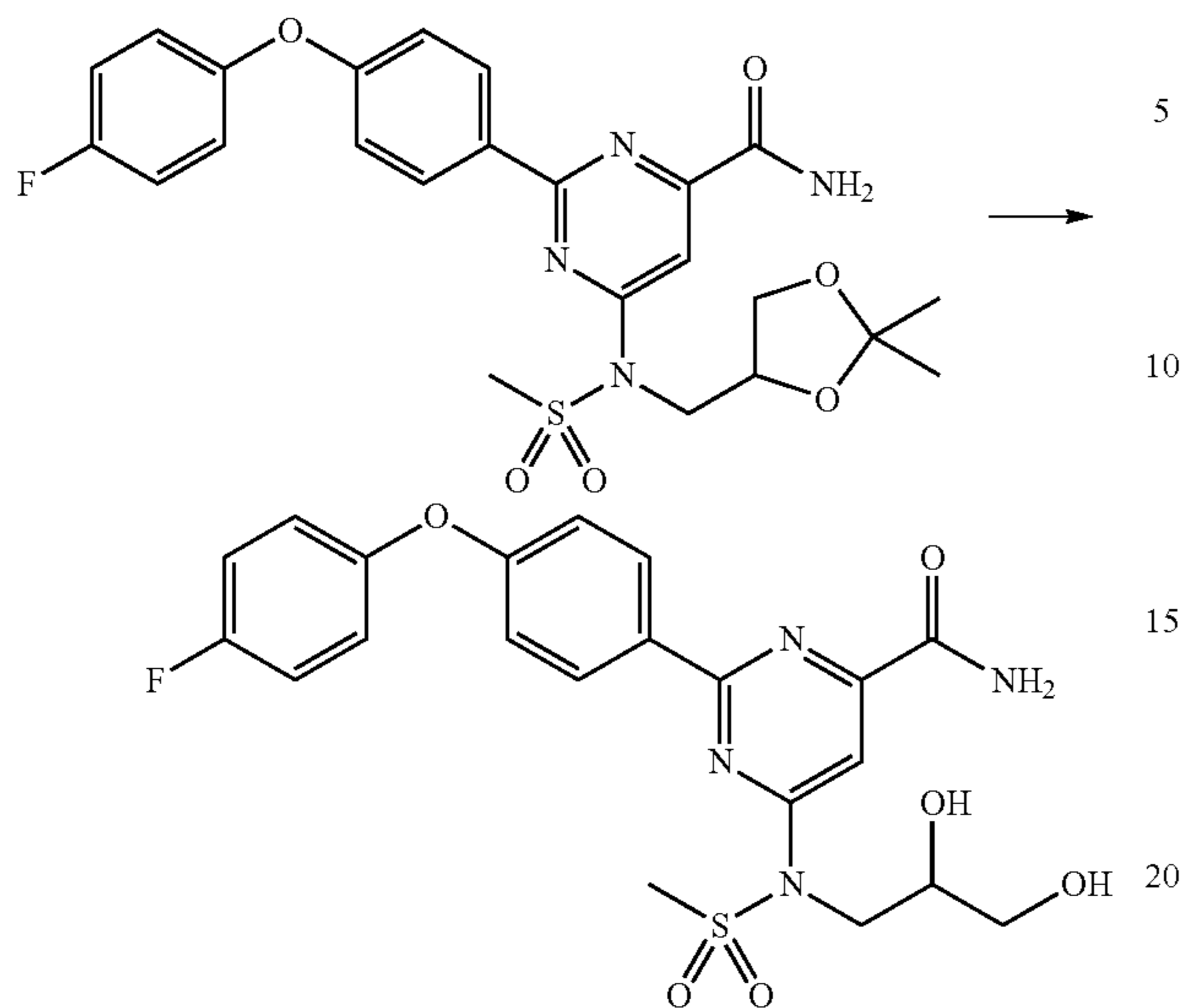
Scheme 36
