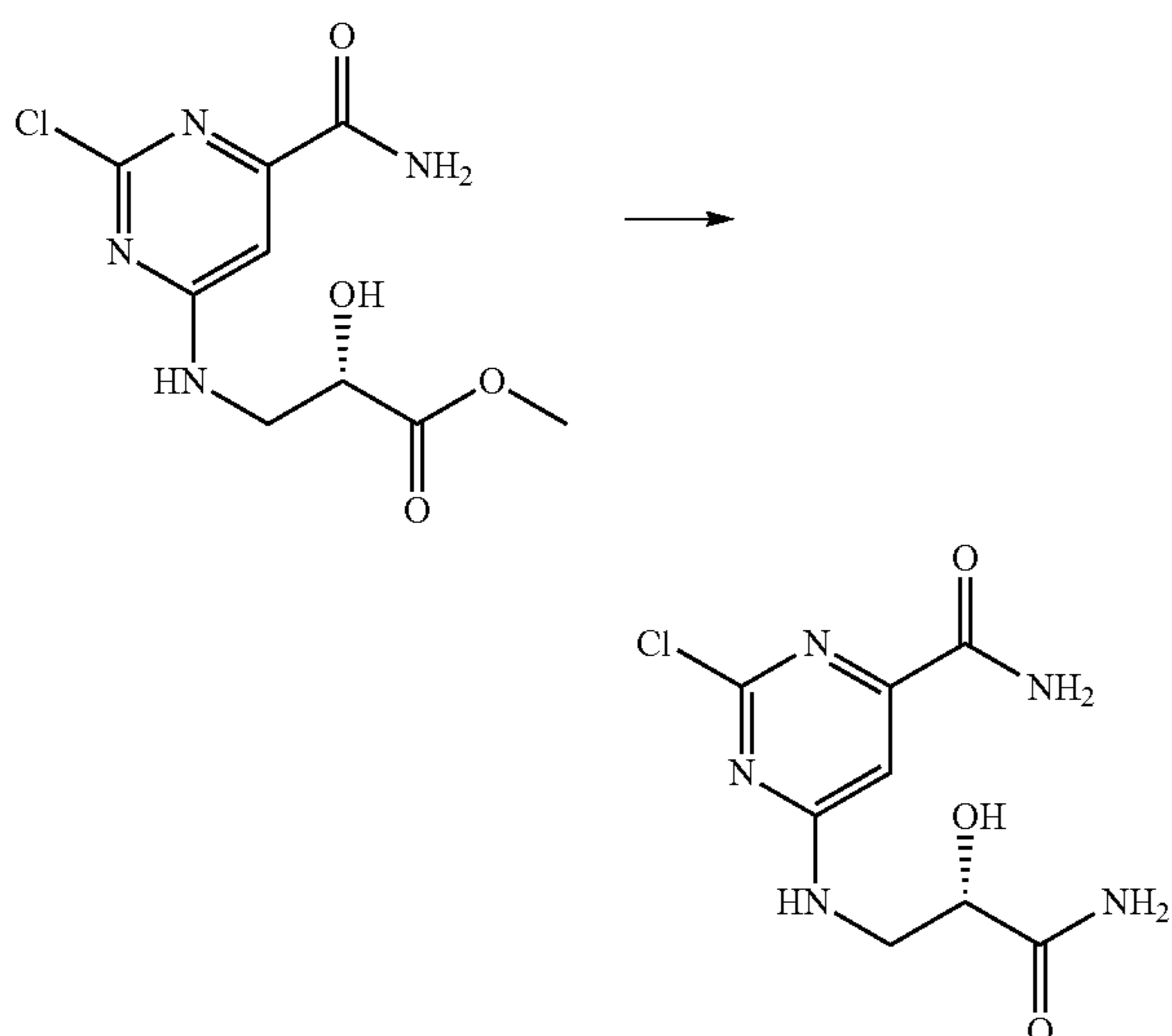
Scheme 29
