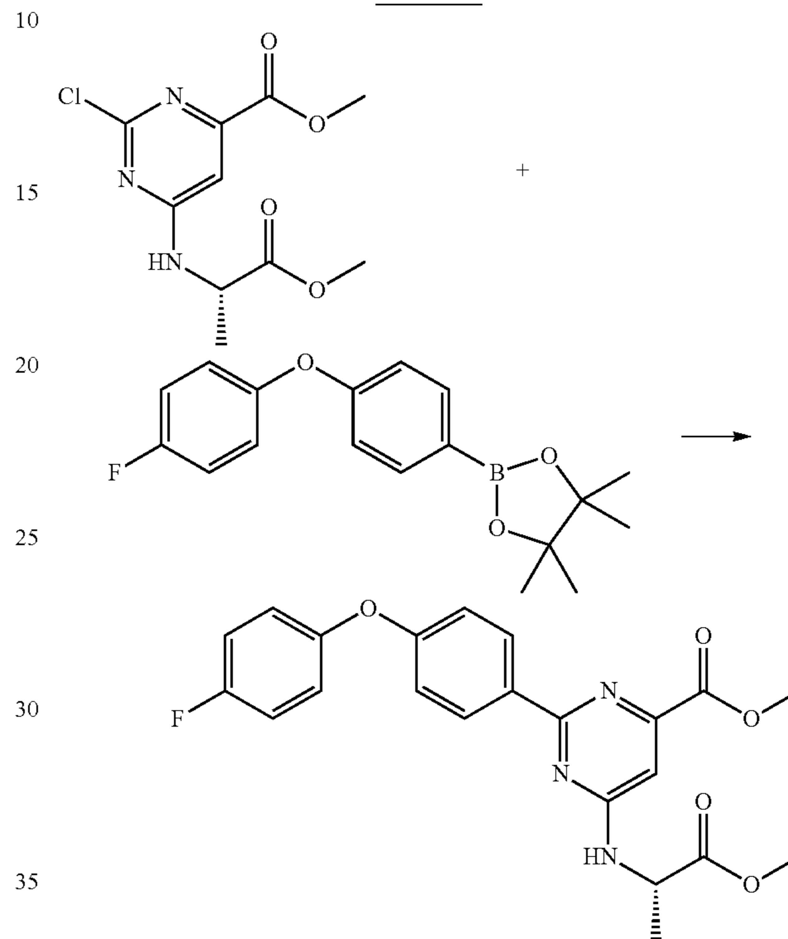
Scheme 20
