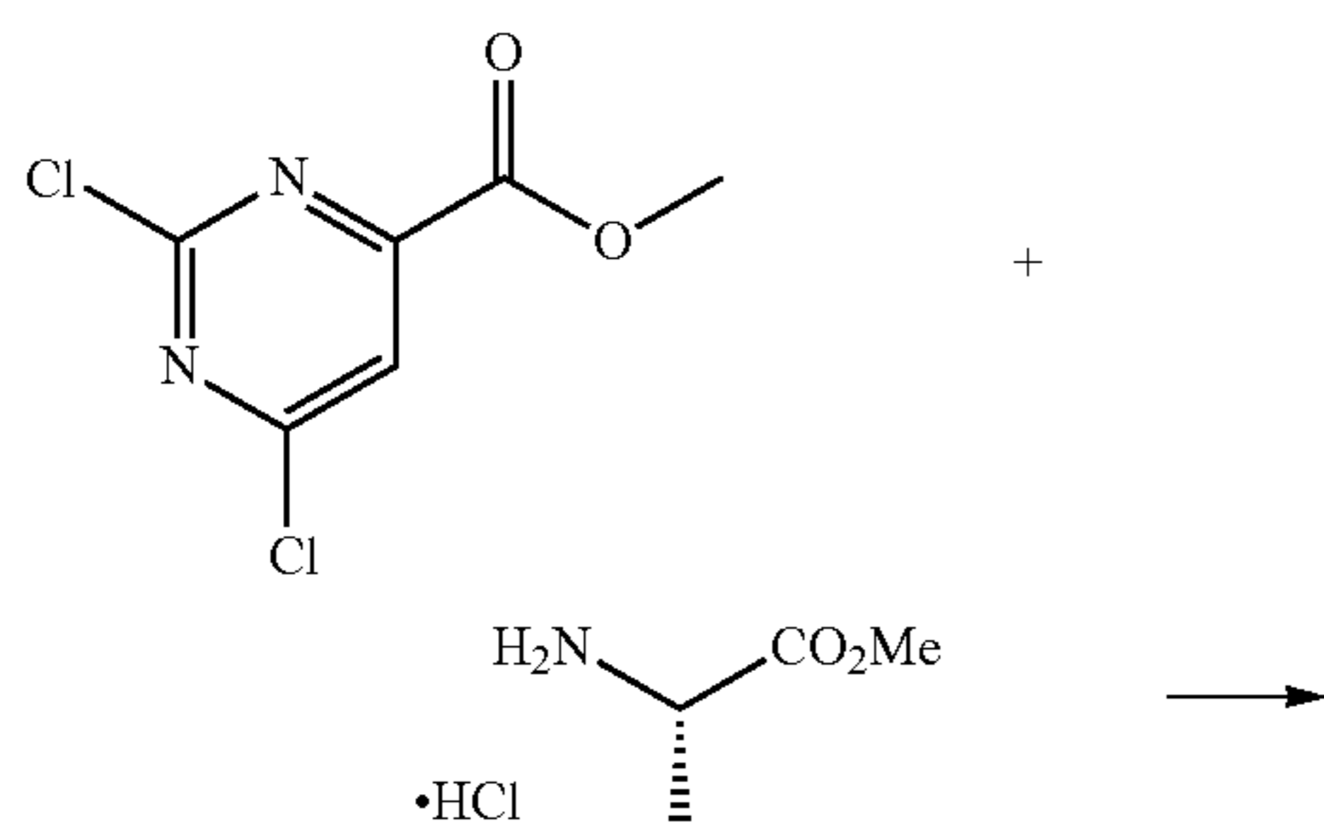
Scheme 17
