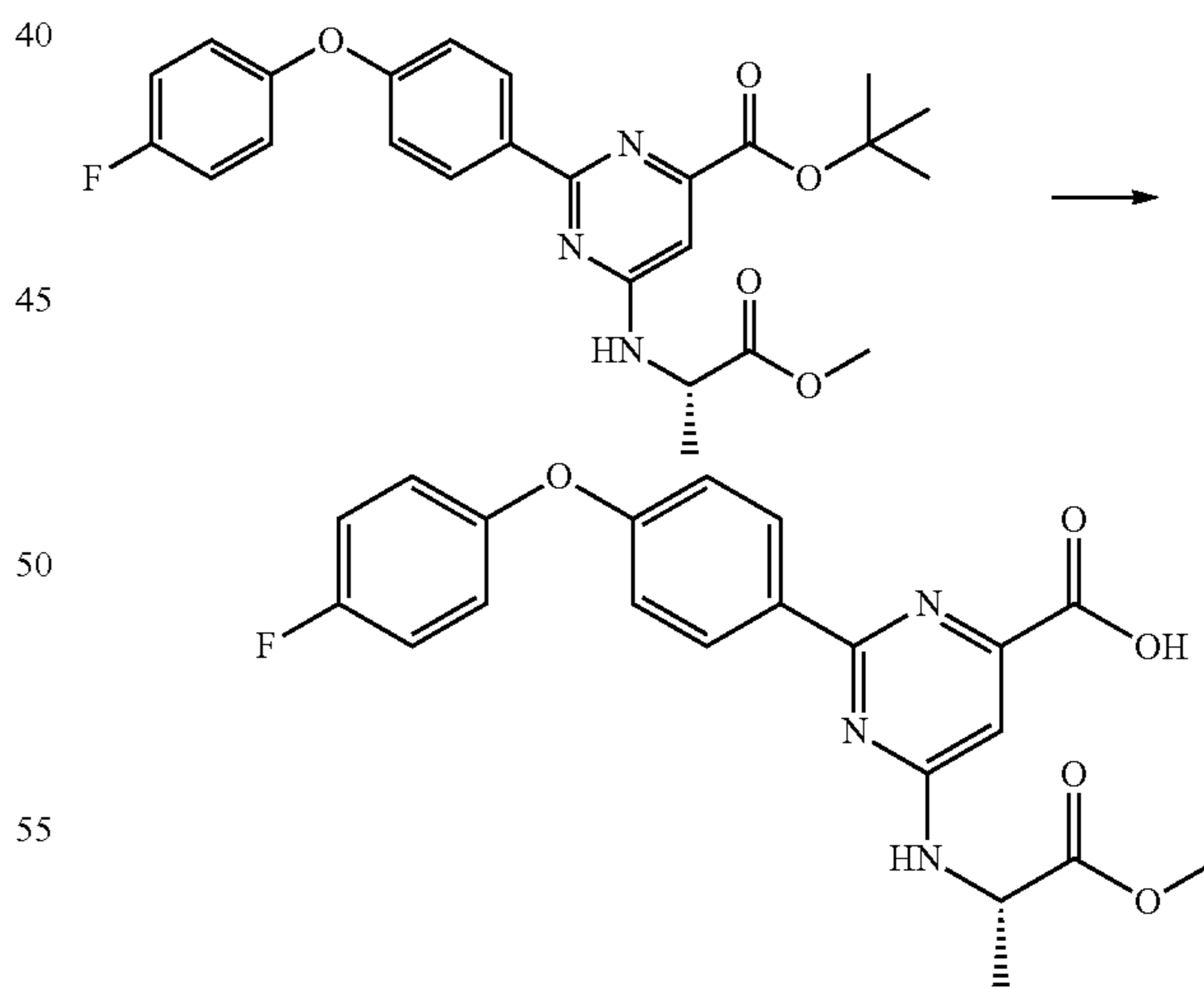
Scheme 13
