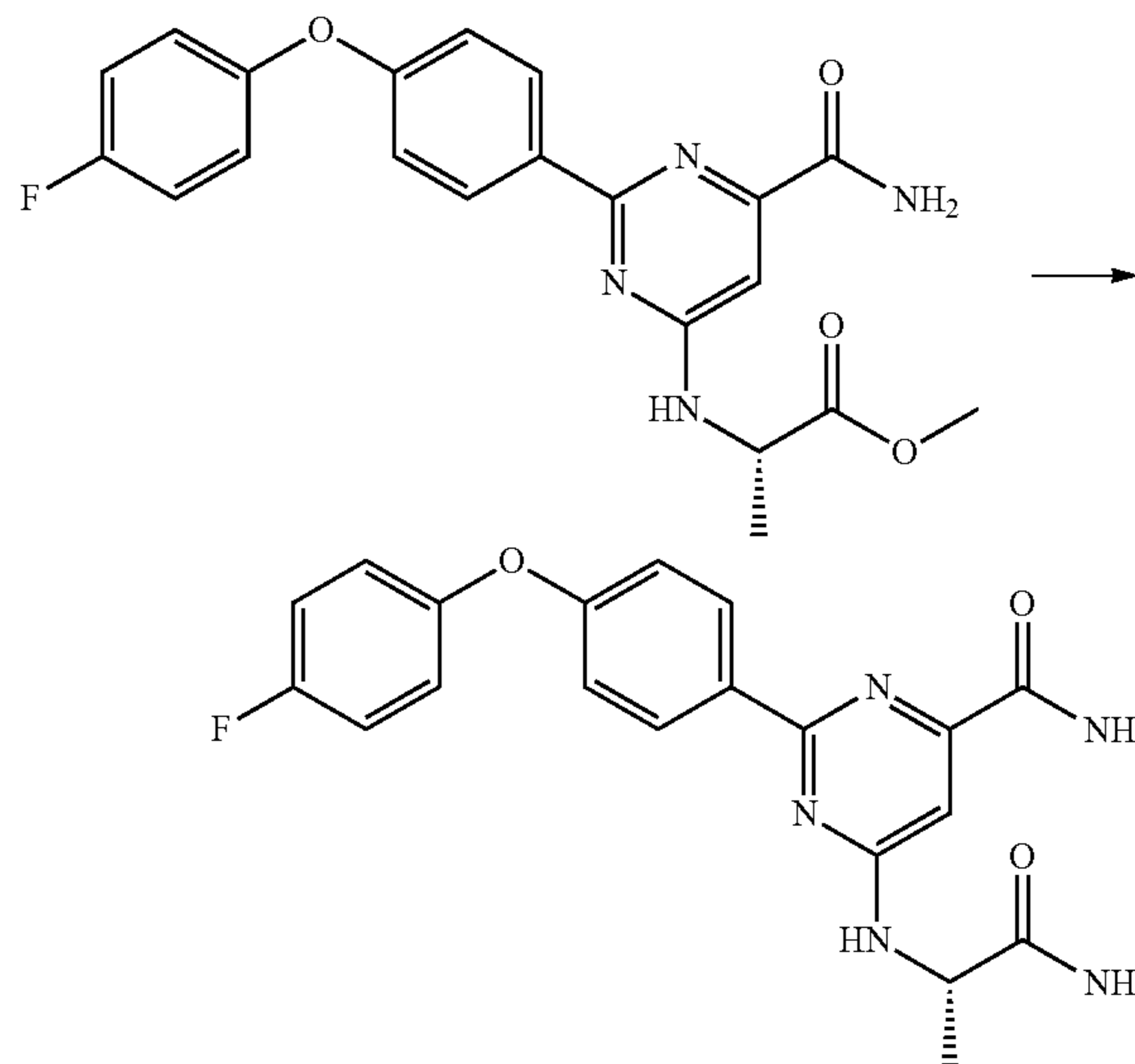
Scheme 6
