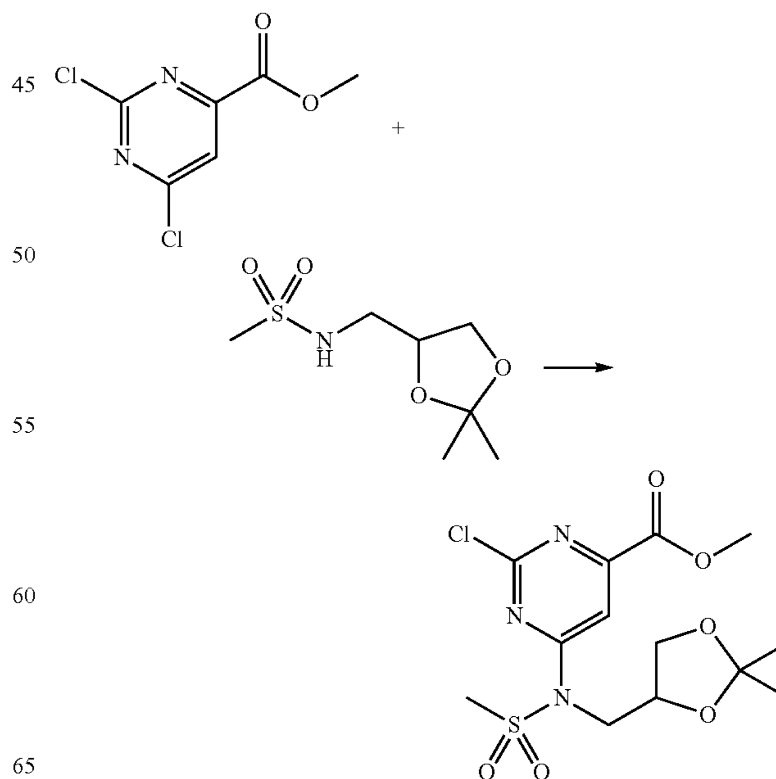
Scheme 33
