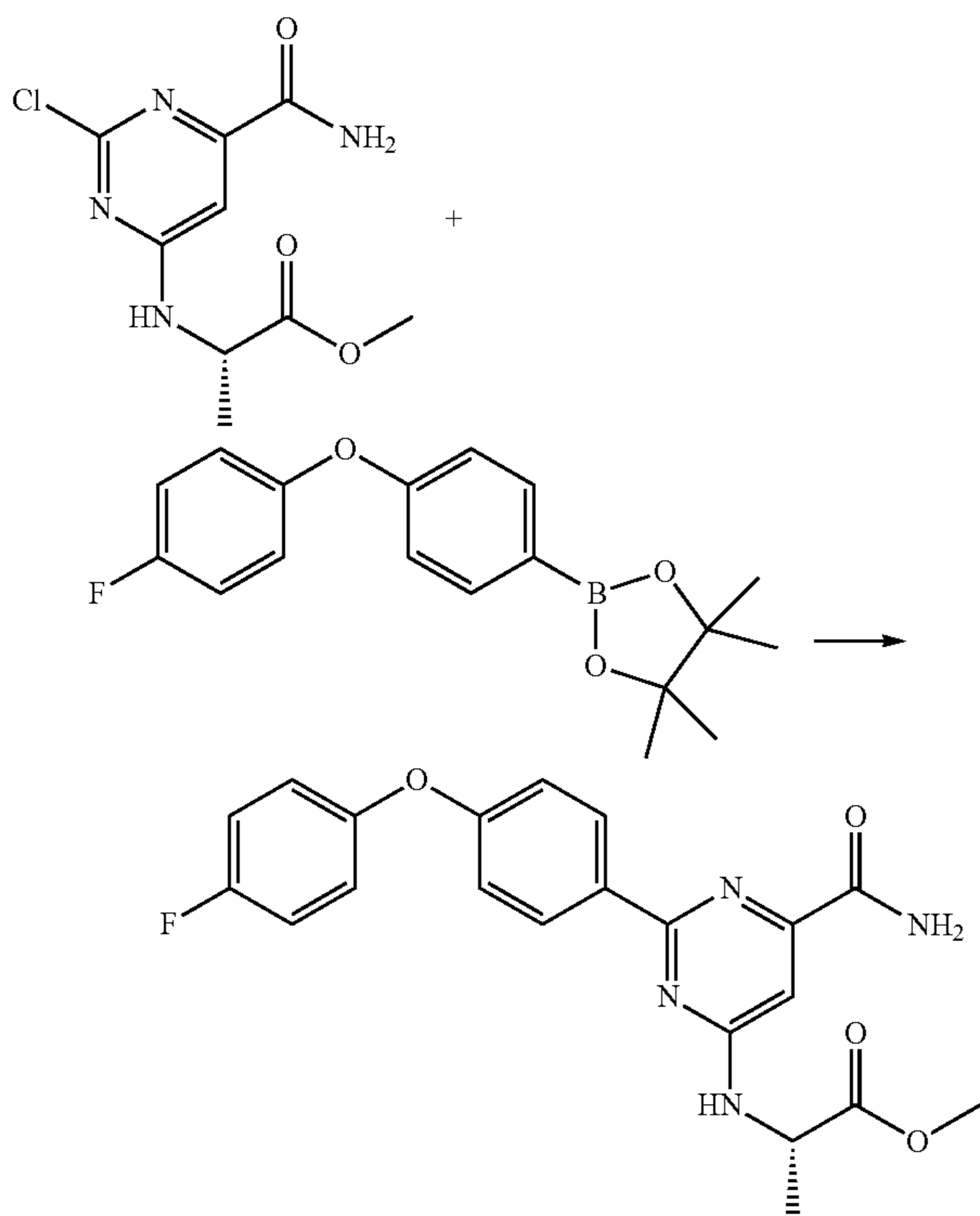
Scheme 5
