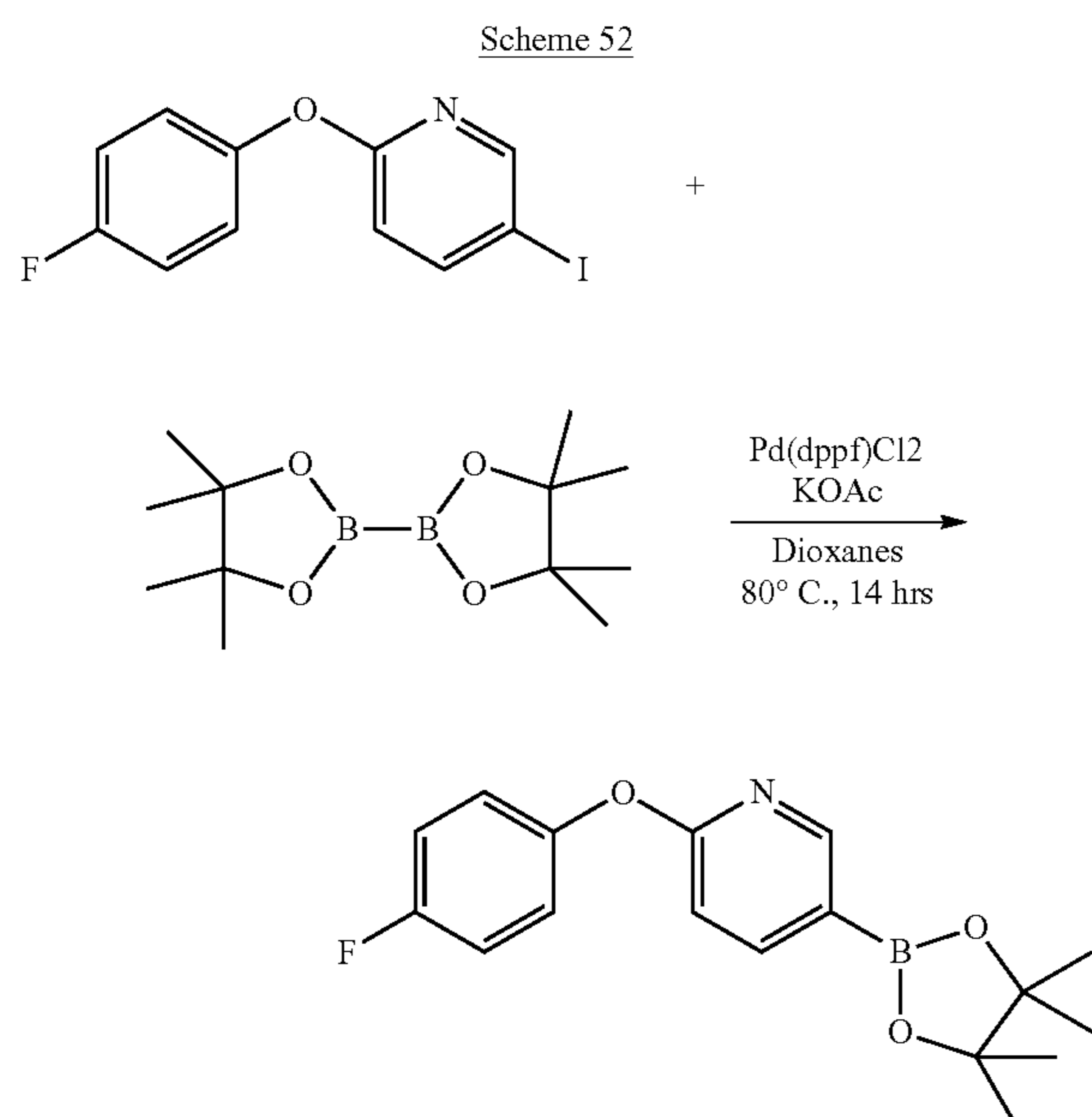
2-(4-fluorophenoxy)-5-(4,4,5,5-tetramethyl-1,3,2-dioxaborolan-2-yl)pyridine
