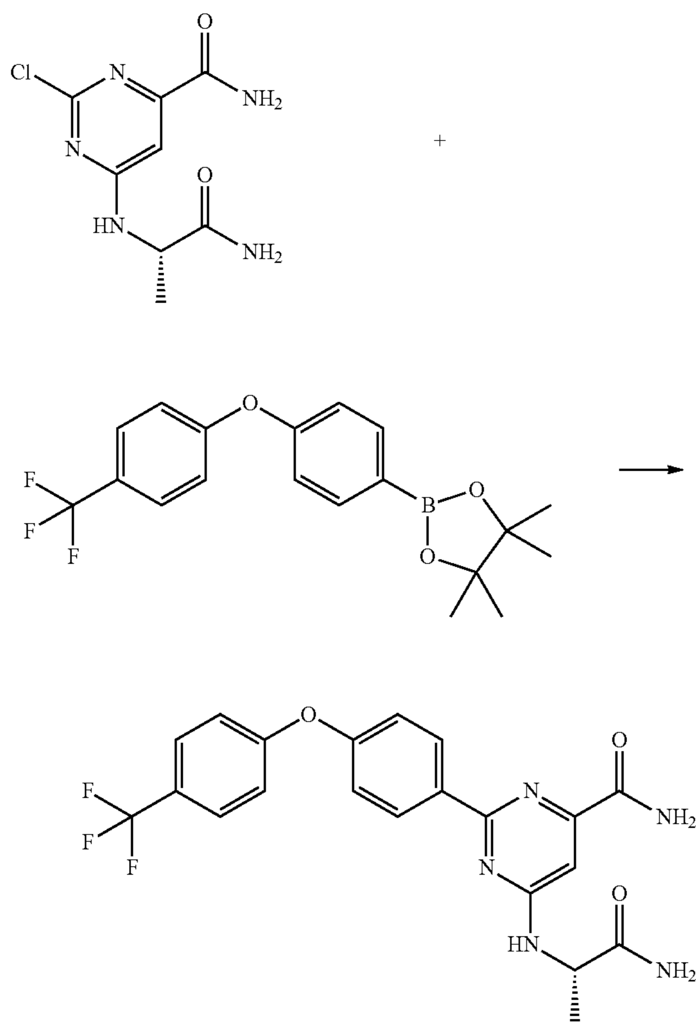
Scheme 19
