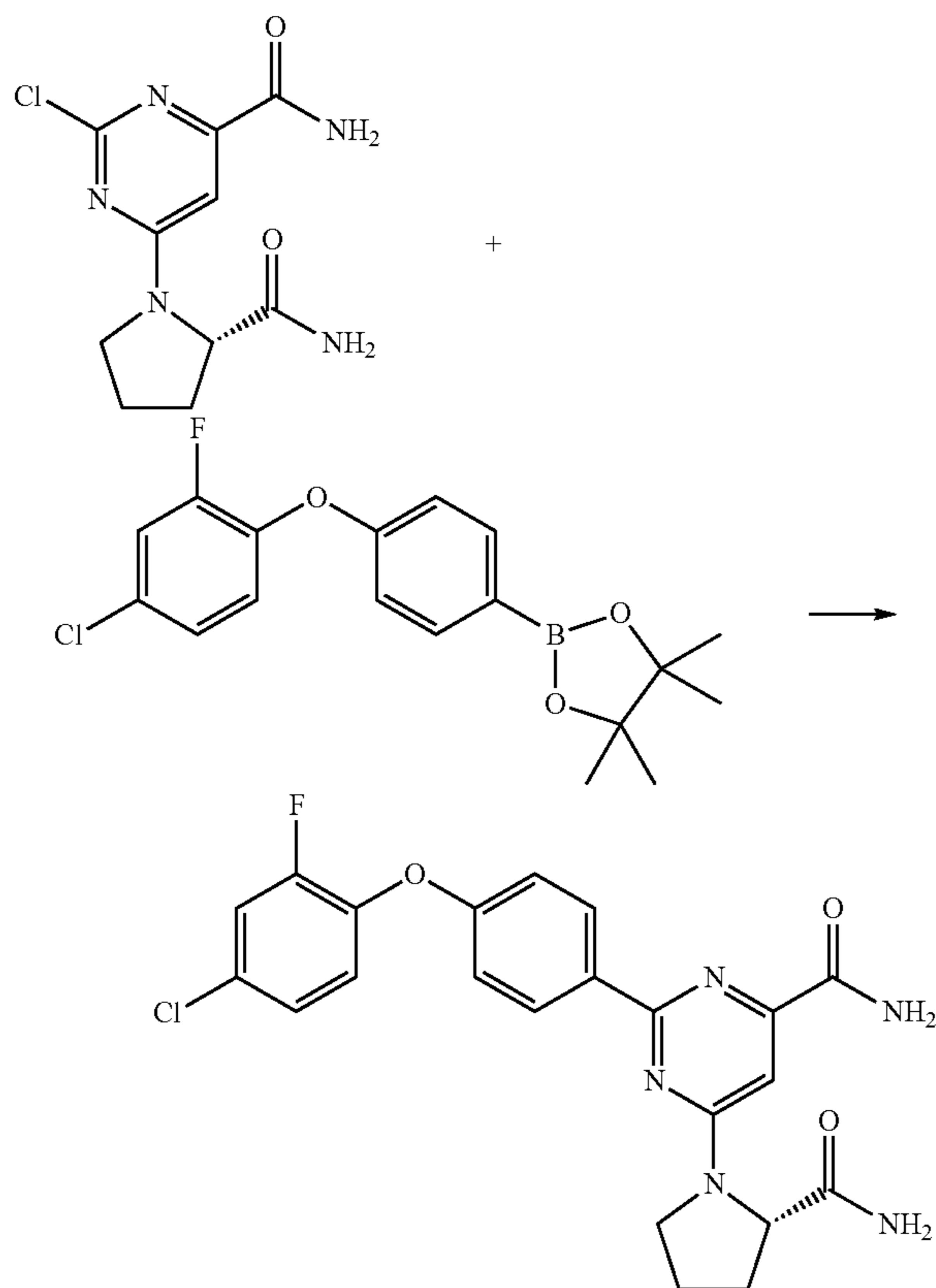
Scheme 57
