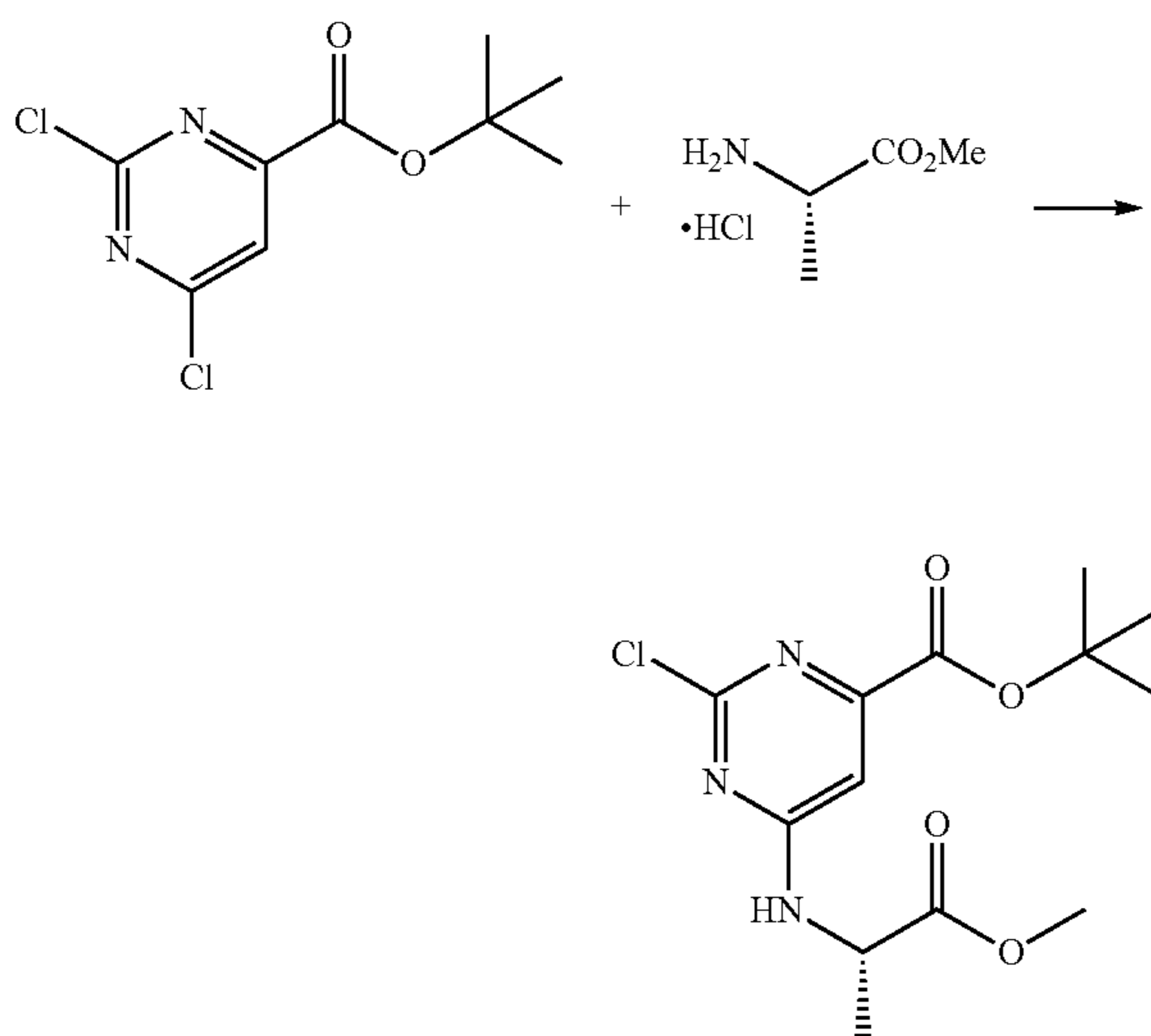
Scheme 11
