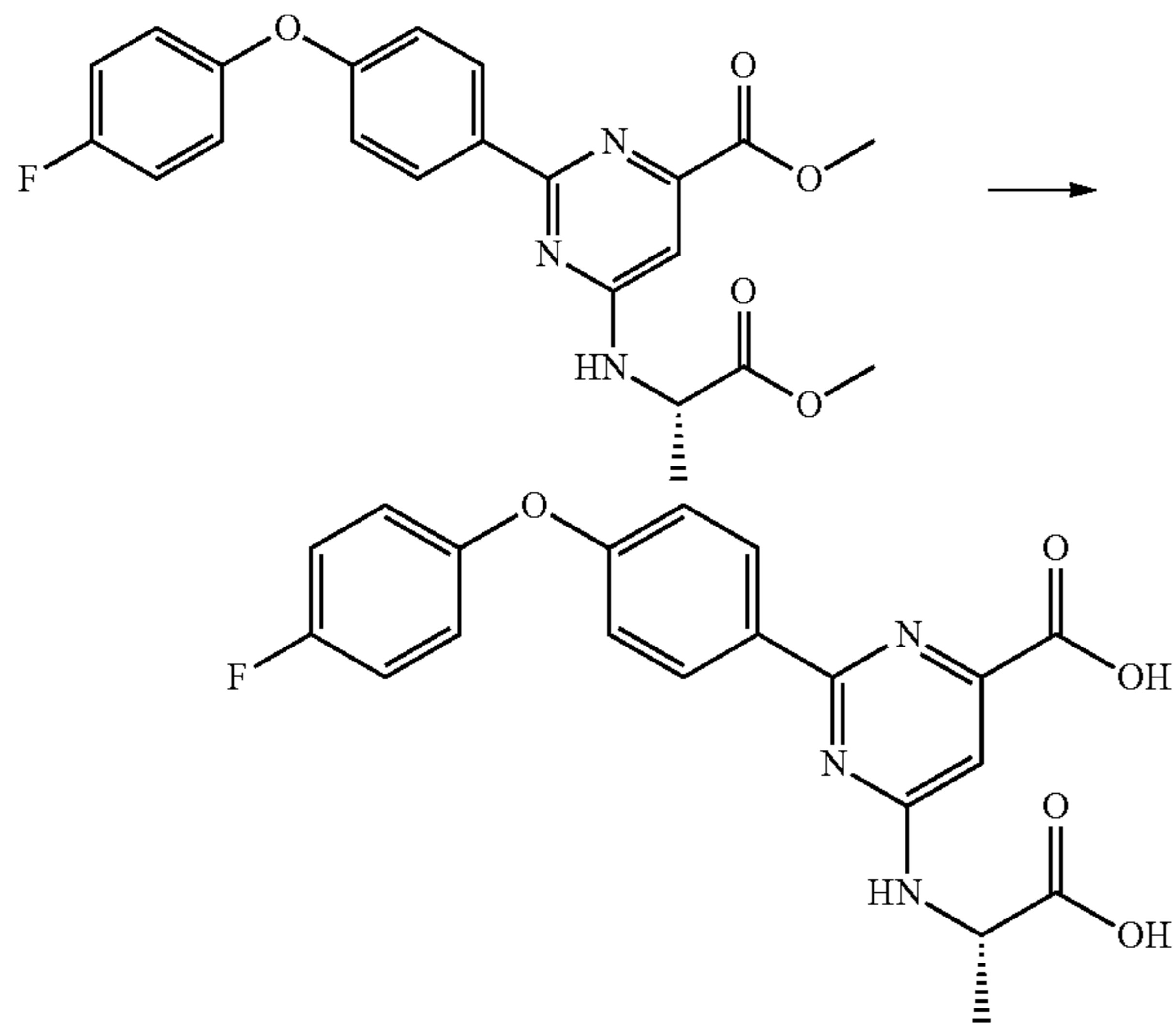
Scheme 21
