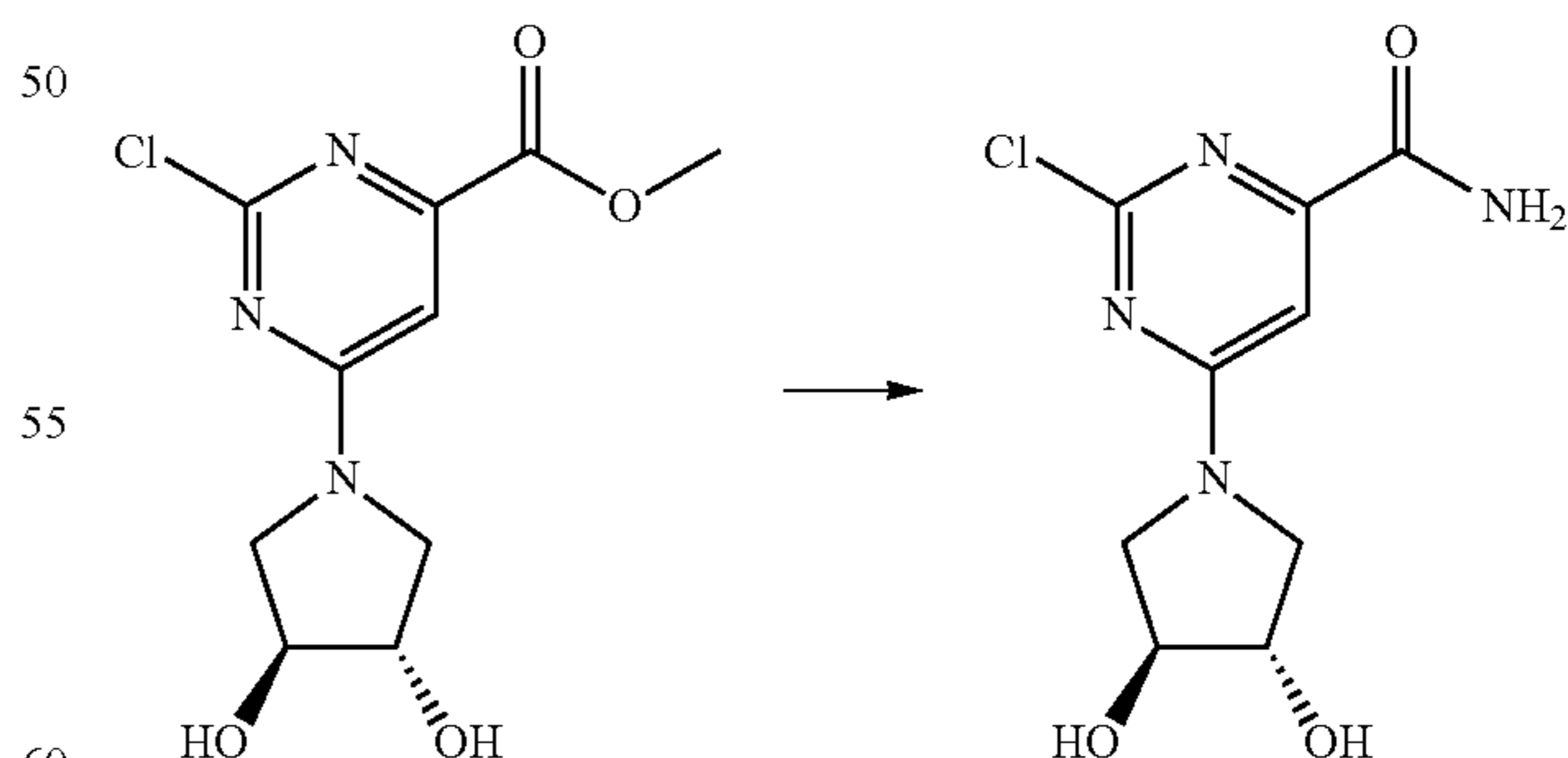
Scheme 59
