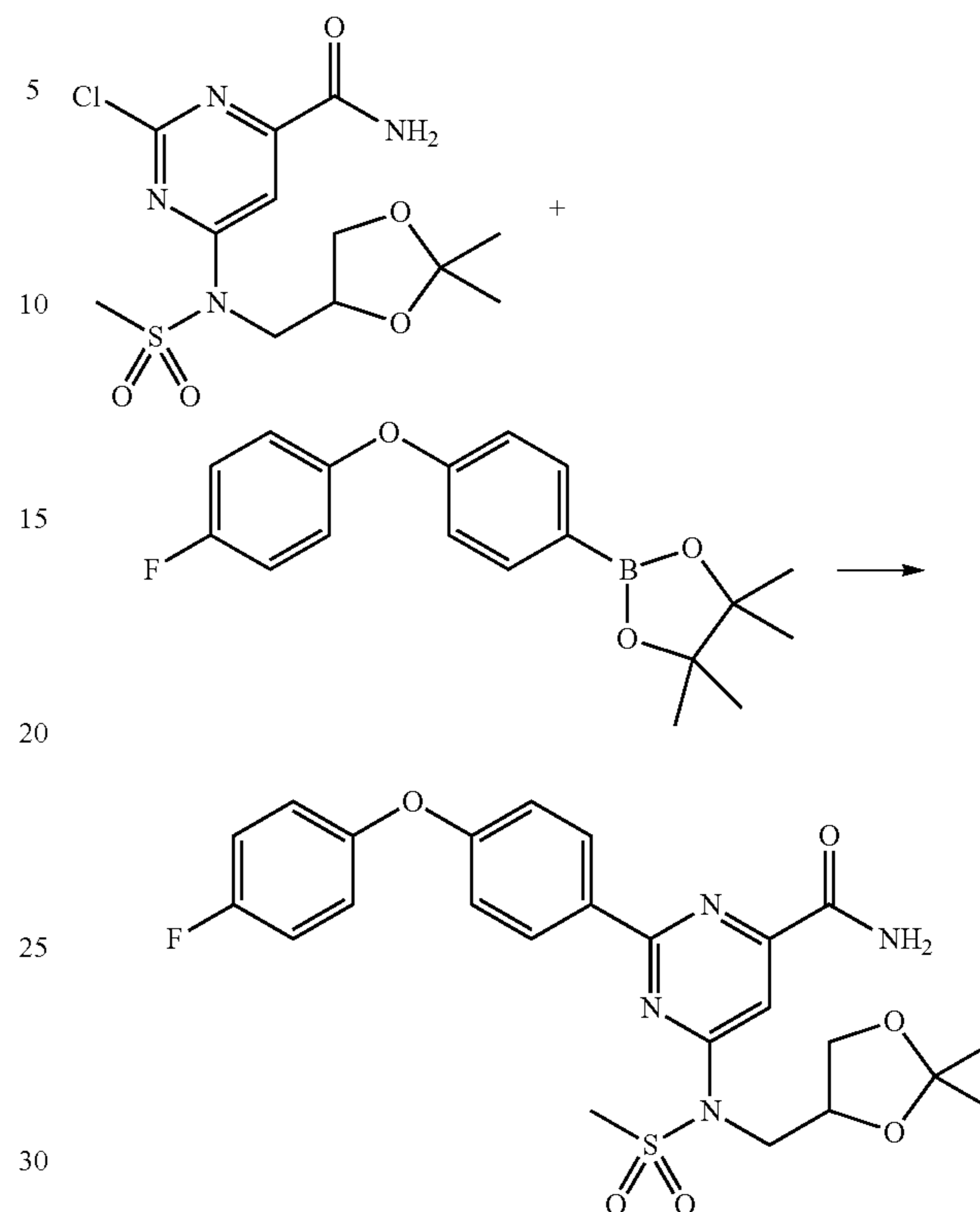
Scheme 35
