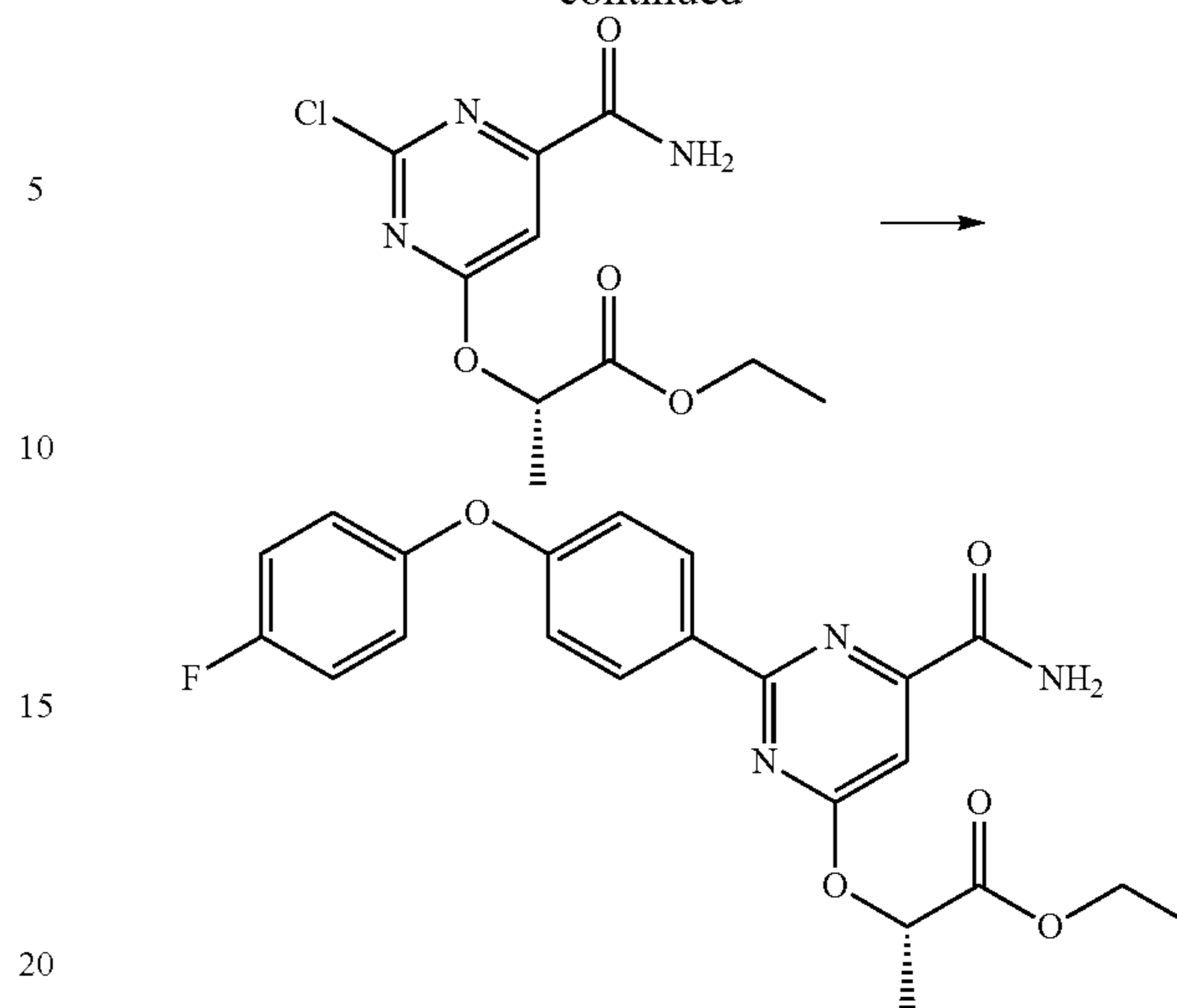
(S)-Ethyl 2-((6-carbamoyl-2-(4-(4-fluorophenoxy)phenyl)pyrimidin-4-yl)oxy)propanoate
