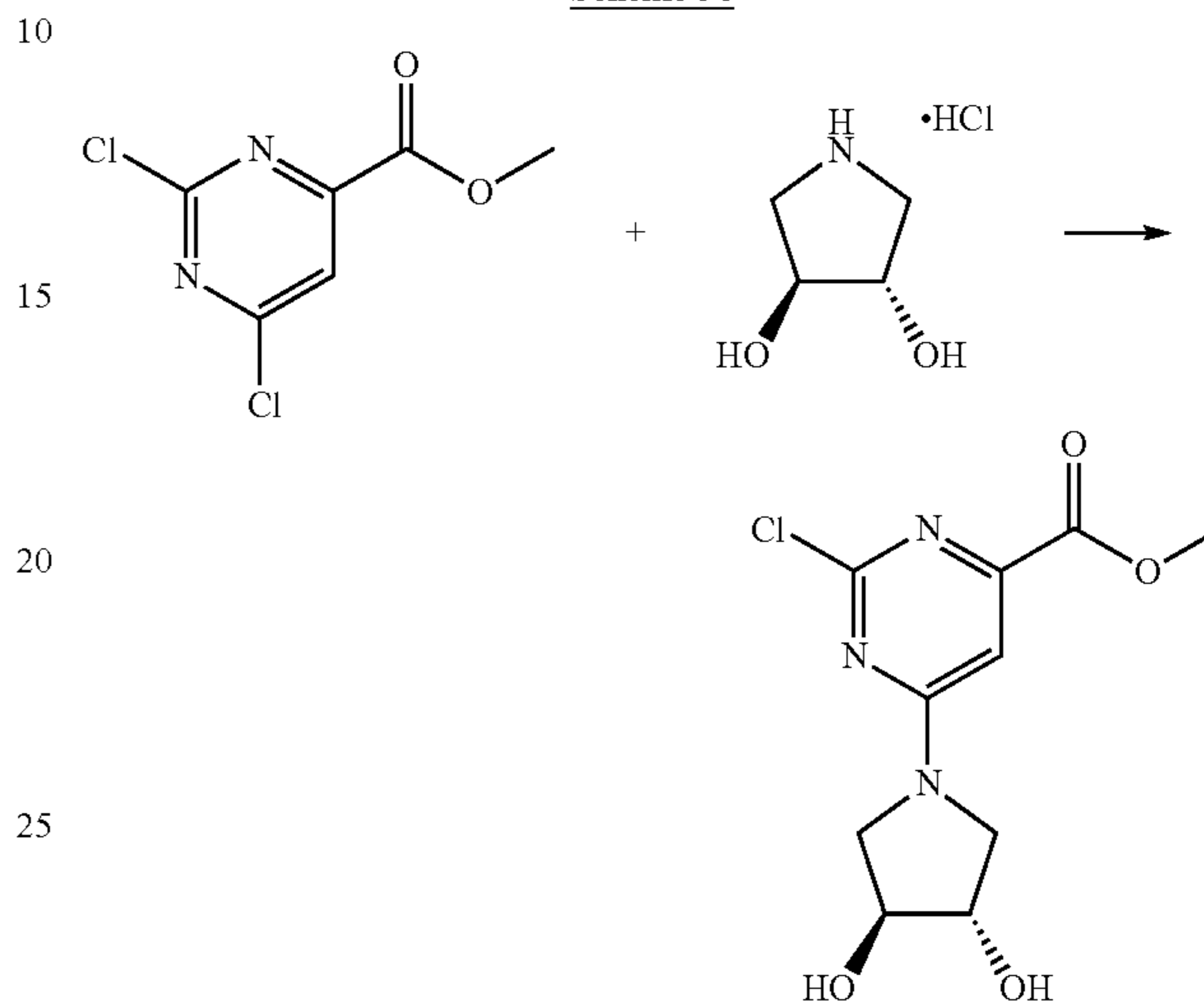
Scheme 58
