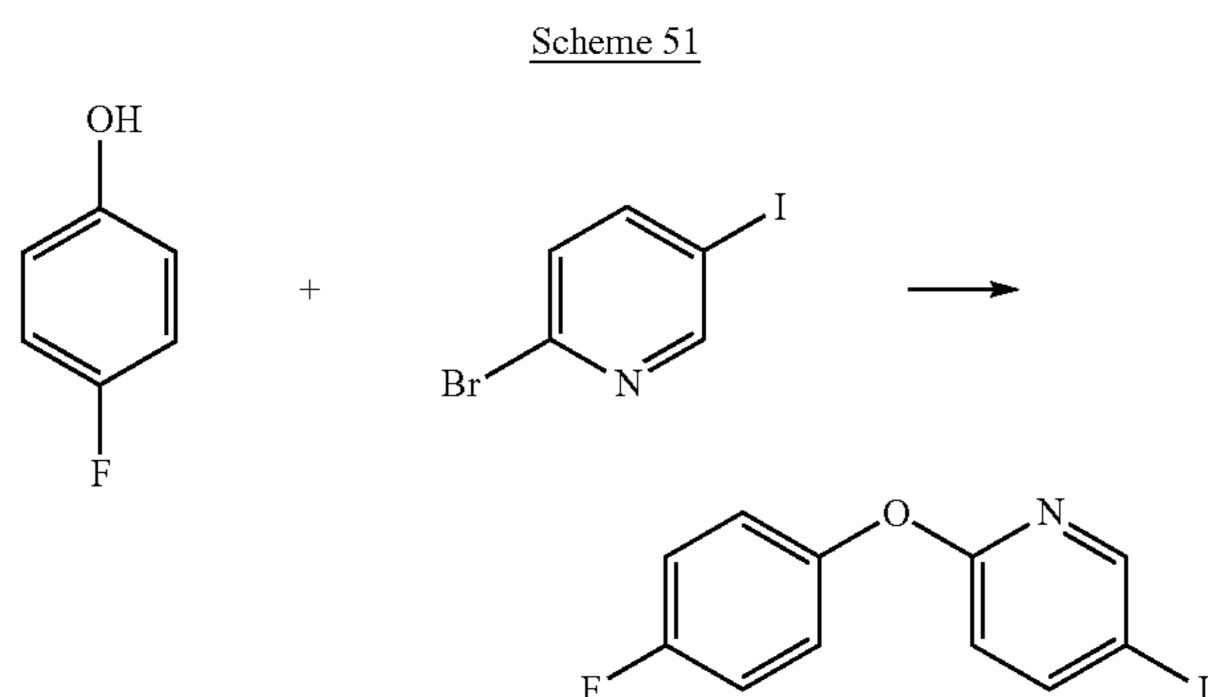
2-(4-fluorophenoxy)-5-iodo-pyridine
