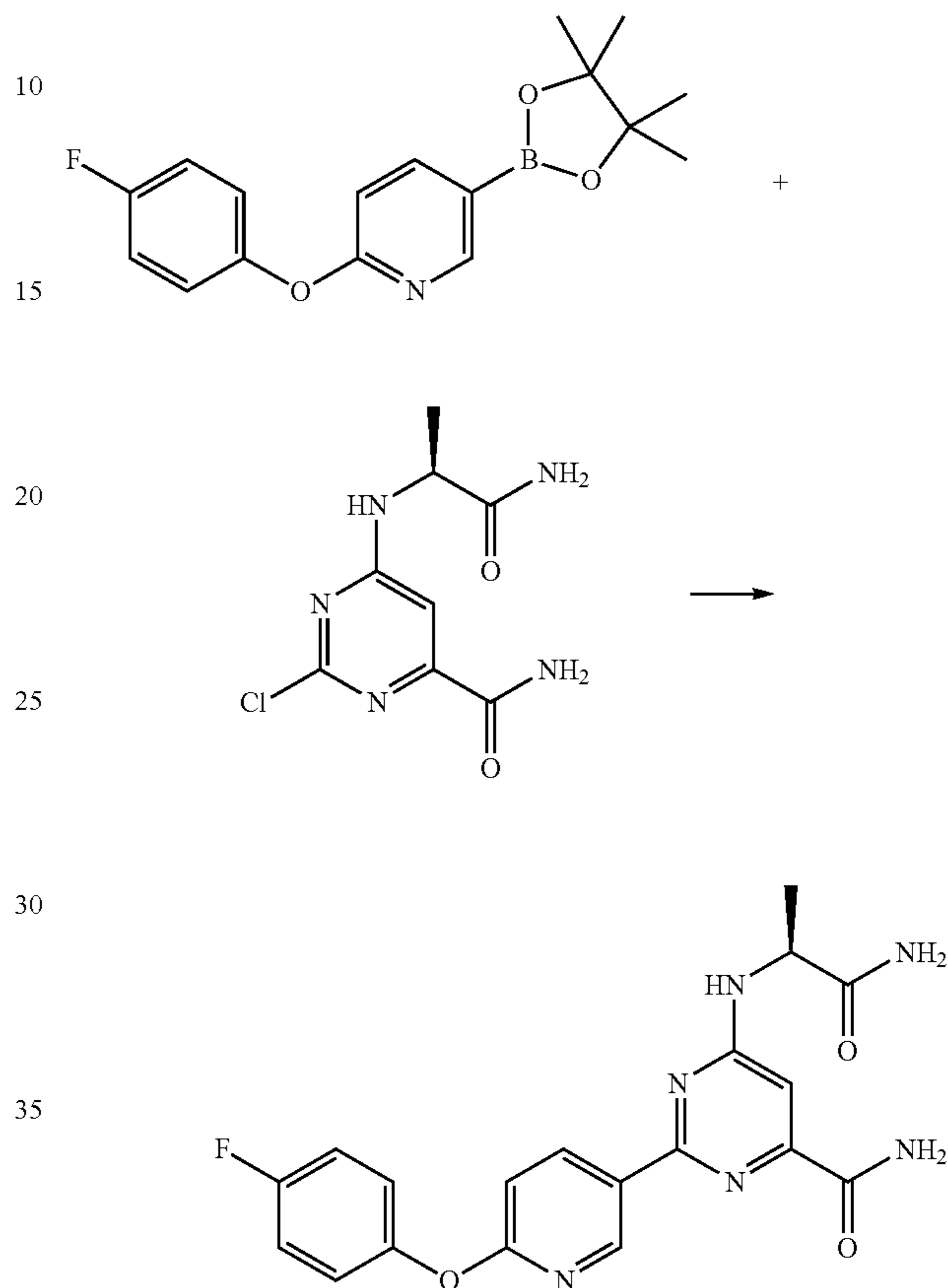
Scheme 53
