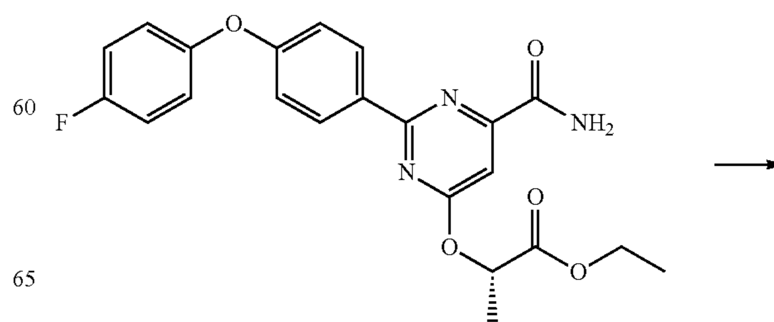
Scheme 43
