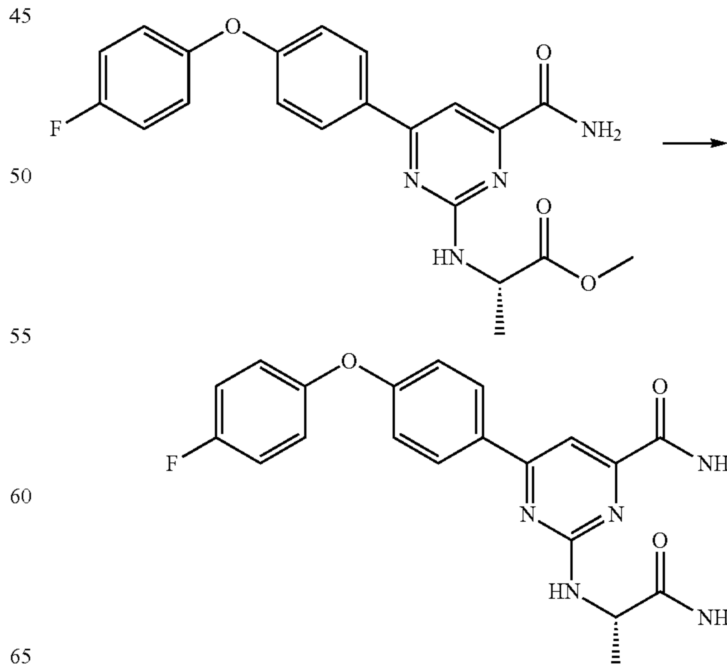
Scheme 38
