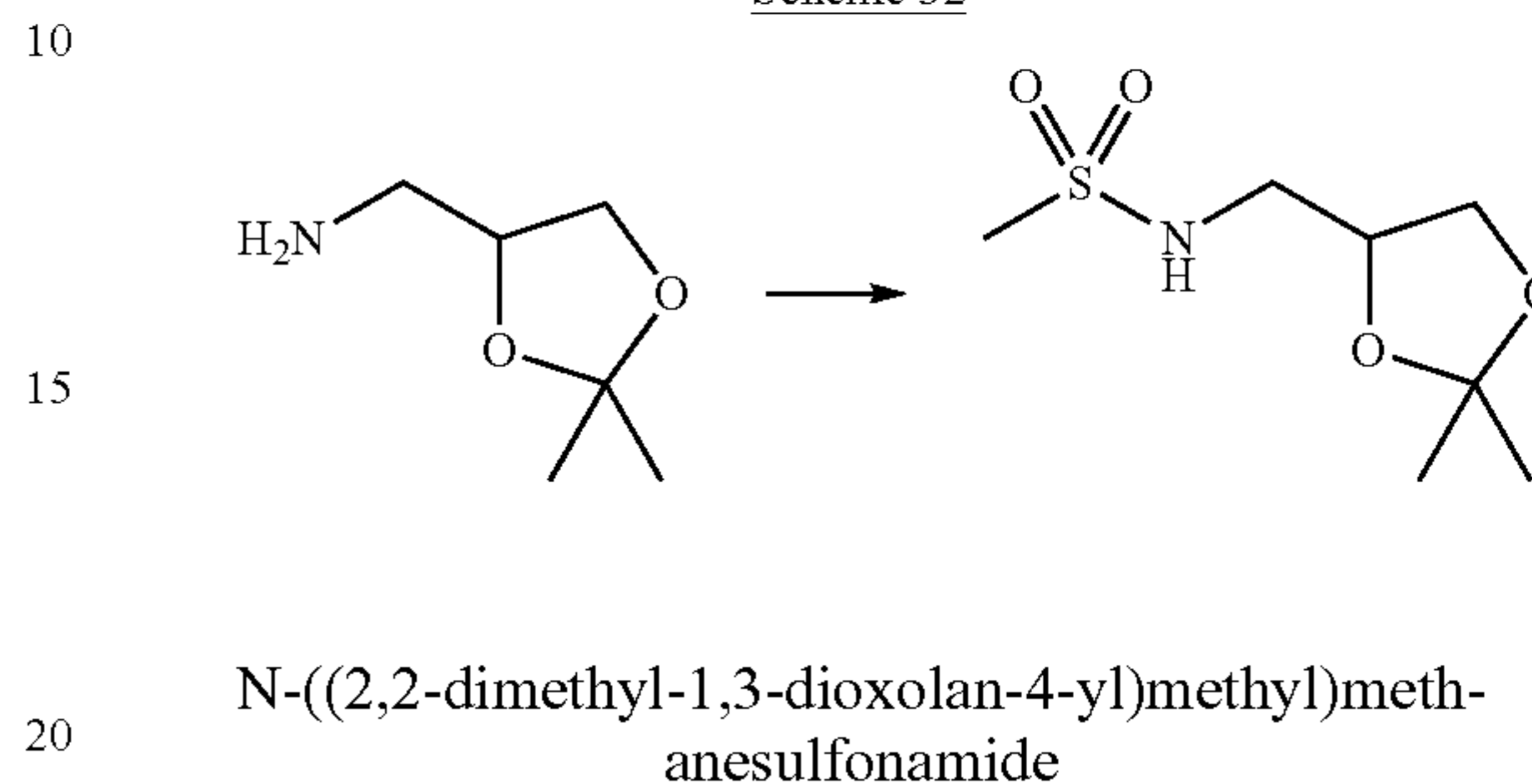
Scheme 32
