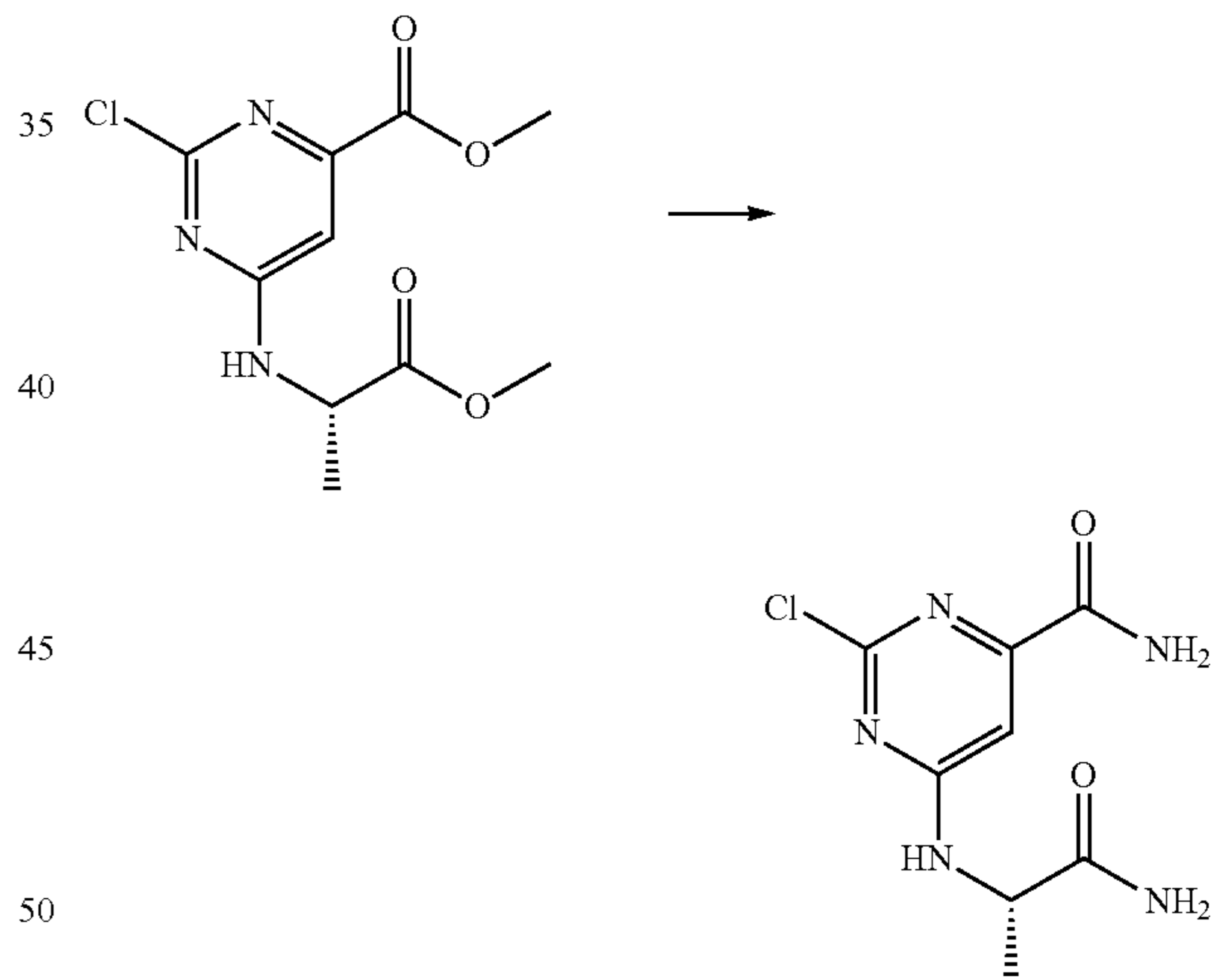
Scheme 18
