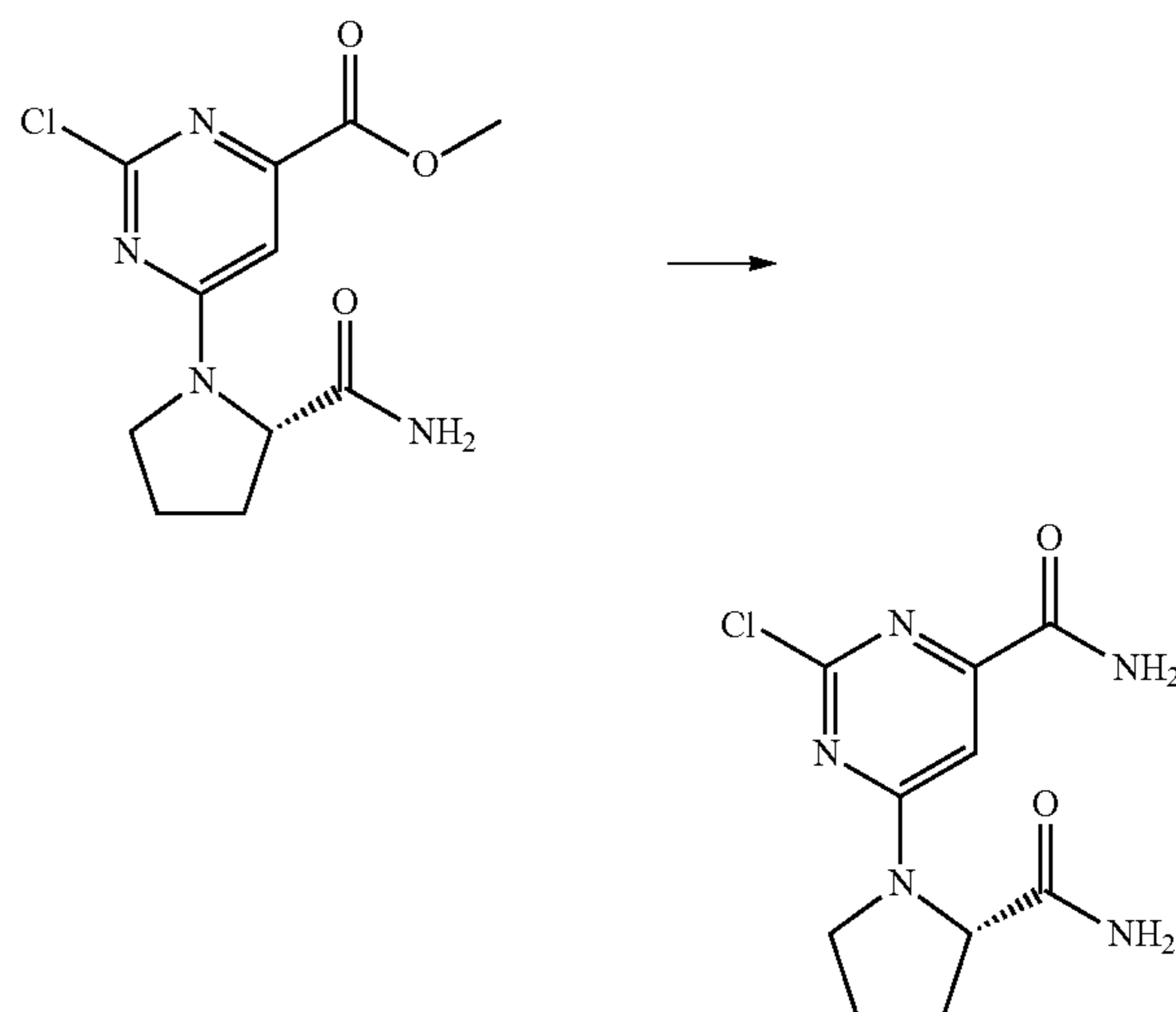
Scheme 56
