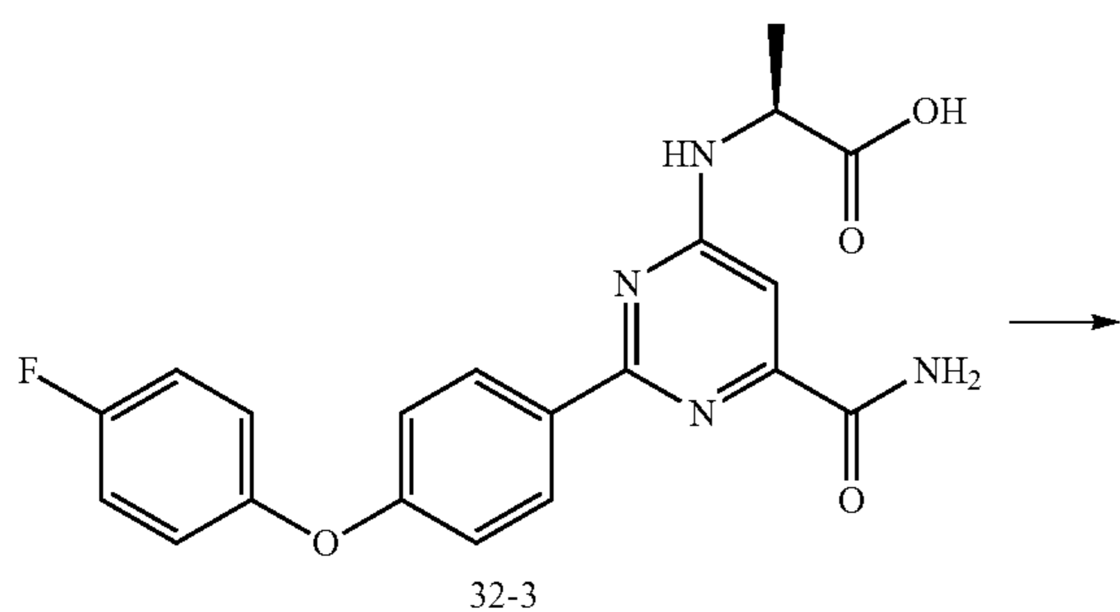
Scheme 75
