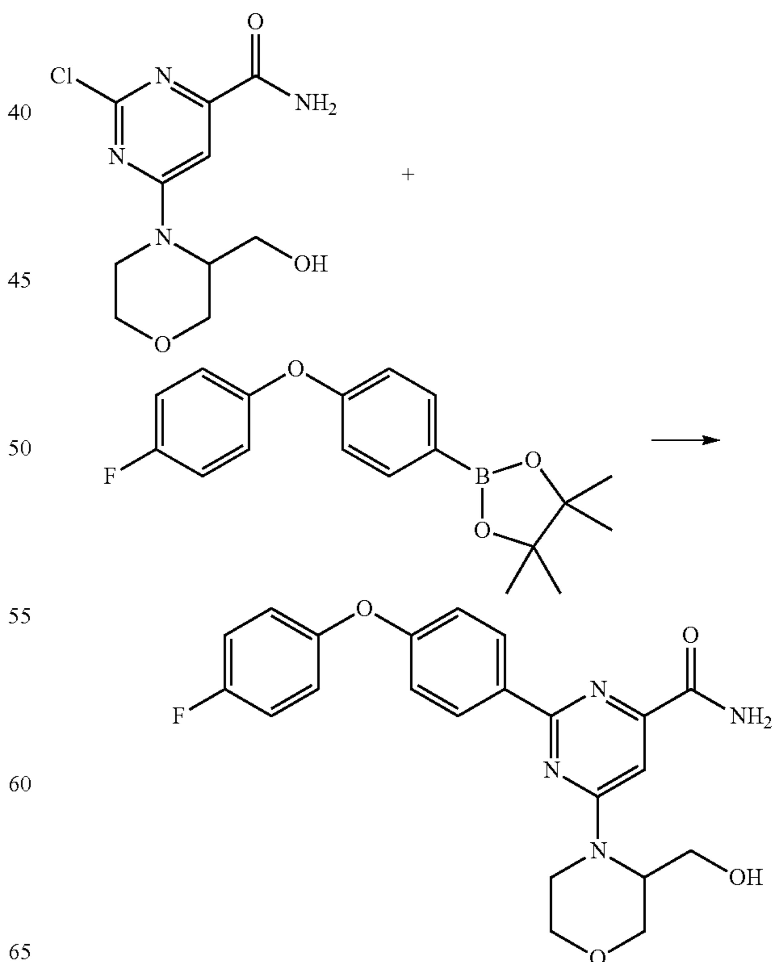
Scheme 23
