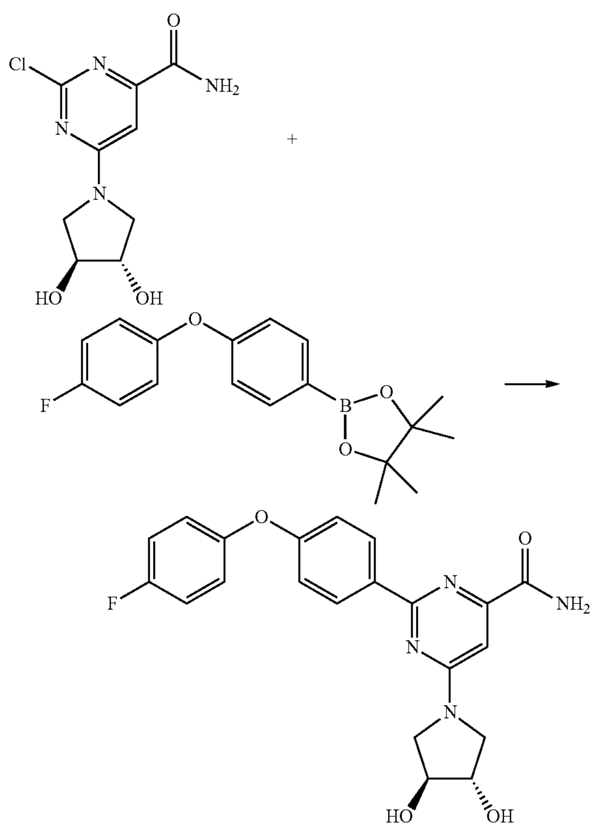
Scheme 60
