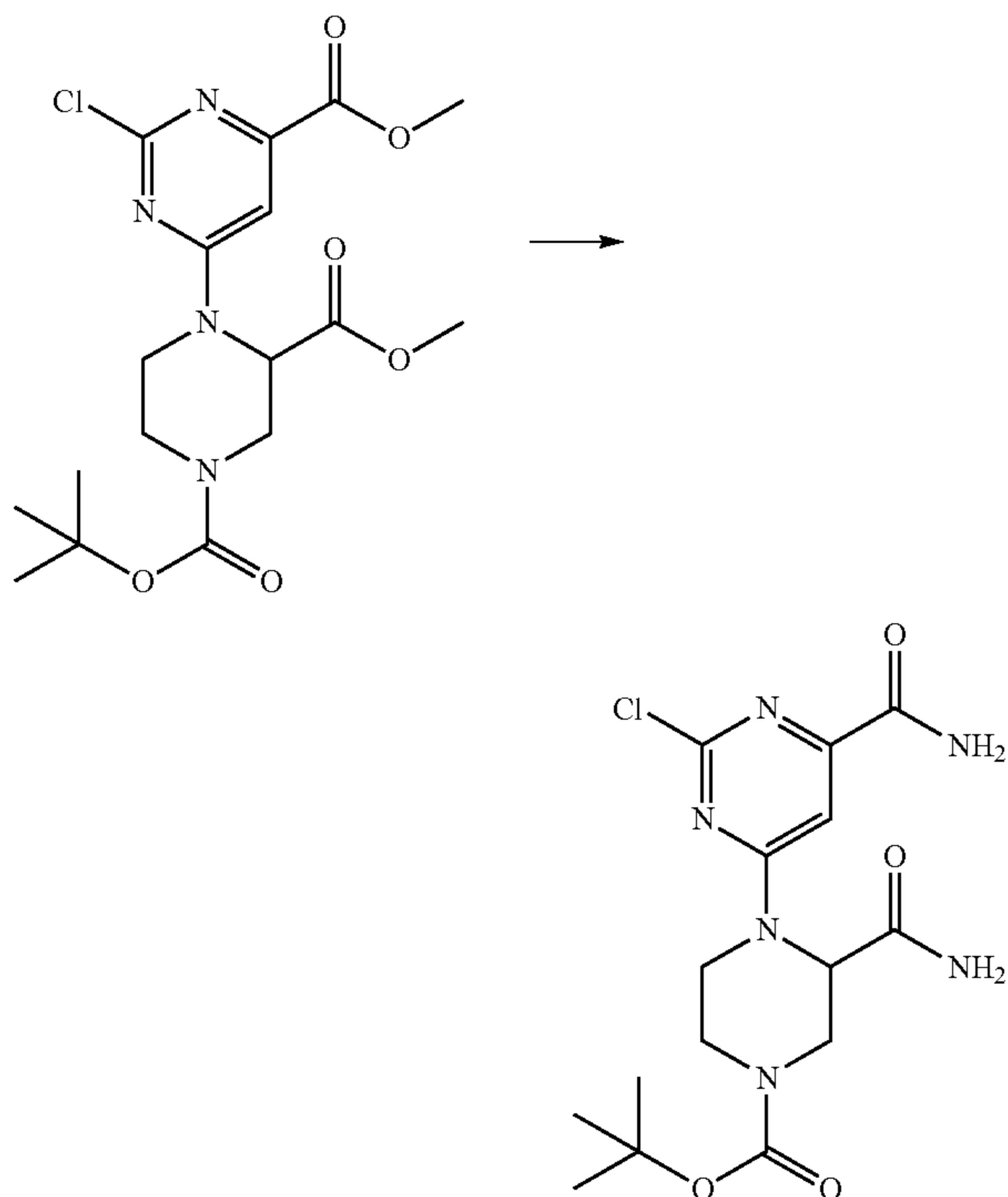
Scheme 62
