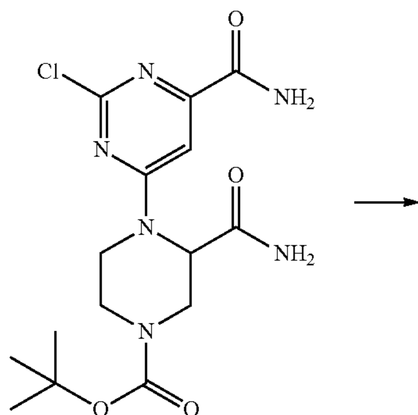
Scheme 63
