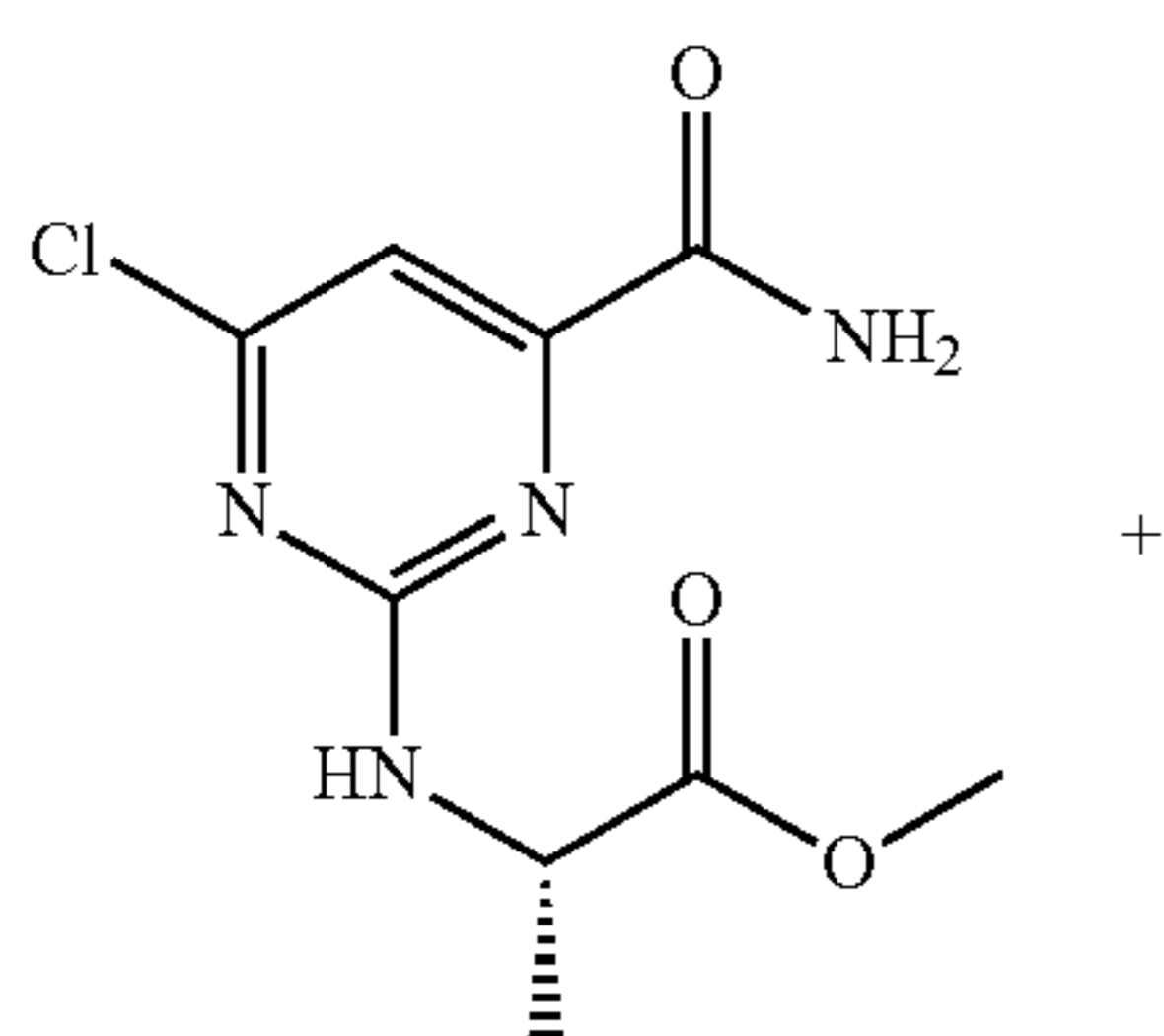
Scheme 37
