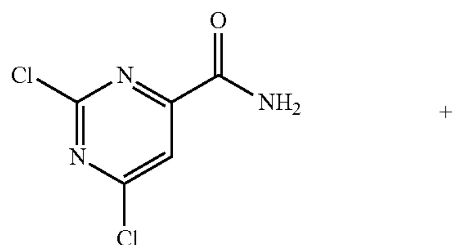
Scheme 22
