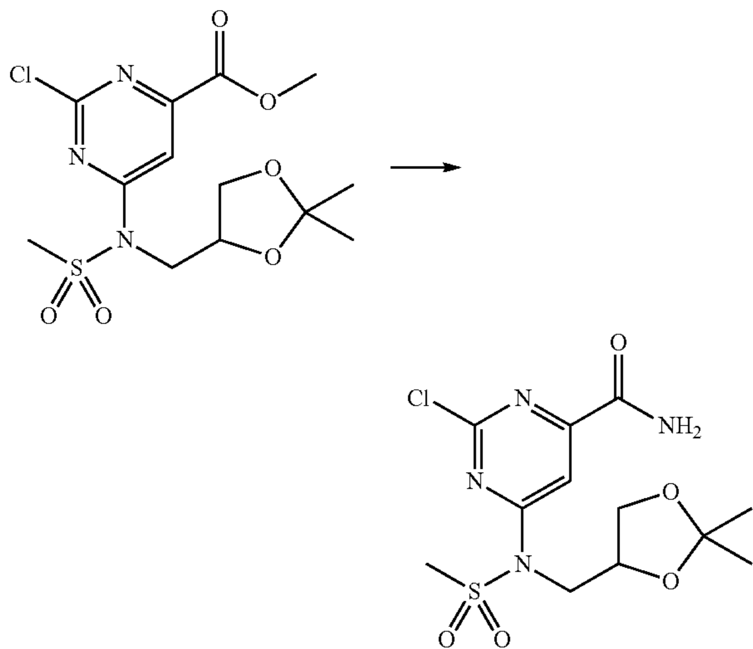
Scheme 34
