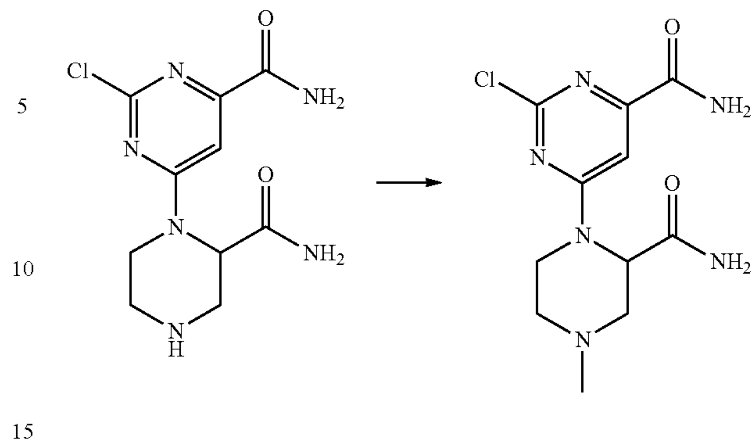
6-(2-Carbamoyl-4-methylpiperazin-1-yl)-2-chloropyrimidine-4-carboxamide
