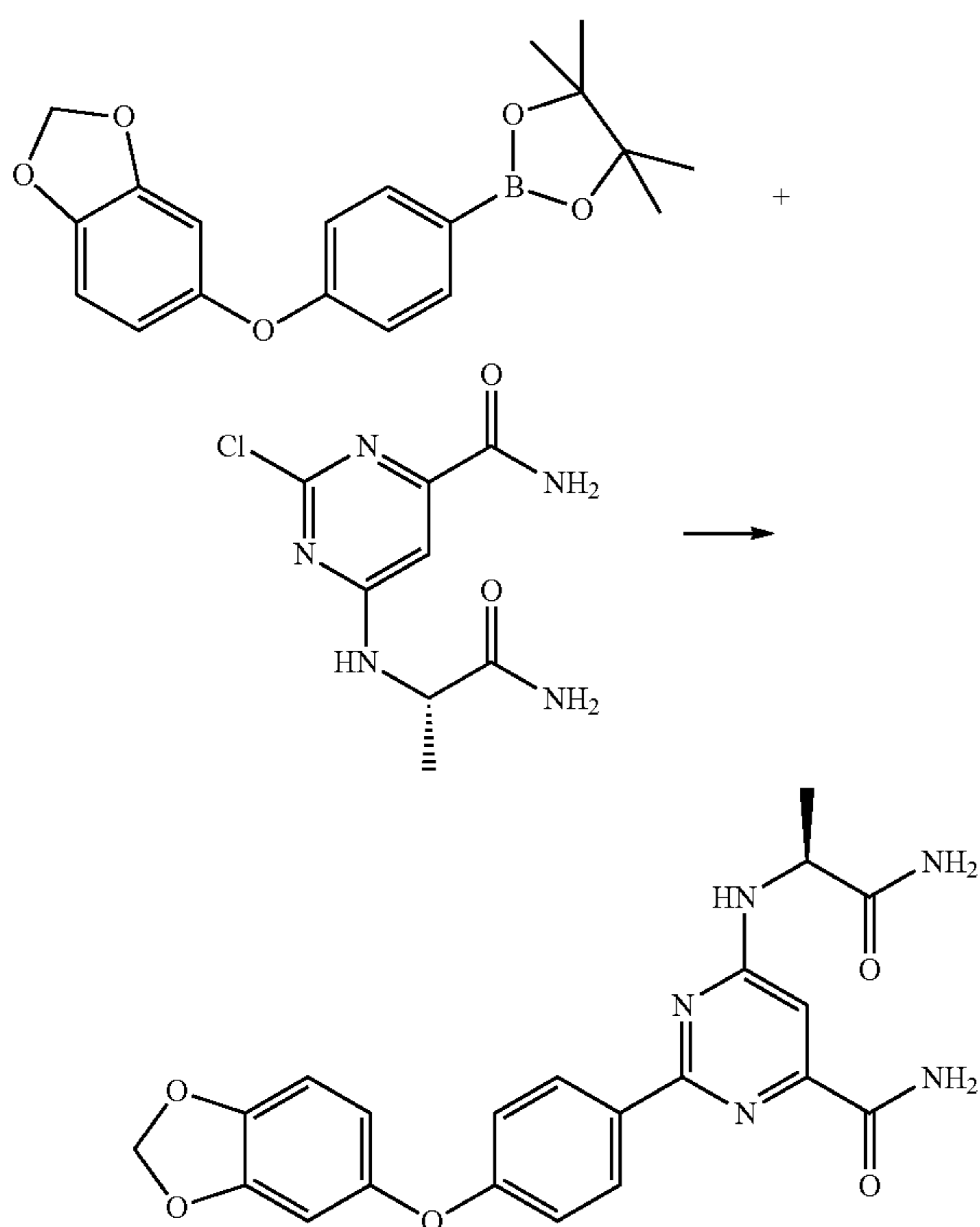
Scheme 72
