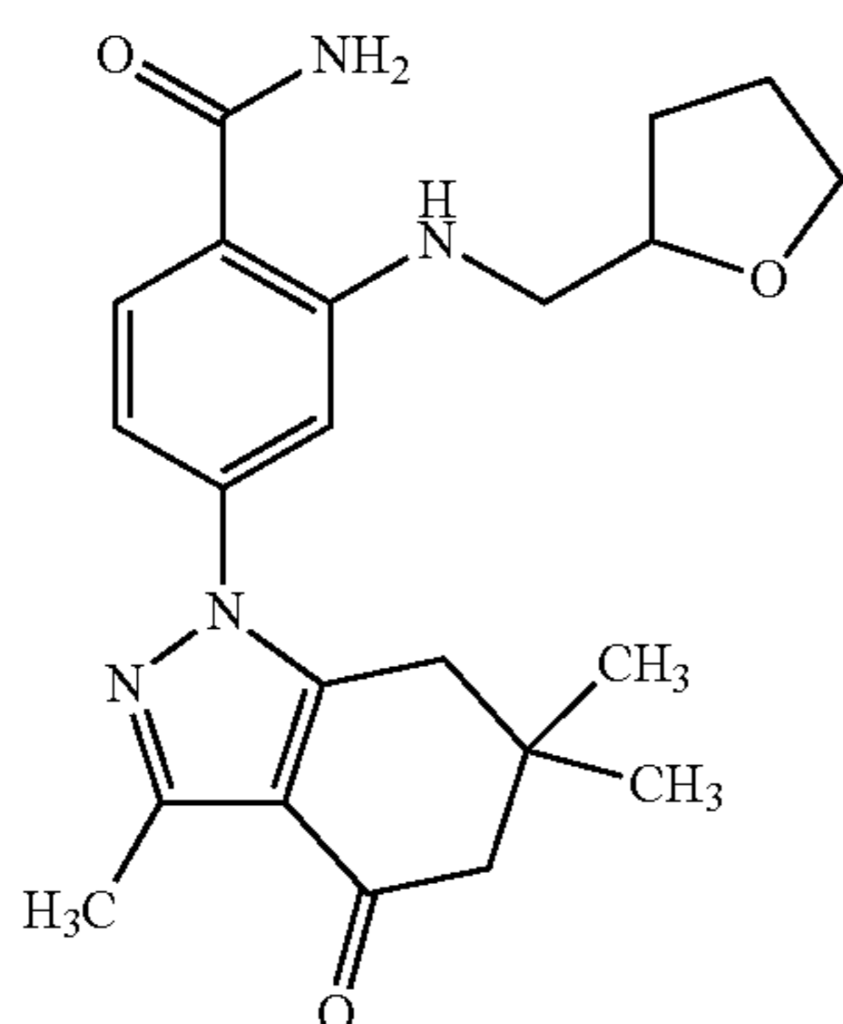
2-[(Tetrahydro-furan-2-ylmethyl)-amino]-4-(3,6,6-trimethyl-4-oxo-4,5,6,7-tetrahydro-indazol-1-yl)-benzamide (Compound 33)
