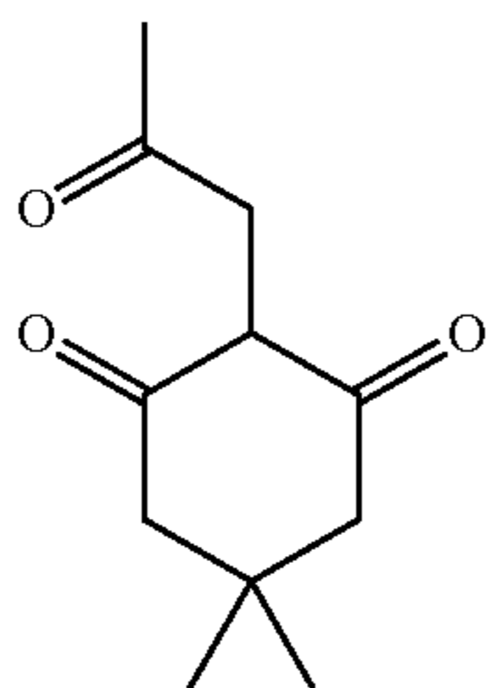
5,5-dimethyl-2-(2-oxopropyl)cyclohexane-1,3-dione (Compound 56)
