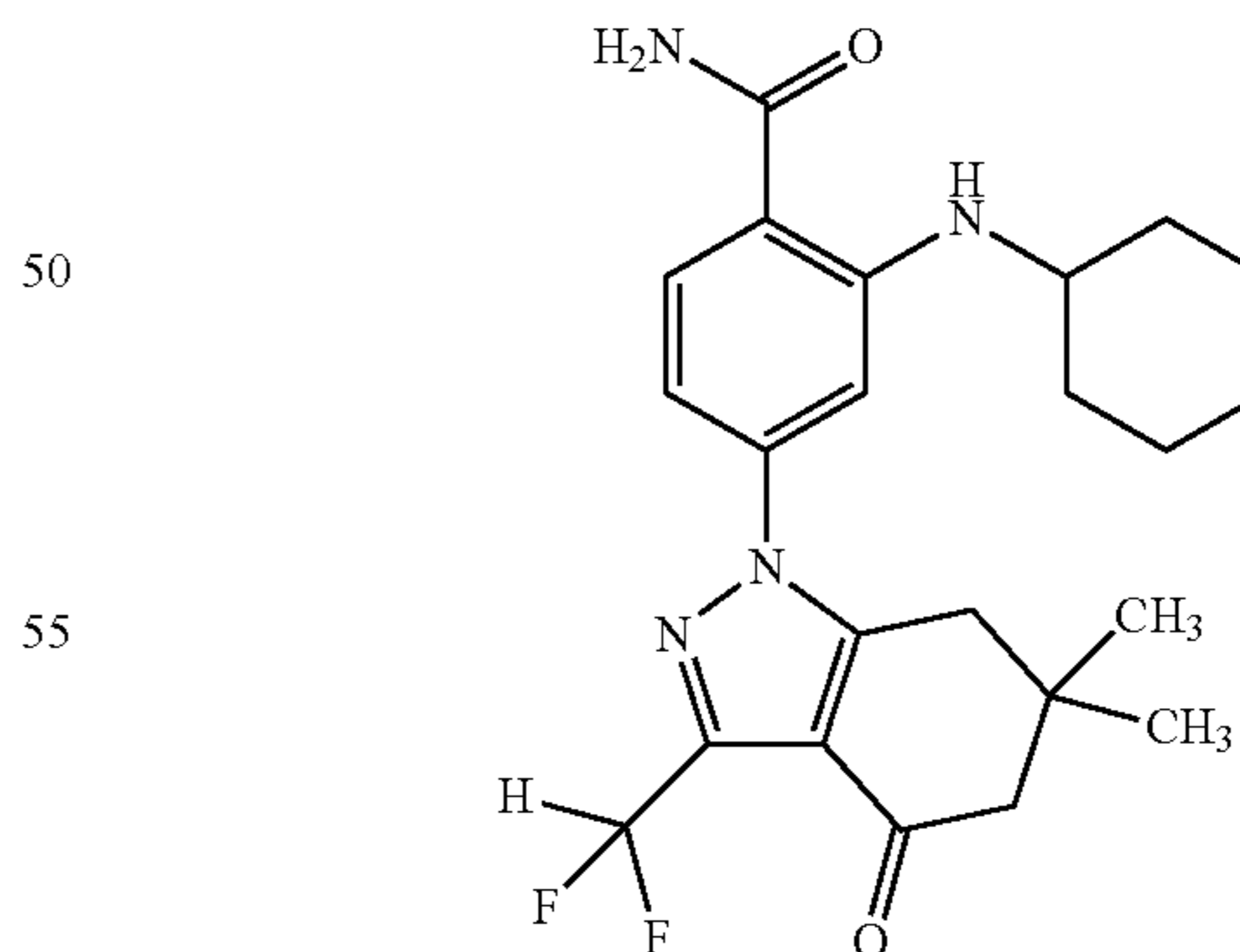
4-(3-Difluoromethyl-6,6-dimethyl-4-oxo-4,5,6,7-tetrahydro-indazol-1-yl)-2-(tetrahydro-thiopyran-4-ylamino)-benzamide (Compound 32)
