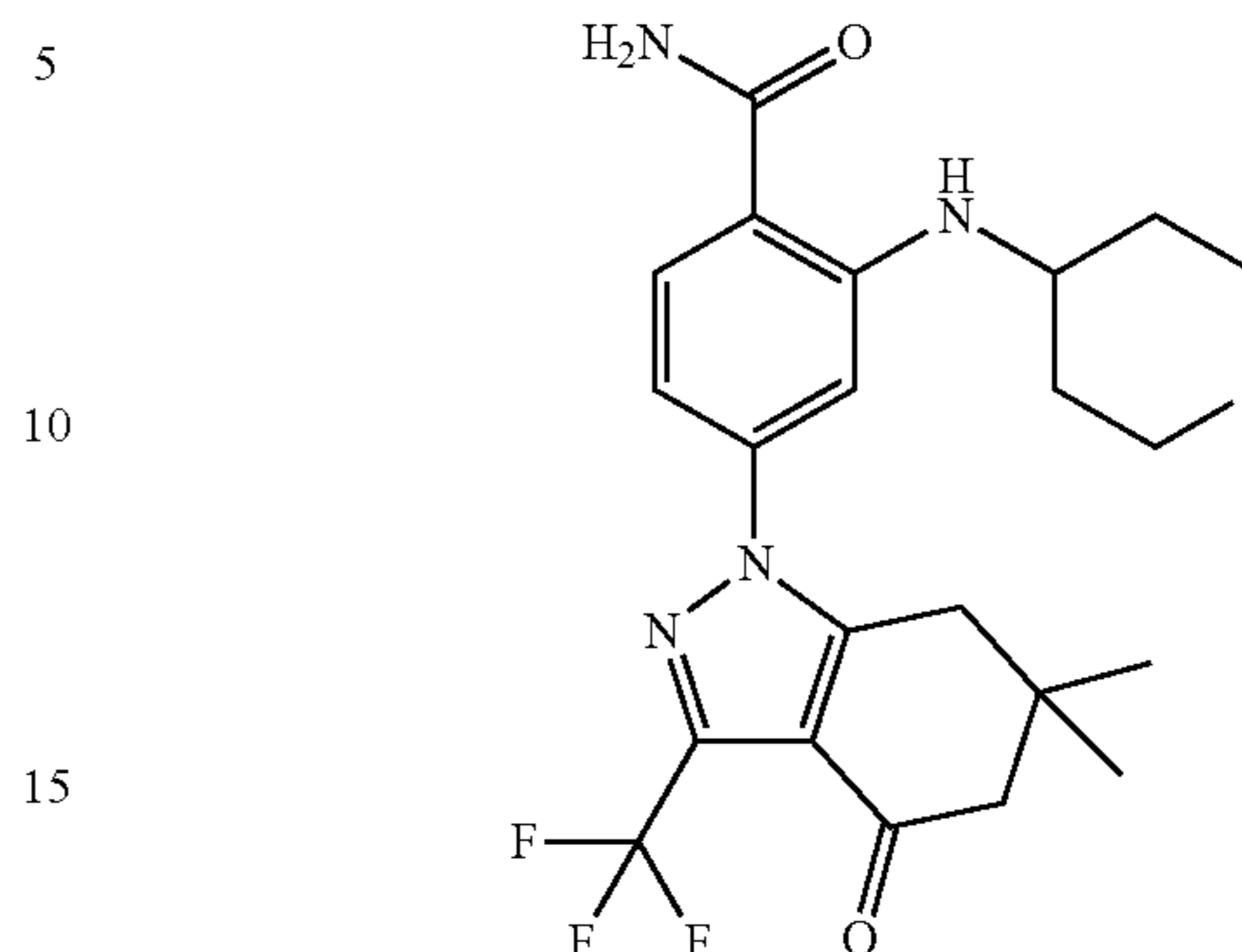
4-(6,6-Dimethyl-4-oxo-3-trifluoromethyl-4,5,6,7-tetrahydro-indazol-1-yl)-2-(tetrahydro-thiopyran-4-ylamino)-benzamide (Compound 31)
