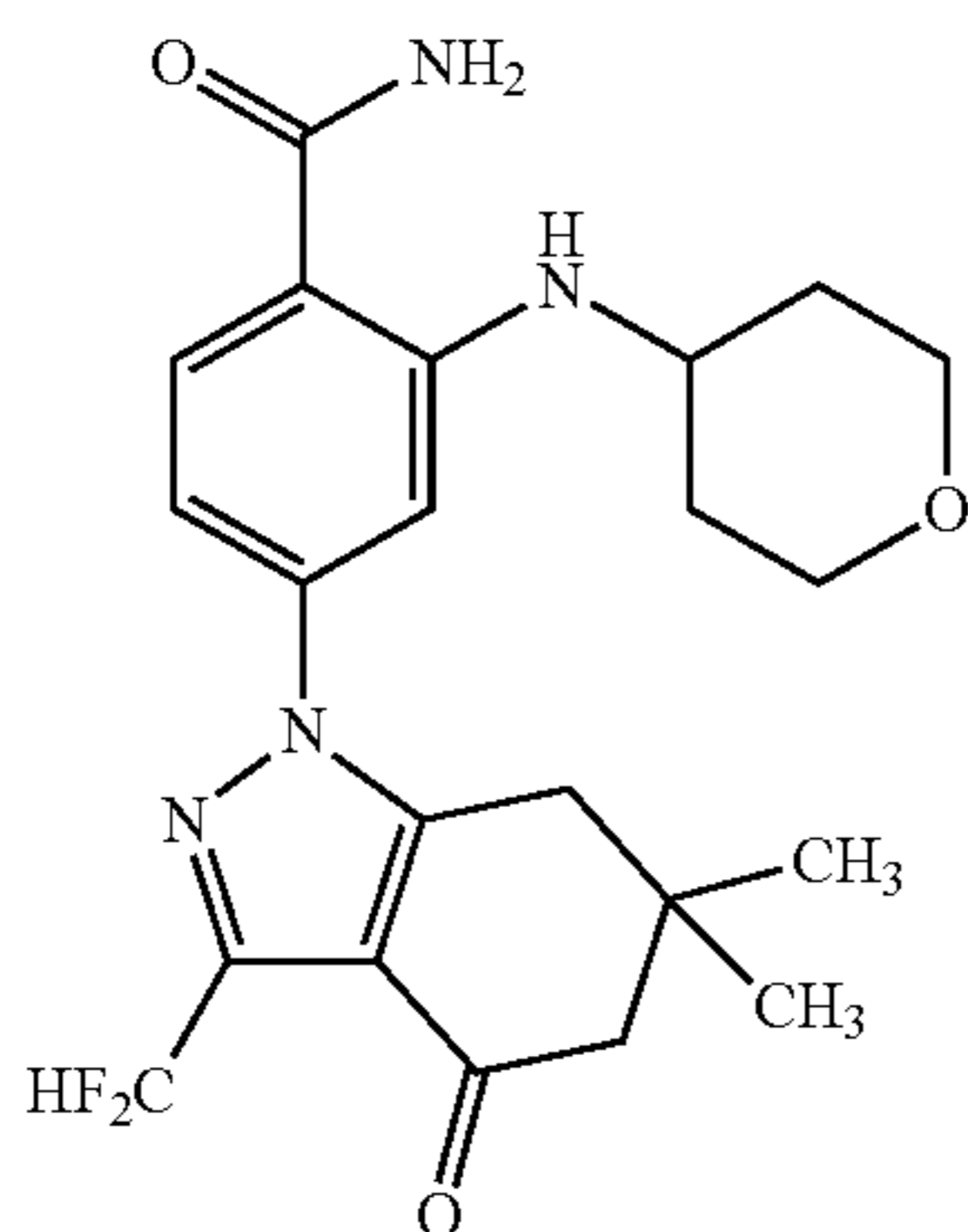
4-(6,6-Dimethyl-4-oxo-3-difluoromethyl-4,5,6,7-tetrahydro-indazol-1-yl)-2-(tetrahydro-pyran-4-ylamino)-benzamide (Compound 26)
