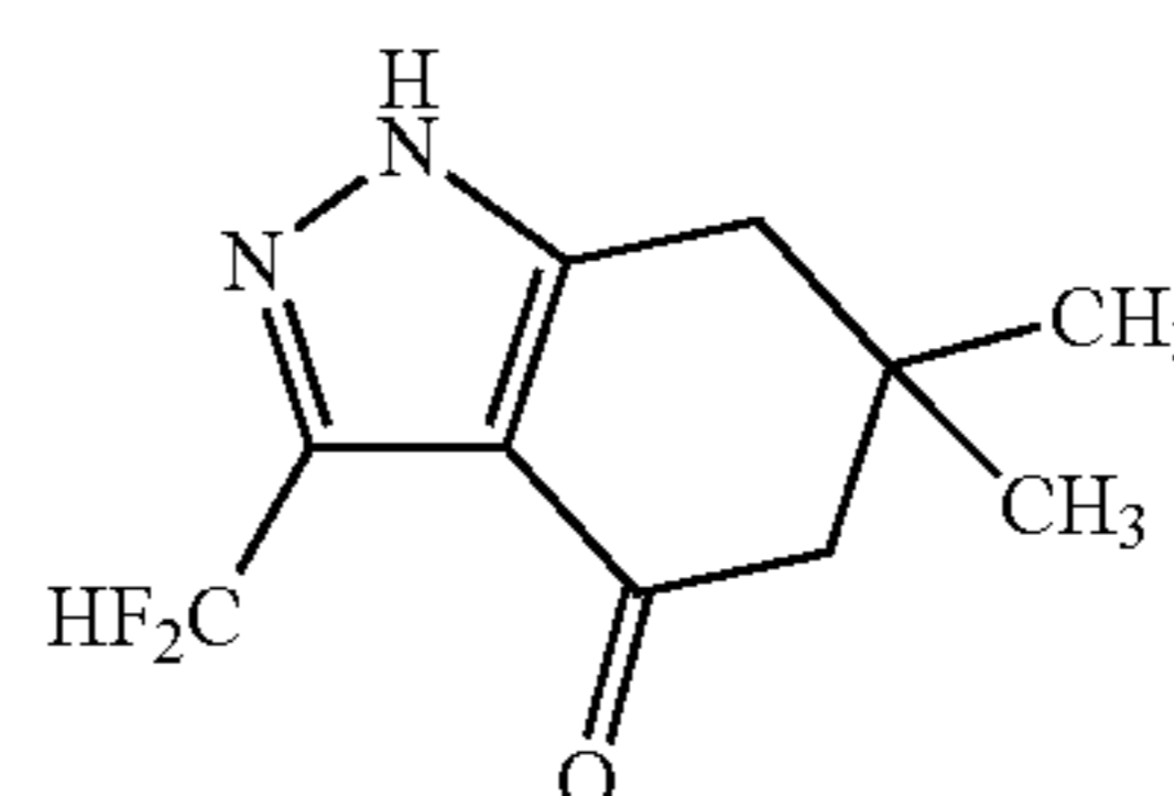
3-Difluoromethyl-6,6-dimethyl-1,5,6,7-tetrahydro-indazol-4-one (Compound 24)
