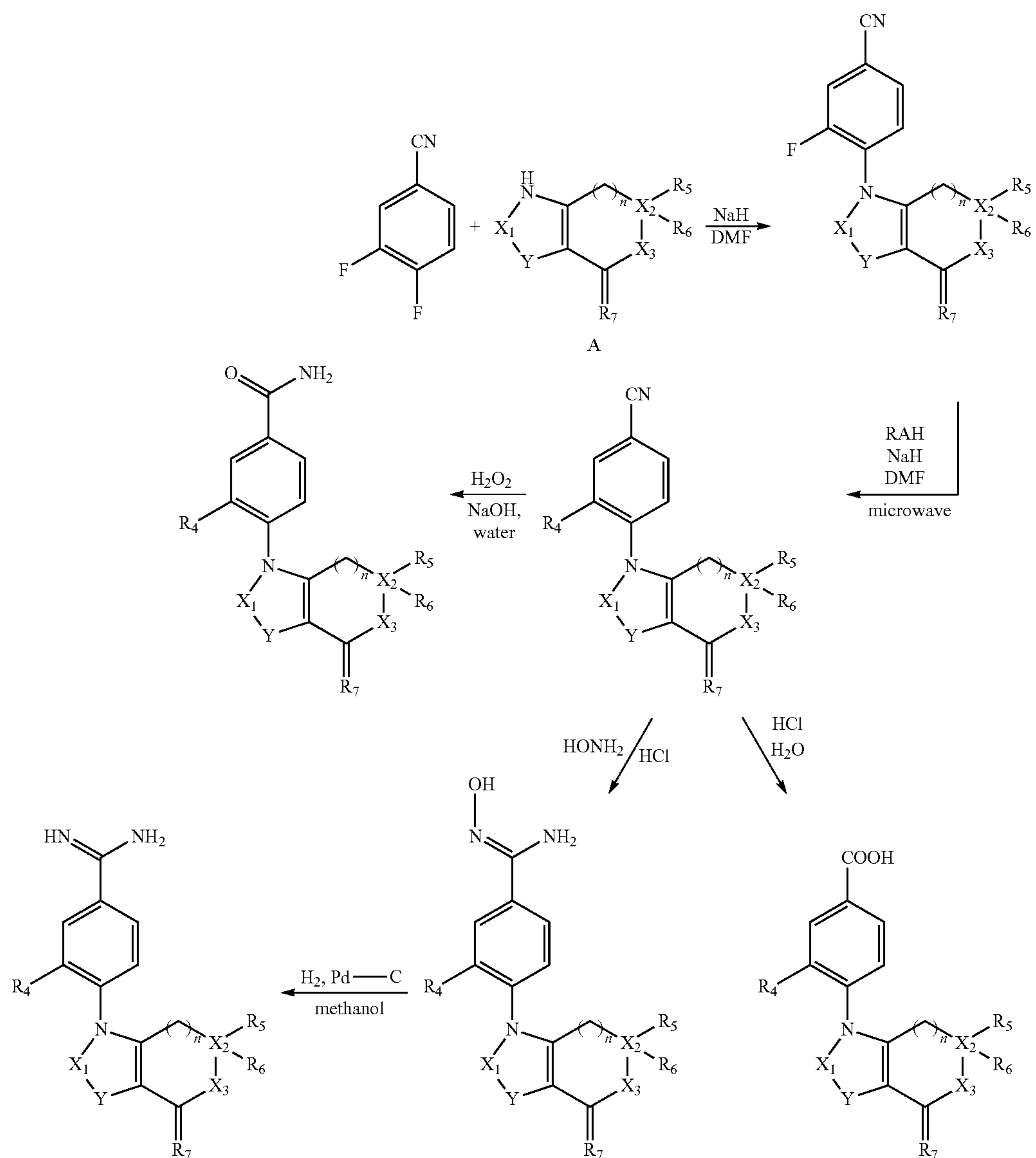
Scheme 8
