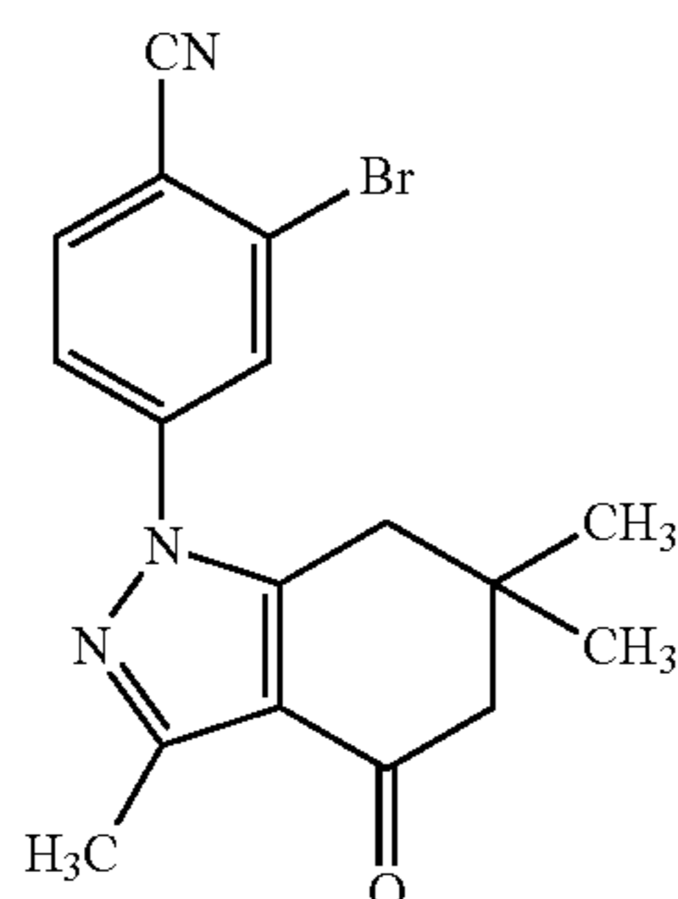
2-Bromo-4-(3,6,6-trimethyl-4-oxo-4,5,6,7-tetrahydro-indazol-1-yl)-benzonitrile (Compound 11)
