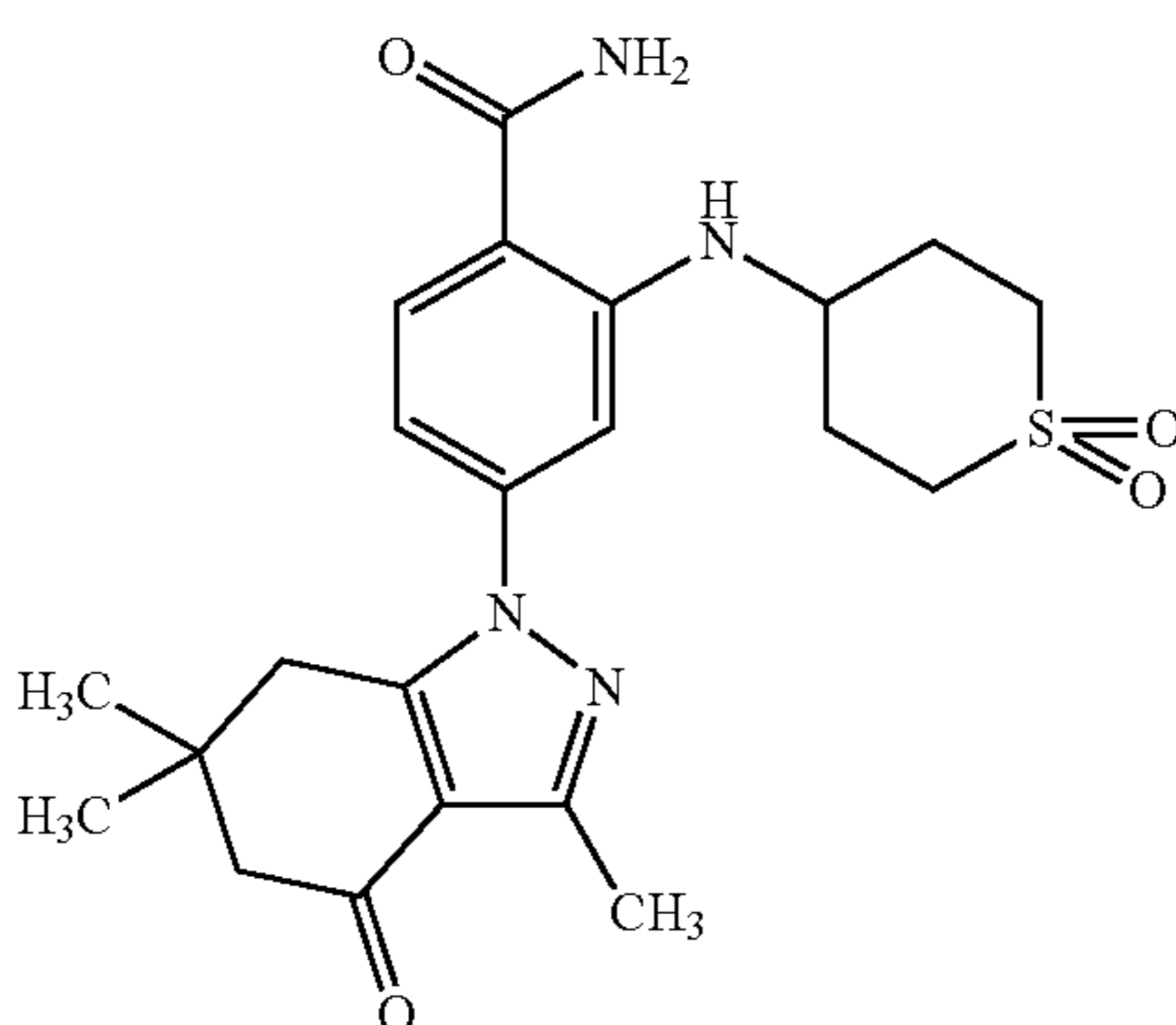
2-(1,1-Dioxo-hexahydro-1-Tetrahydrothiopyran-4-ylamino)-4-(3,6,6-trimethyl-4-oxo-4,5,6,7-tetrahydroindazol-1-yl)benzamide (Compound 15)
