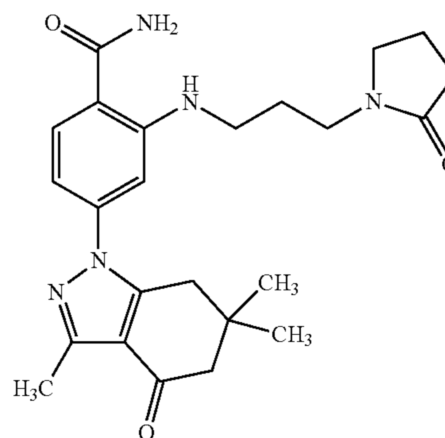
2-[3-(2-Oxo-pyrrolidin-1-yl)-propylamino]-4-(3,6,6-trimethyl-4-oxo-4,5,6,7-tetrahydro-indazol-1-yl)-benzamide (Compound 34)
