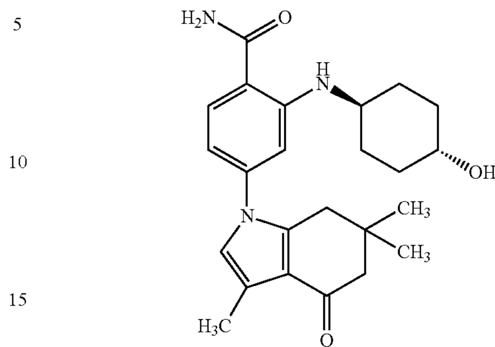
2-(trans-4-Hydroxy-cyclohexylamino)-4-(3,6,6-trimethyl-4-oxo-4,5,6,7-tetrahydro-indol-1-yl)-benzamide (Compound 3)
