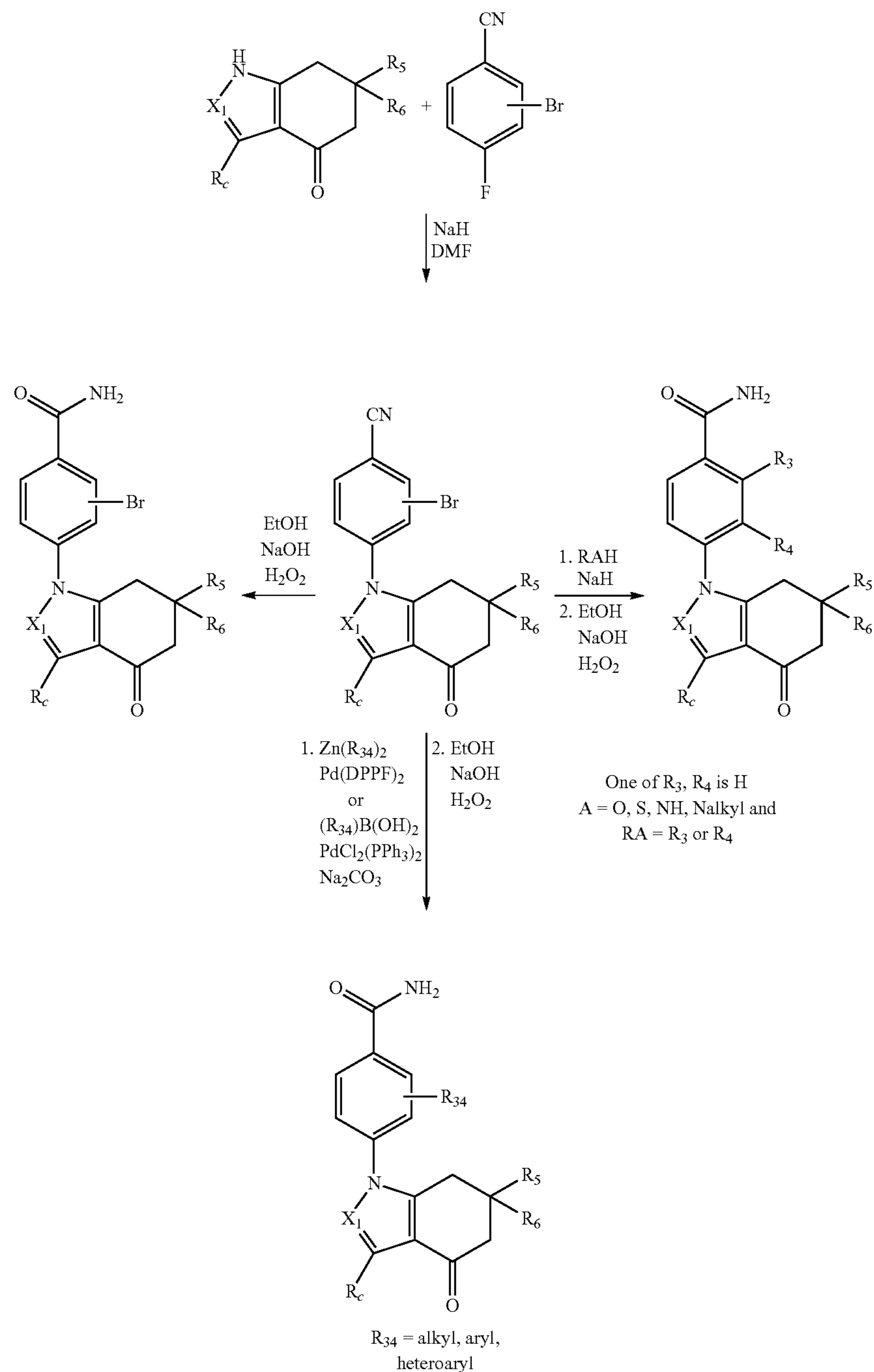
Scheme 9
