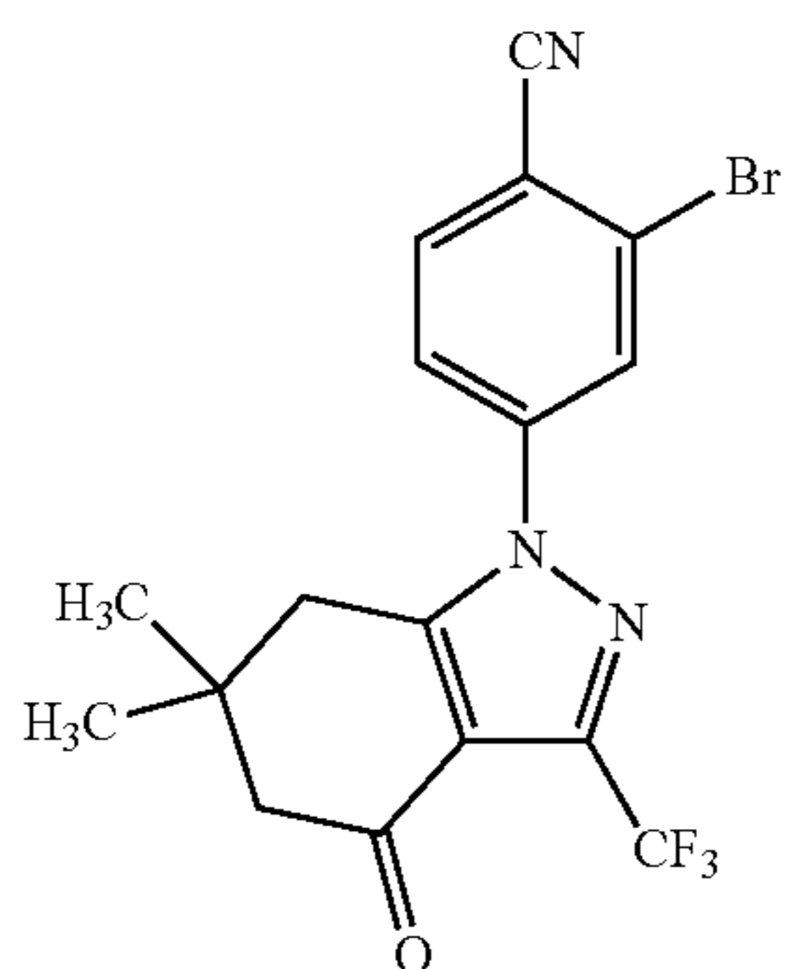
2-bromo-4-(6,6-dimethyl-4-oxo-3-trifluoromethyl-4,5,6,7-tetrahydro-indazol-1-yl)-benzotrile (Compound 17)
