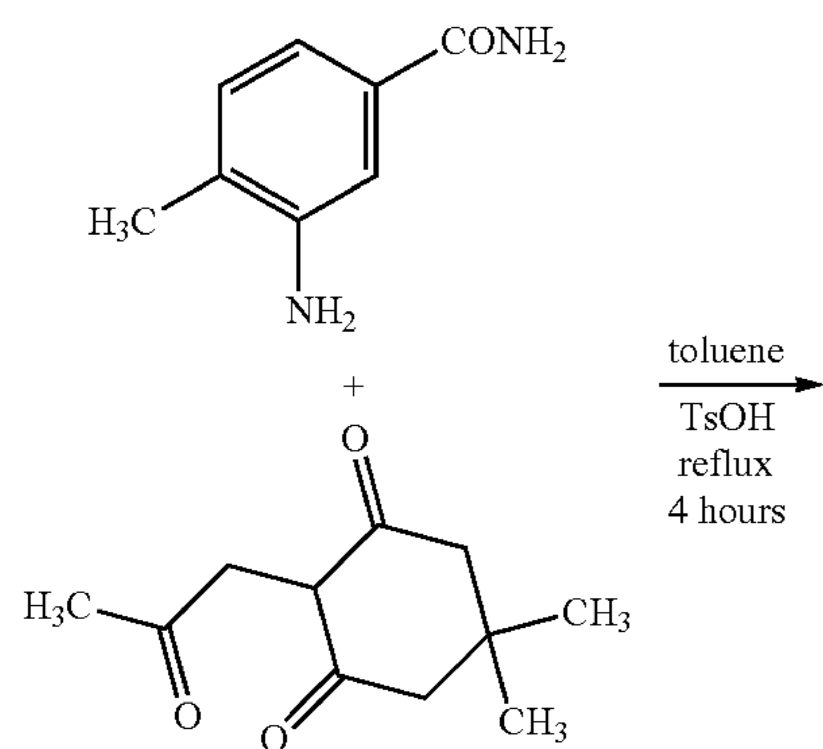
Scheme 7
