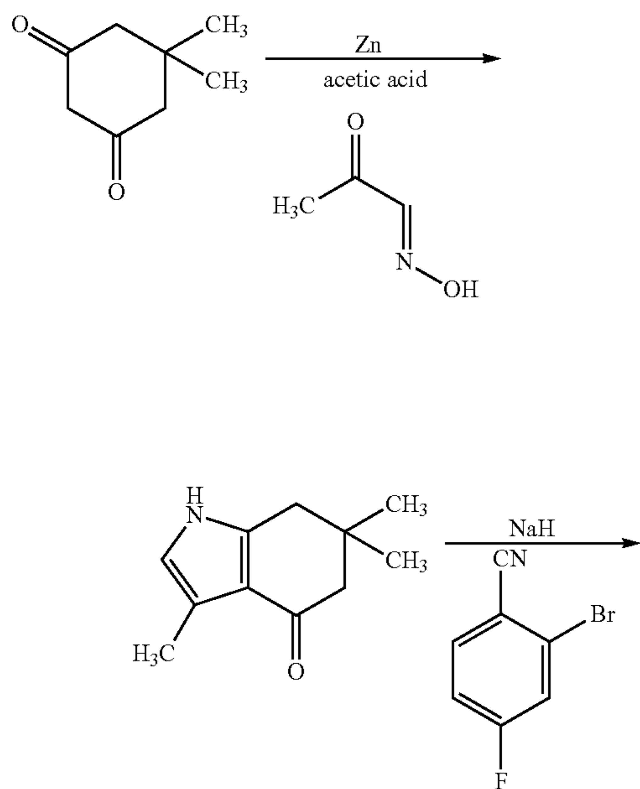
Scheme 3
