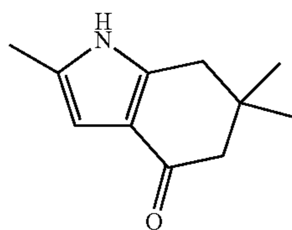
2,6,6-trimethyl-6,7-dihydro-1H-indol-4(5H)-one (Compound 57)
