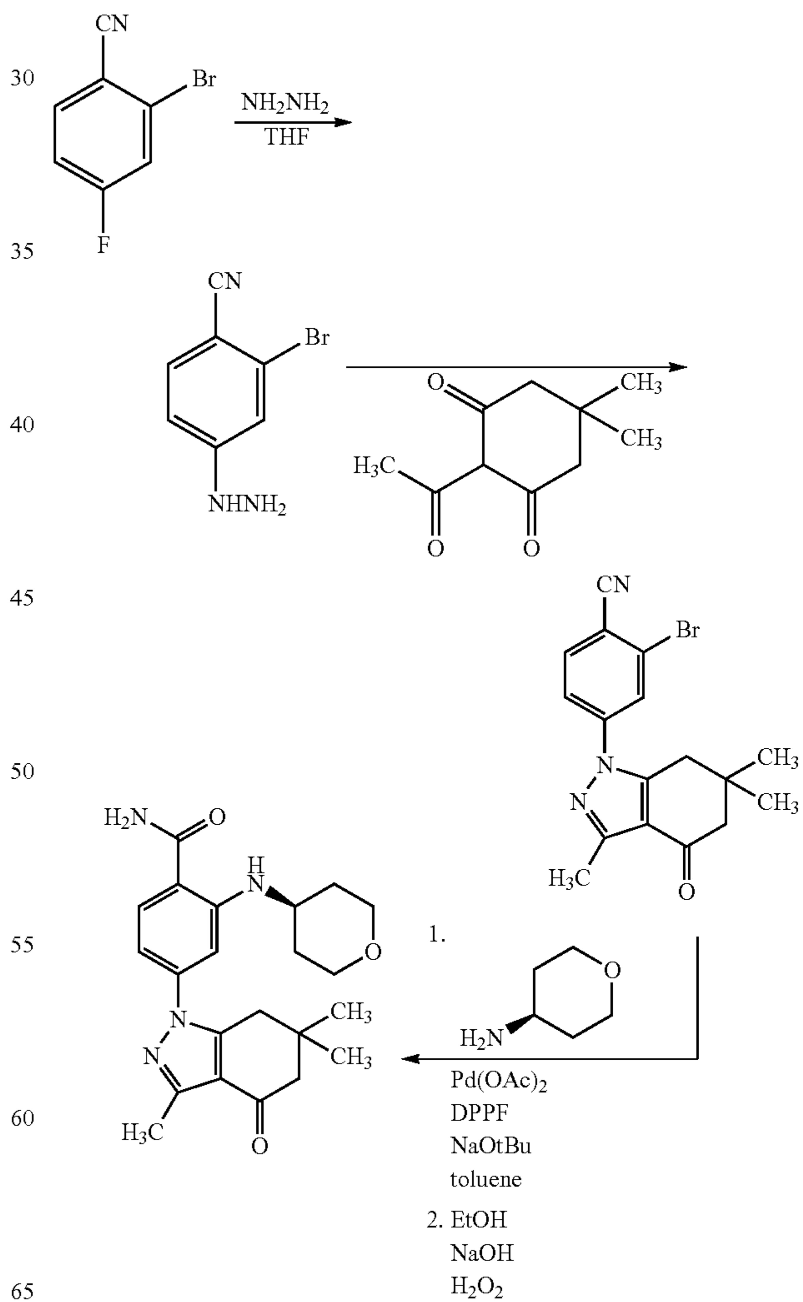
Scheme 4
