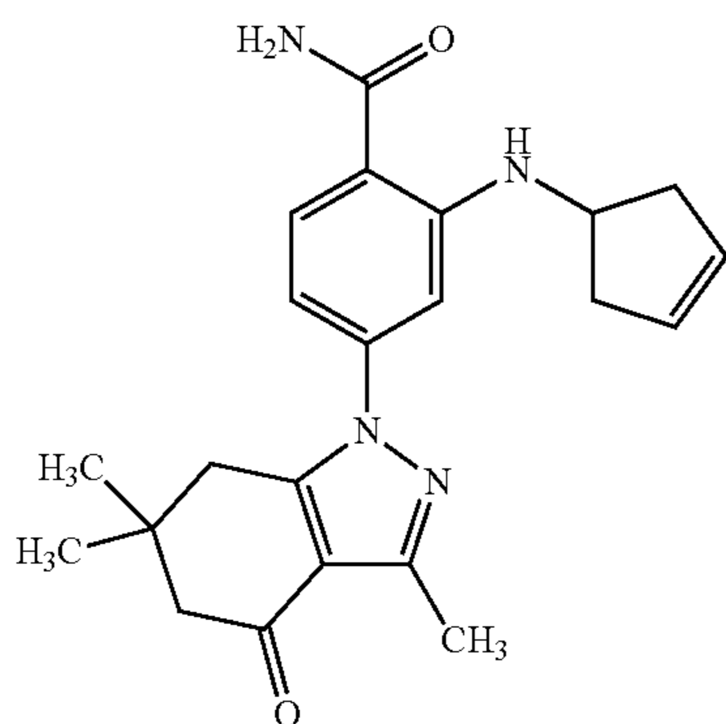
2-(Cyclopent-3-enylamino)-4-(3,6,6-trimethyl-4-oxo-4,5,6,7-tetrahydro-indazol-1-yl)benzamide (Compound 18)
