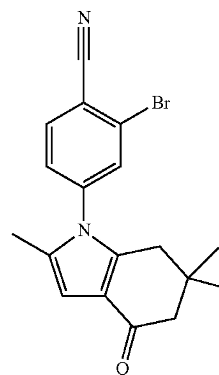
2-bromo-4-(2,6,6-trimethyl-4-oxo-4,5,6,7-tetrahydro-1H-indol-1-yl)benzotrile (Compound 58)
