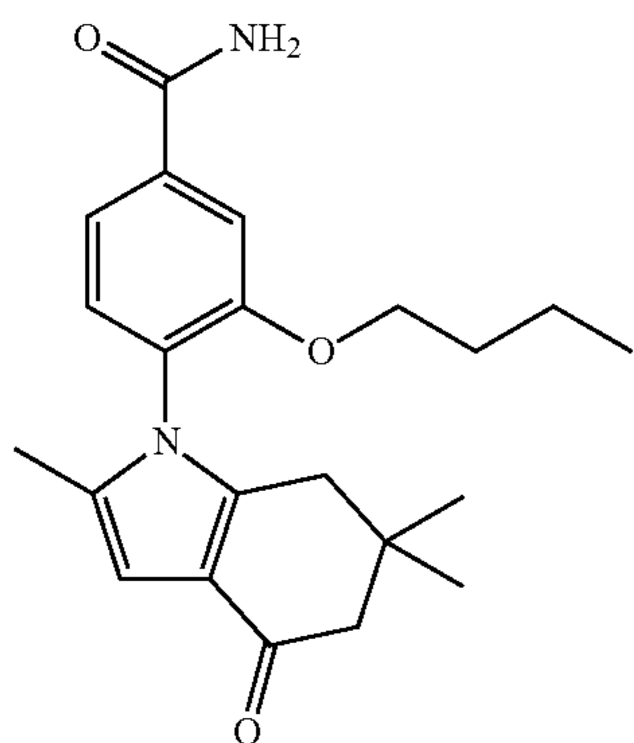
3-butoxy-4-(2,6,6-trimethyl-4-oxo-4,5,6,7-tetrahydro-1H-indol-1-yl)benzamide (Compound 60)
