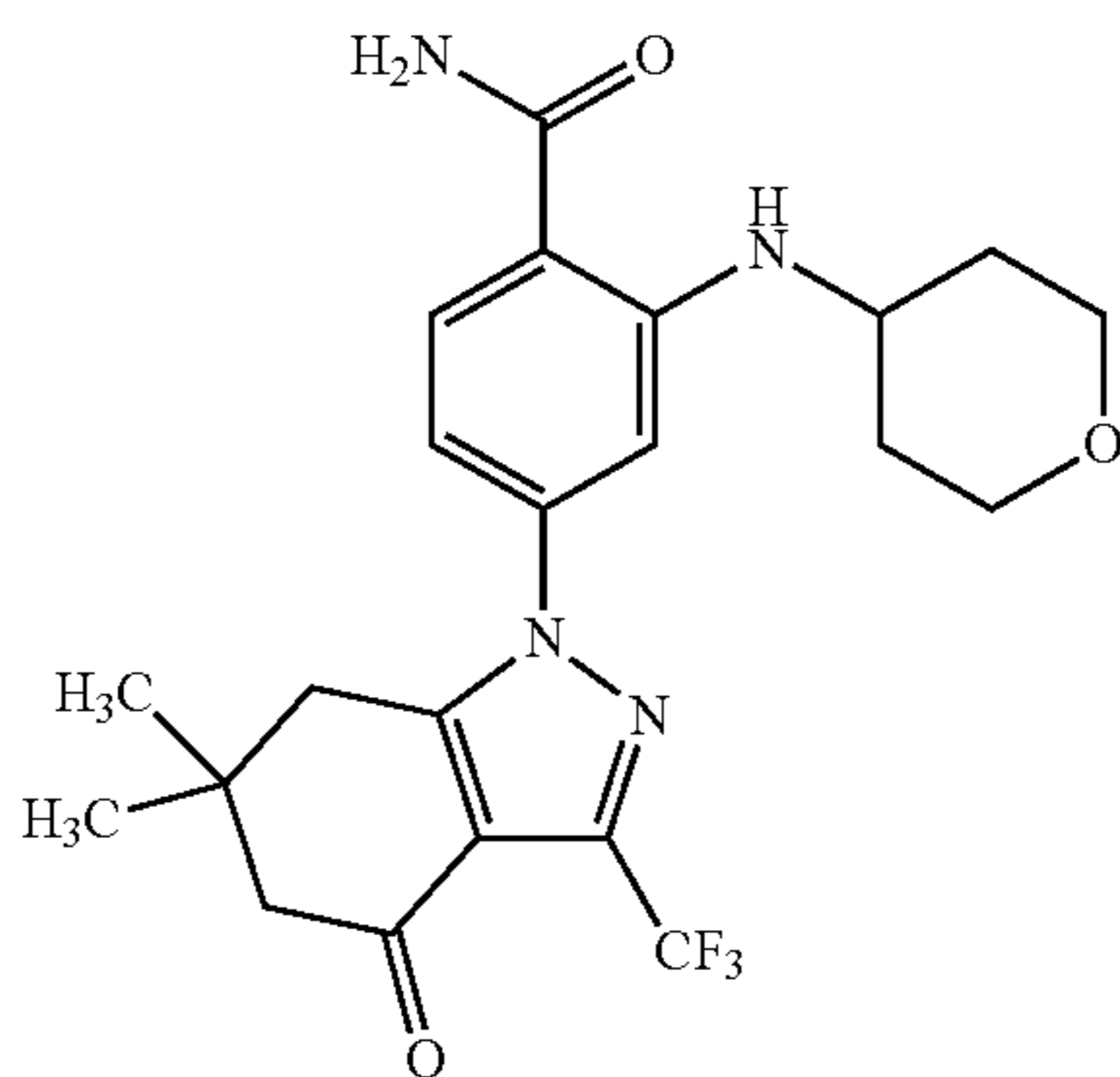
4-(6,6-Dimethyl-4-oxo-3-trifluoromethyl-4,5,6,7-tetrahydro-indazol-1-yl)-2-(tetrahydro-pyran-4-ylamino)-benzamide (Compound 23)
