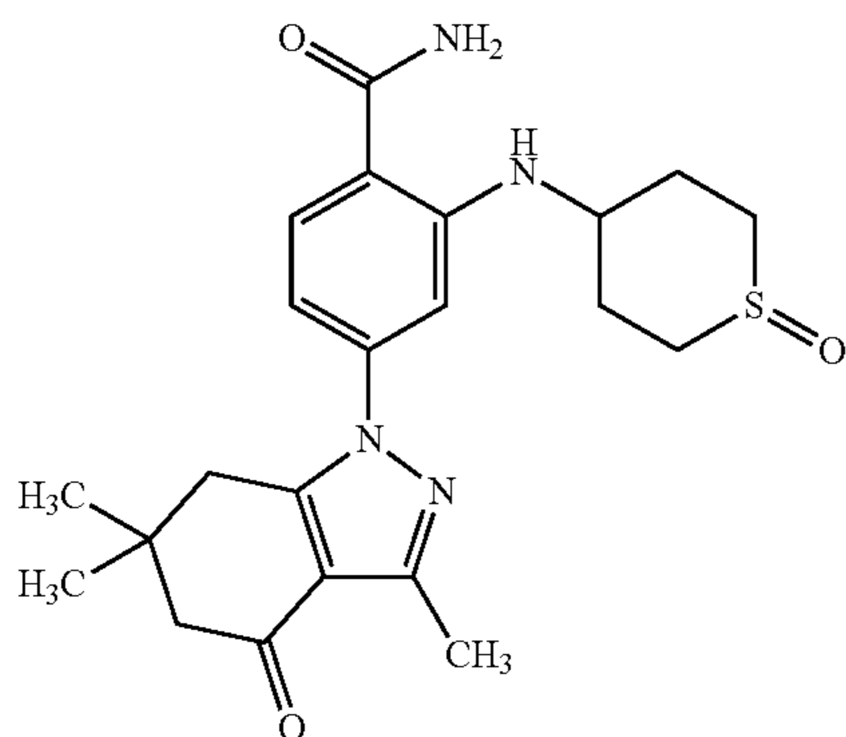
2-(1-Oxo-hexahydro-1-Tetrahydrothiopyran-4-ylamino)-4-(3,6,6-trimethyl-4-oxo-4,5,6,7-tetrahydroindazol-1-yl)benzamide (Compound 14)
