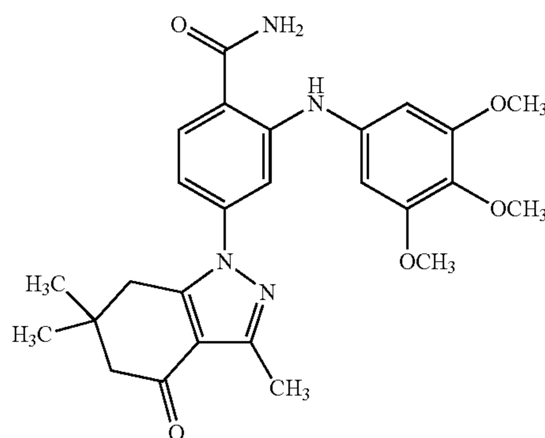
4-(6,6-Dimethyl-4-oxo-3-methyl-4,5,6,7-tetrahydro-indazol-1-yl)-2-(3,4,5-trimethoxyanilino)-benzamide (Compound 19)
