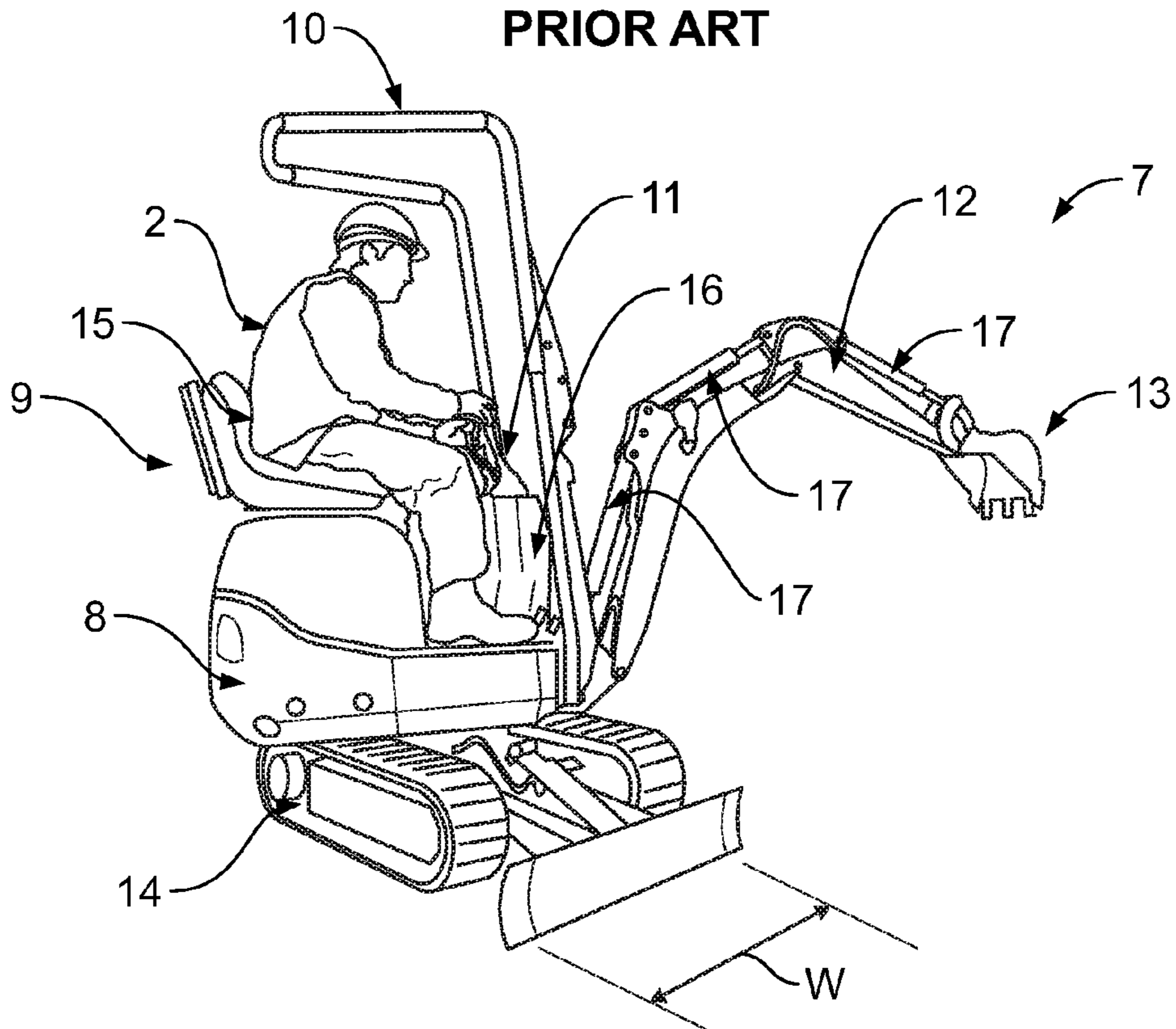
FIG. 2 PRIOR ART
