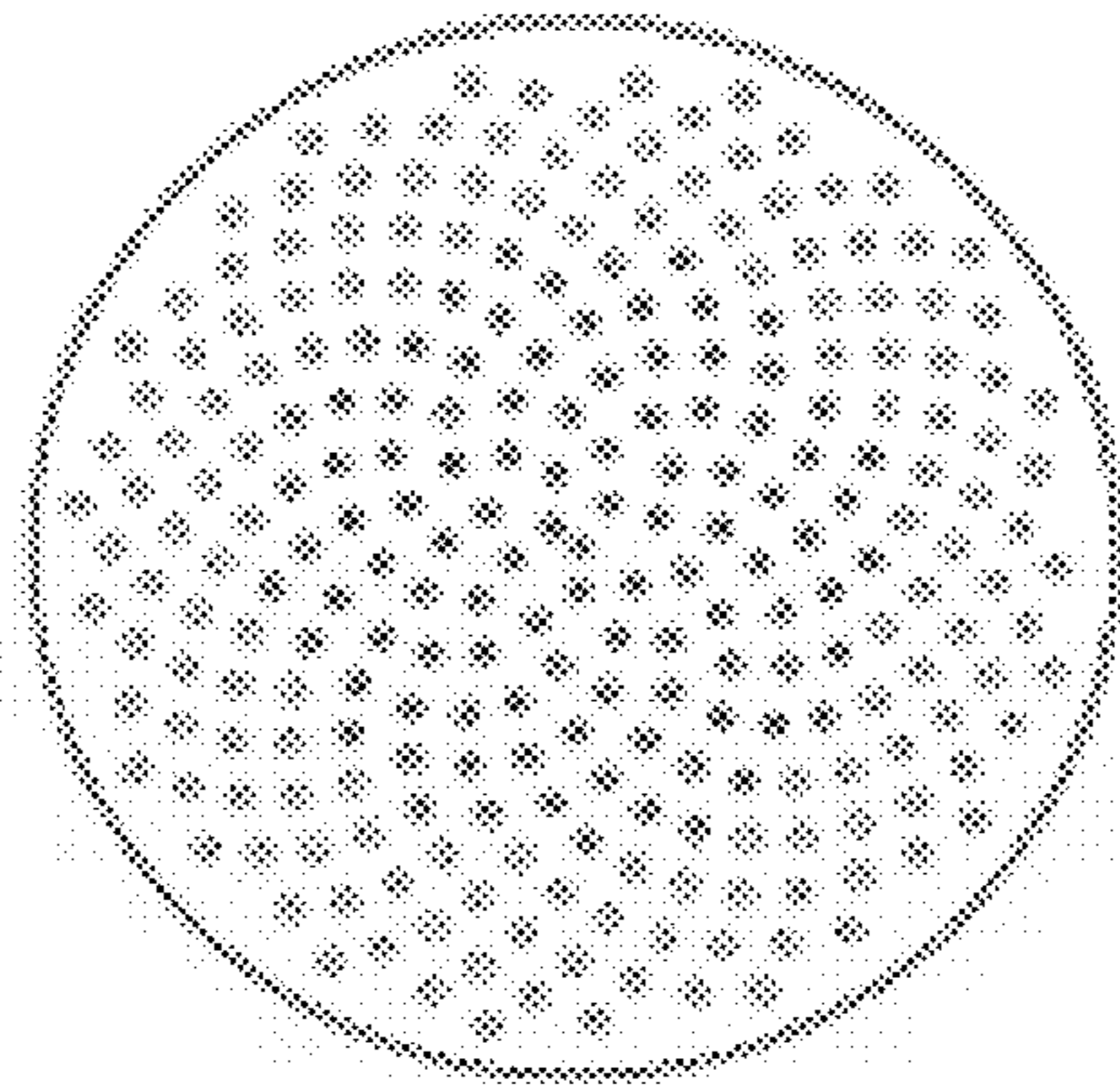
2.65 mm dia 250 holes 5" disc 10.8% removed area
