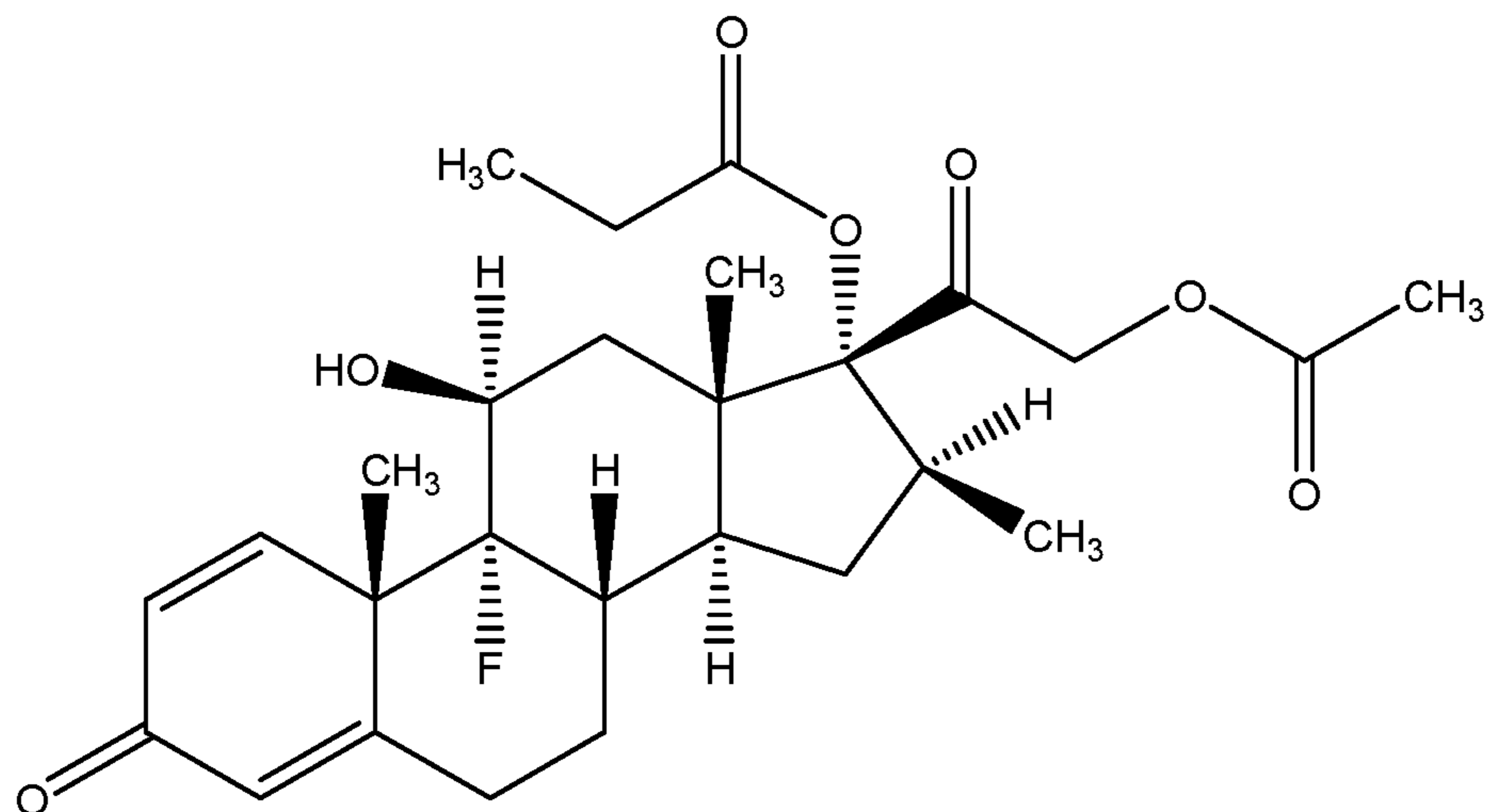
Impurity C (Betamethasone 17-propionate, 21-acetate)
