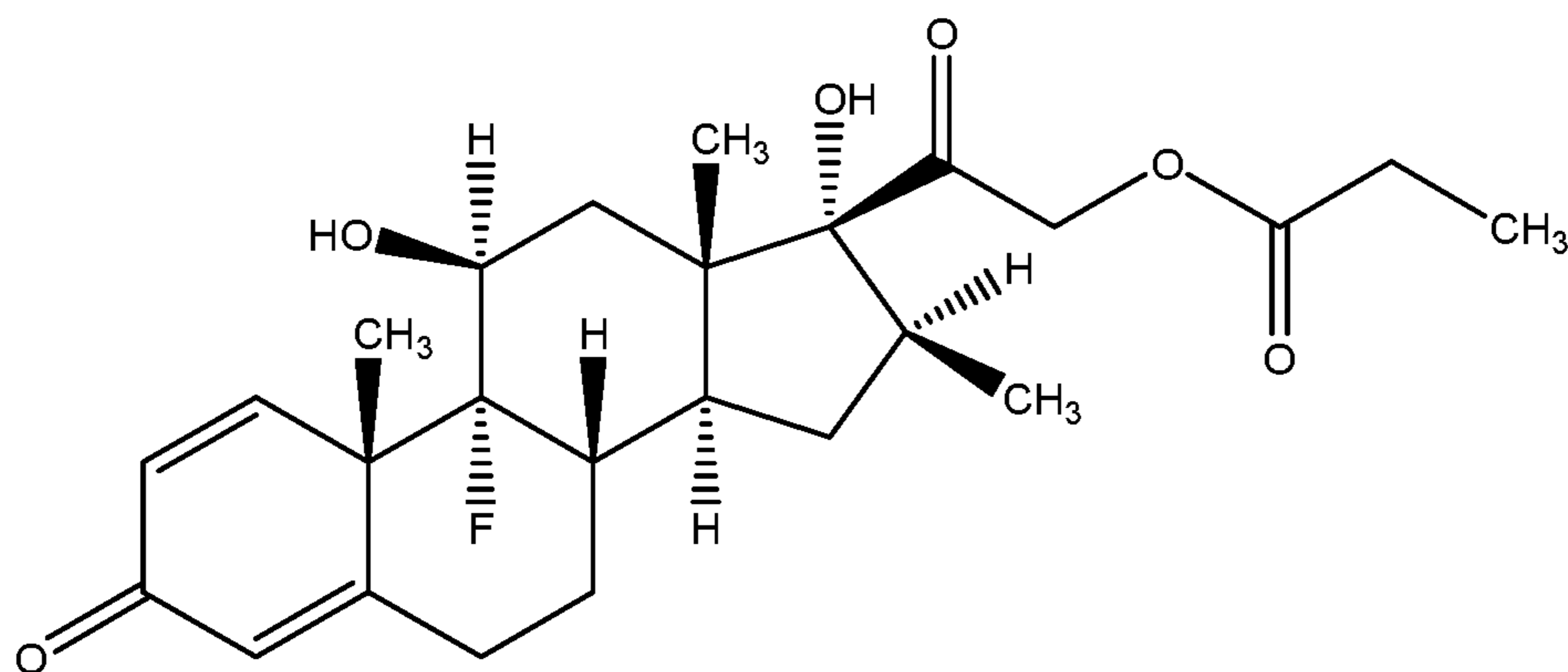
Impurity B (Betamethasone 21-propionate)
