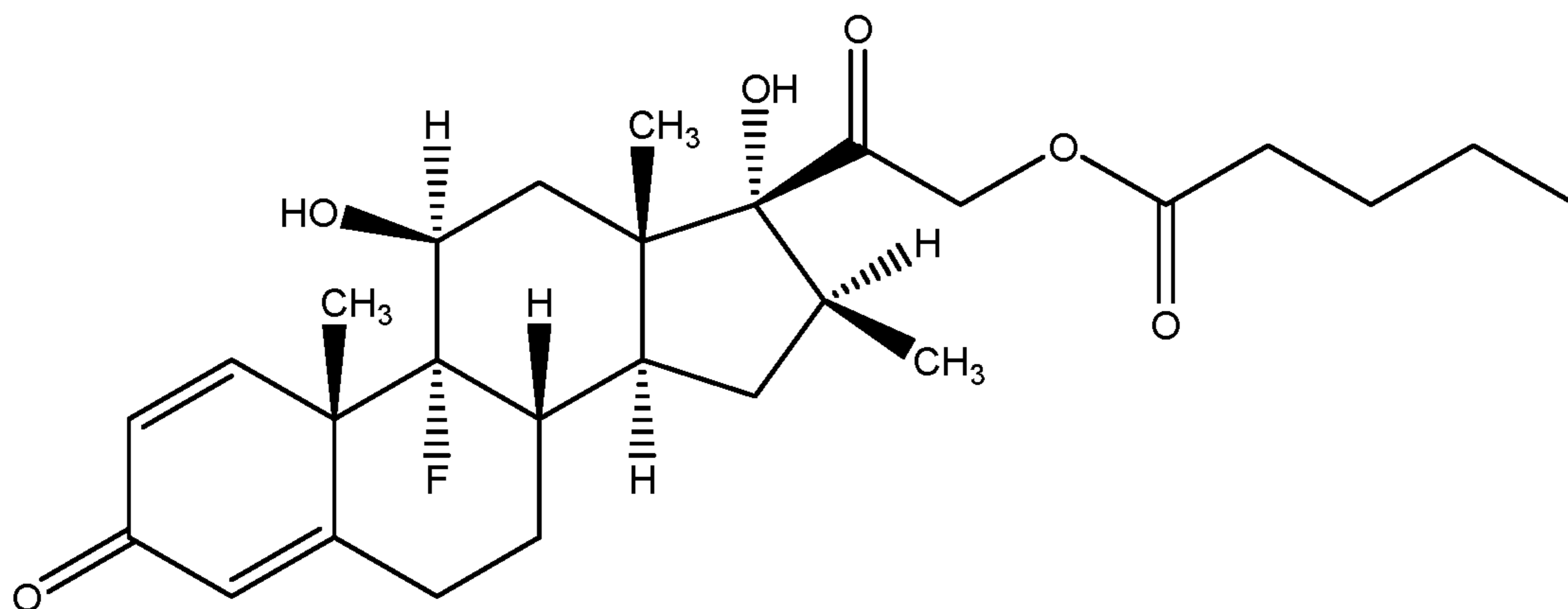
Impurity D (Betamethasone 21-valerate)
