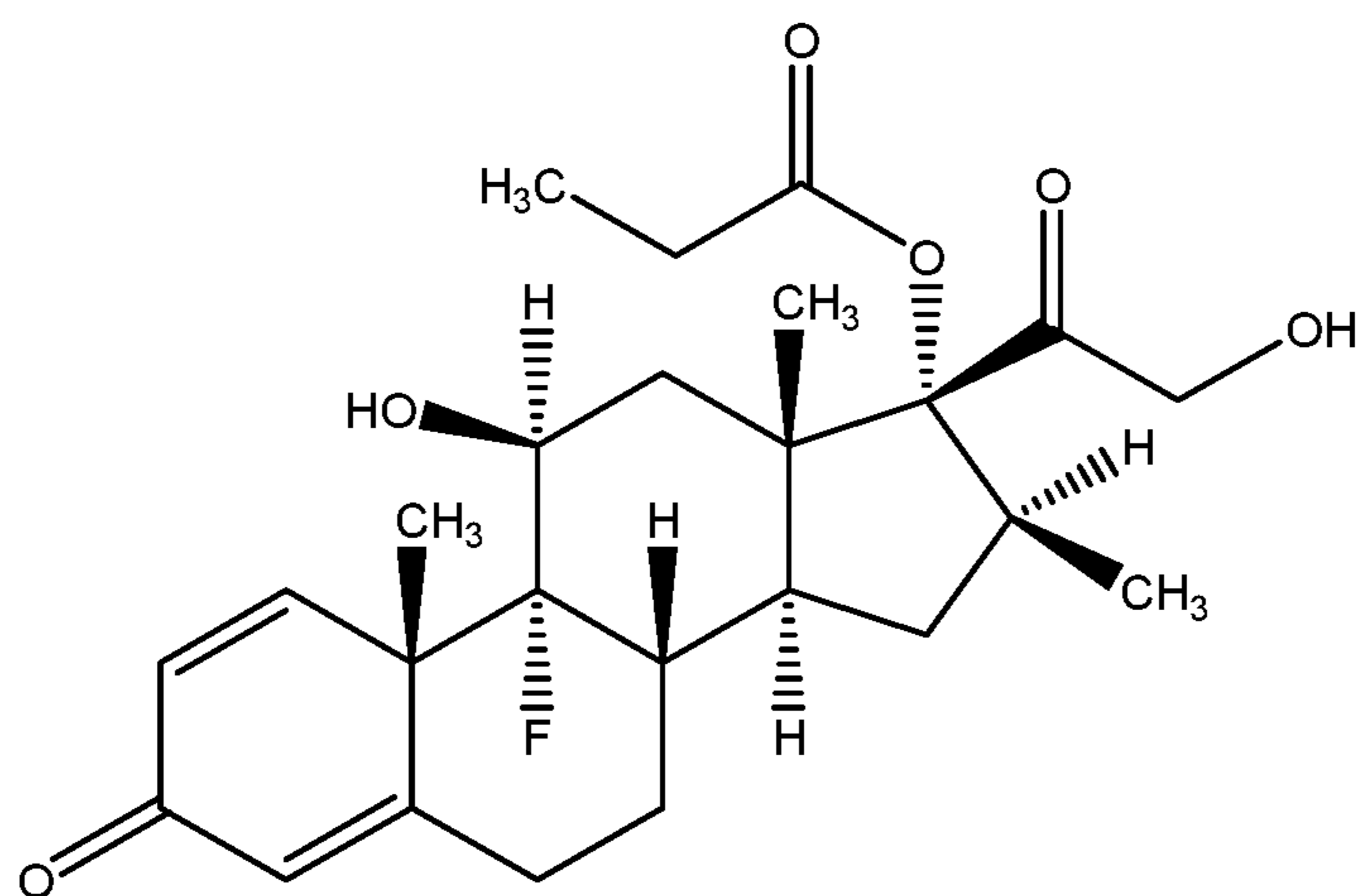
Impurity A (Betamethasone 17-propionate)
