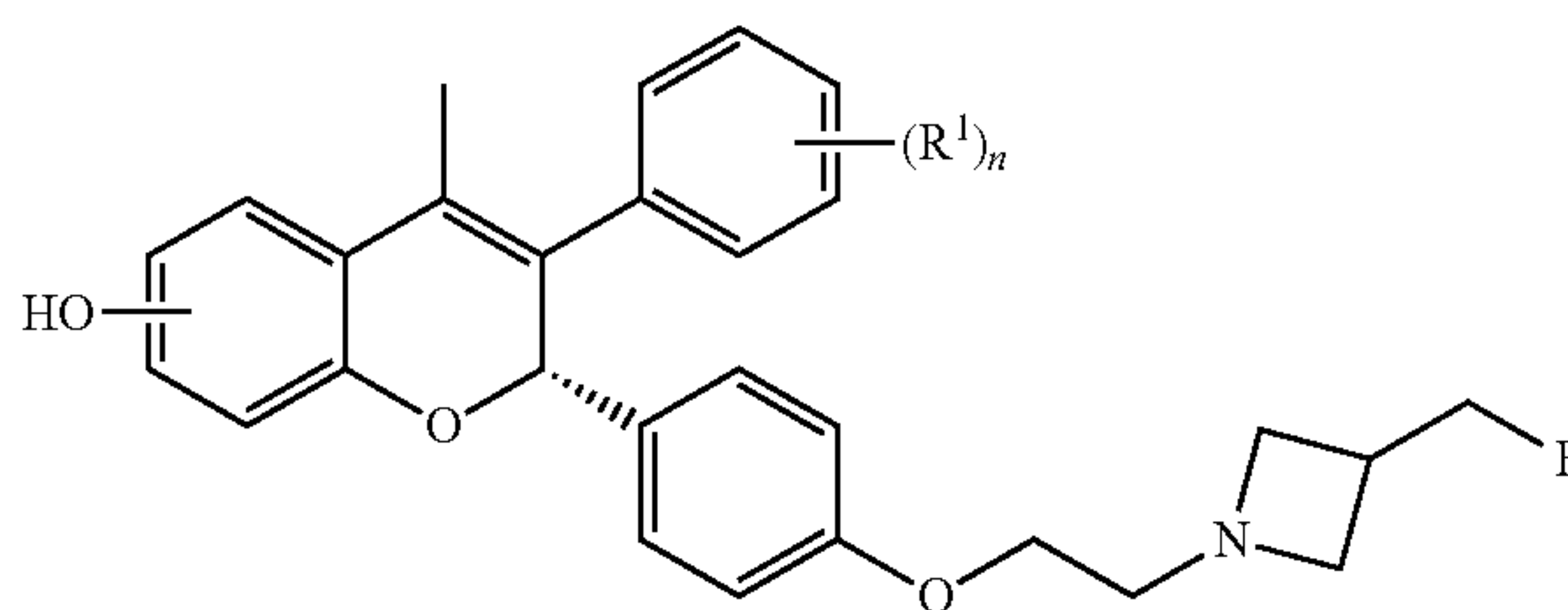
Formula (III)
