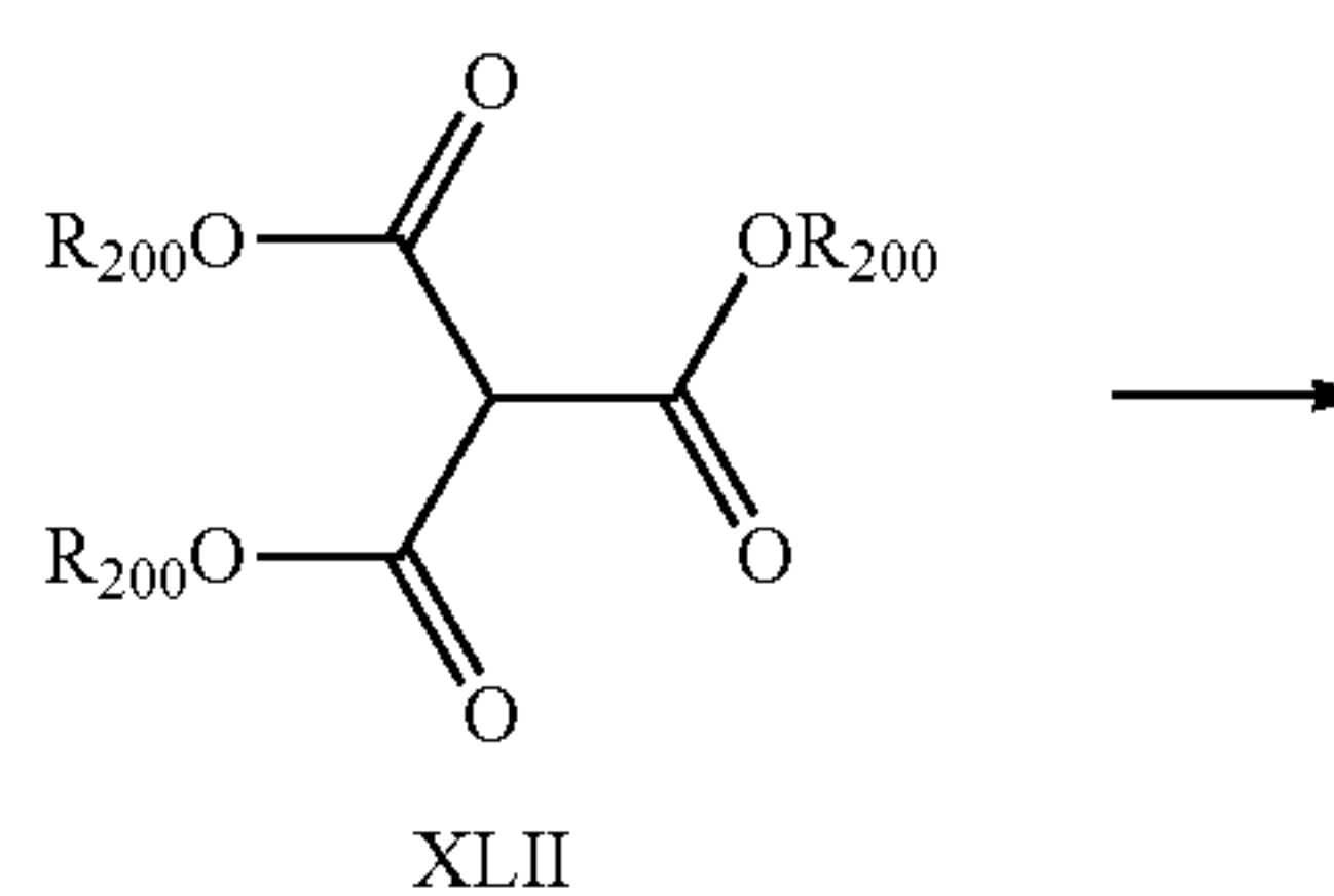
Scheme 12.
