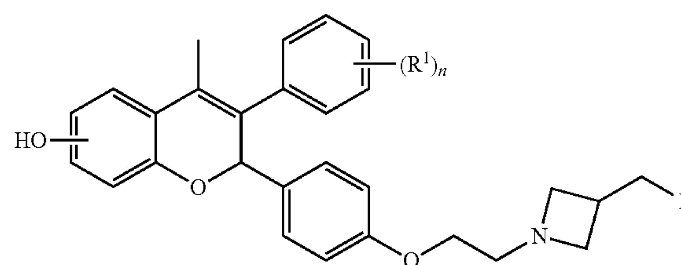
Formula (I)
