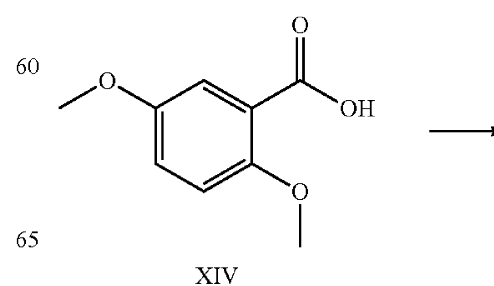
Scheme 4:
