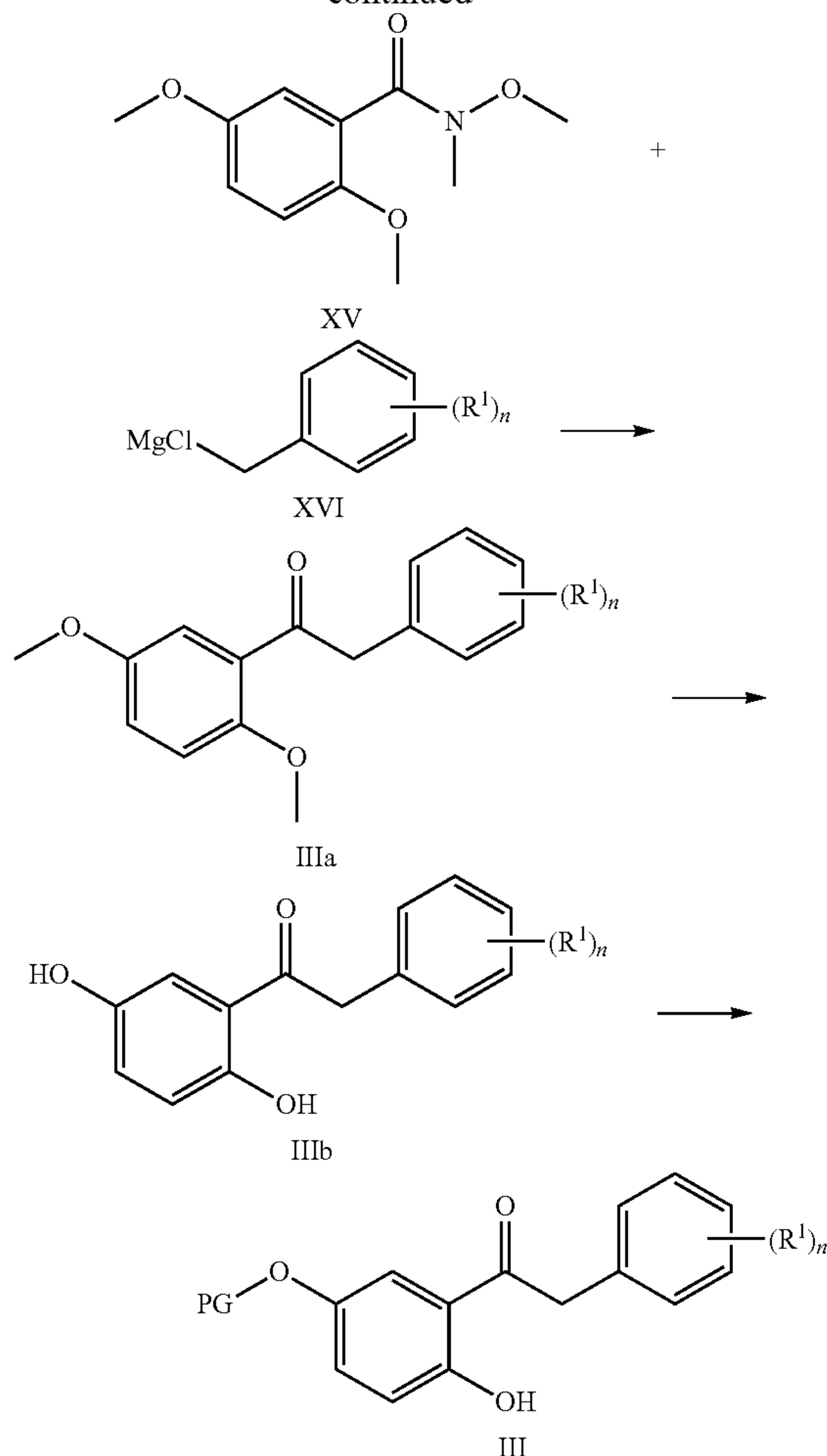
Scheme 6:
