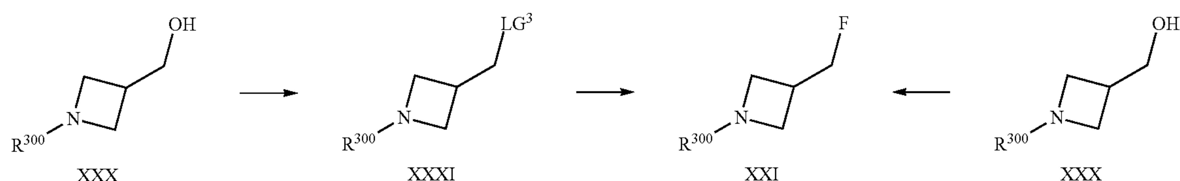
Scheme 9.
