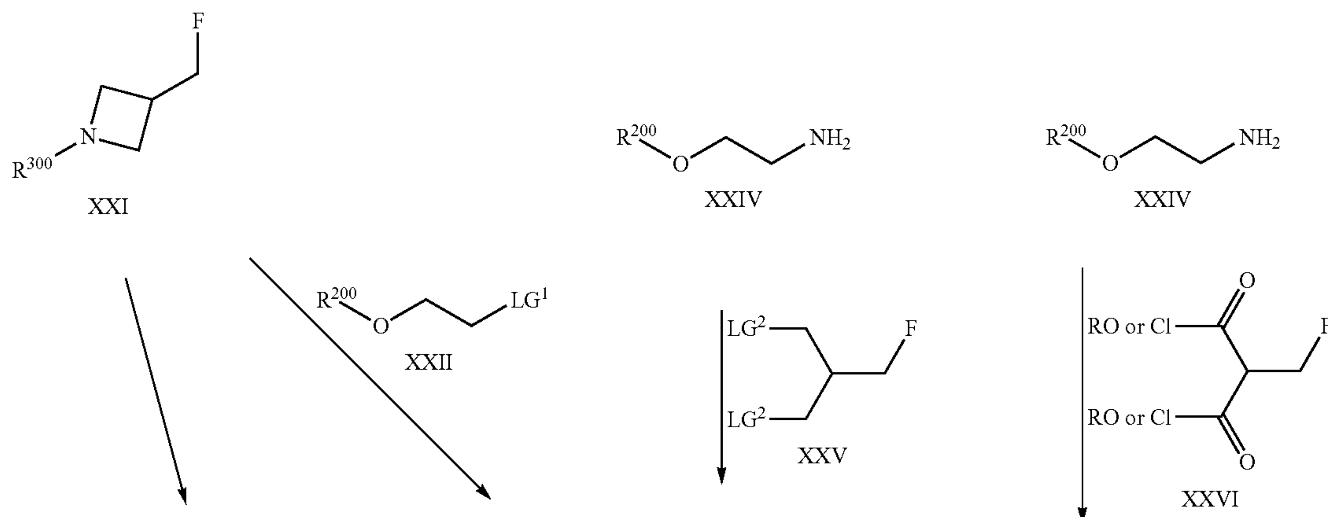
Scheme 8:
