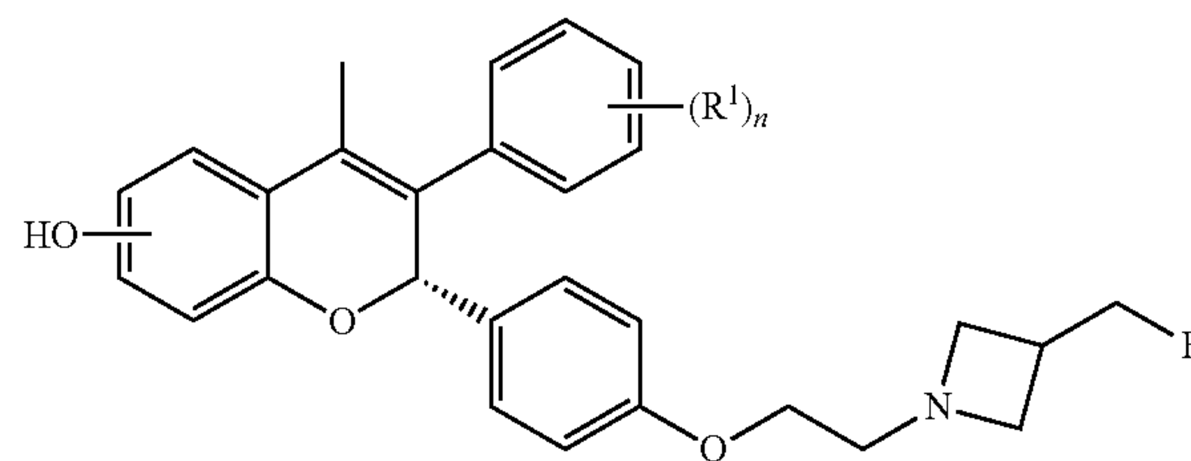
Formula (III)
