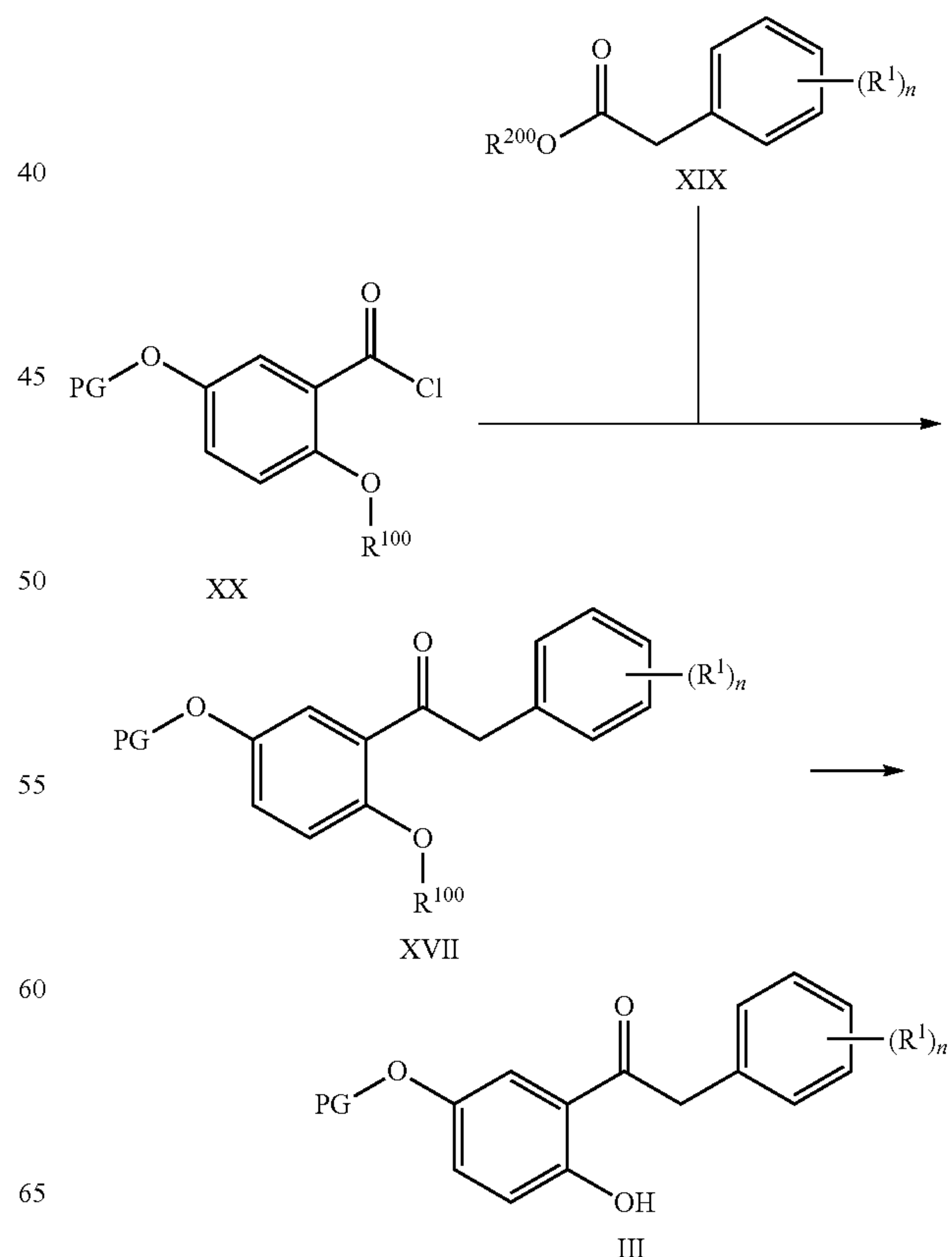
Scheme 6:
