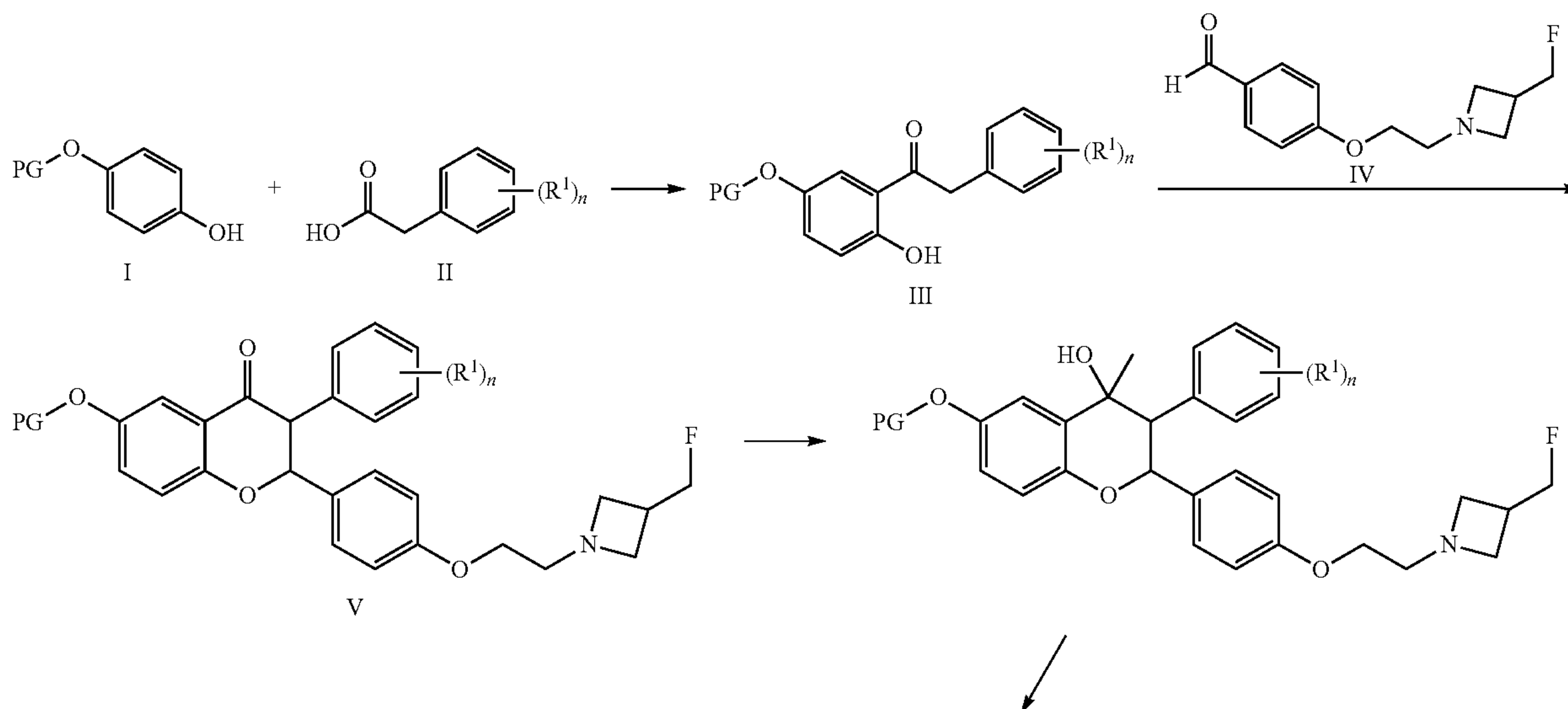
Scheme 1:
