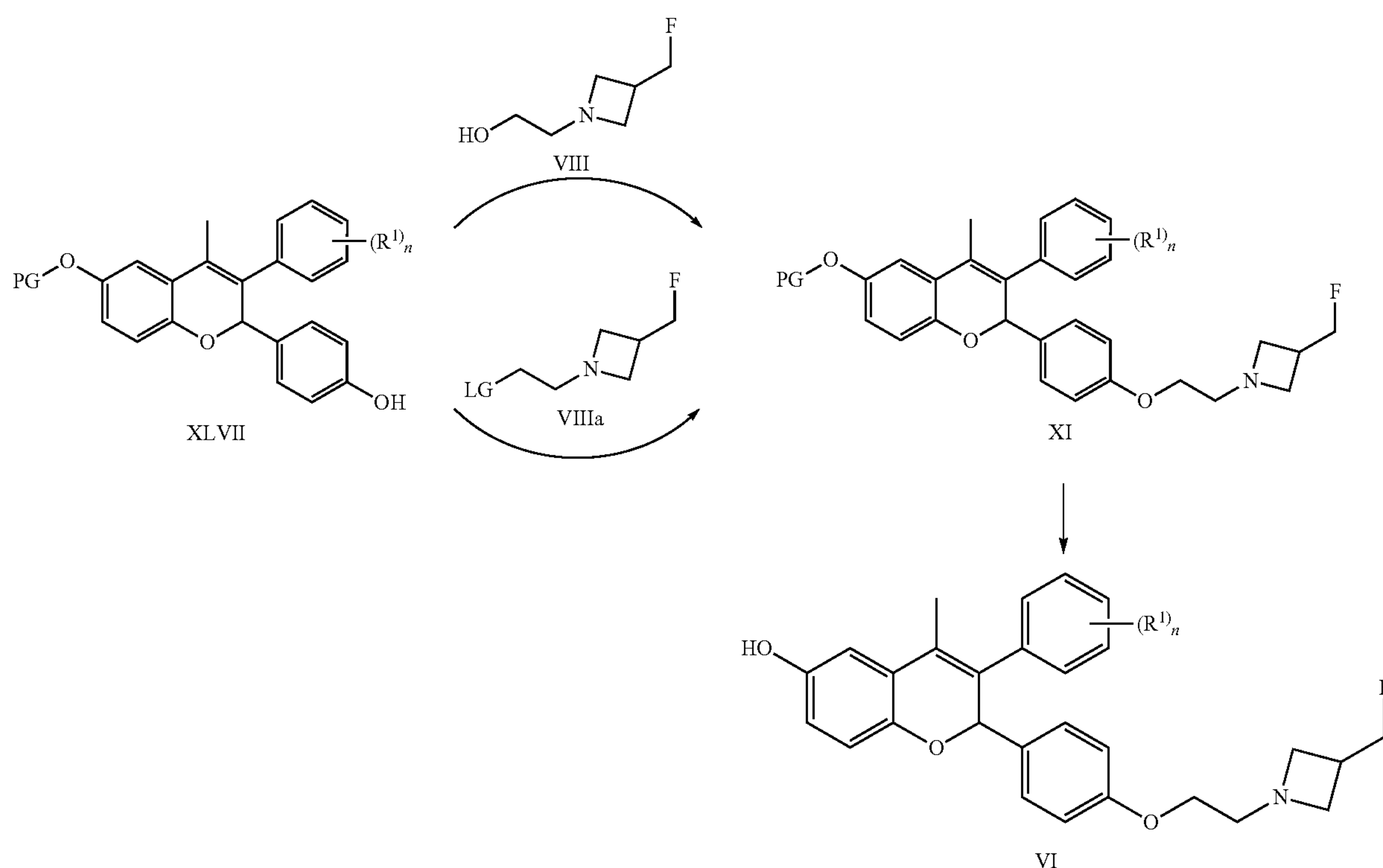
Scheme 13.
