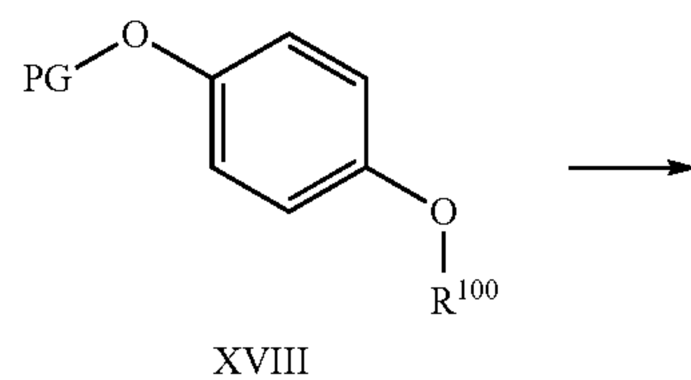
Scheme 5:
