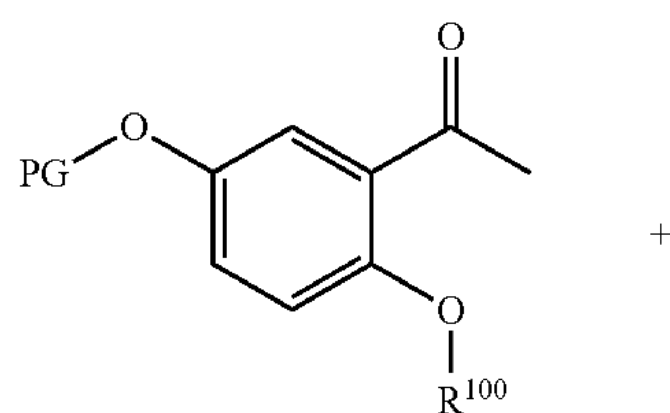
Scheme 7.
