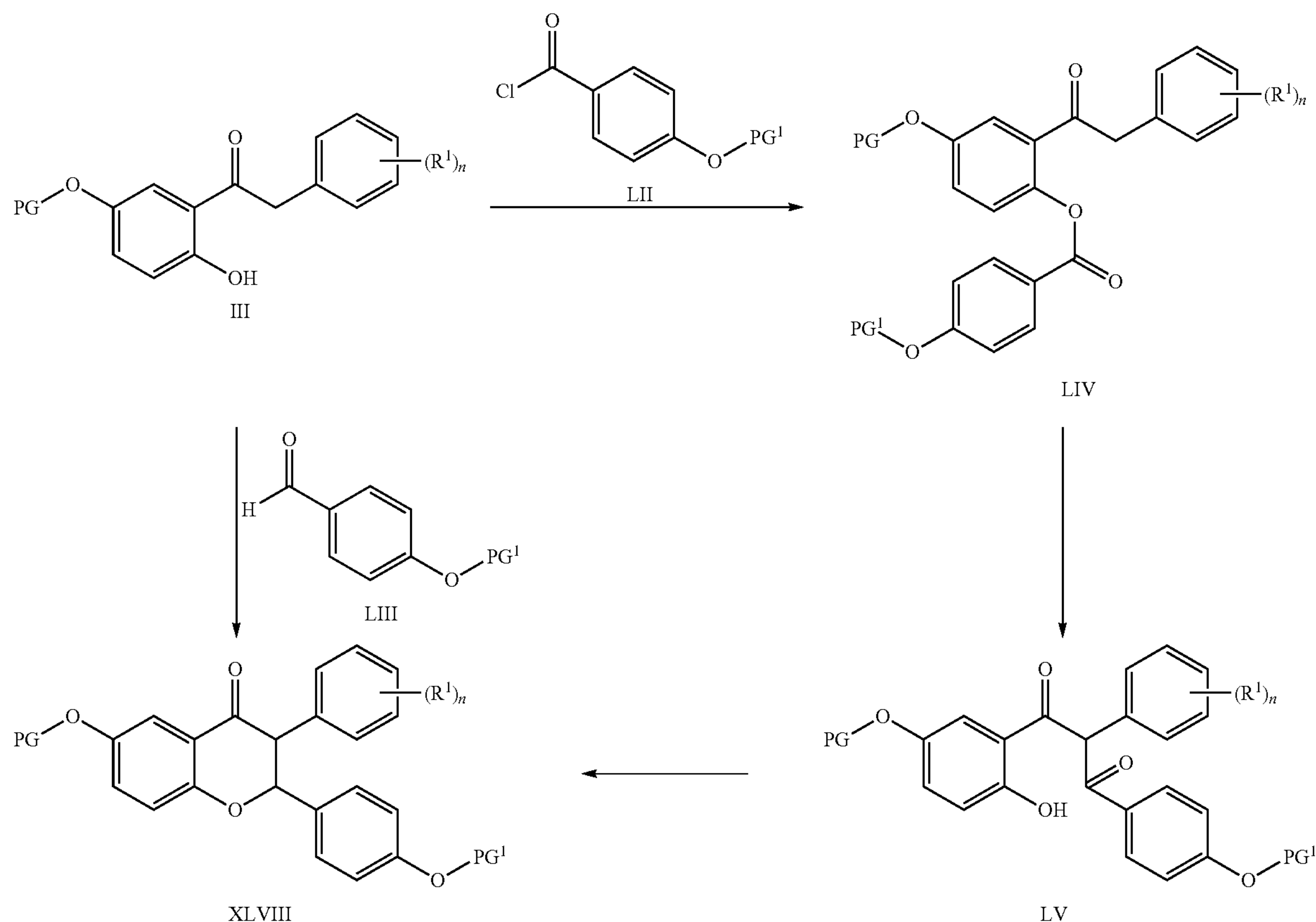
Scheme 15.
