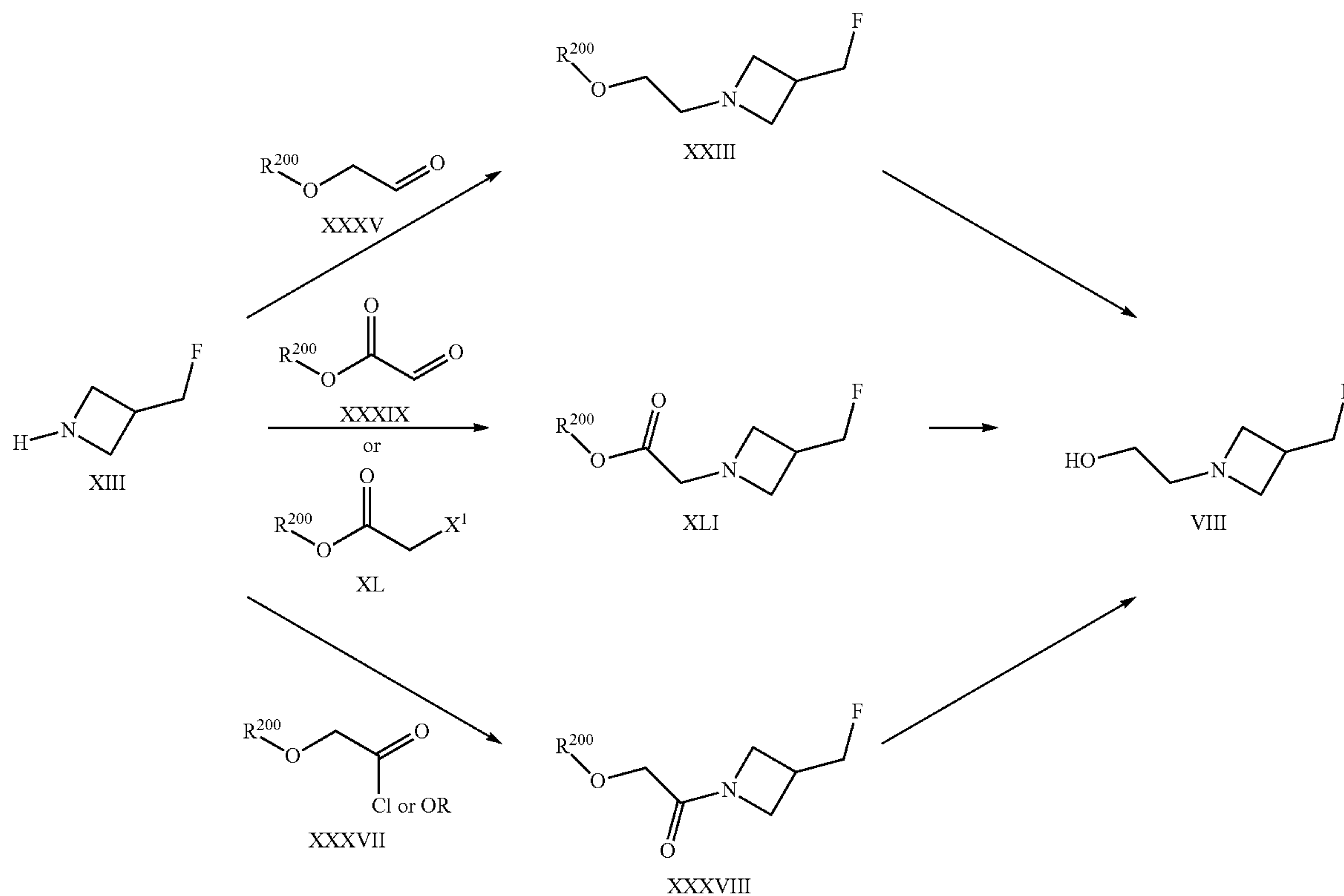
Scheme 11
