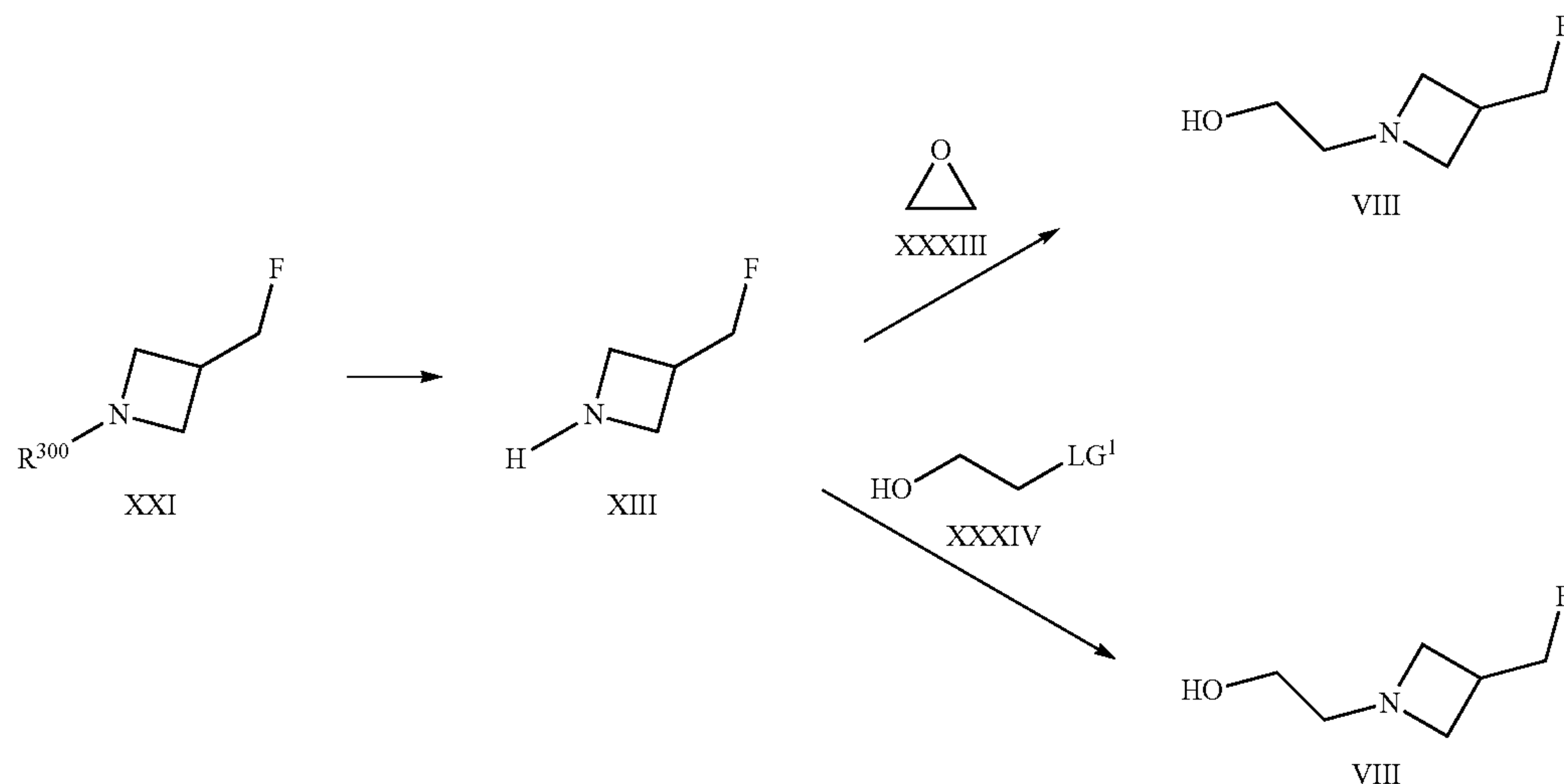
Scheme 10.
