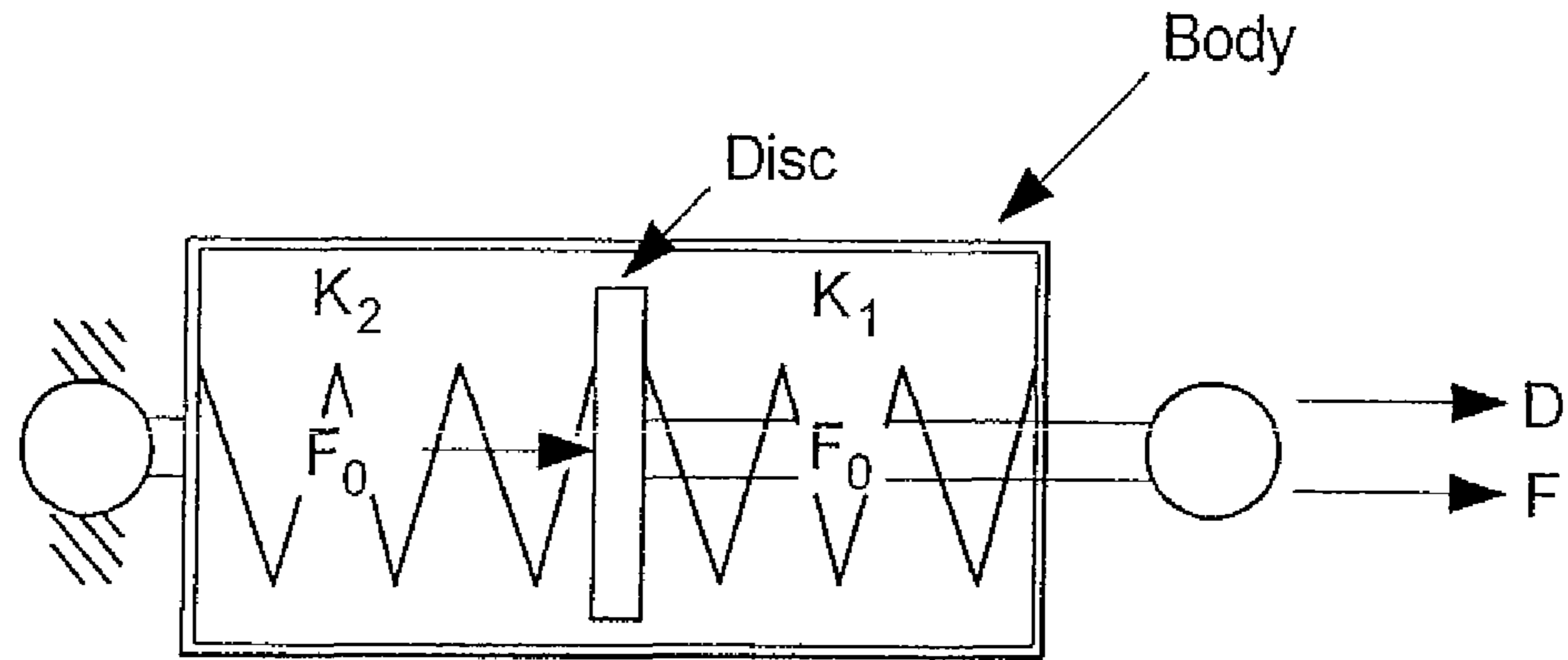
Free-body diagram
