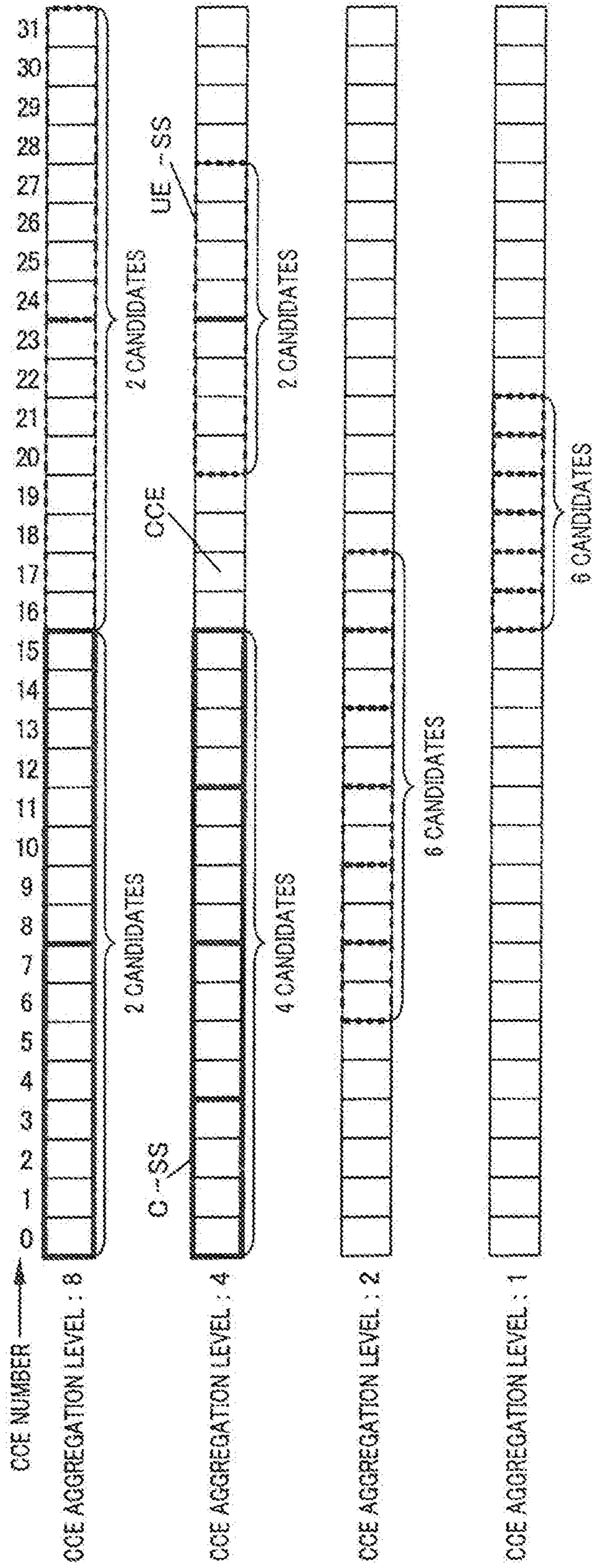
FIG. 2 PRIOR ART
