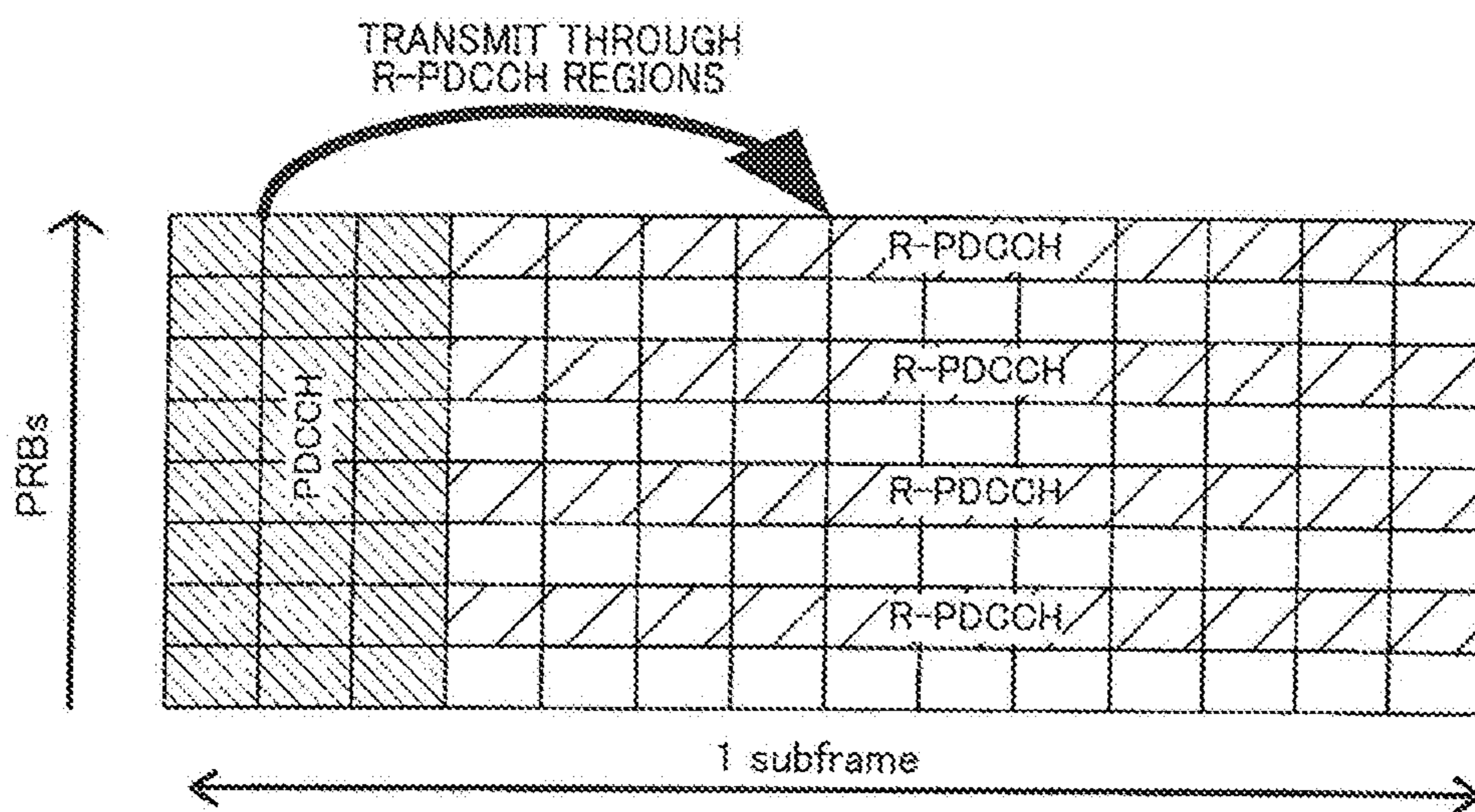
FIG. 6 PRIOR ART
