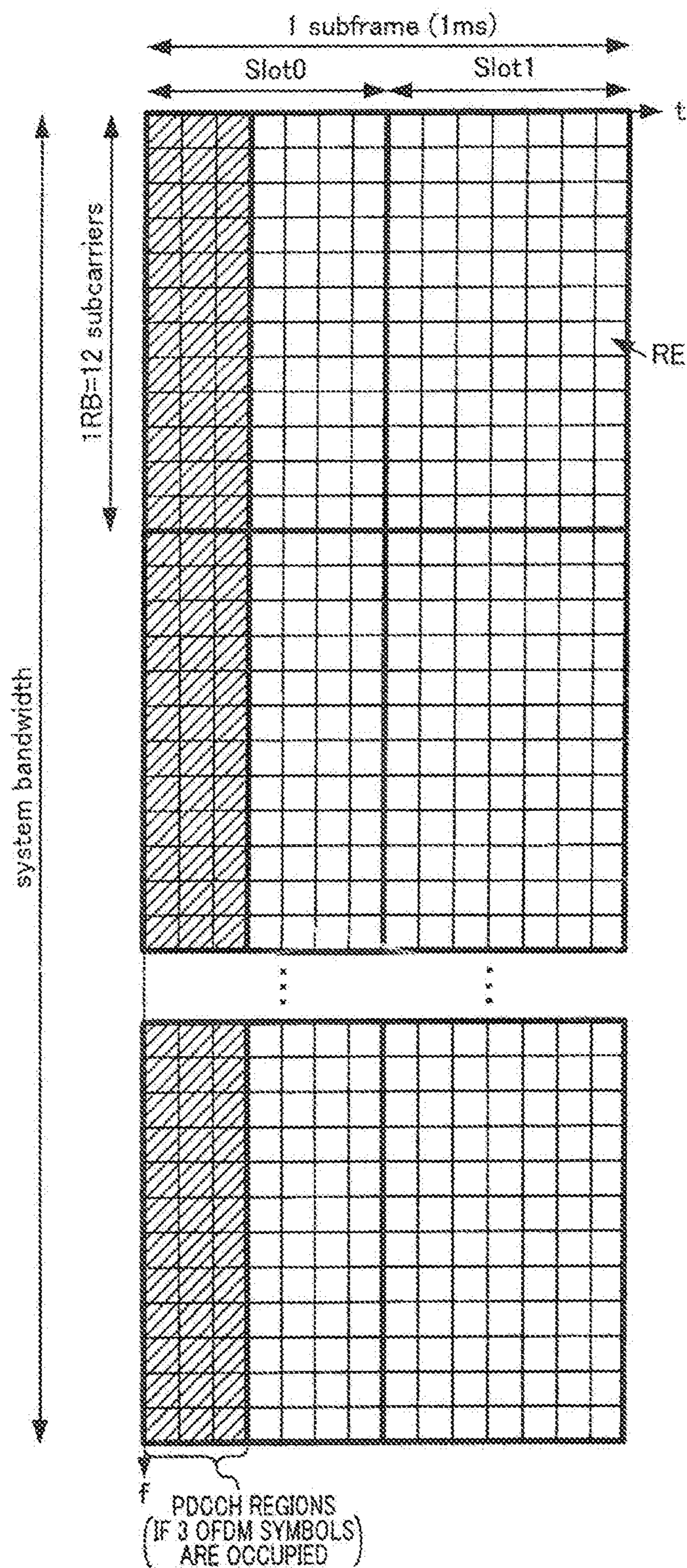
FIG. 1 PRIOR ART
