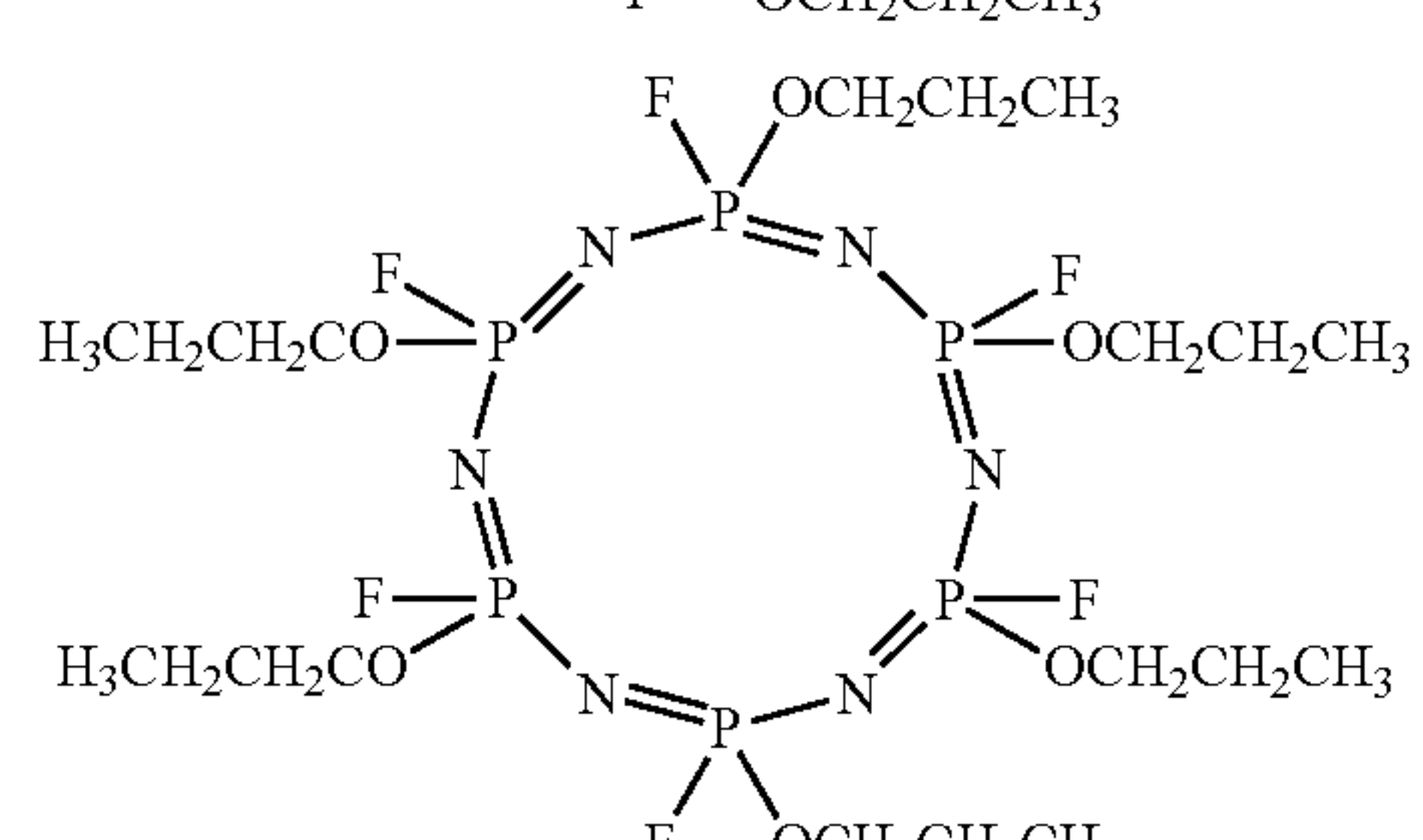
(cyclohexaphosphazenes having propyl group(s) through oxygen)
