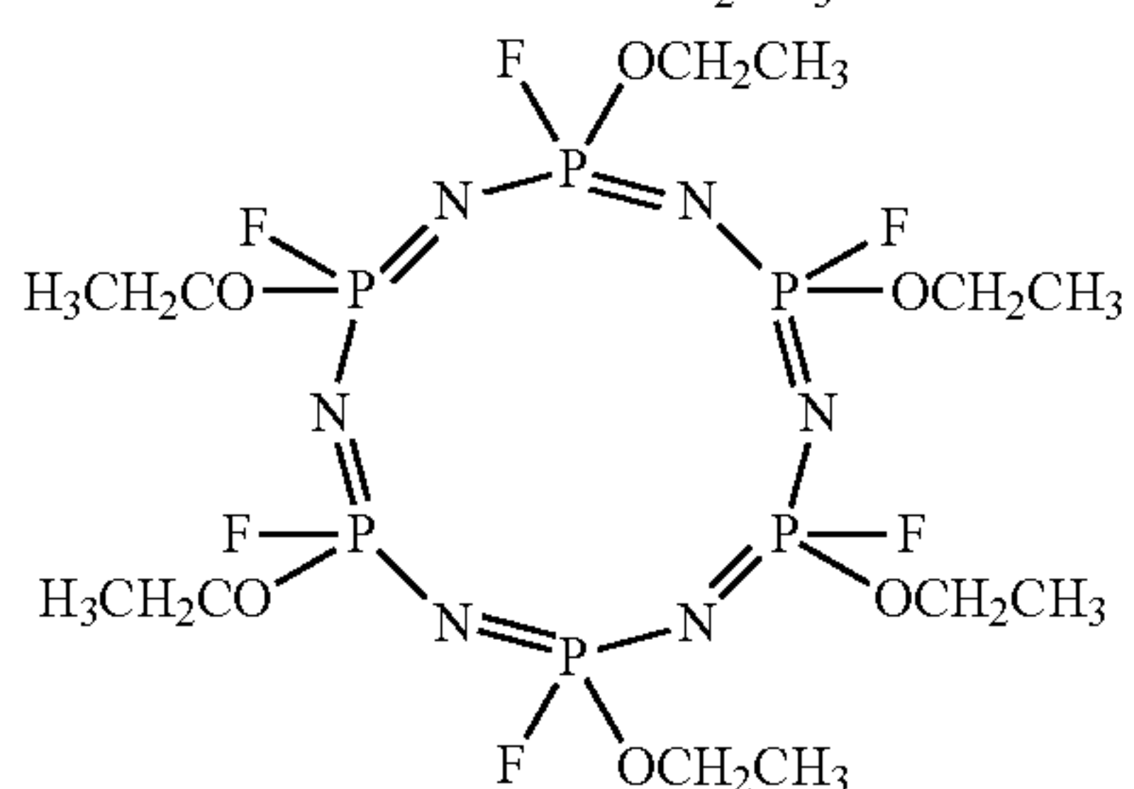
(cyclohexaphosphazenes having ethyl group(s) through oxygen)
