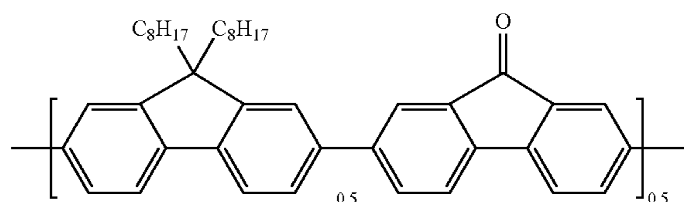
PFFO (poly(9,9-dioctylfluorene-co-fluorenone))
