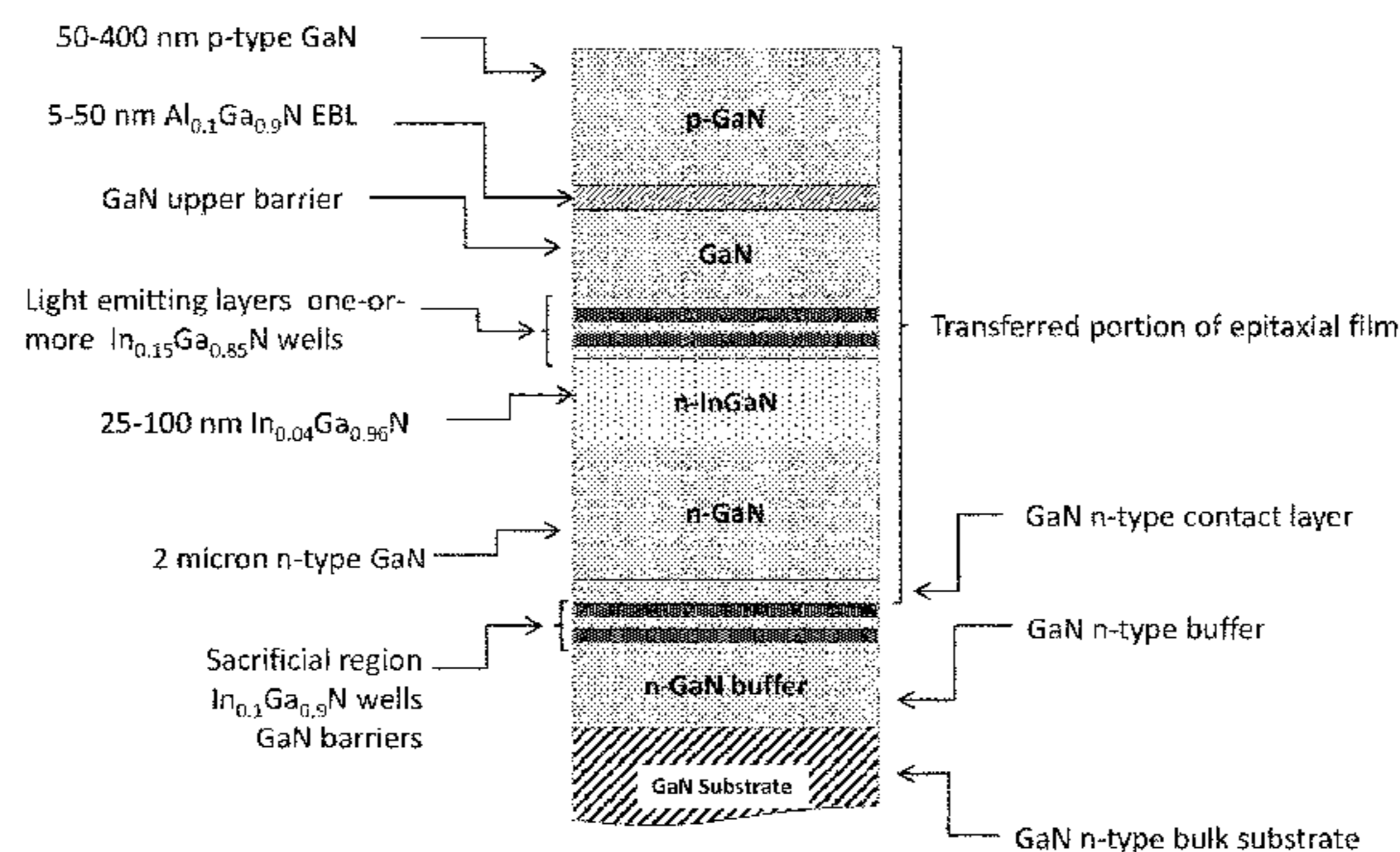
schematic of epitaxial structure of LED
