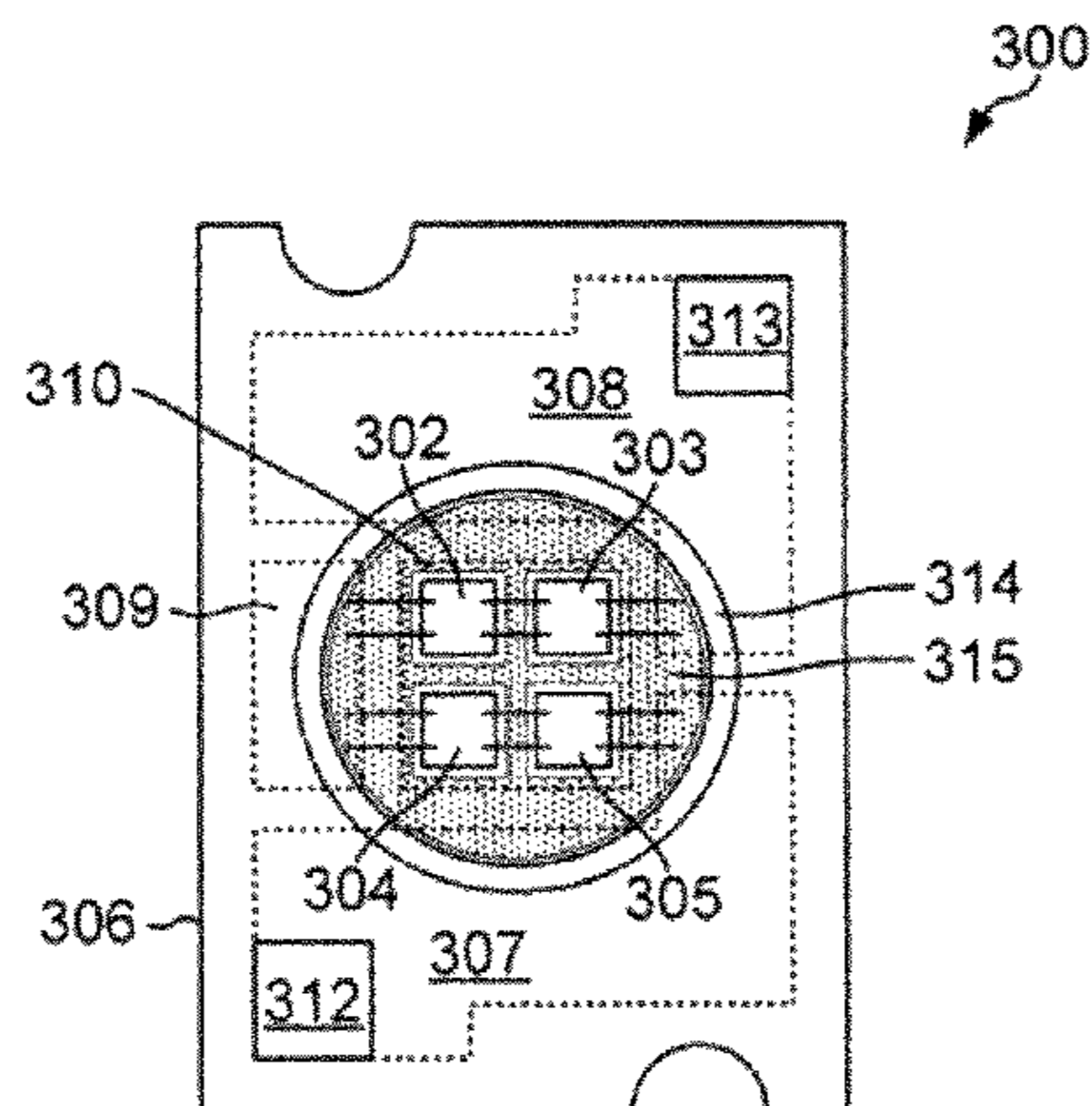
TOP-DOWN VIEW OF WHITE LED ASSEMBLY
