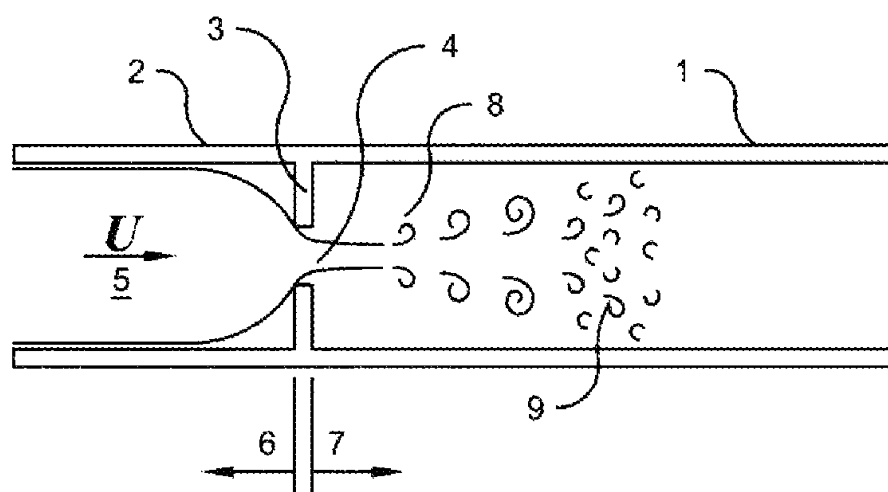
Fig. 1 (Prior Art)
