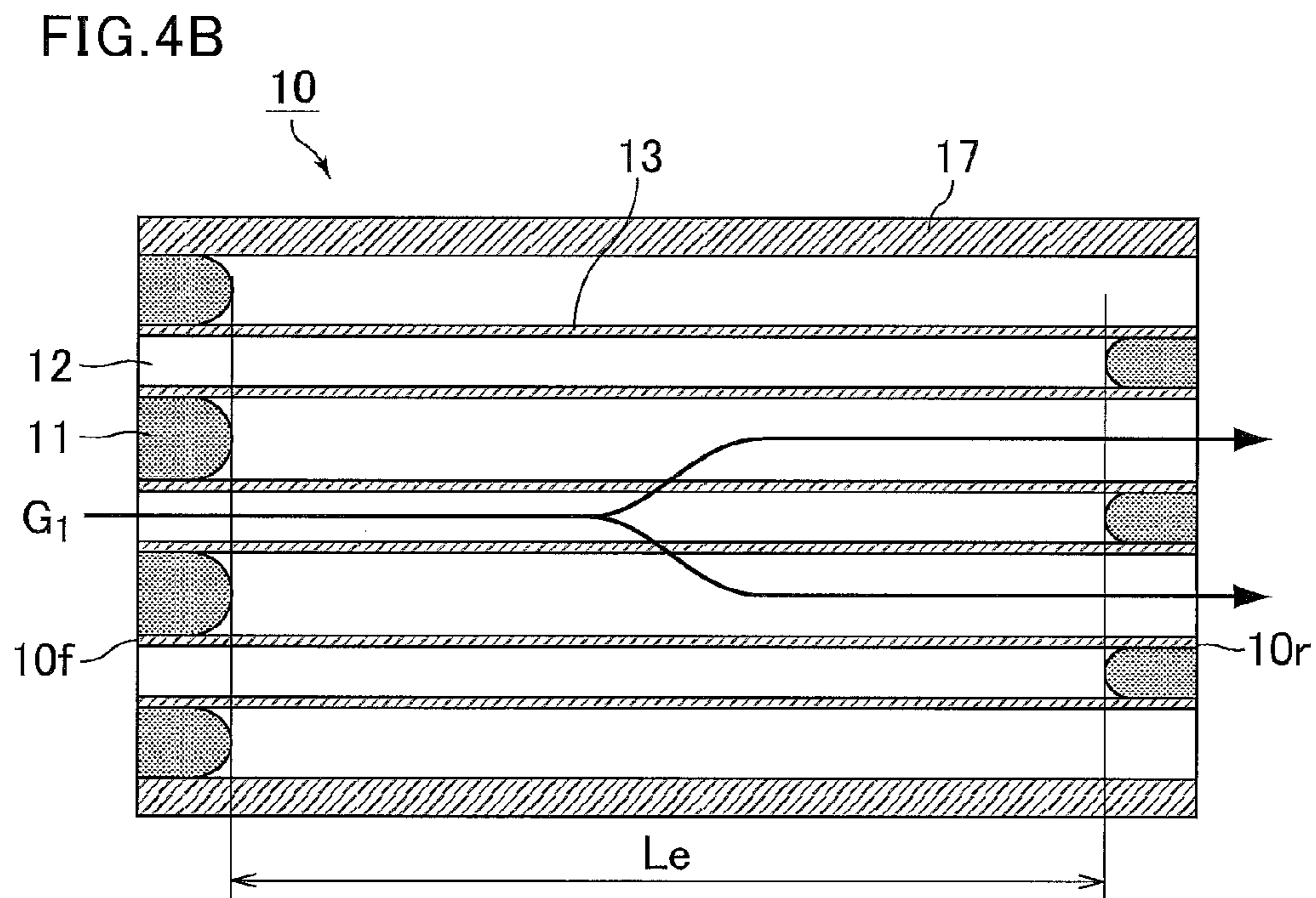
A-A line cross sectional view
