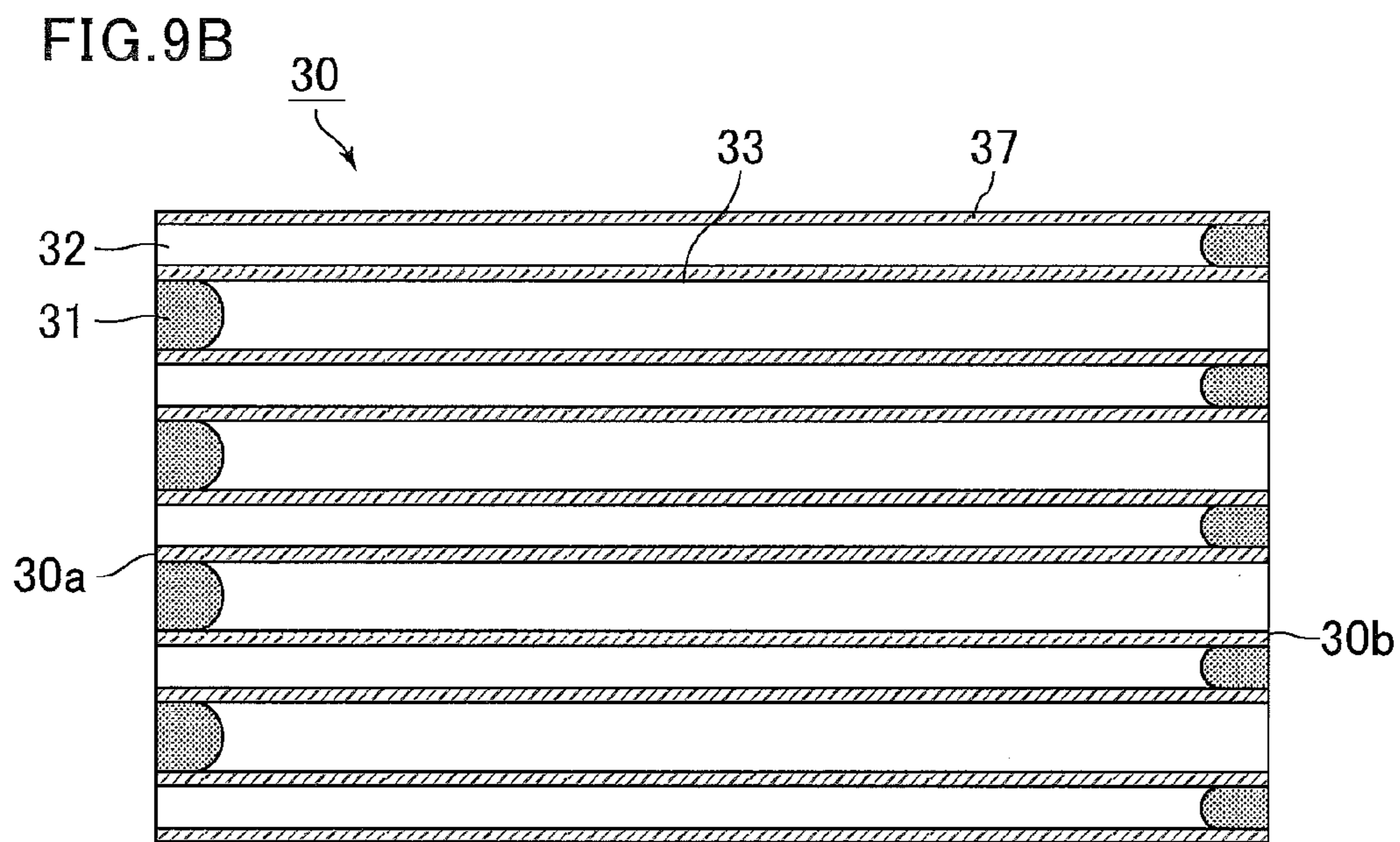
B-B line cross sectional view
