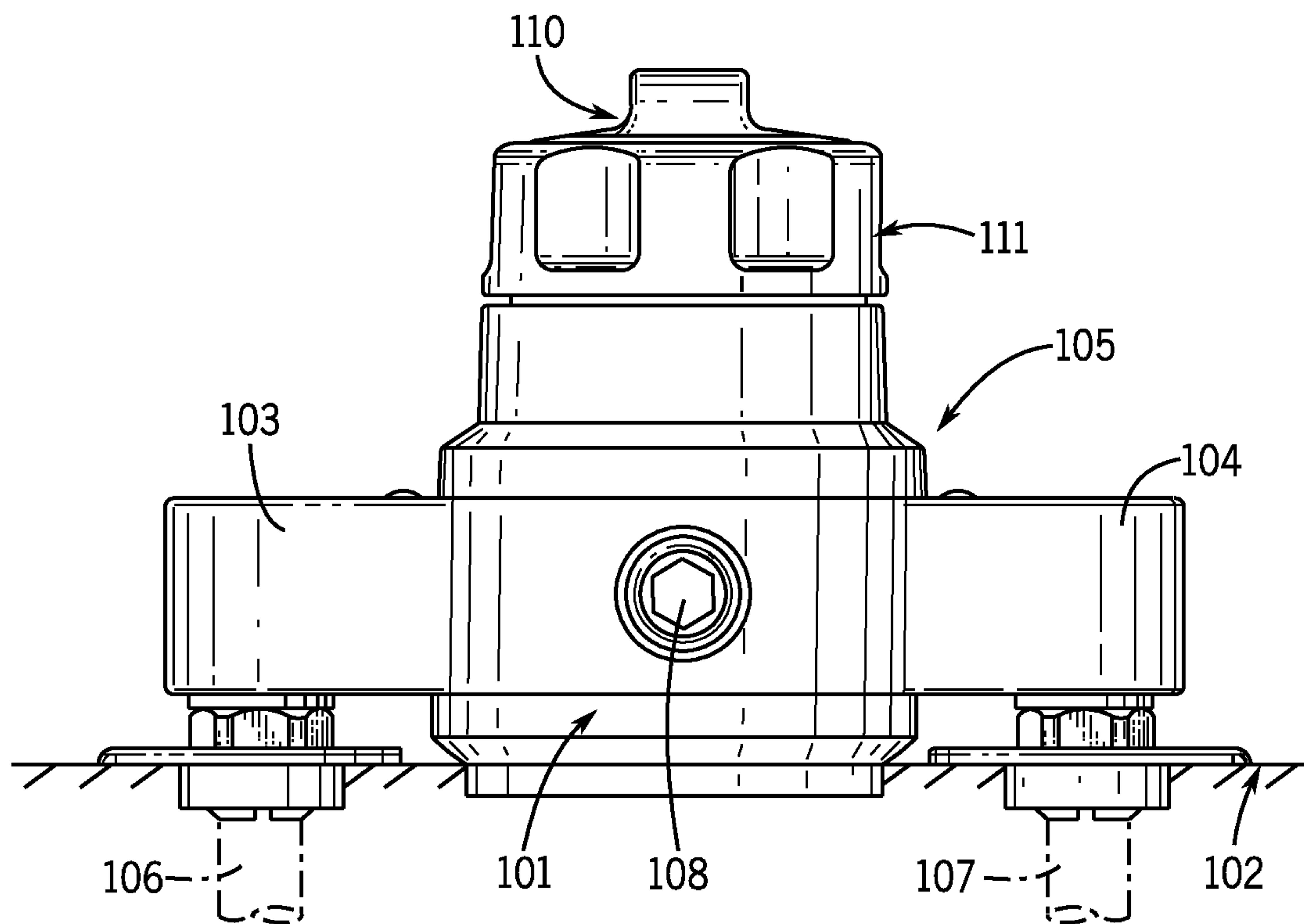
FIG. 13 PRIOR ART
