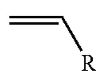
Scheme 1. Schematic showing of the basic mechanism of RAFT polymerization using a telechelic chain transfer agent. AIBN is an exemplary chain initiator, azobisisobutyronitrile; and
