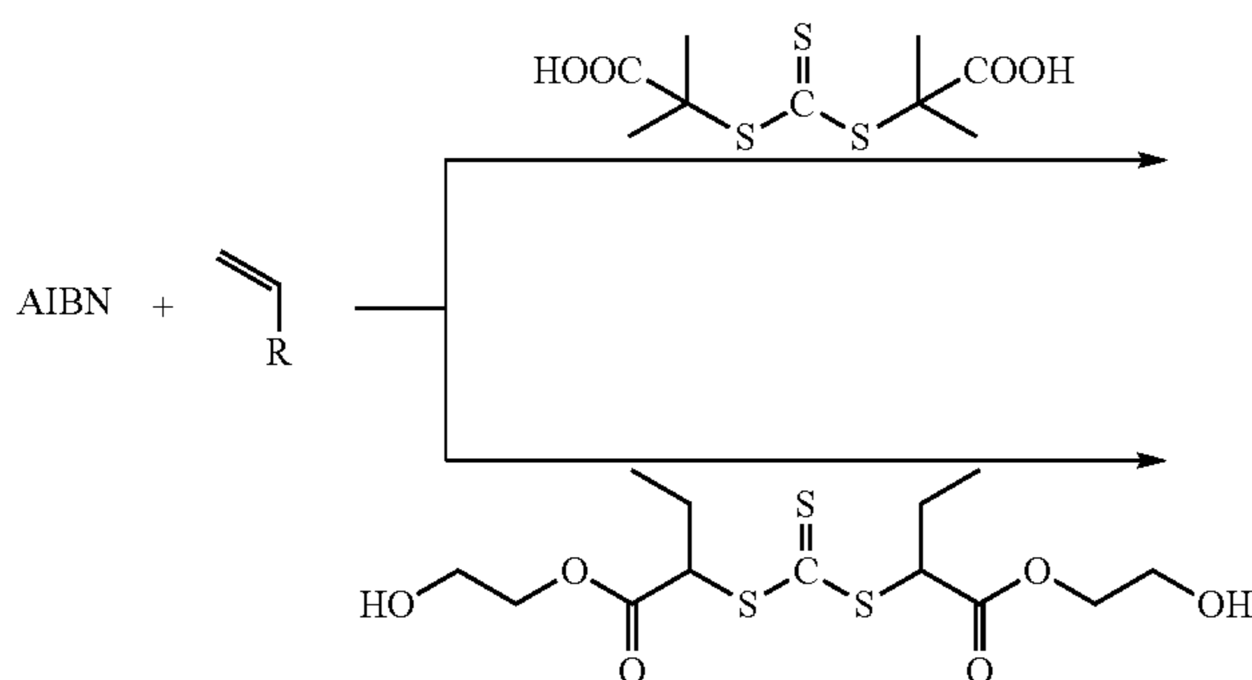
Scheme 1. Schematic showing of the basic mechanism of RAFT polymerization using a telechelic chain transfer agent. AIBN is an exemplary chain initiator, azobisisobutyronitrile; and
