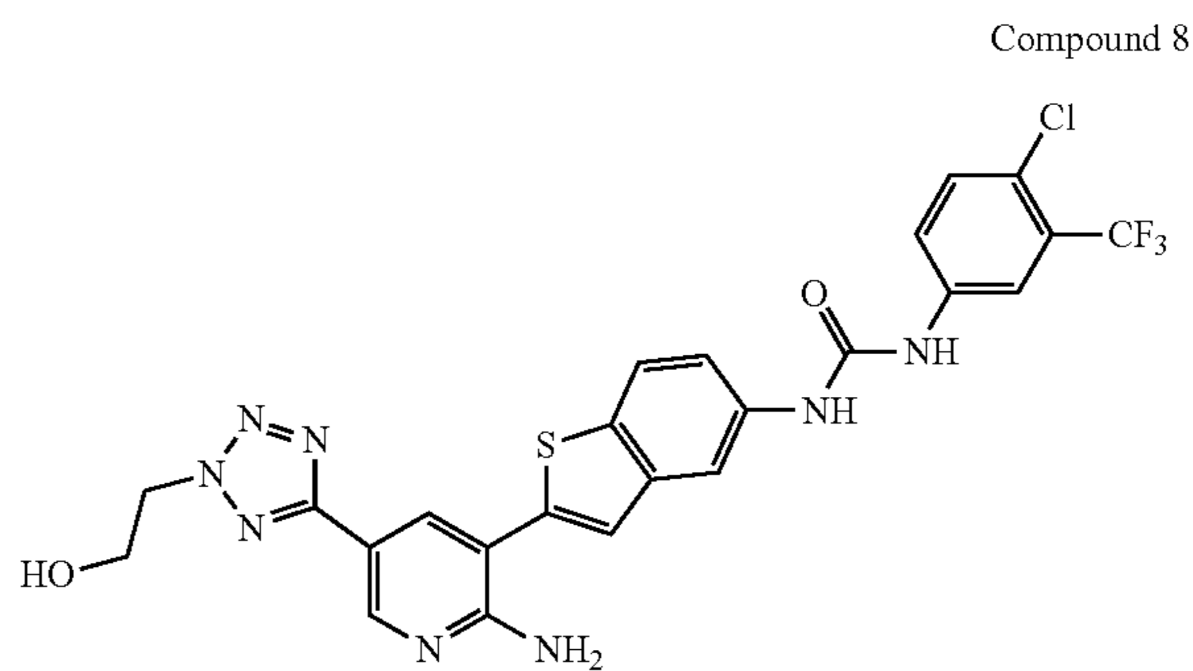
1-(2-{2-amino-5-[2-(2-hydroxyethyl)-2H-tetrazol-5-yl]pyridin-3-yl}-1-benzothien-5-yl)-3-[4-chloro-3-(trifluoromethyl)phenyl]urea
