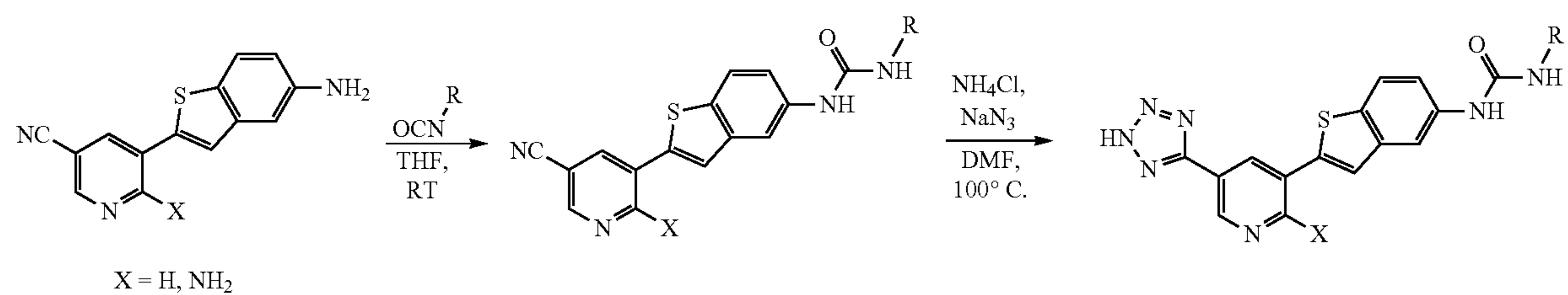
Scheme 3
