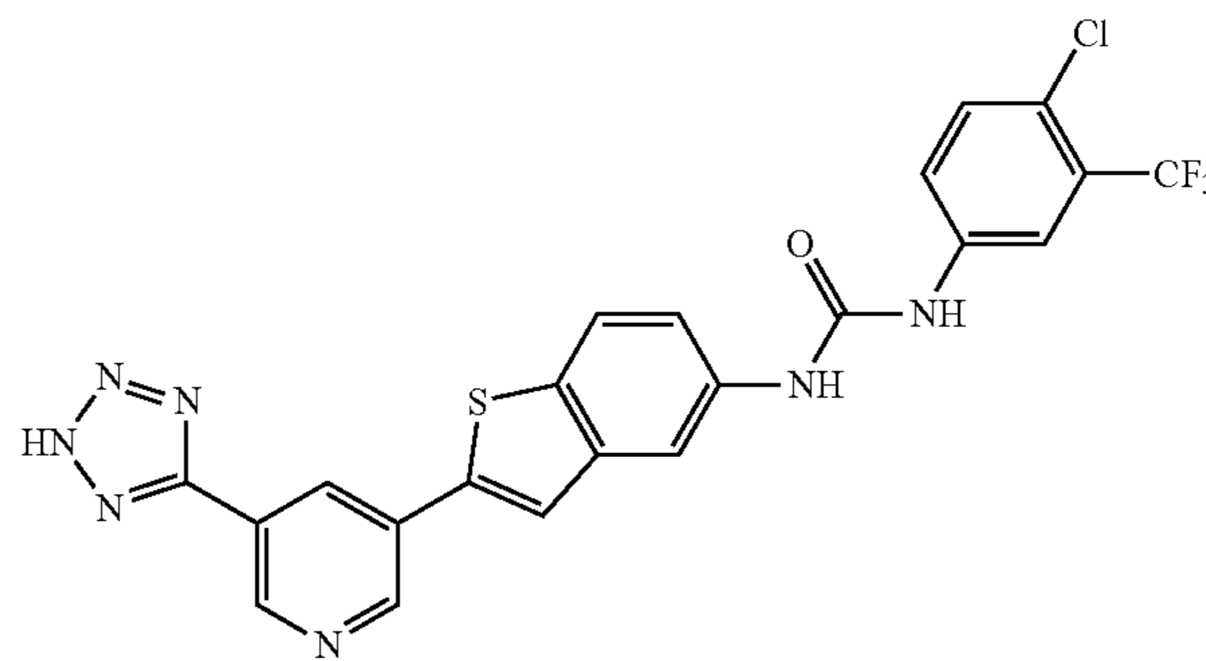
Compound 1
