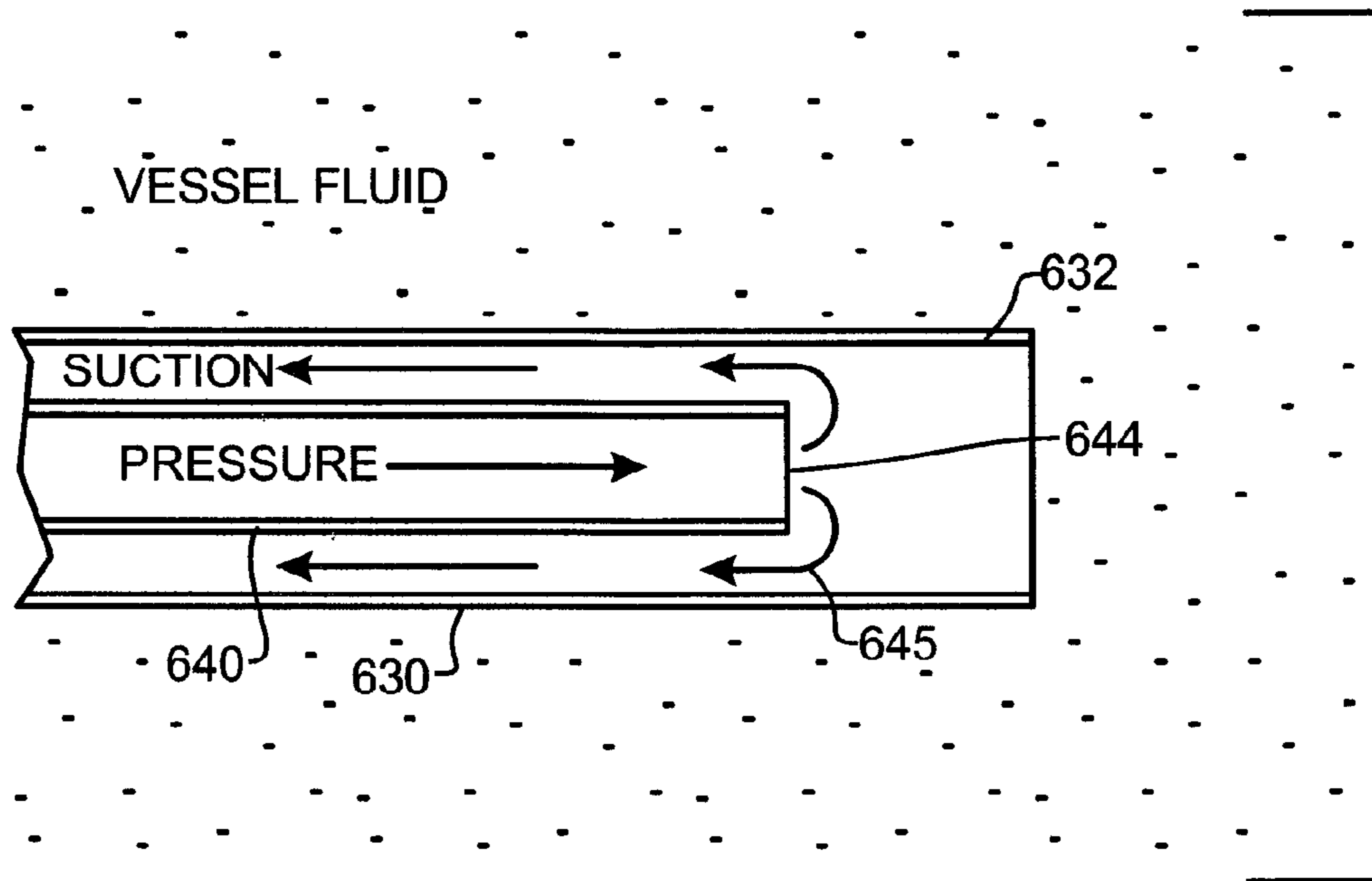
FIG. 11 (PRIOR ART)
