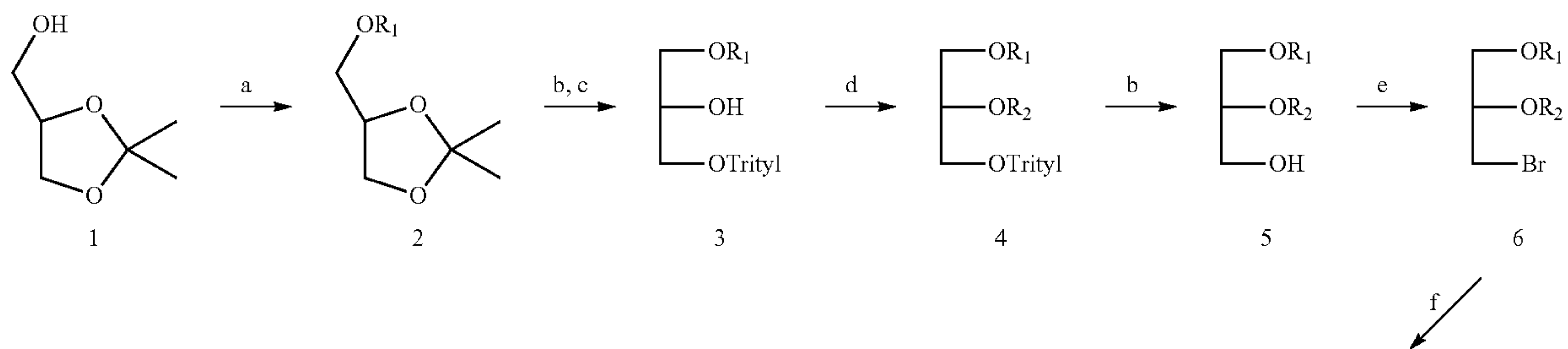
Scheme V
