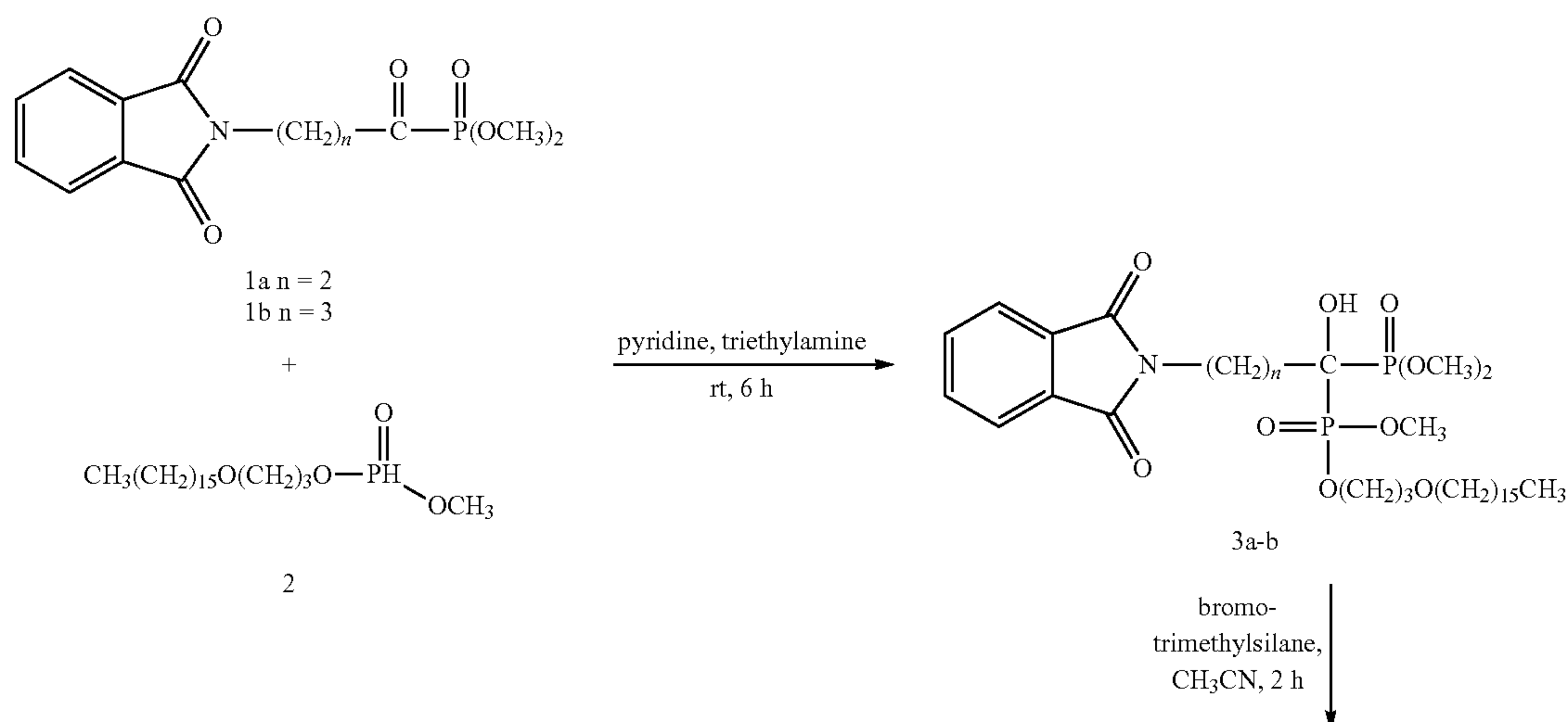
Scheme I
