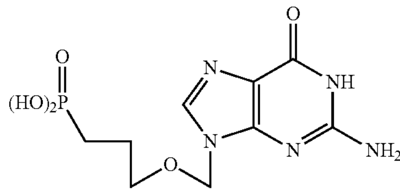
Acyclovir phosphonate
