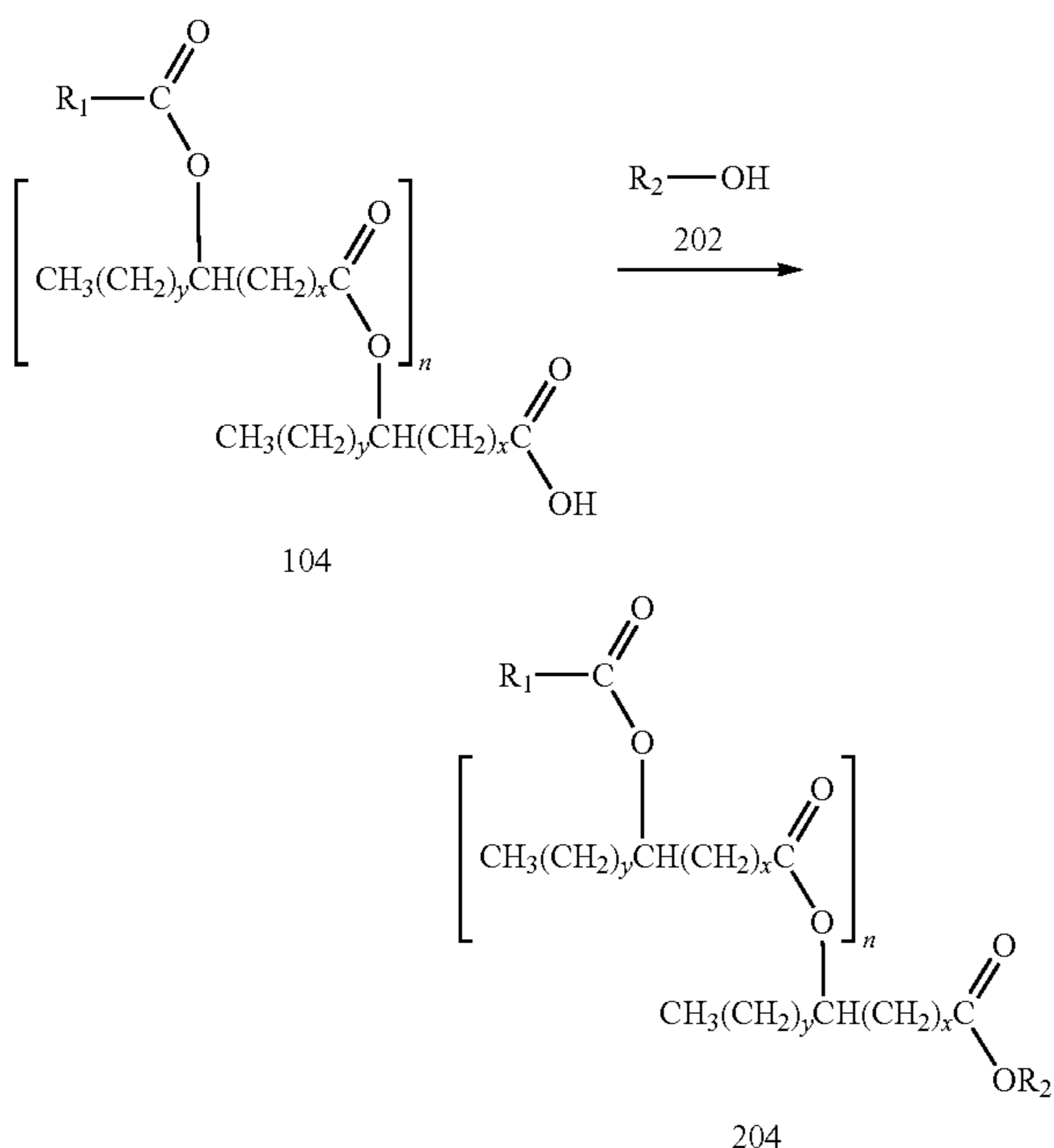
Scheme 2
