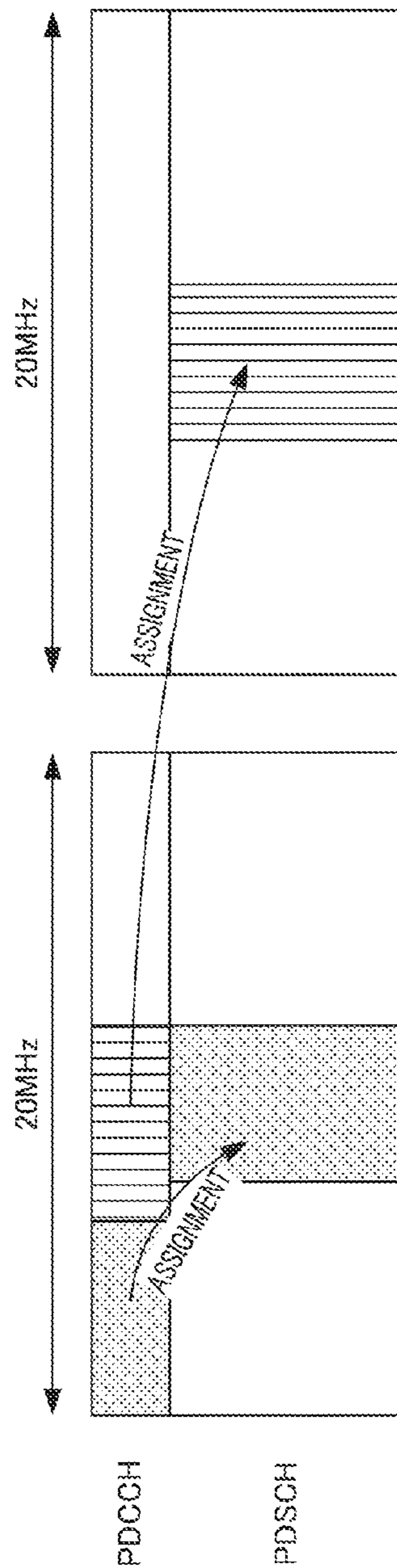
(Cross carrier scheduling) FIG. 3B
