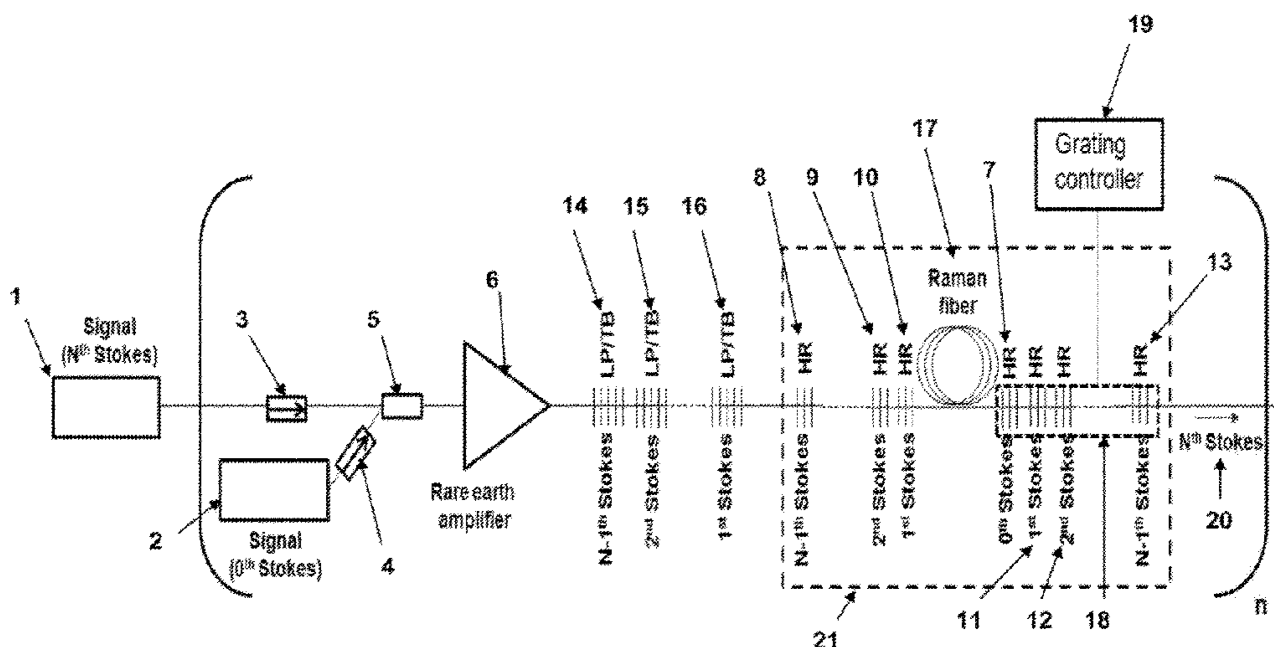
Configuration with Nested Raman Resonators
