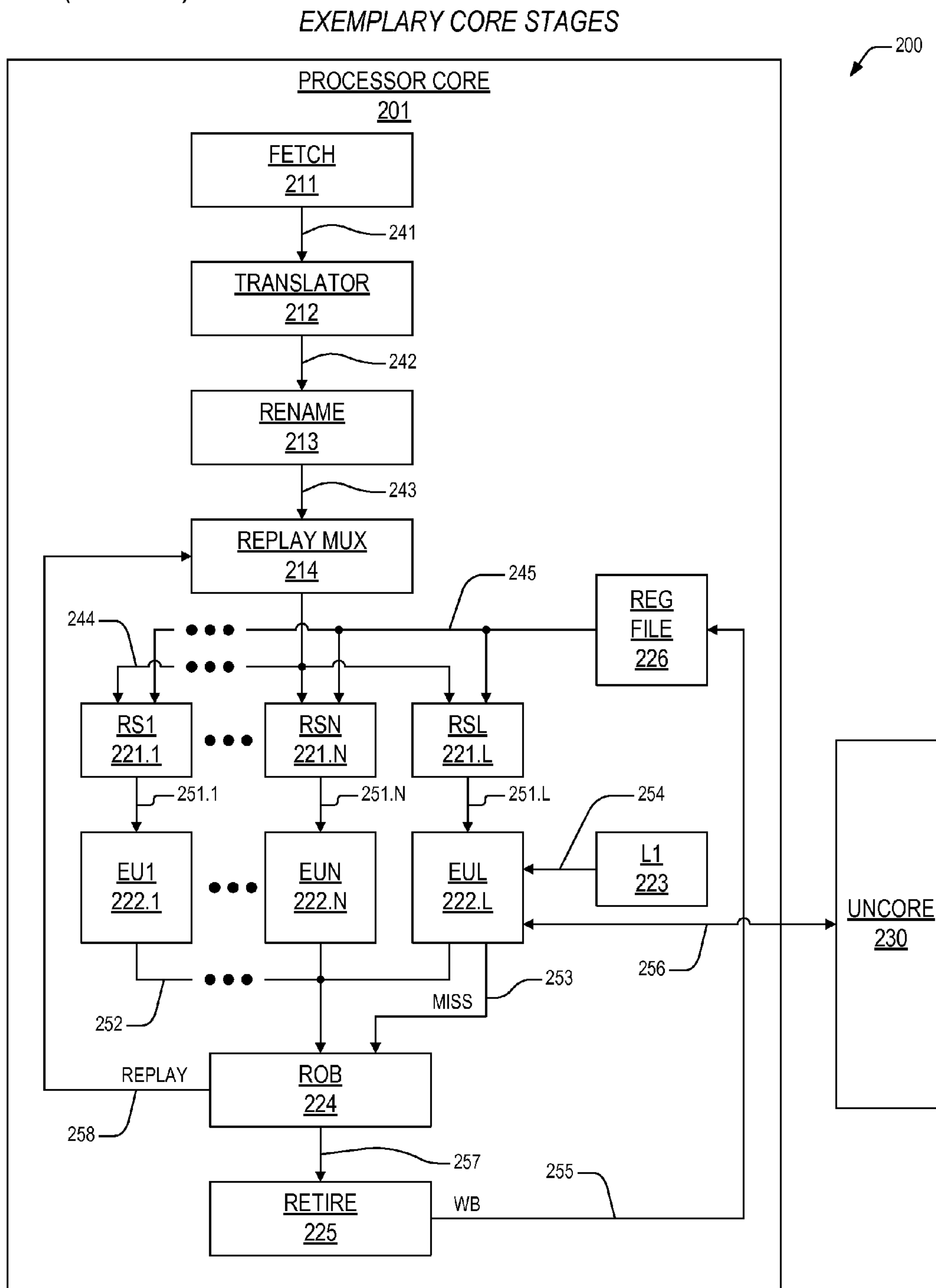
FIG. 2 (Prior Art)
