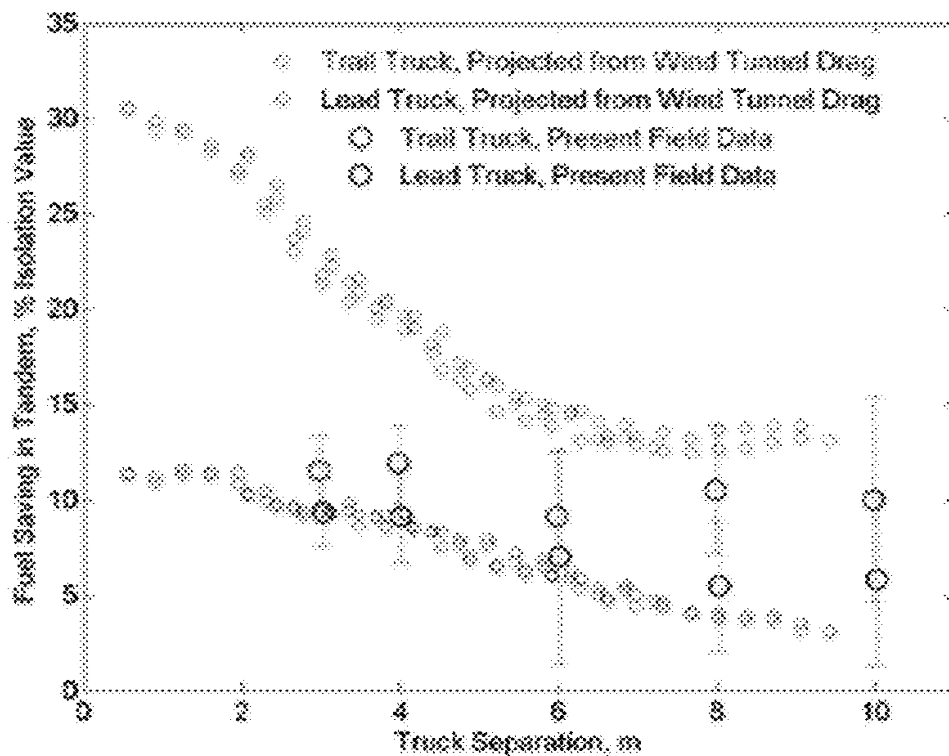
Figure 5: Fuel savings versus vehicle gap (Heavy Trucks)
