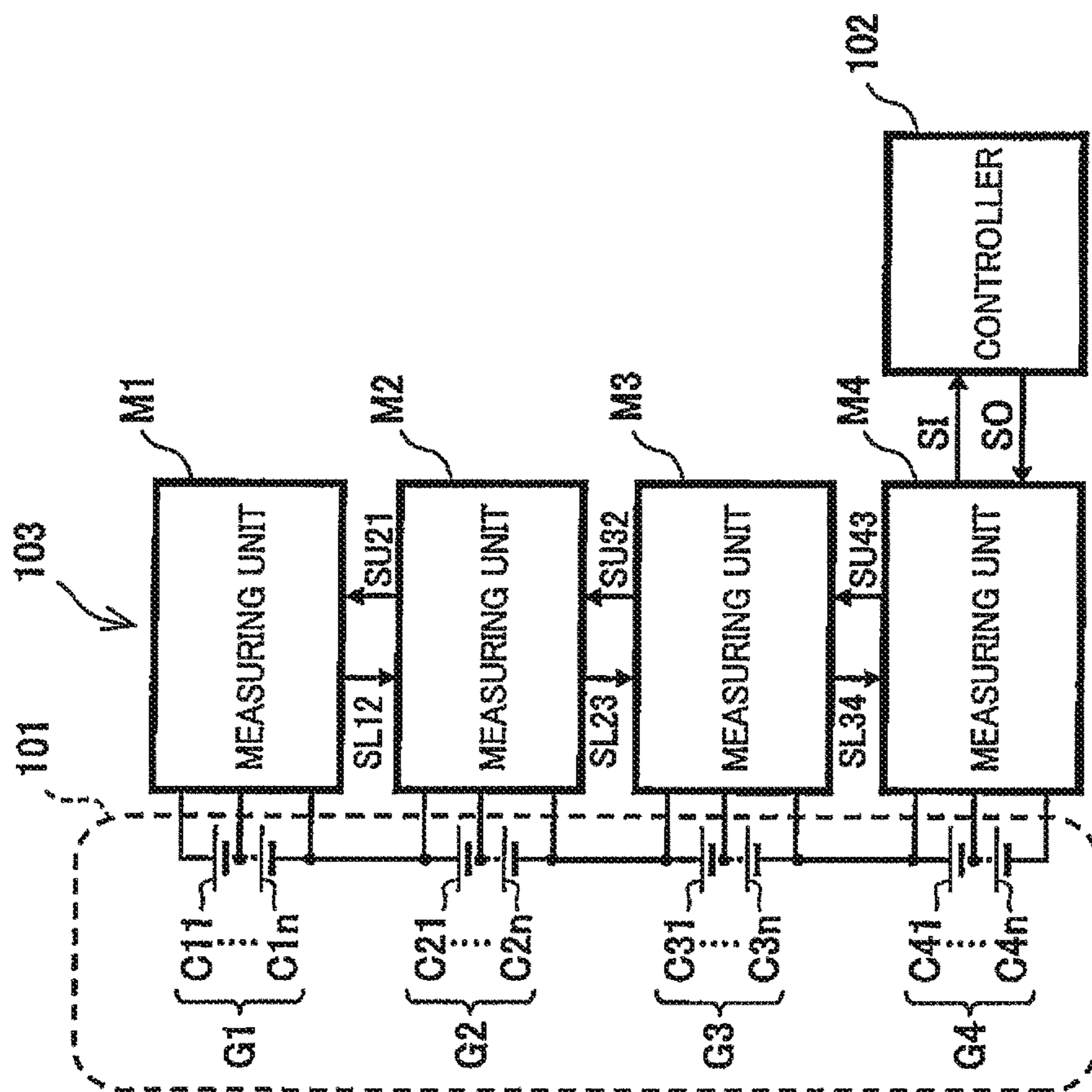
Fig. 5 PRIOR ART
