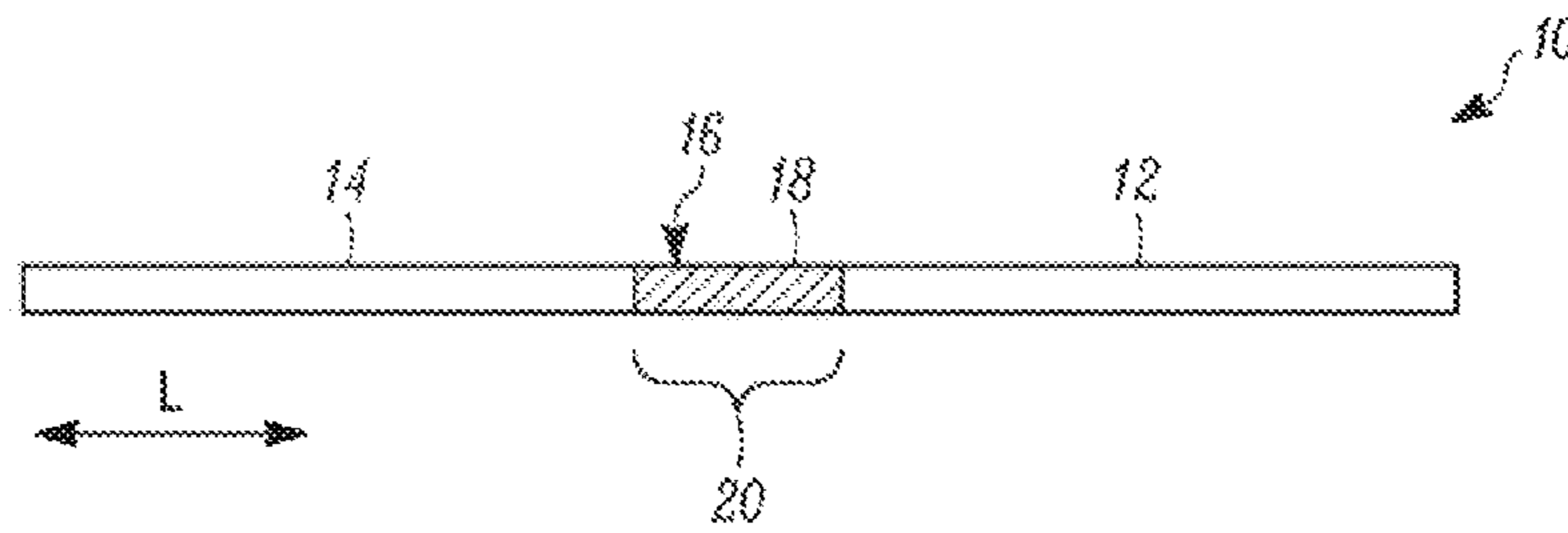
FIG. 1 (PRIOR ART)
