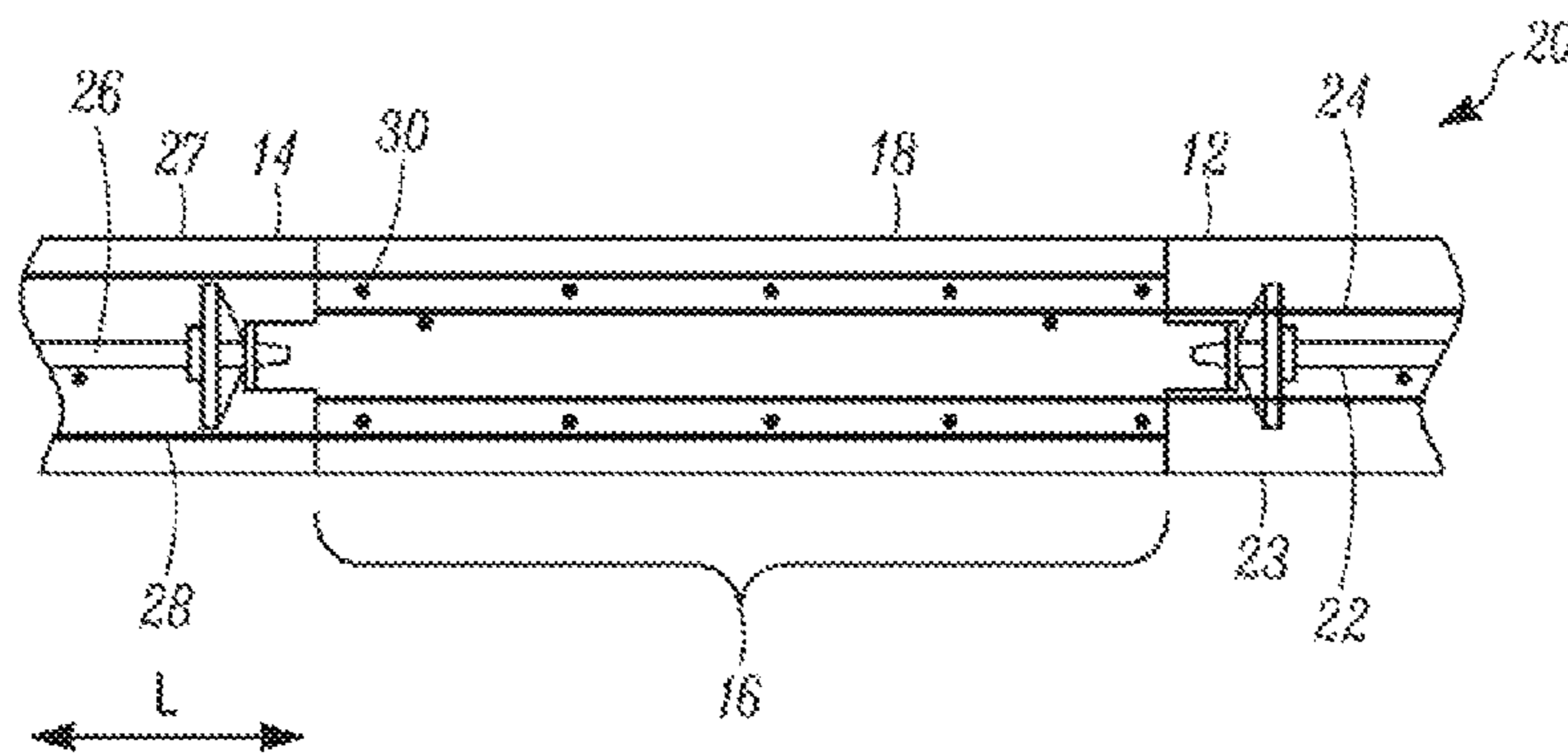
FIG. 3 (PRIOR ART)
