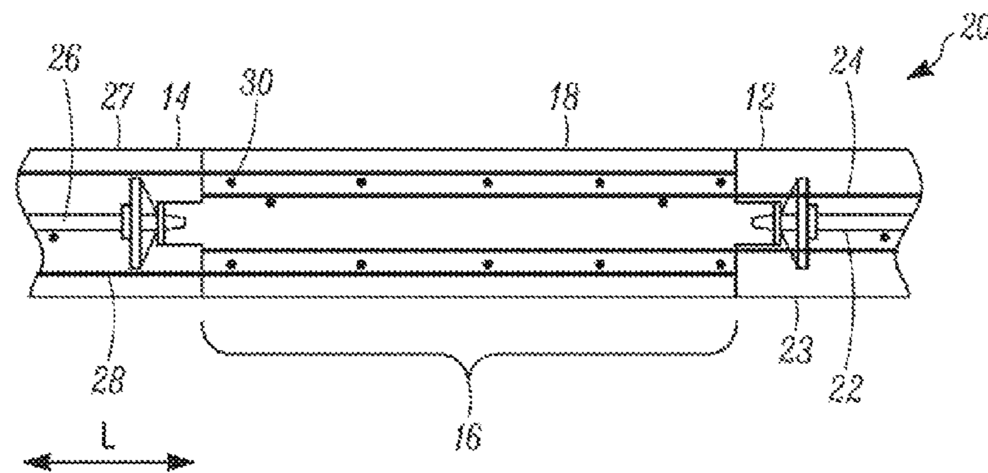
FIG. 3 (PRIOR ART)
