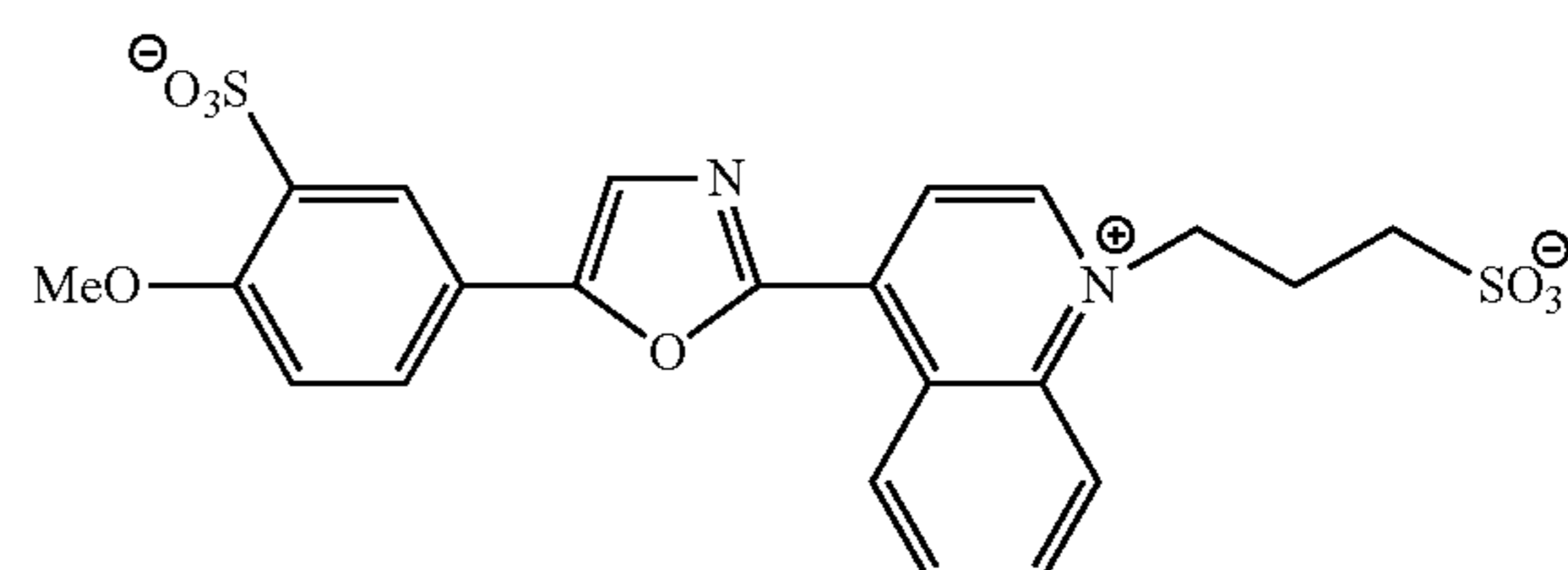
Compound 15
