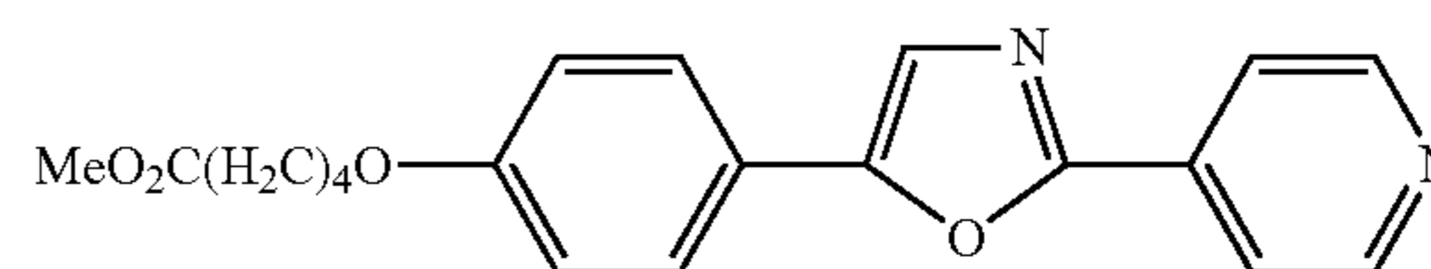
Compound 6
