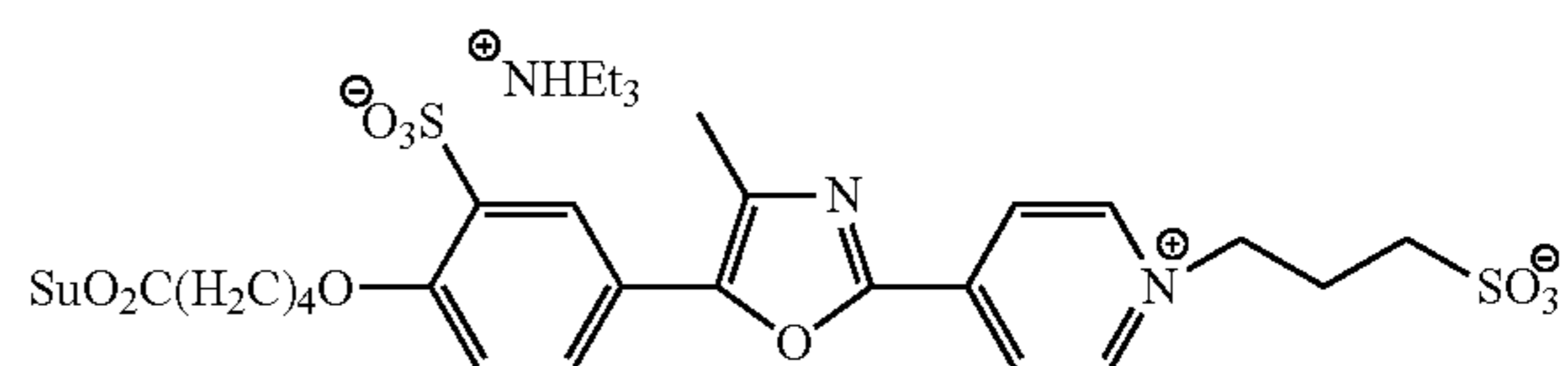
Compound 13
