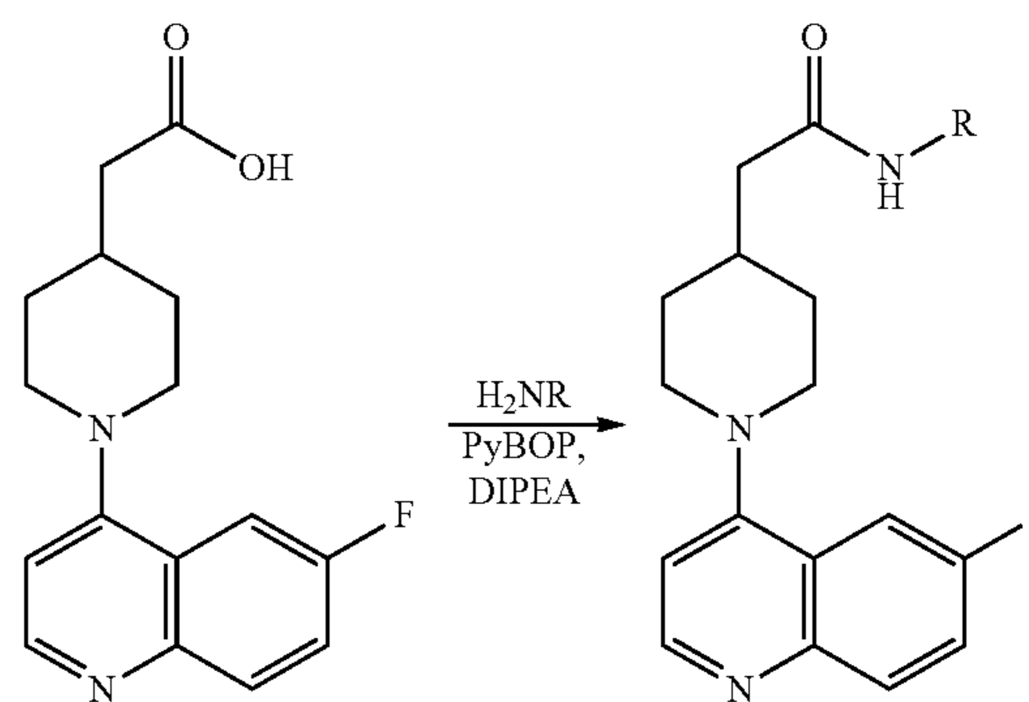
Scheme 3
