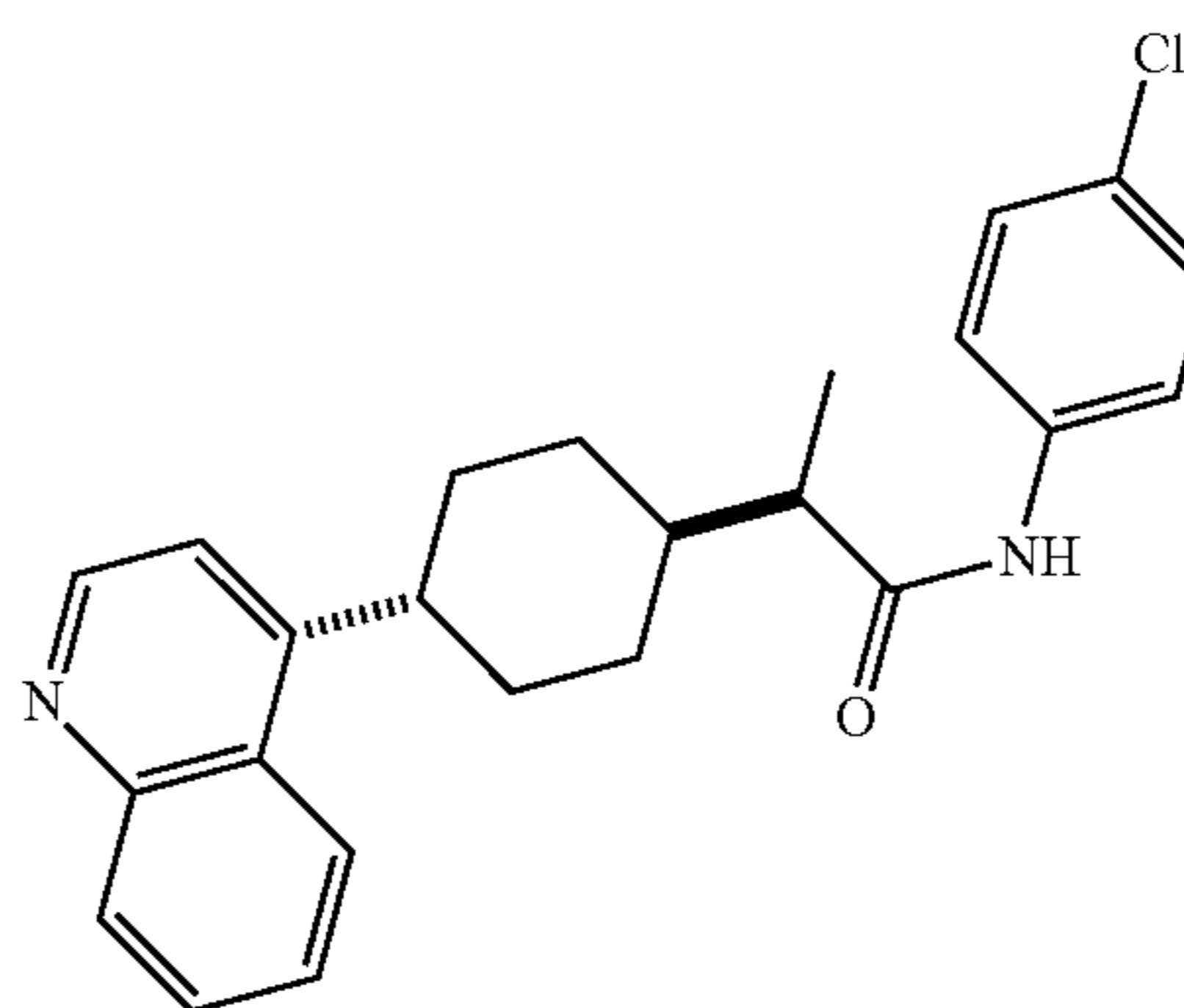
N-(4-chlorophenyl)-2-(cis-4-(quinolin-4-yl)cyclohexyl)propanamide
