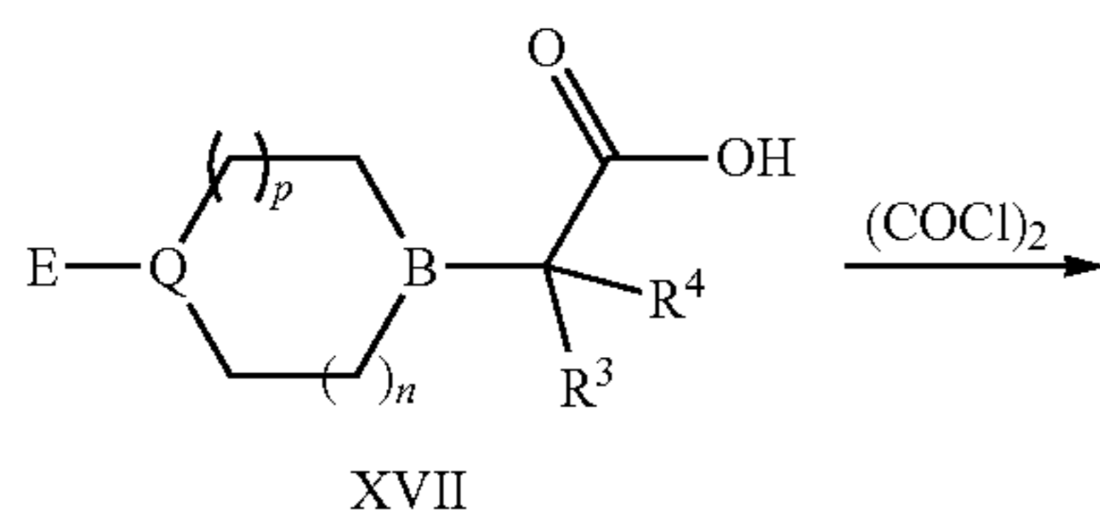
Scheme 4
