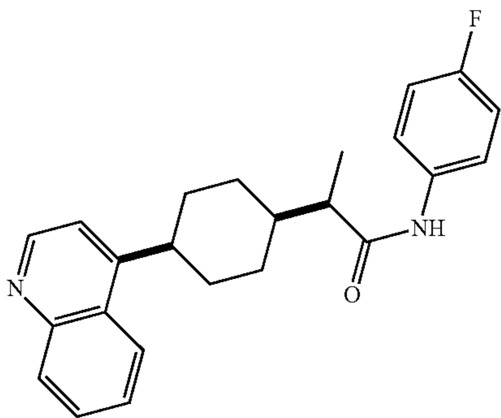
Intermediate 16A
