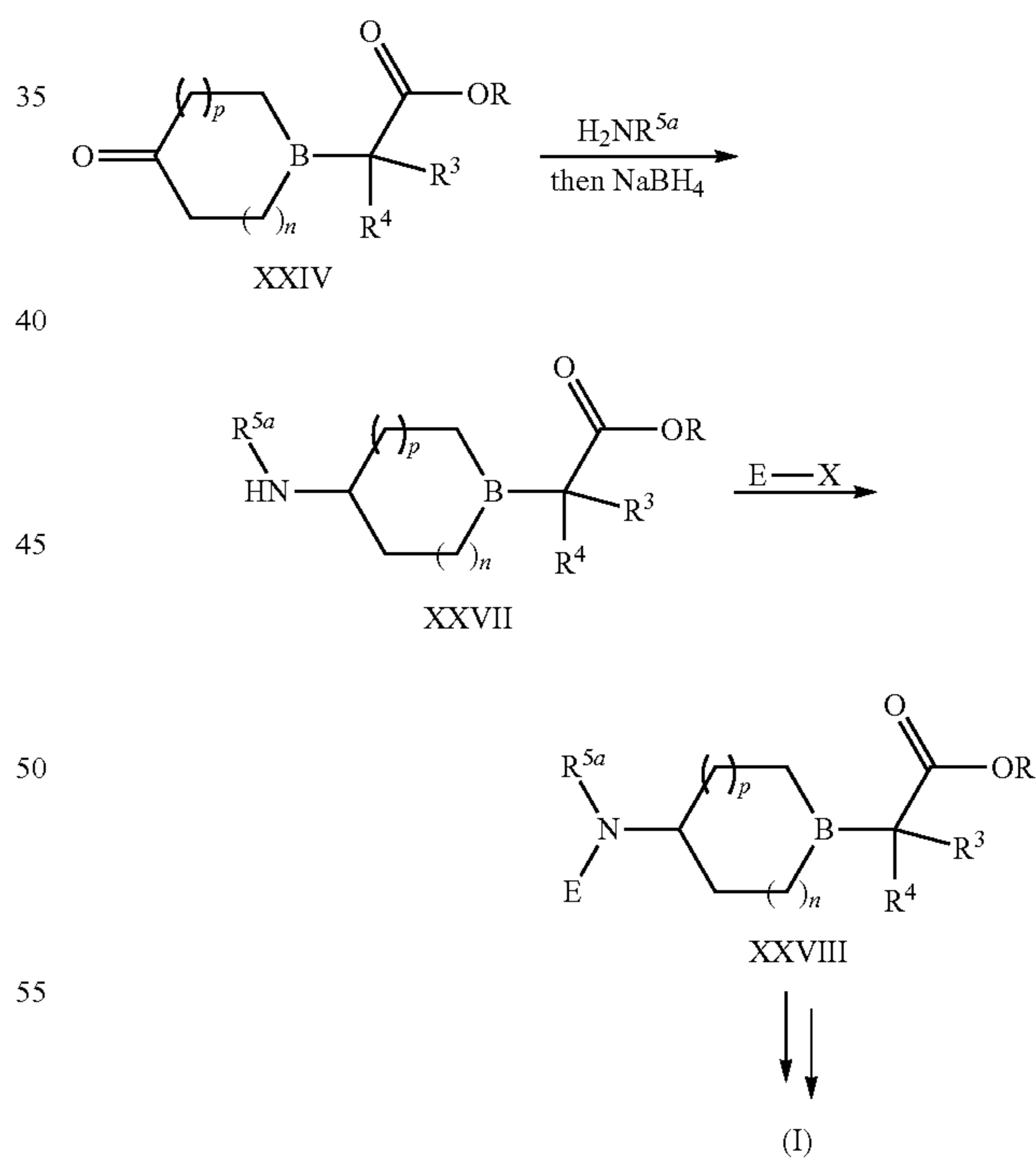
Scheme 7
