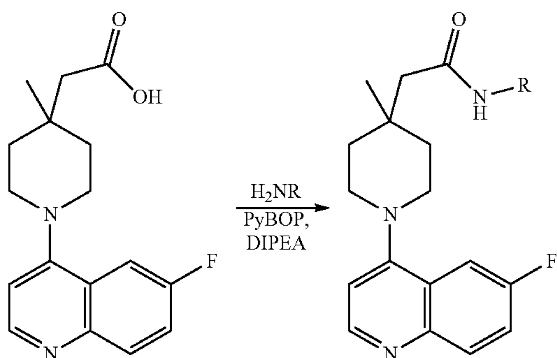
Scheme 4
