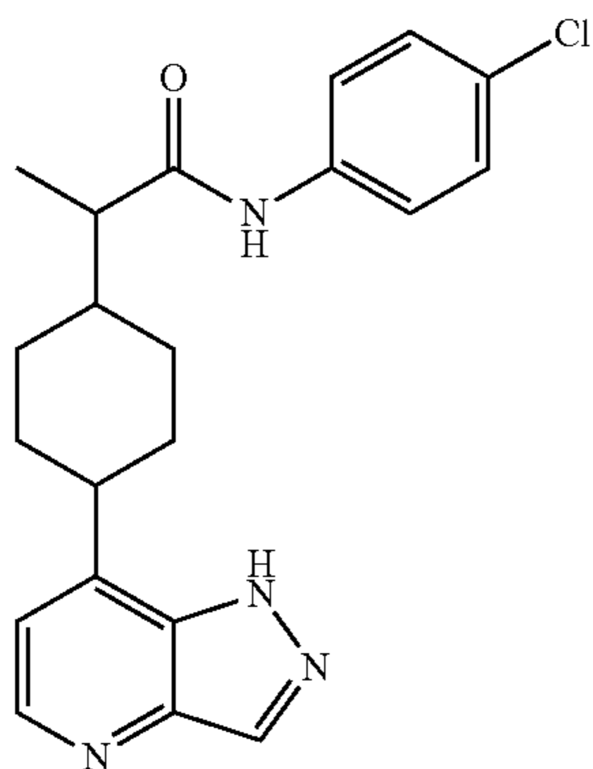
Intermediate 149A
