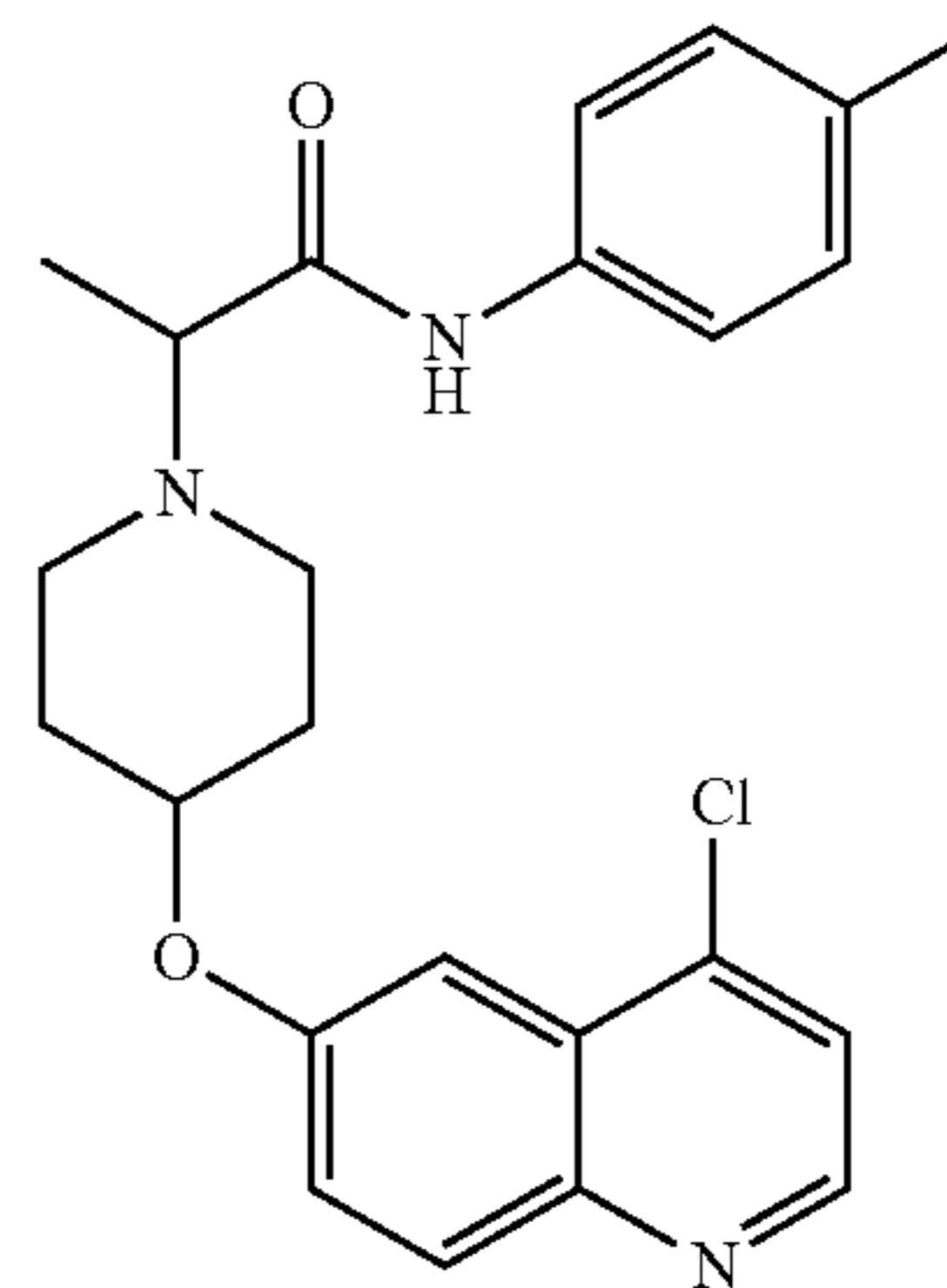
Example 92
