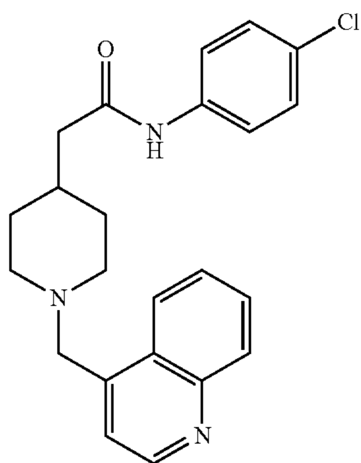
Intermediate 113A
