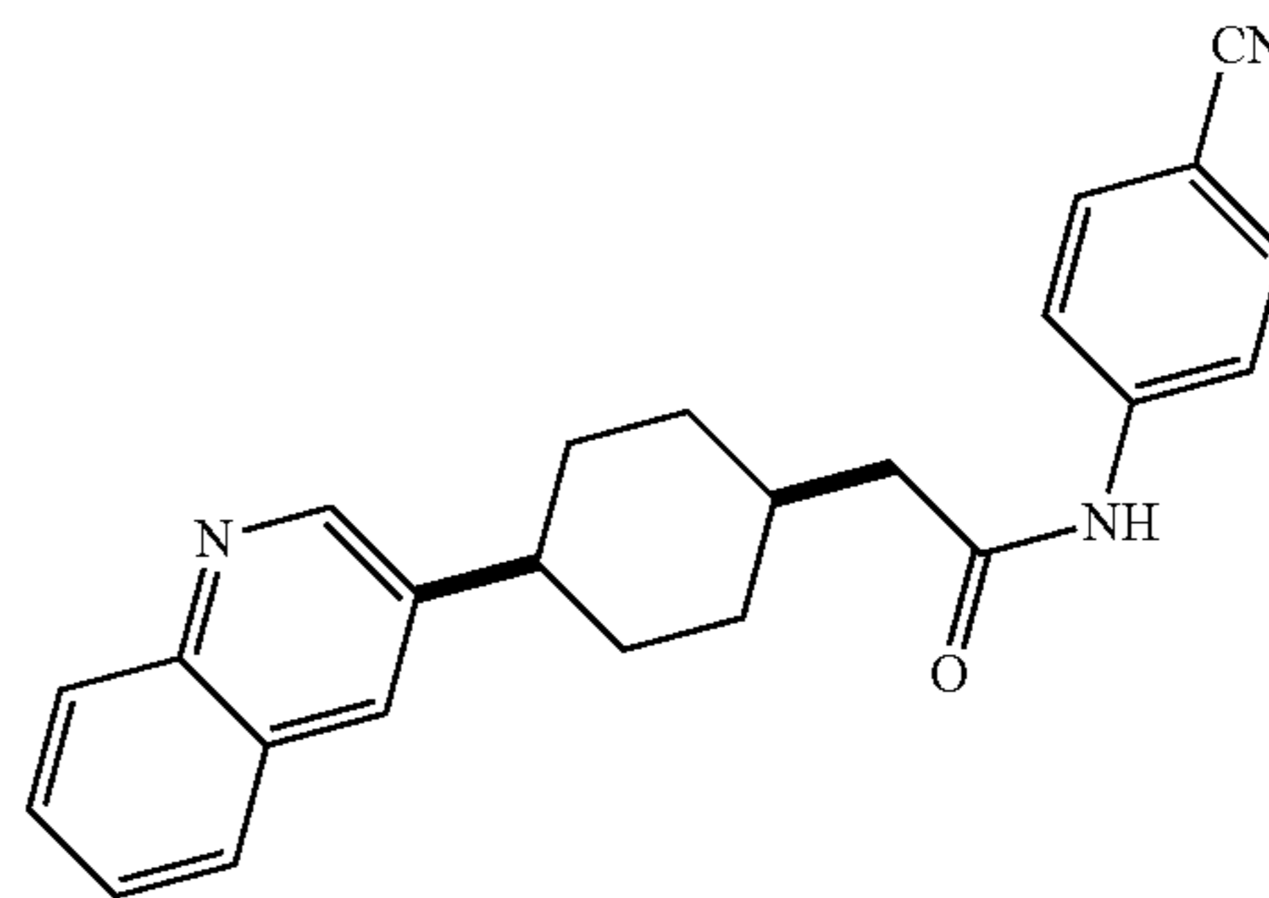
N-(4-cyanophenyl)-2-(trans-4-(quinolin-3-yl)cyclohexyl)acetamide
