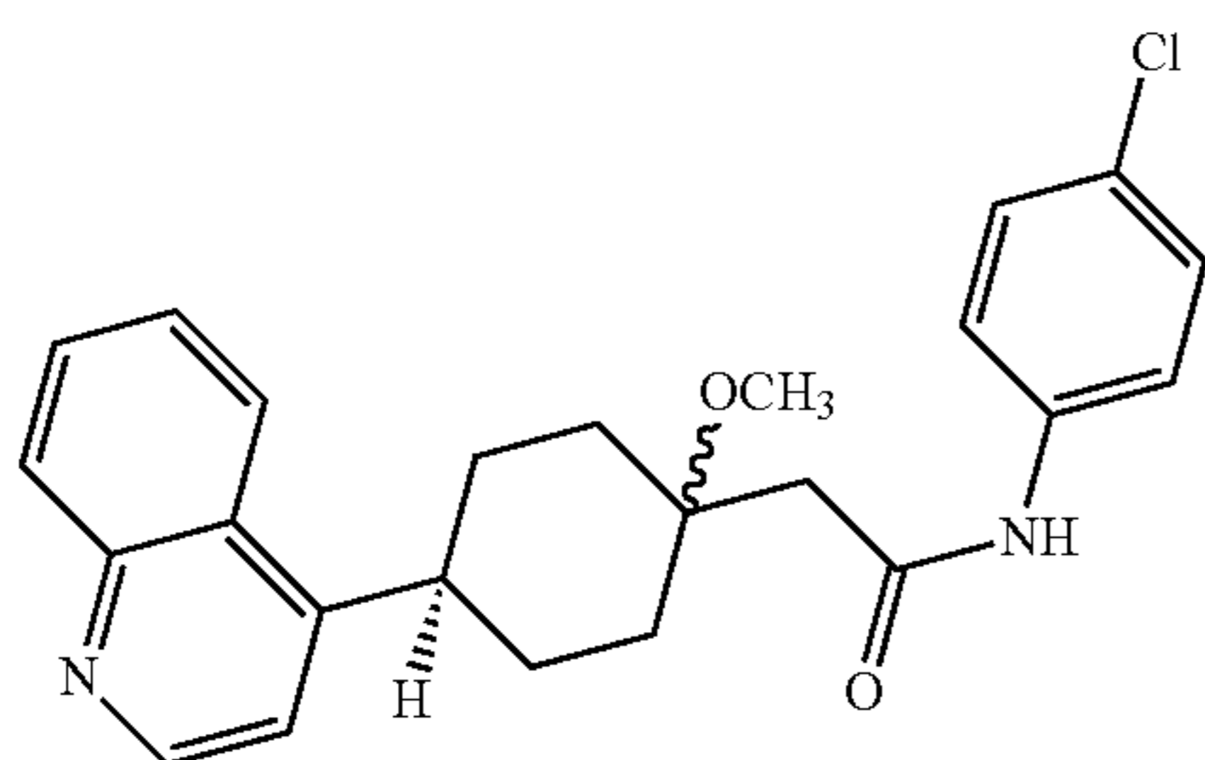
Intermediate 158A
