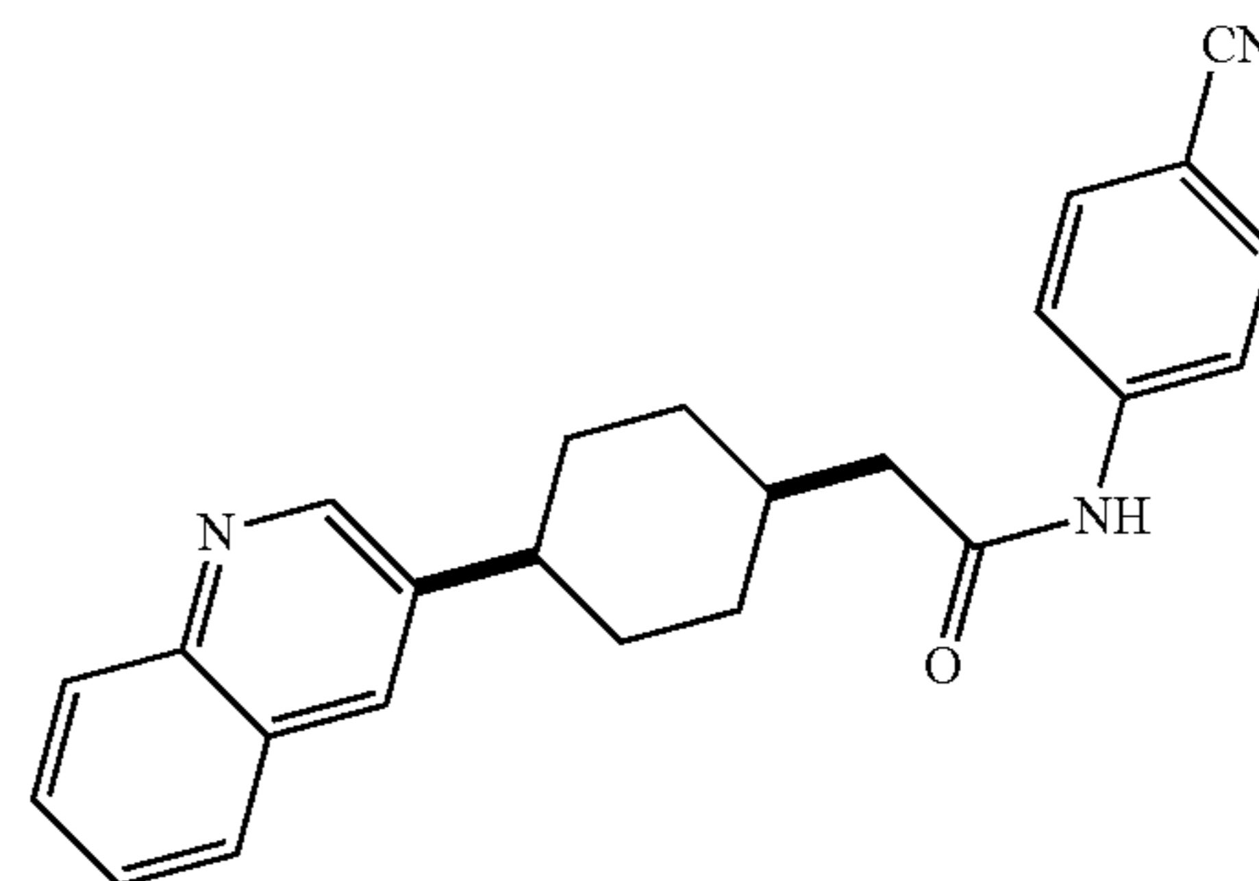
N-(4-cyanophenyl)-2-(trans-4-(quinolin-3-yl)cyclohexyl)acetamide
