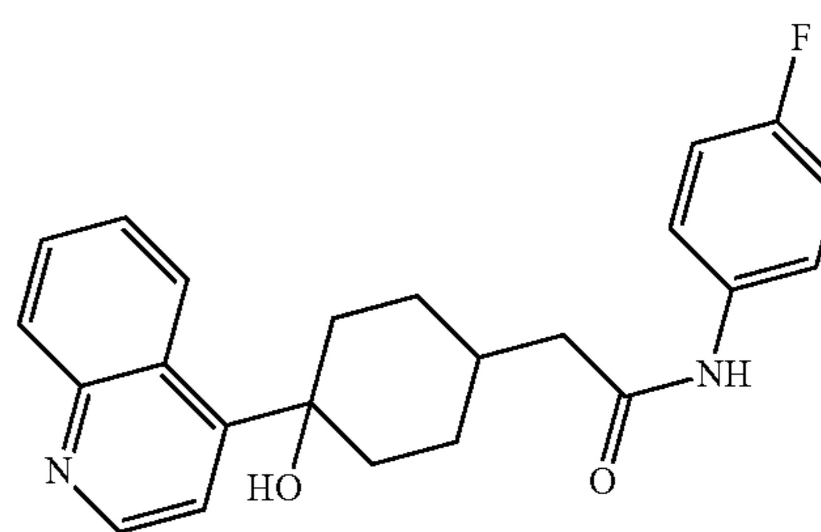
Intermediate 159A
