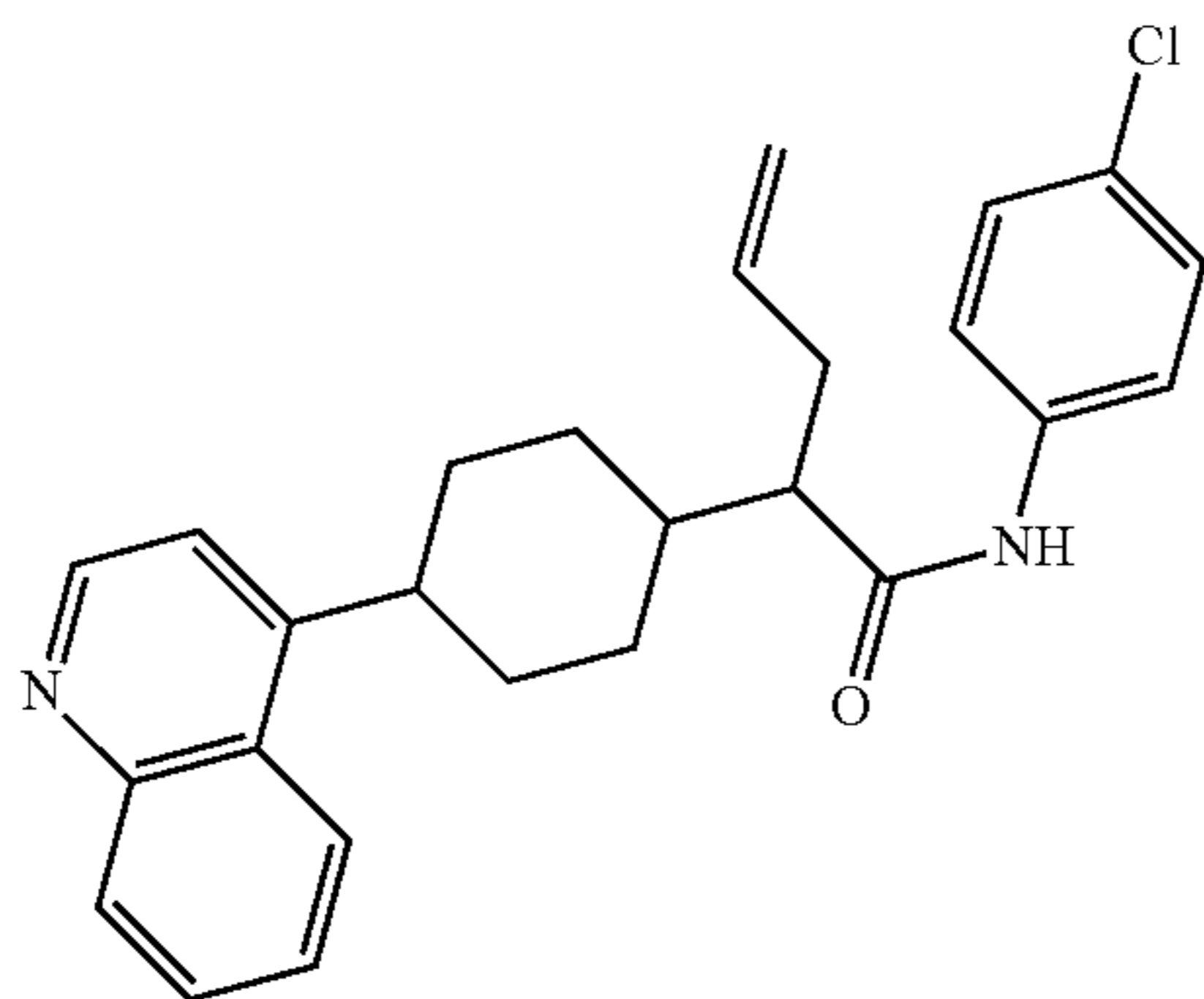
Intermediate 42A
