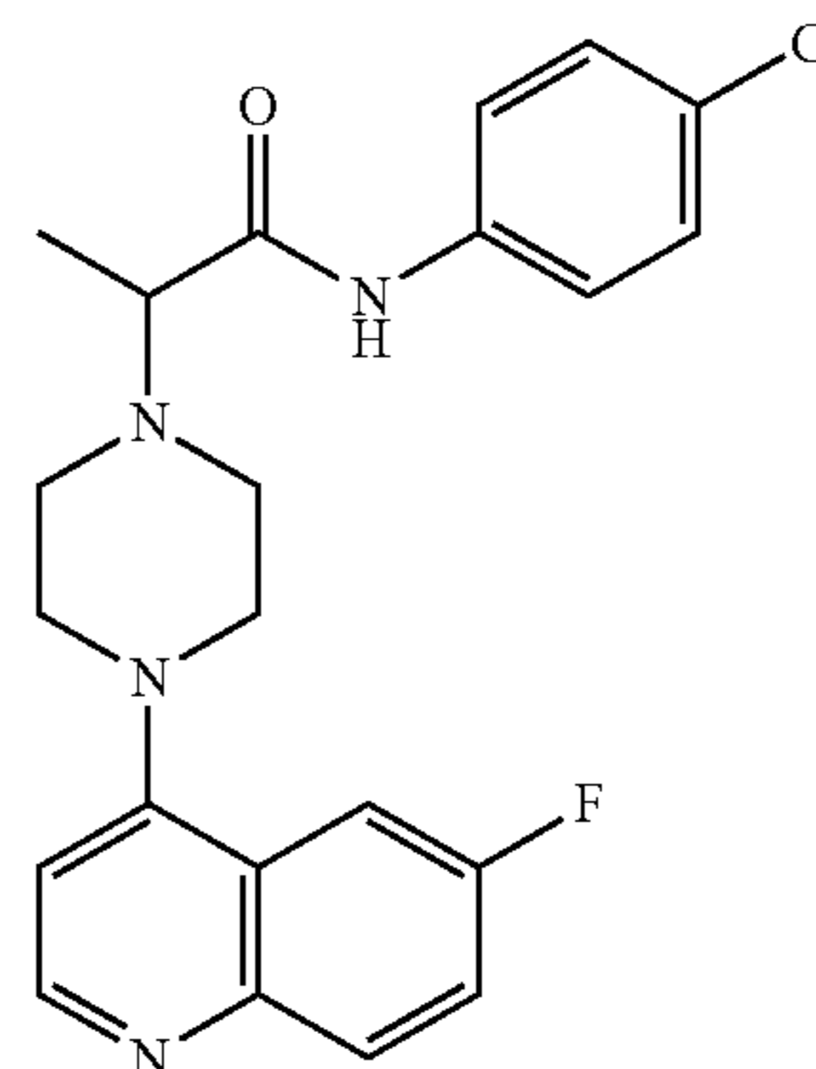
Intermediate 126A
