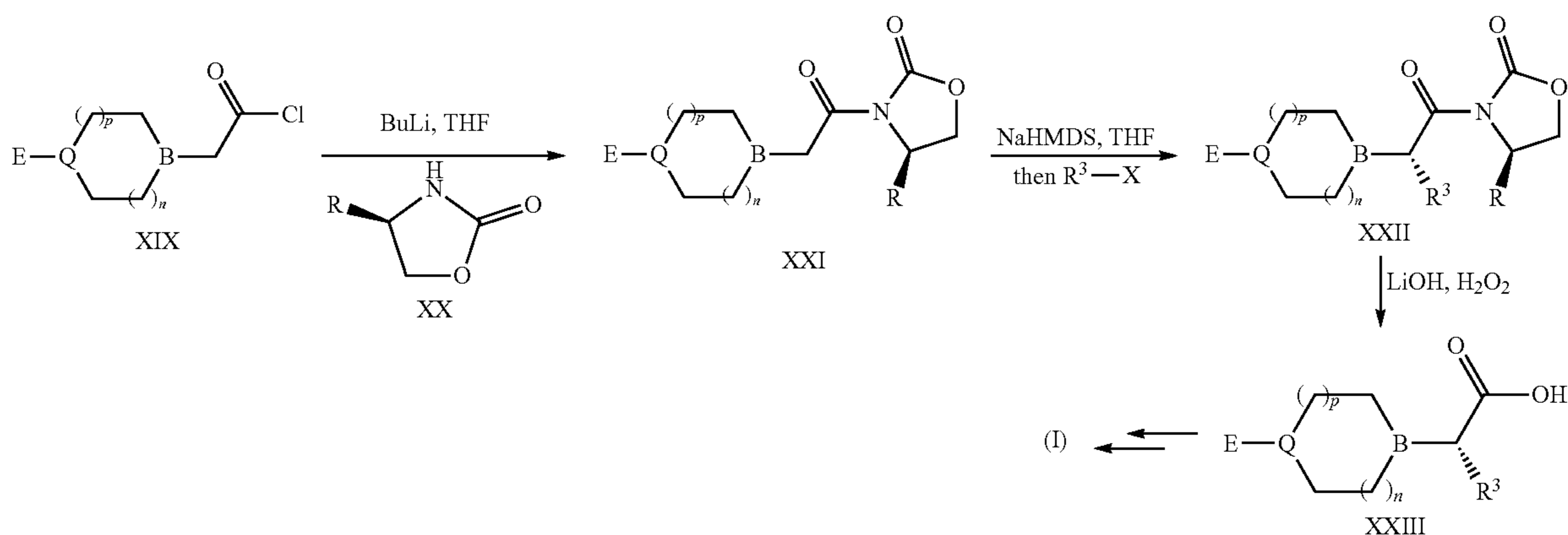
Scheme 5
