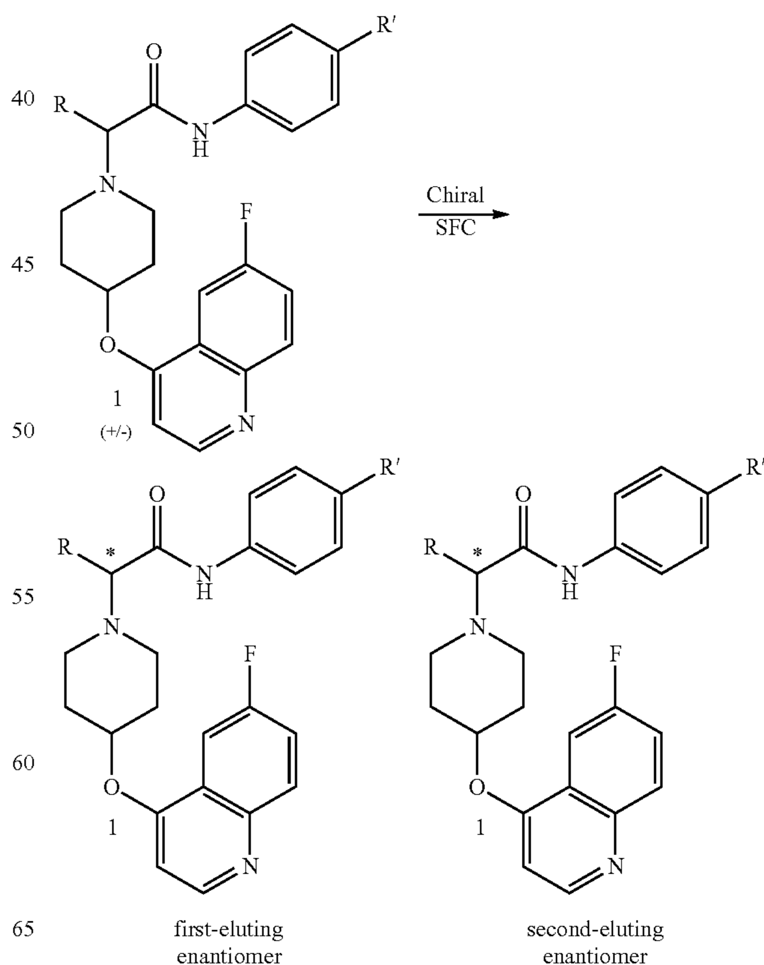
Scheme 2
