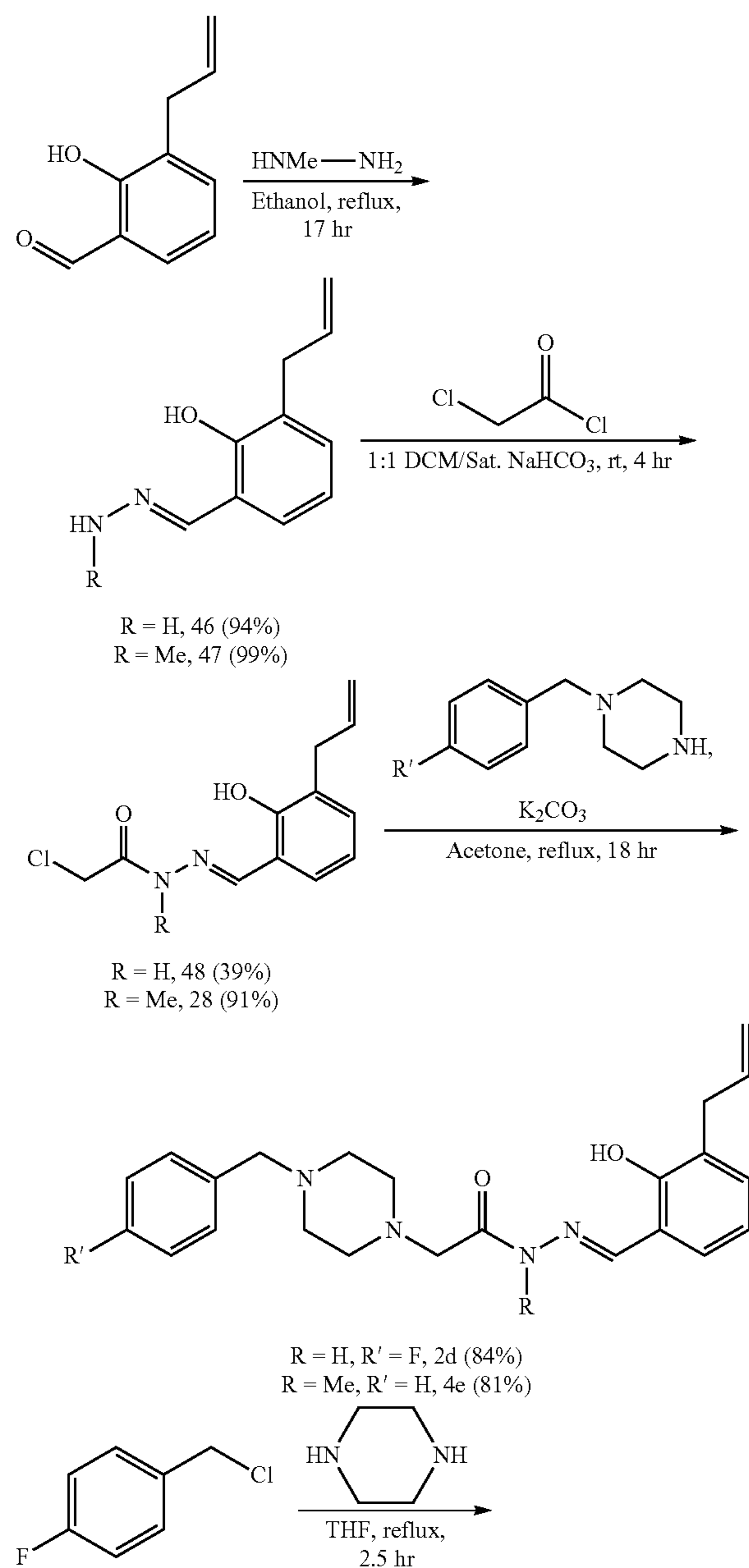
Scheme S5. Syntheses of 2d and 4e
