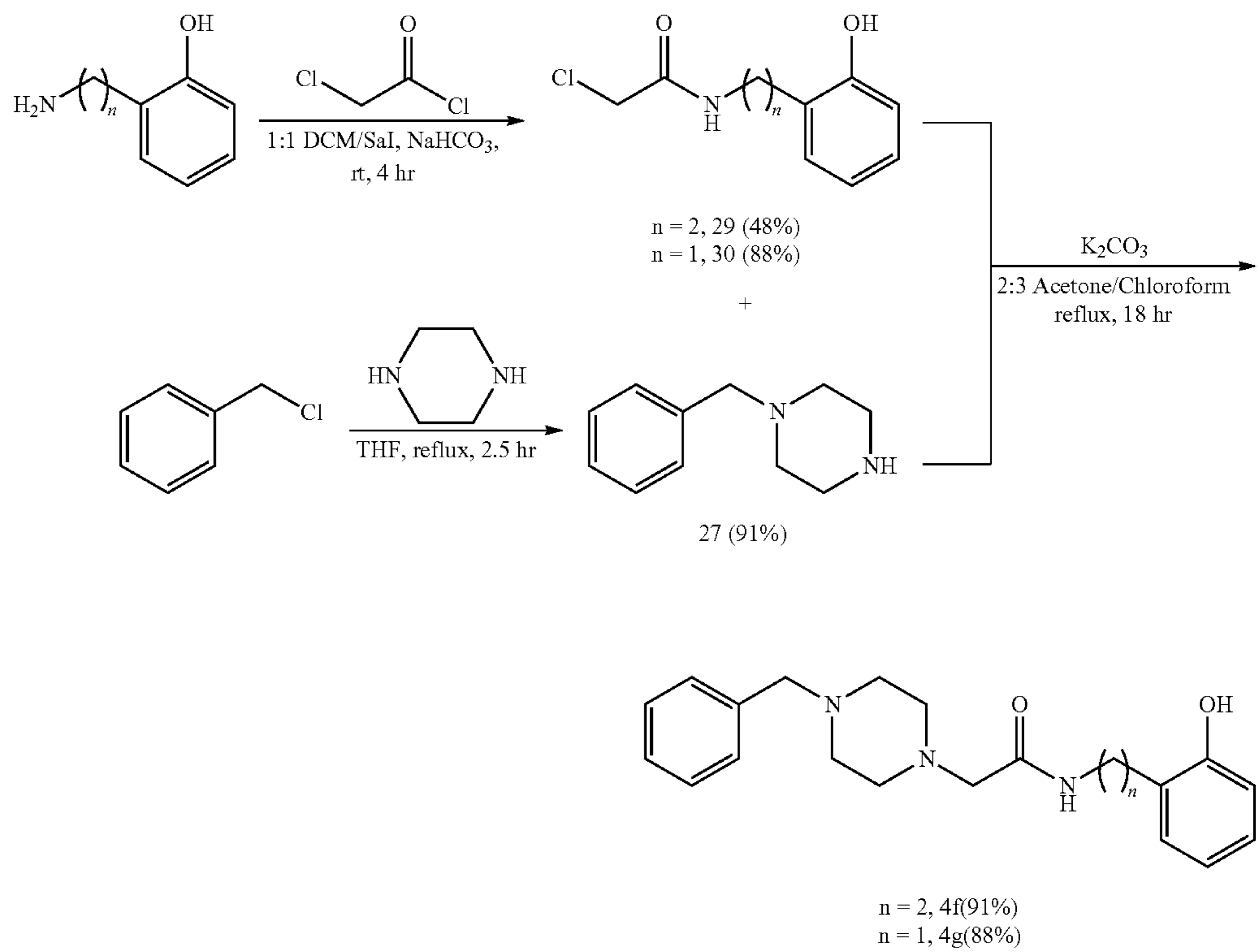
Scheme S4. Syntheses of 4f-g
