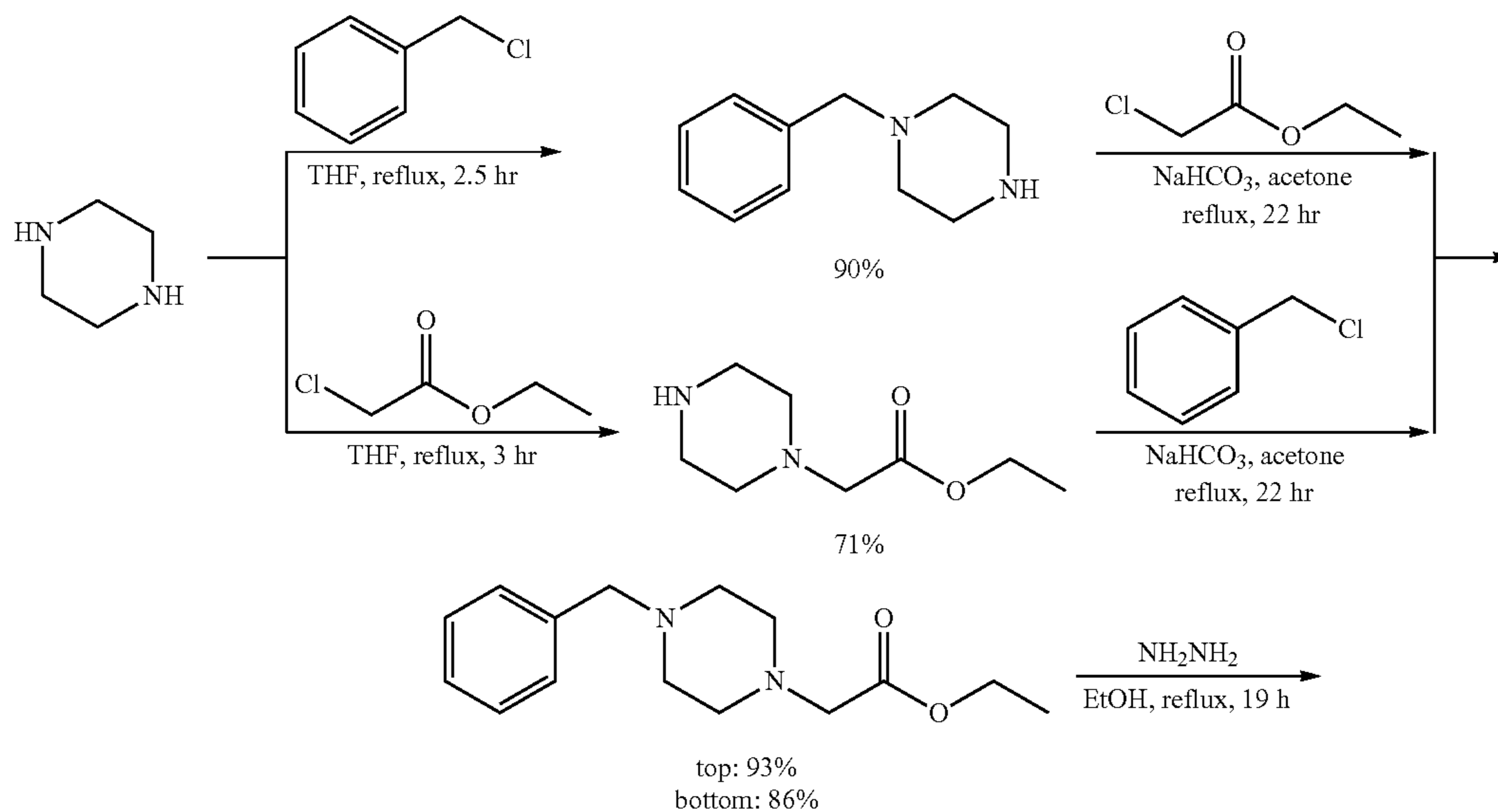
Scheme 3. Synthesis of PAC-1
