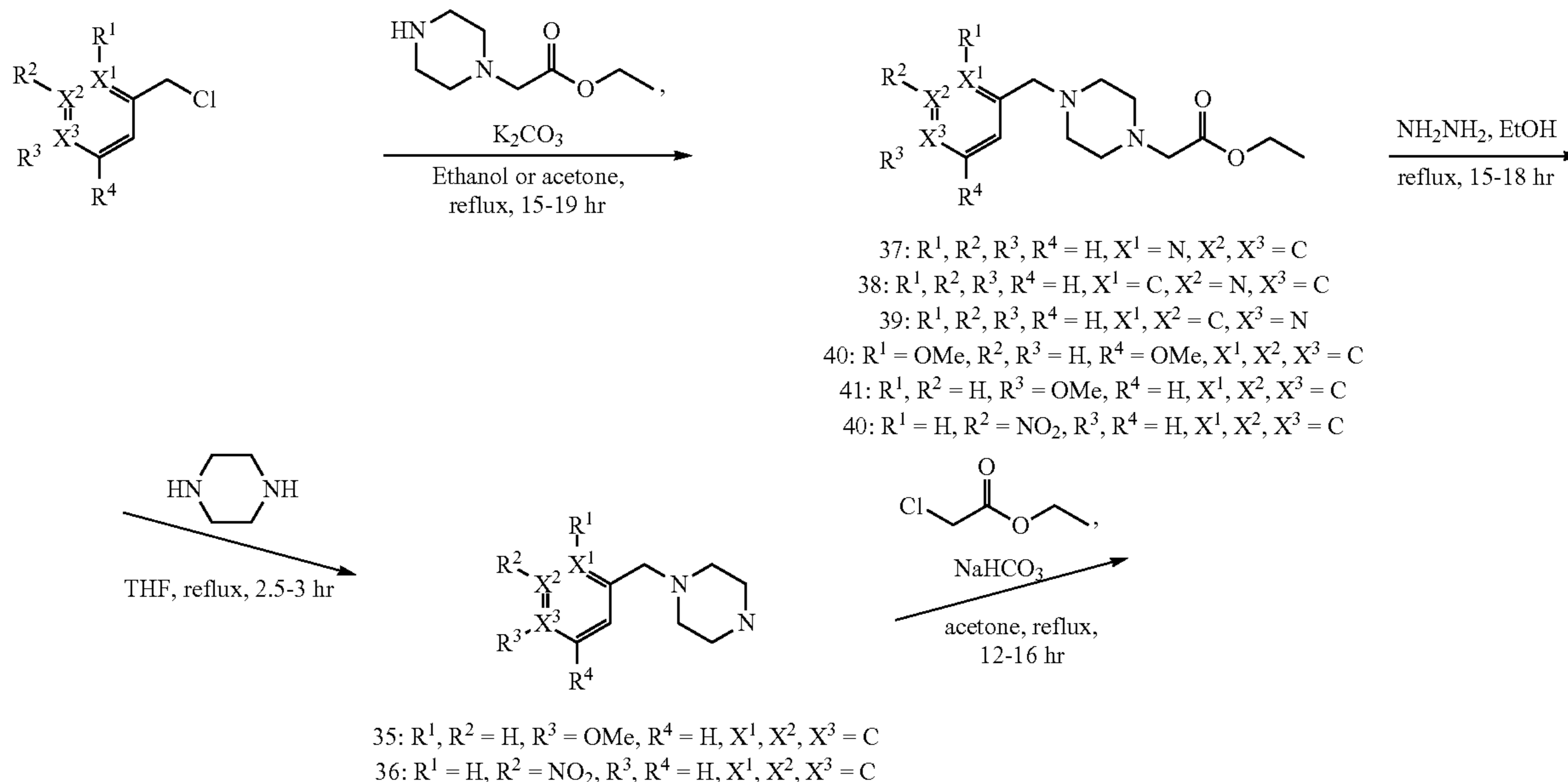
Scheme S1. Syntheses of PAC-1 derivatives
