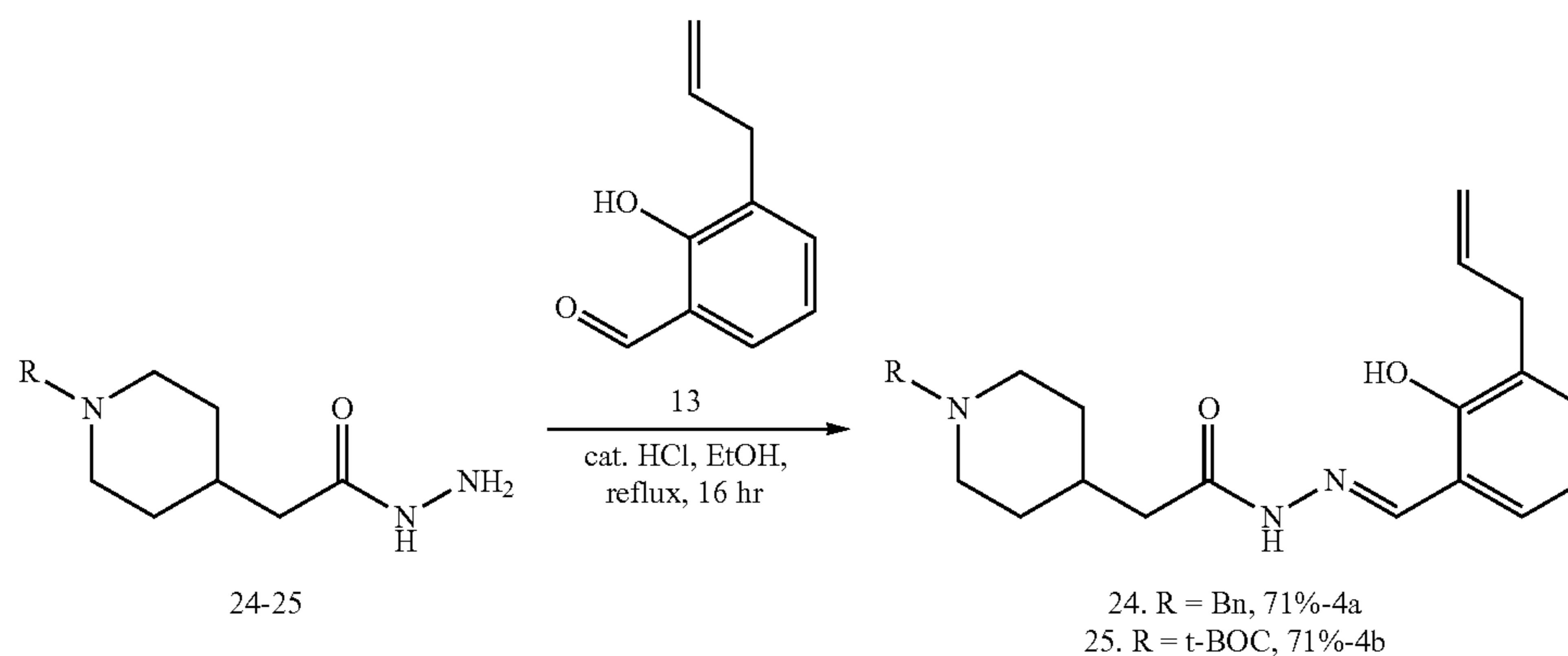
Scheme 4A.
