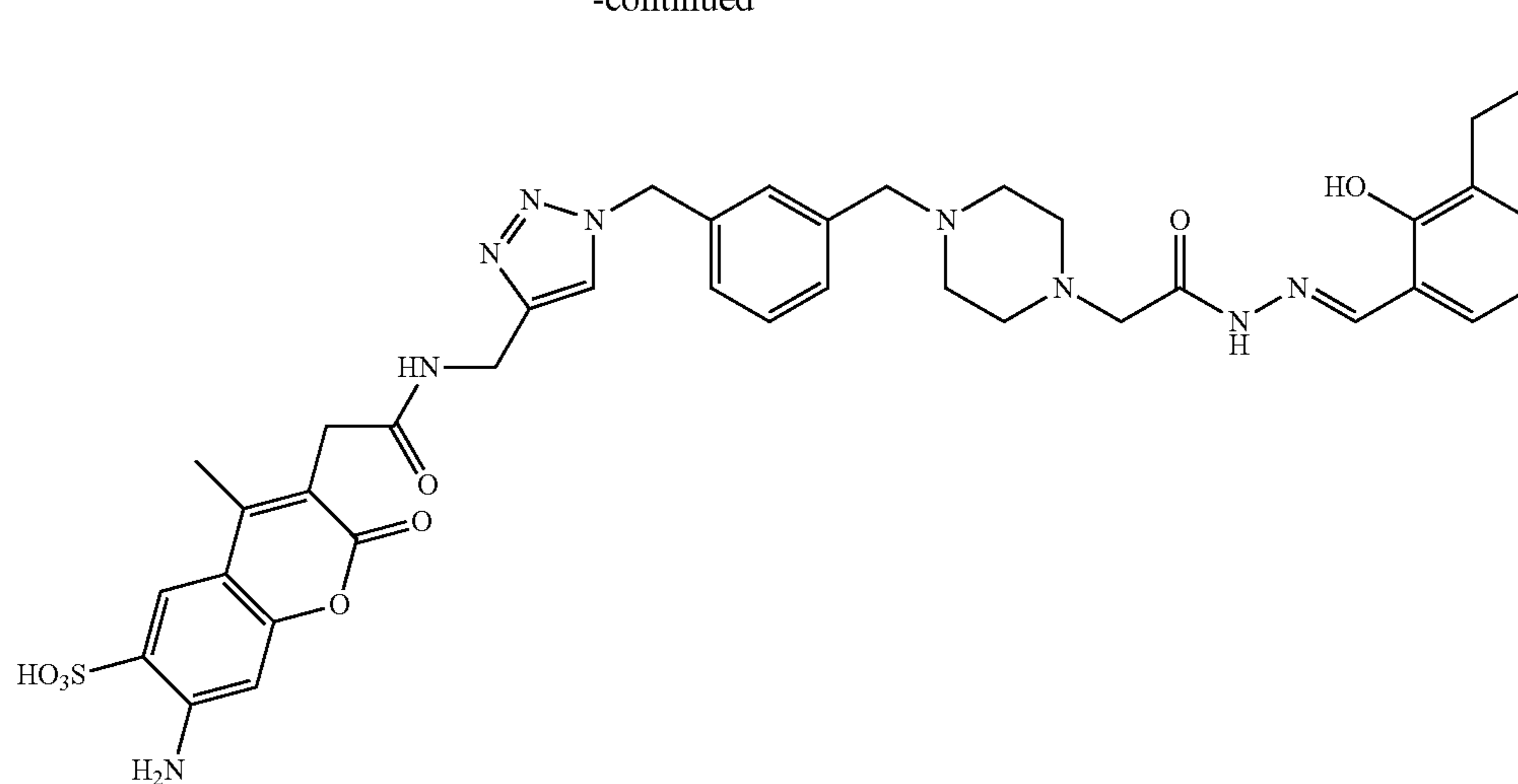
Alexa Fluor 350-linked PAC-1 25% (2 Steps) IC_{50} : 10.7 \mu M (AF-PAC-1)
