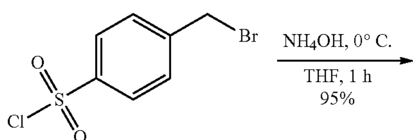
Scheme 7. Minigram-scale synthesis of S-PAC-1.
