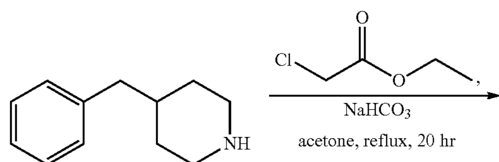
Scheme S2. Synthesis of 4c
