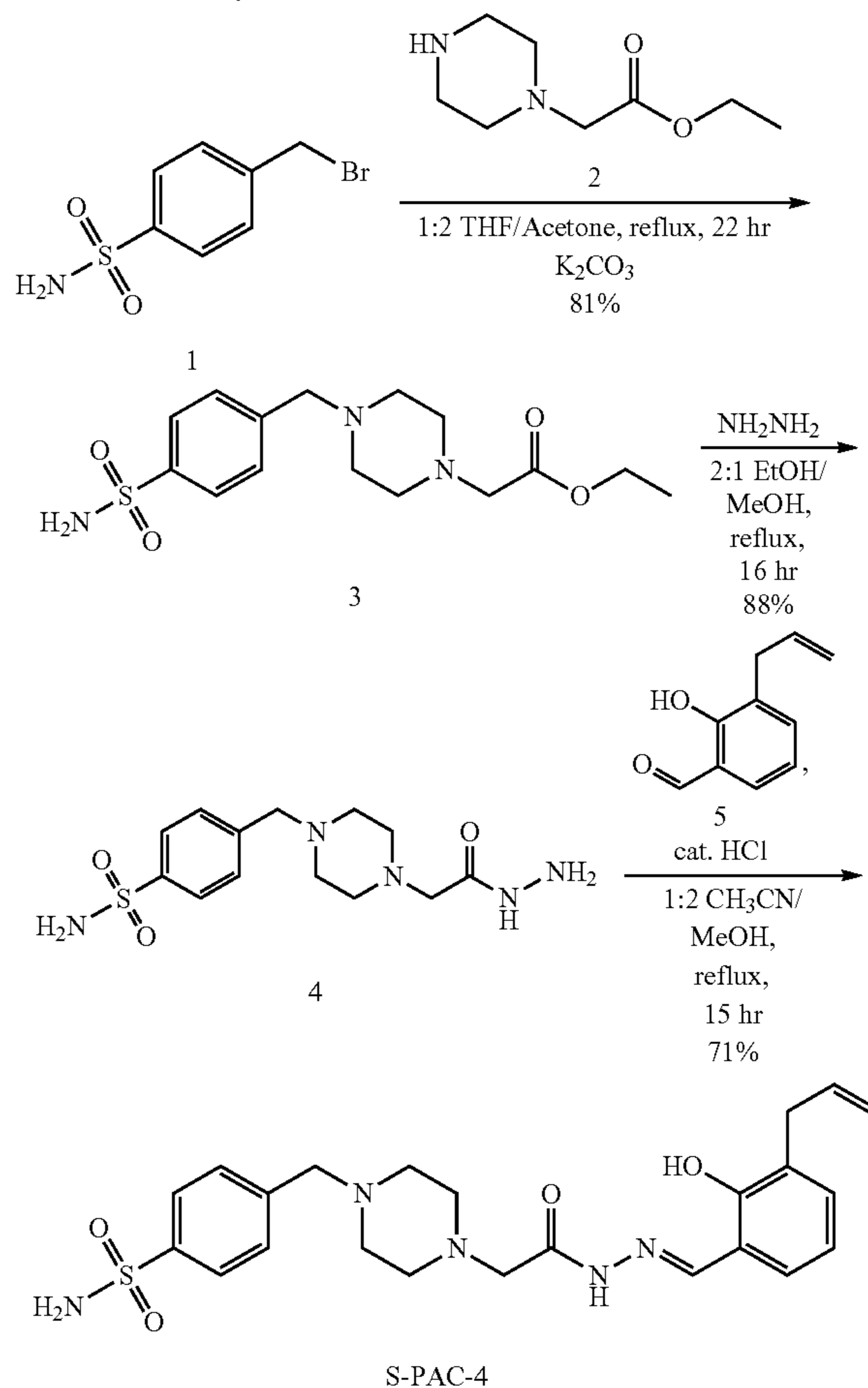
Scheme 1
