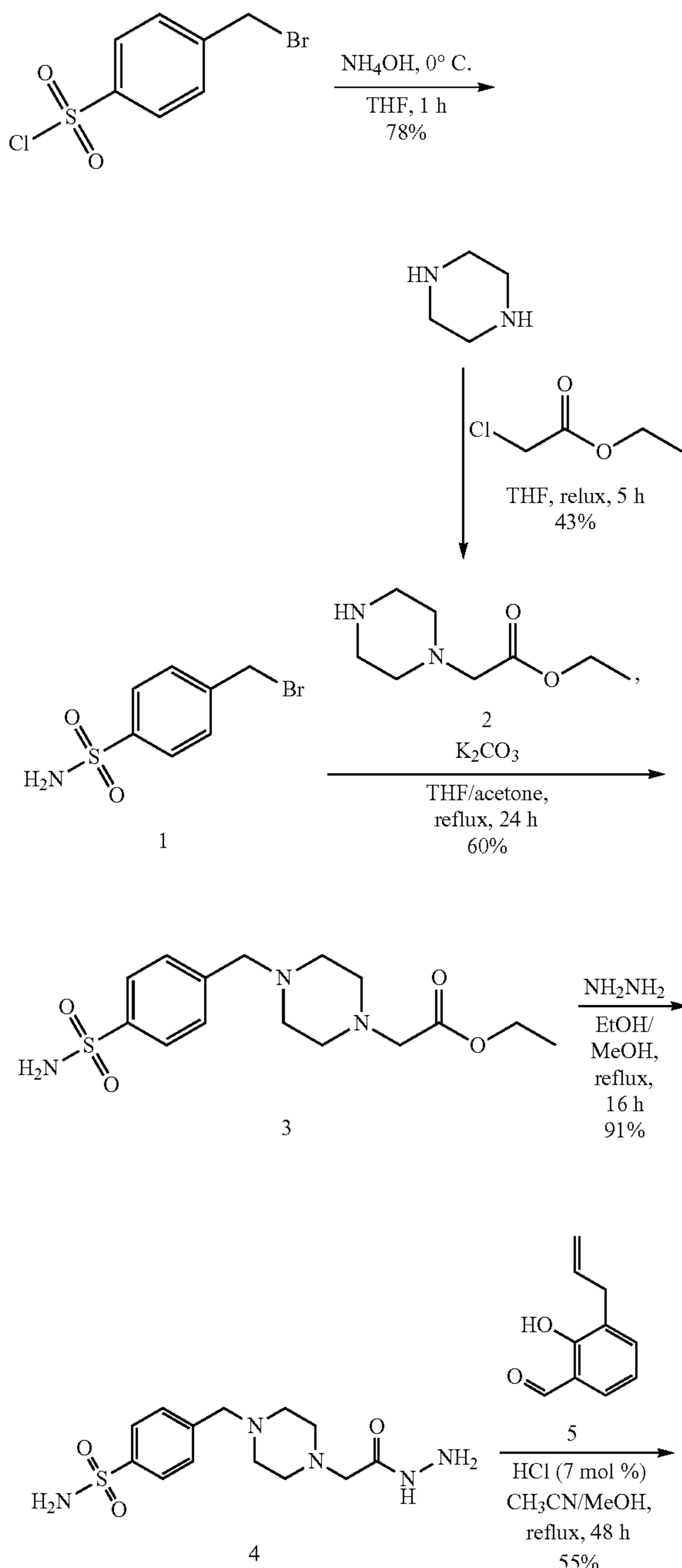
Scheme 8. Gram-scale synthesis of S-PAC-1.
