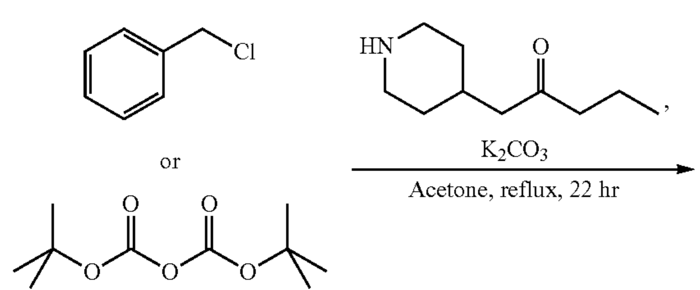
Scheme S3. Syntheses of 4a-b
