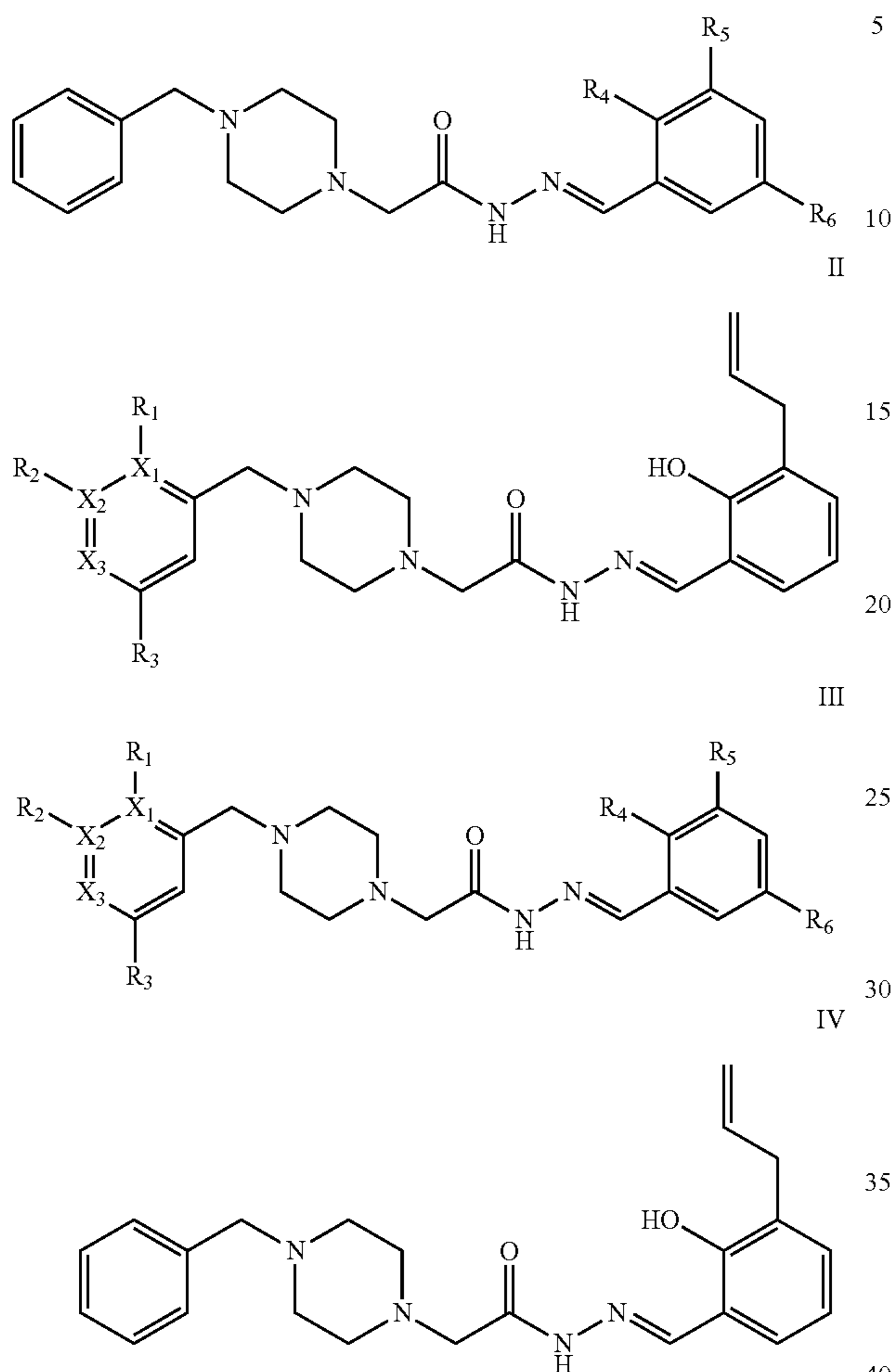
Scheme 2
