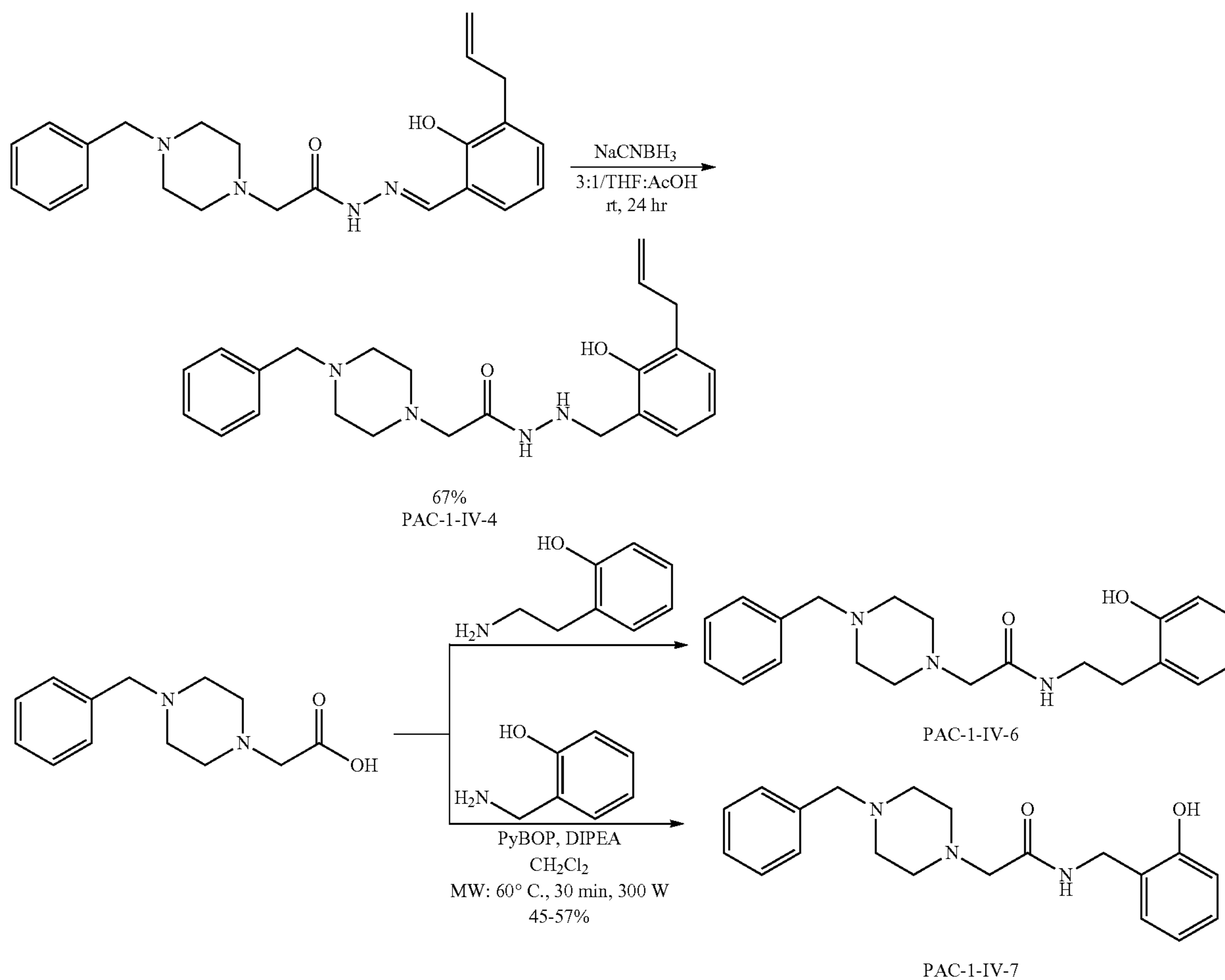
Scheme 4. Synthesis of class IV compounds.
