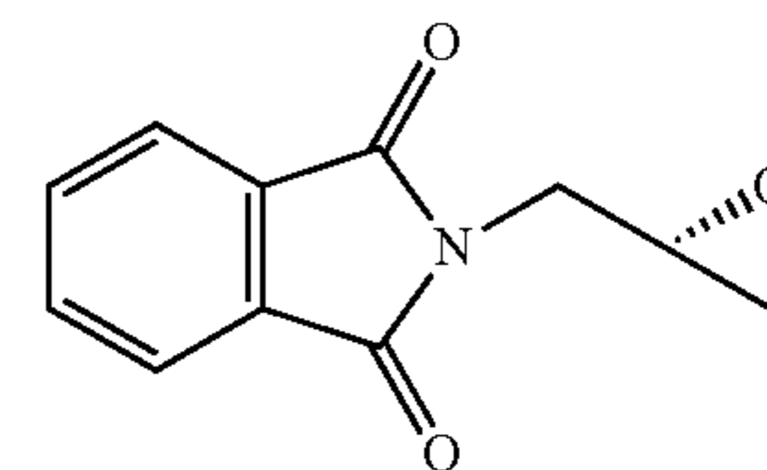
2-[(2S)-Oxiran-2-ylmethyl]-1H-isoindole-1,3(2H)-dione (I)
